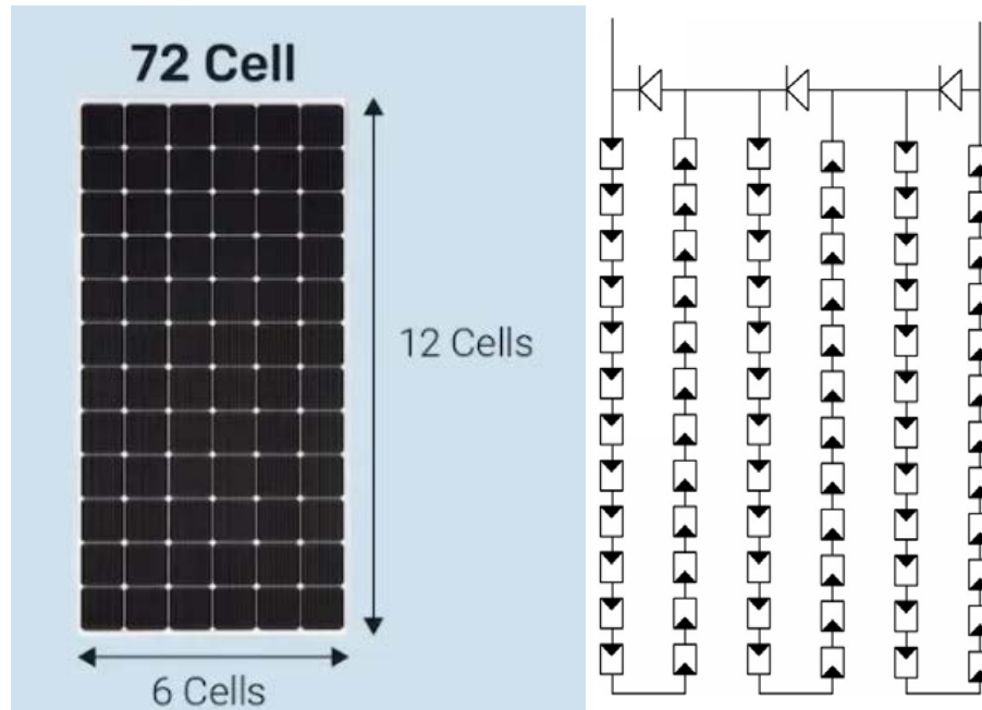
Figure 4. 72 cell
