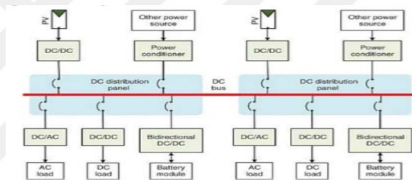
Figure 8. D C micro grid
