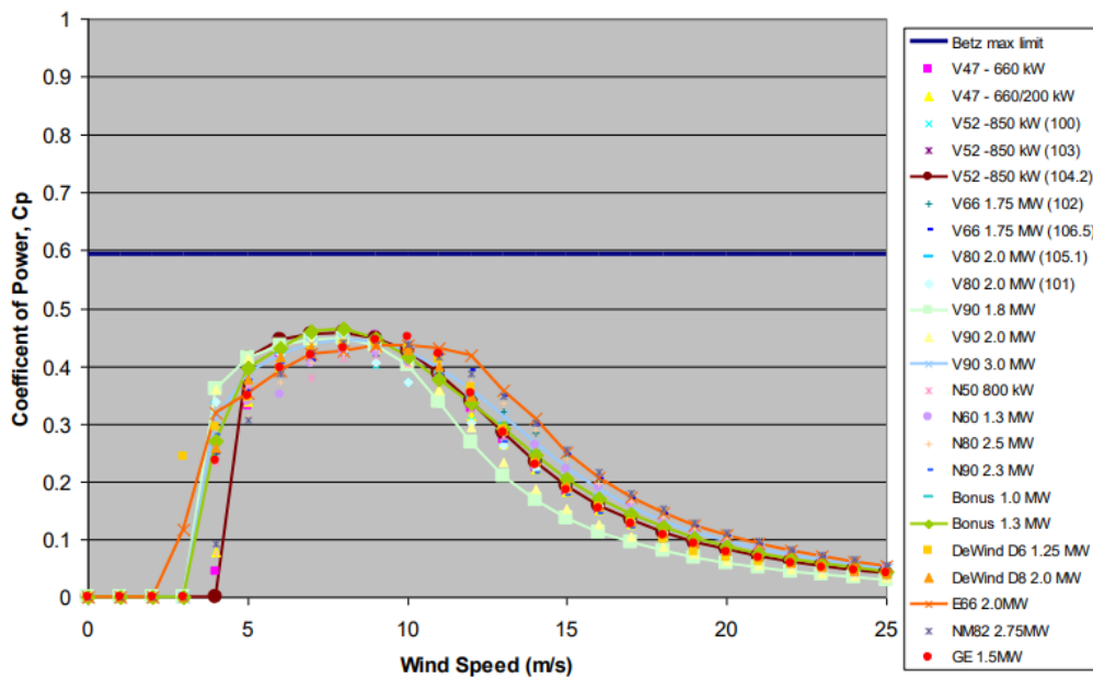
Figure 22. Coefficient power
