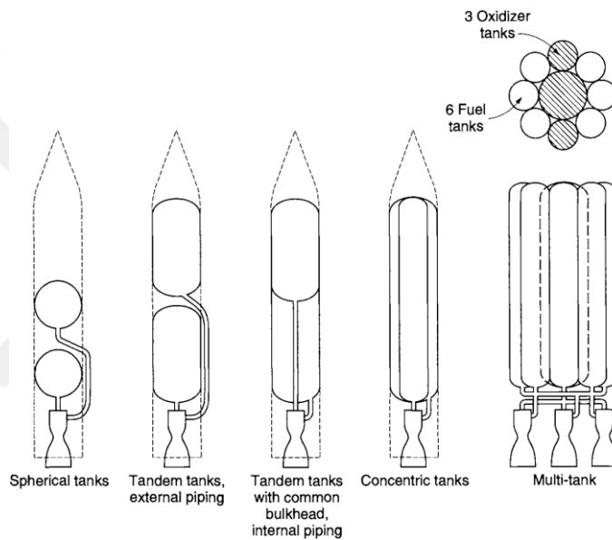
Figure 2.10 Common tank configurations for major liquid propellant rocket engines (Sutton & Oscar, Rocket Propulsion Elements, 2001) Reproduced with permission from John Wiley & Sons
