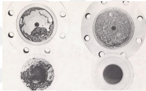
Figure 2.9 Corrosion on stainless steel caps and aluminum test tubes after 400-hour long storage of white fuming nitric acid at 77°C (Feiler & Morrell, 1952)
