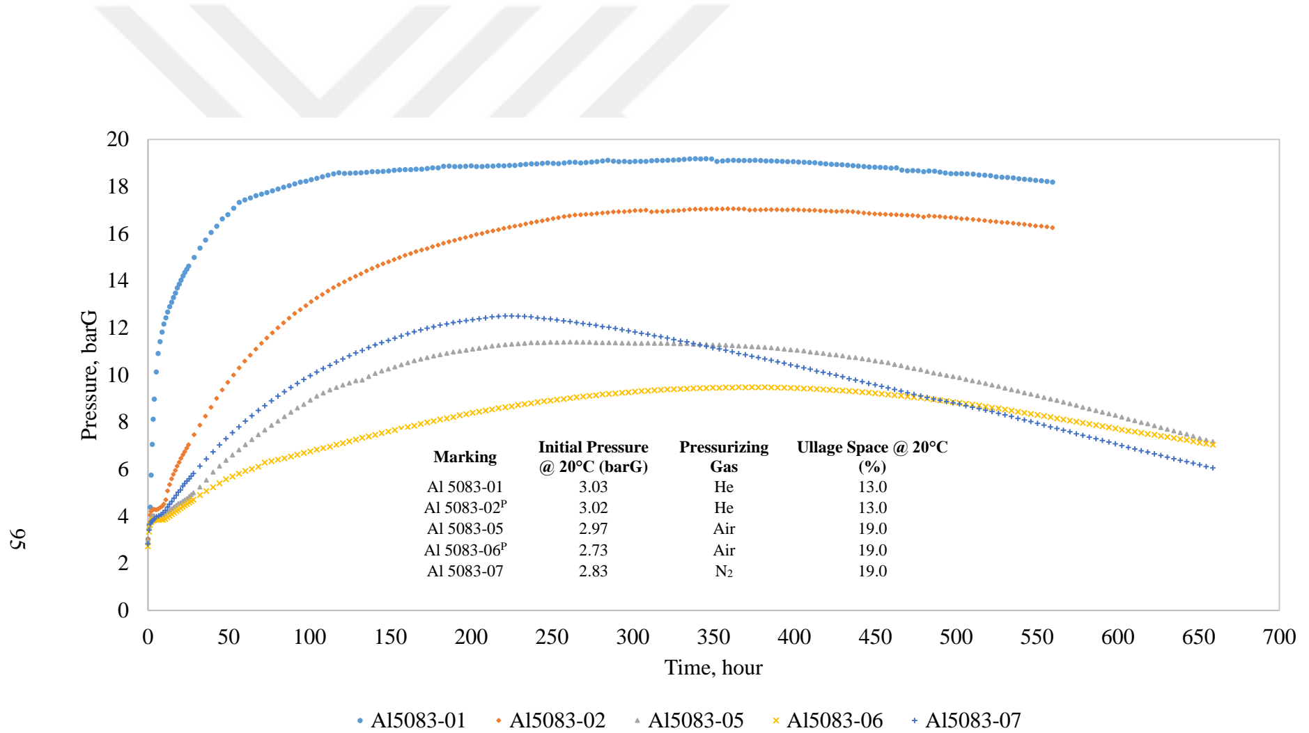
Figure 4.9 Time-dependent pressure data of WFNA stored in Al5083-H111 tubes @ 50°C
