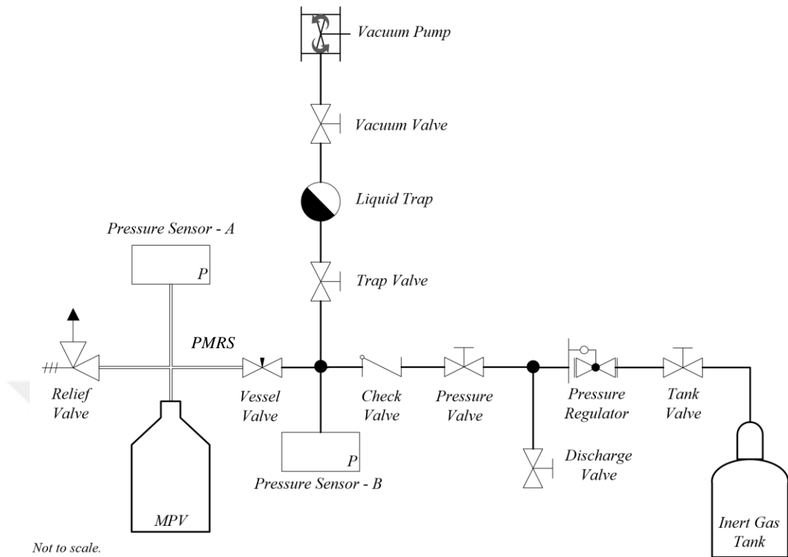
Figure 3.6 Schematic of Vacuum & Pressurization System (VPS) and Mini Pressure Vessel (MPV) fixture
