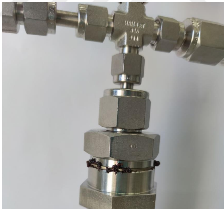
Figure 4.6 Leak through MPV body and PMRS connection occurred during with the PTFE-04 tube storage
