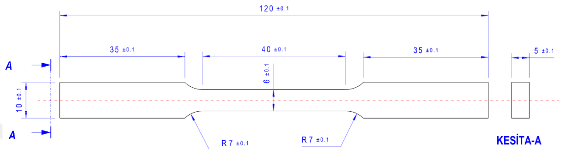
Figure D.1 Tensile test specimen according to ASTM designation E8/E8M – 16
