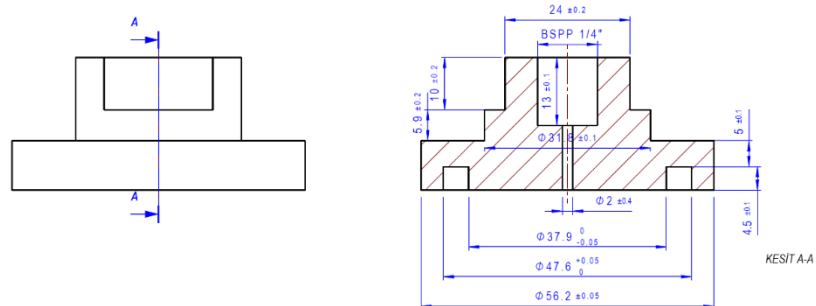
Figure A.10 Sealing cap component's detailed engineering drawing
