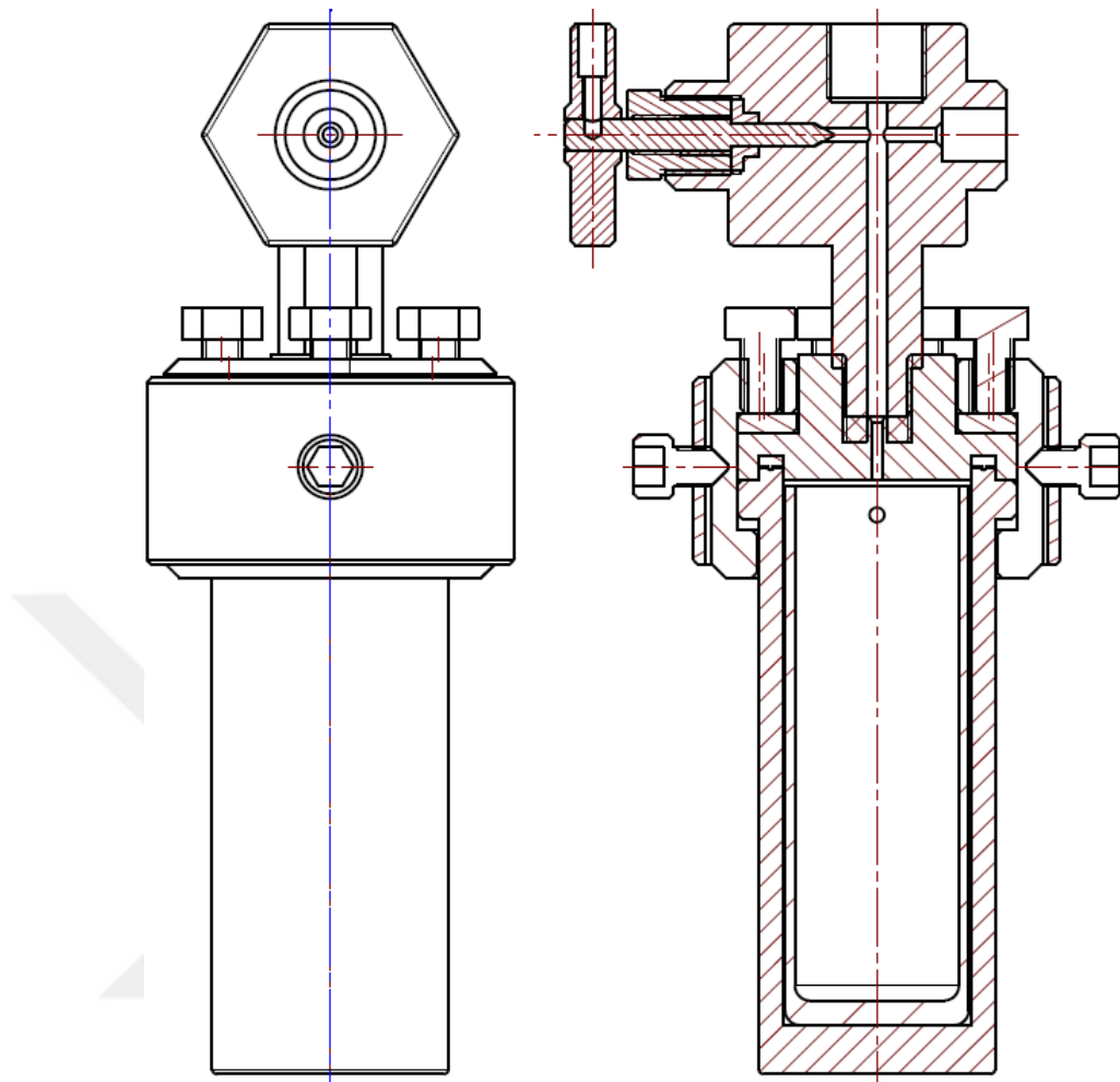
Figure 3.1 Detailed engineering section view of the first test set-up prototype
