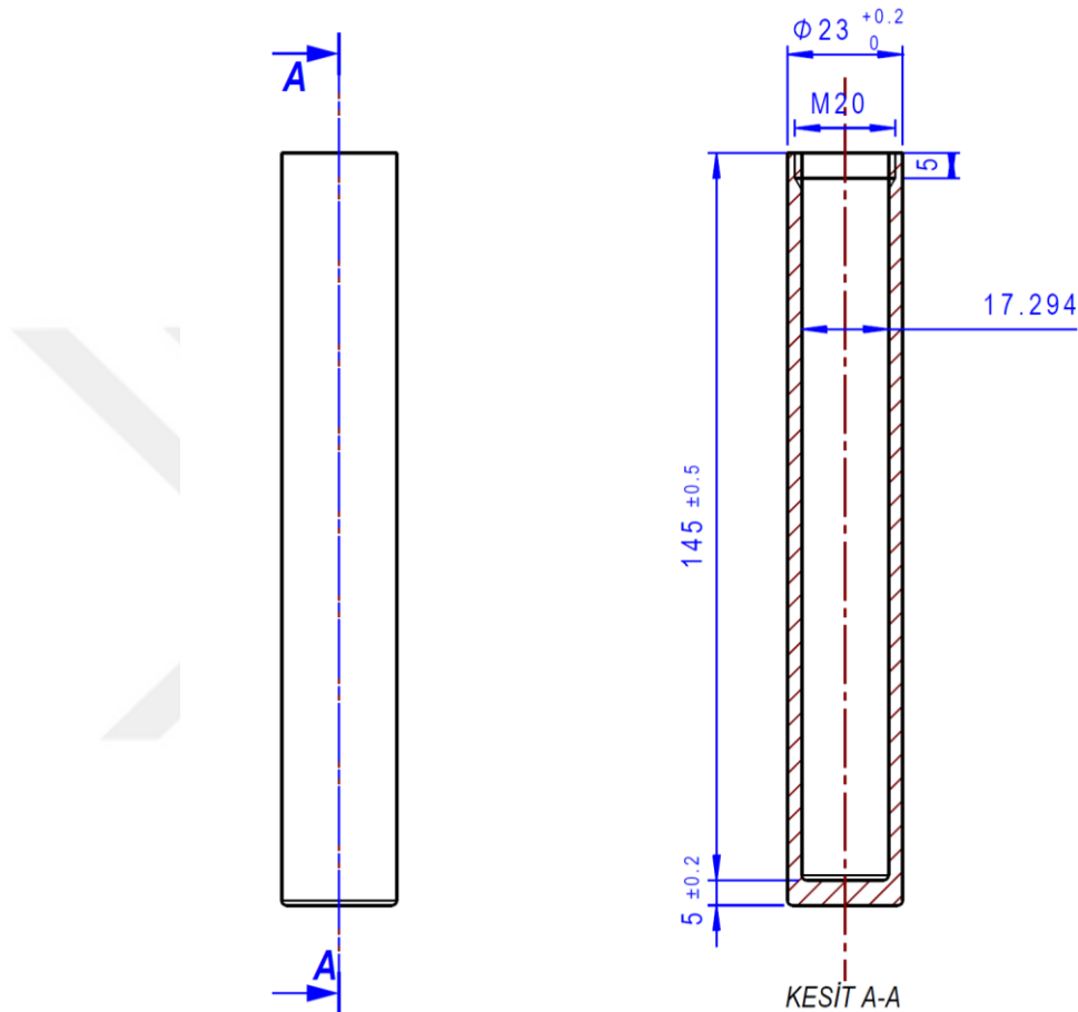
Figure B.3 Mini test tube component's detailed engineering drawing
