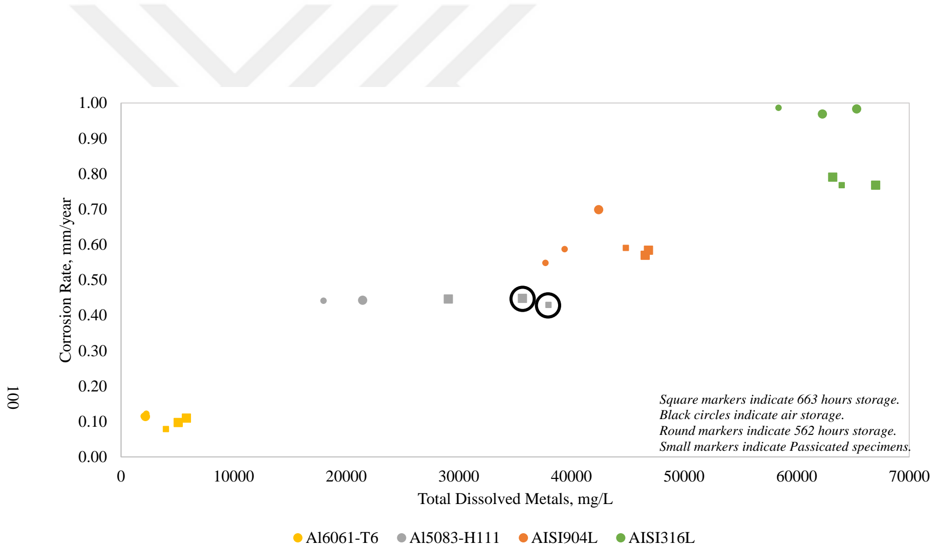
Figure 4.12 Variation of corrosion rate (mm/year) in metal tubes as function of total dissolved metal concentration (mg/L)
