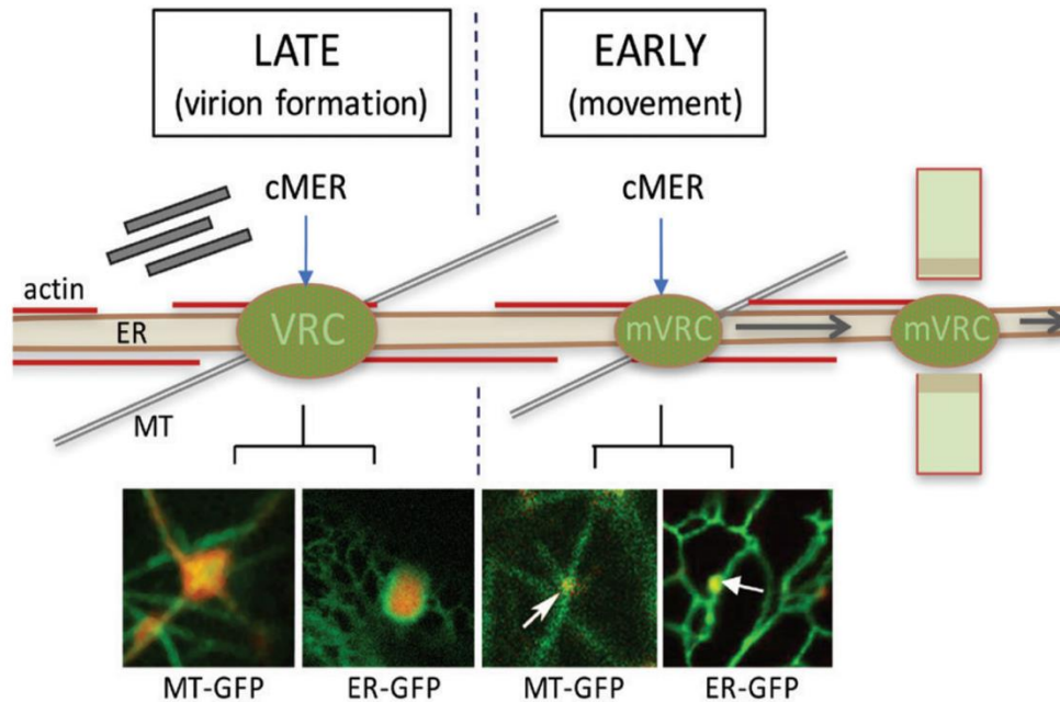
Figure 2.7. Targeting of viral replication complex (VRCs) to the cortical microtubule-associated ER sites during late and early TMV infection. At early infection, VRC are mobile (mobile VRC or mVRC) along the MT tracks till it can be detached at intersections of the cortical MT with ER-actin system, or the cortical microtubule-ER associated sites (cMER), to move along the ER-actin system through PD. At late infection stages, MT are involved in the subsequent degradation of the MP and the anchoring of large VRC, or X-body (Image from Pitzalis N and Heinlein M, 2018).
