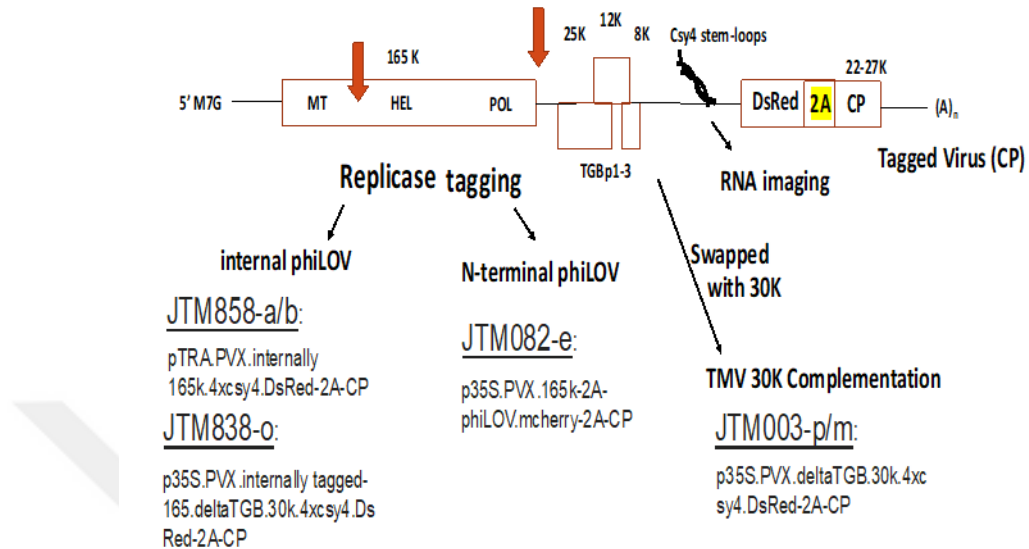
Figure 3.2. Schematic representation of all plasmid constructs used in that research
