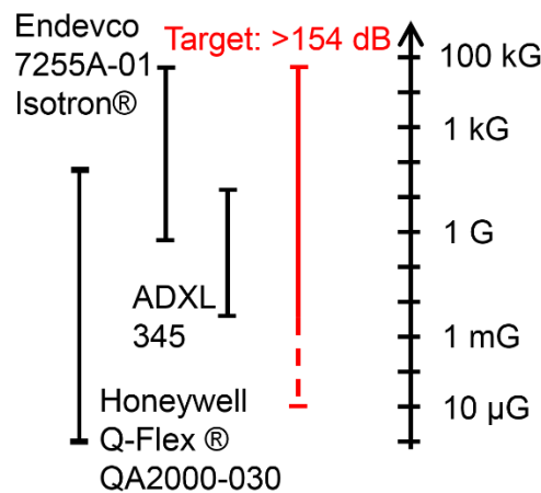
Figure 1.3. Acceleration range covered by different accelerometer models.
