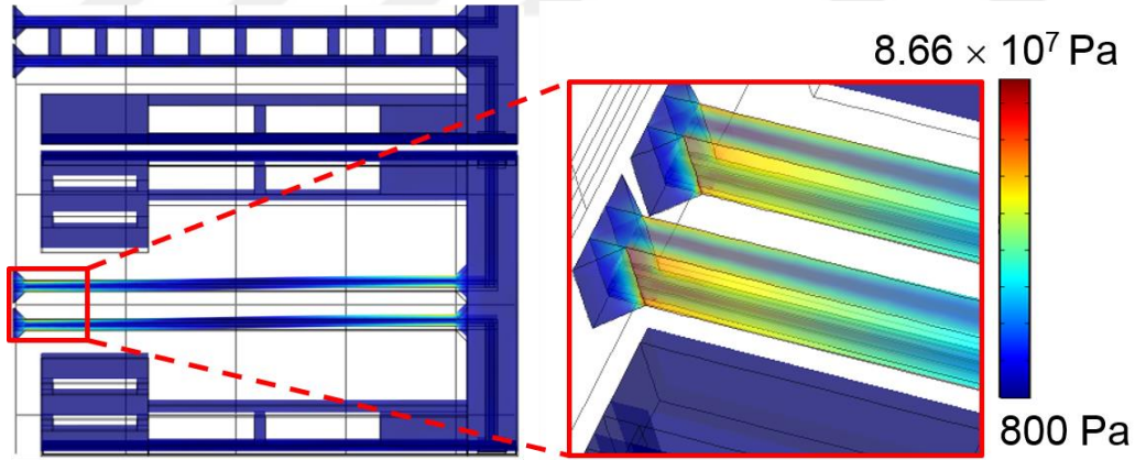
Figure 2.5. Finite-element analysis of von-Mises stress at the flexure anchors under 50 kG acceleration.
