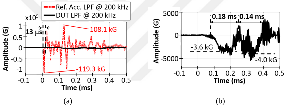
Figure 5.11. (a) Reference accelerometer output from sled impact of more than 100 kG amplitude and 13 \mu s duration followed by lower amplitude oscillations. (b) Corresponding DUT accelerometer output with an expanded y-axis scale.
