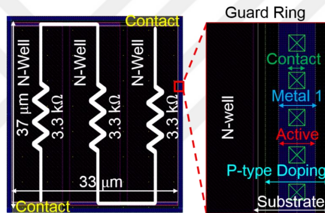
Figure 4.12. N-well resistor layout for n-type piezoresistive stress sensors.
