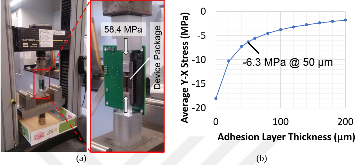
Figure 4.16. (a) Instron stress test setup for the sensitivity characterization of the piezoresistive stress sensors. (b) The transferred stress from the package to the substrate surface as a function of adhesion layer thickness.
