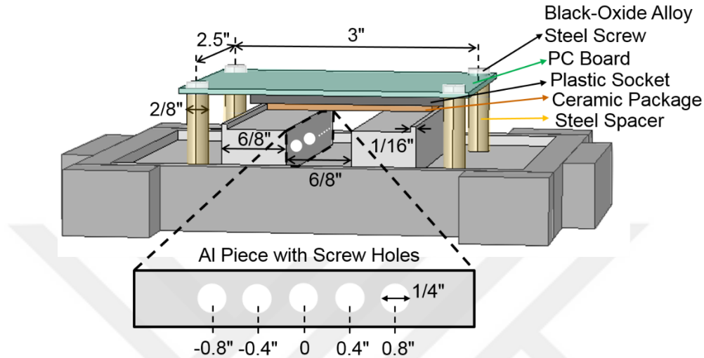
Figure 5.9. Printed-circuit board mounting on the sled of the split Hopkinson bar test setup.
