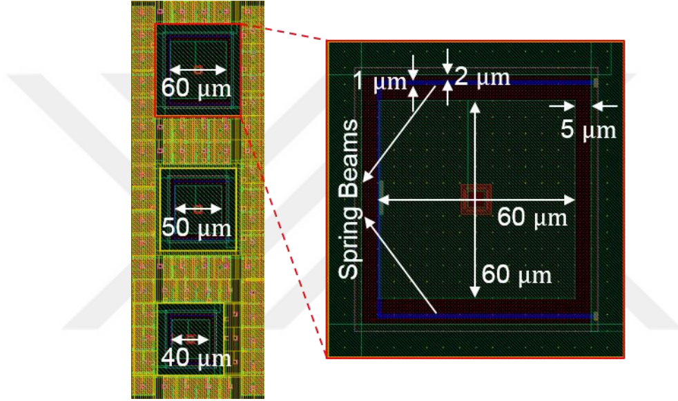
Figure 3.5. Release-test structures used for informing 20 \mu\text{m} , 25 \mu\text{m} and 30 \mu\text{m} undercut length.
