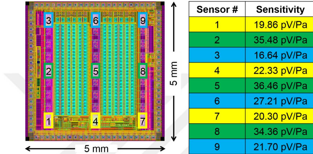
Figure 4.19. The measured sensitivity of n-type piezoresistive normal stress sensors at different sensor areas in the second-generation accelerometer system (without taking any stress attenuation into account).
