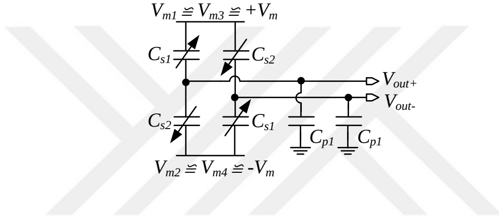
Figure 2.15. Simplified differential capacitive bridge model of the accelerometer array.
