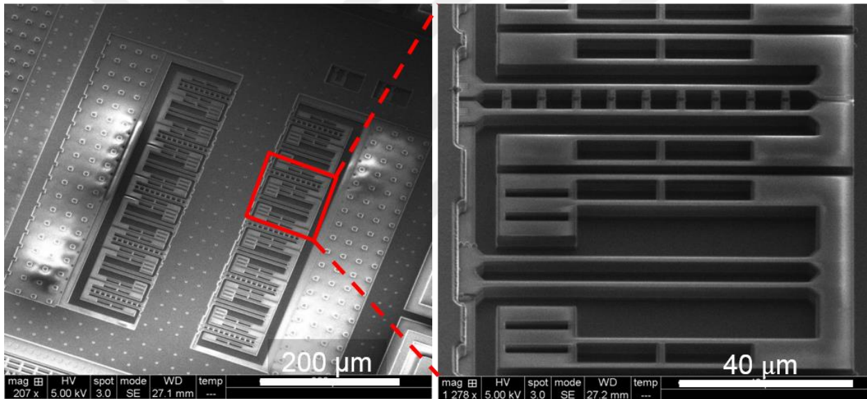
Figure 3.8. Accelerometer cell after etching the metal-4 CMOS layer with chlorine-based dry aluminum etch.
