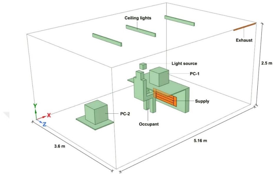
Figure 4.7. CFD model geometry created for simulating the experiments of Loomans (1998)
