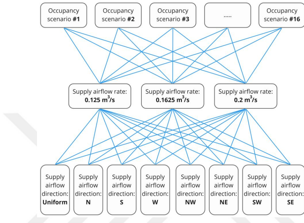
Figure 4.12. Variable combinations for simulation scenarios
