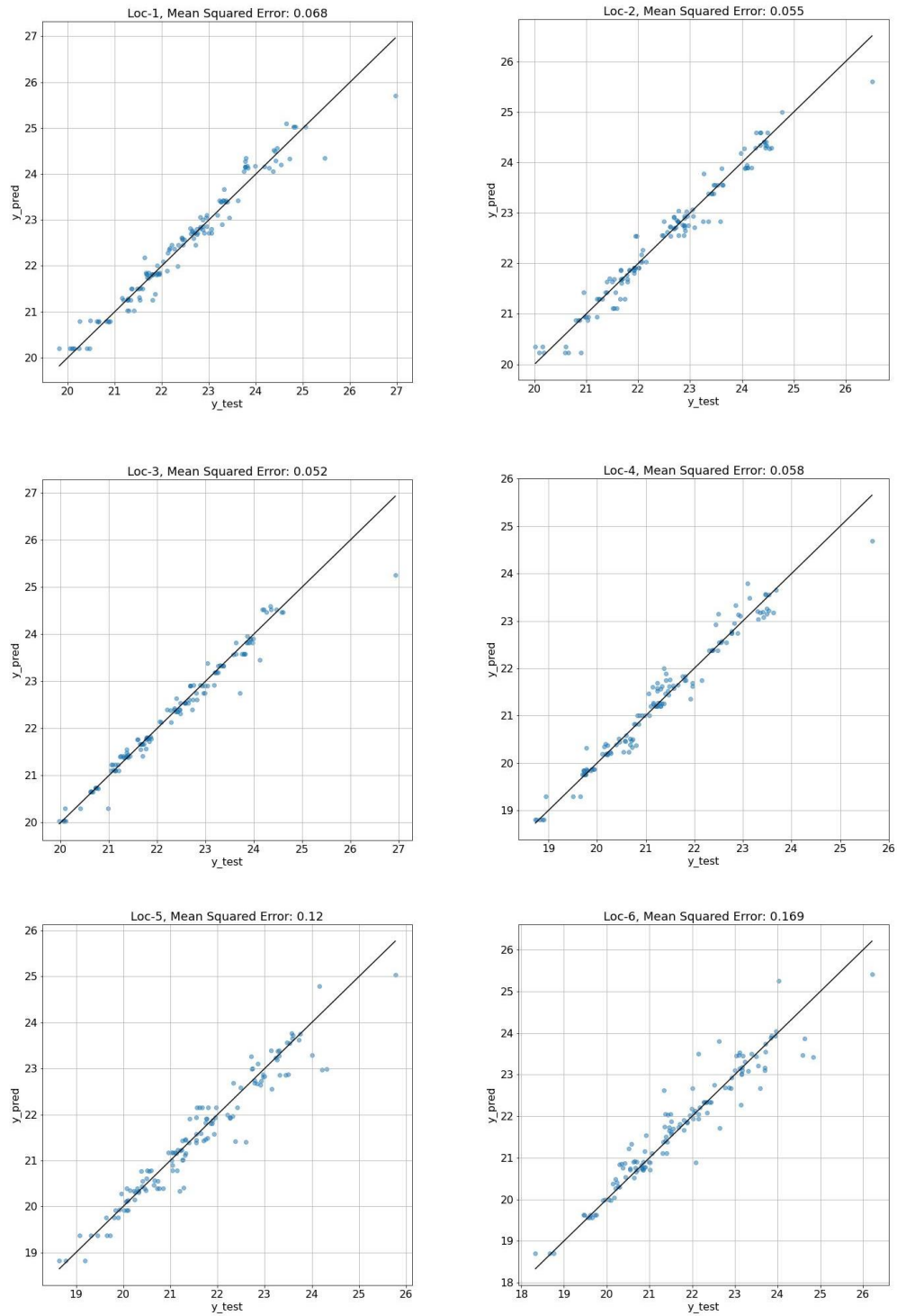
Figure 4.23. Predictive performance of Random Forest models, developed for each occupant location
