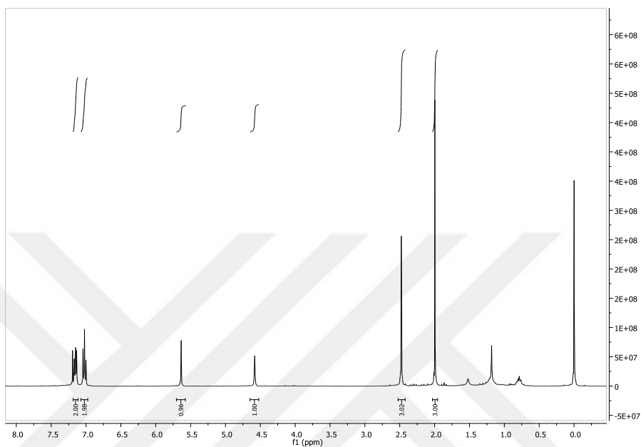
Figure 0.17. ^1\text{H} NMR Spectrum of (36ha)
