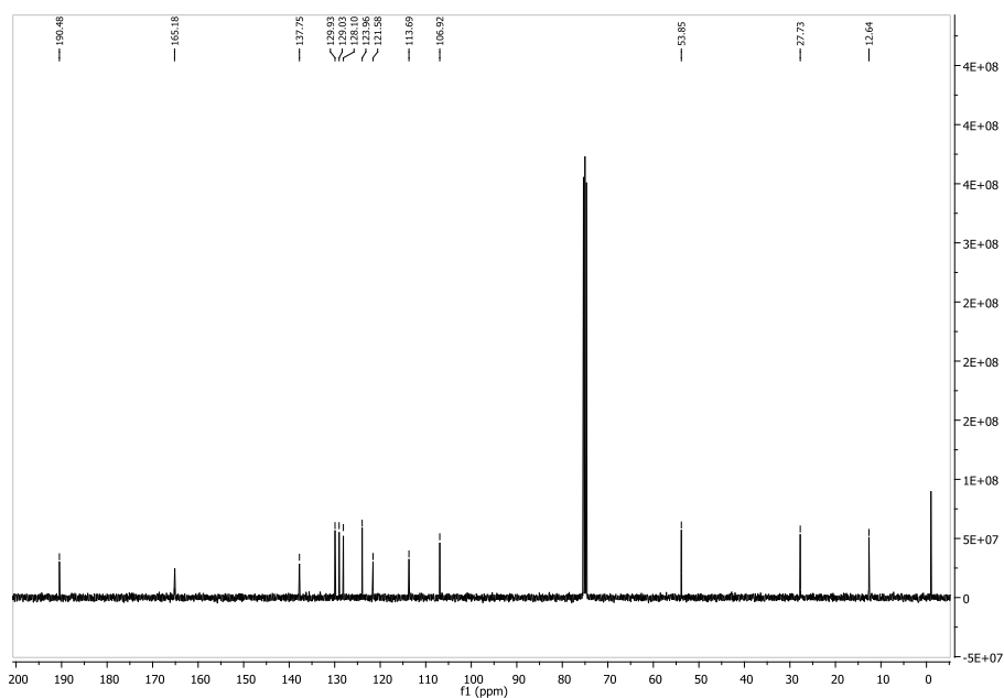
Figure 0.8. 13 C NMR Spectrum of (36ca)
