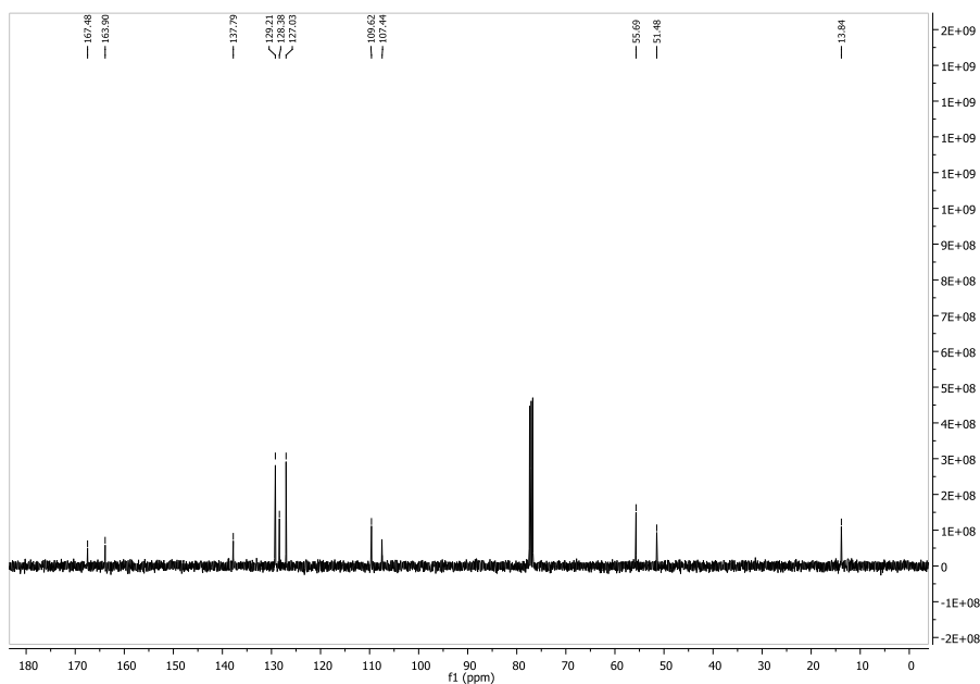
Figure 0.28. 13 C NMR Spectrum of (36ad)
