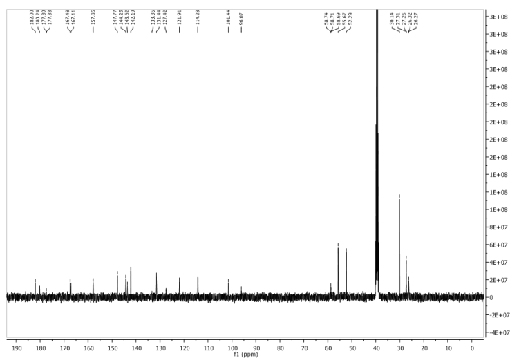
Figure 0.2. ^{13}\text{C} NMR Spectrum of Quinine / t -butyl Squaramide (20)
