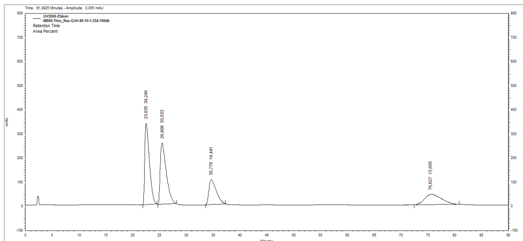
Figure 0.49. HPLC Chromatogram of racemic (36ja)
