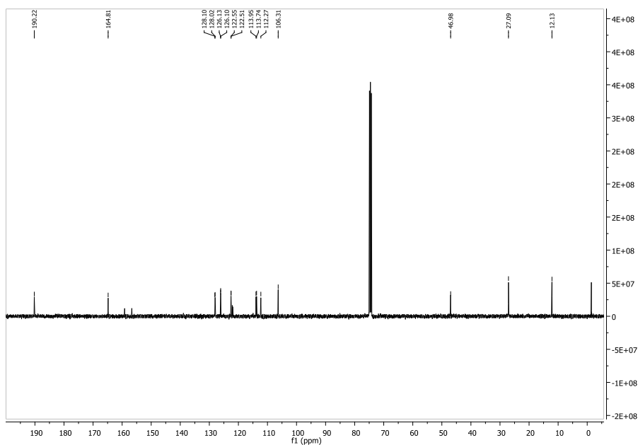
Figure 0.6. 13 C NMR Spectrum of (36ba)
