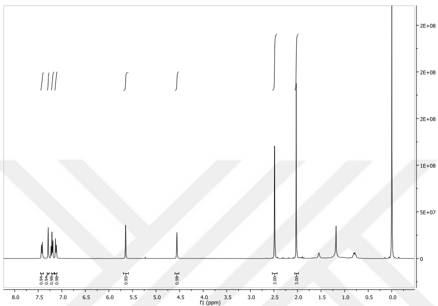
Figure 0.7. 1 H NMR Spectrum of (36ca)
