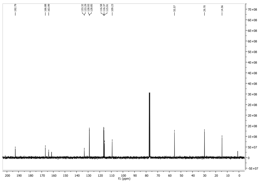
Figure 0.18. ^{13}\text{C} NMR Spectrum of (36ha)
