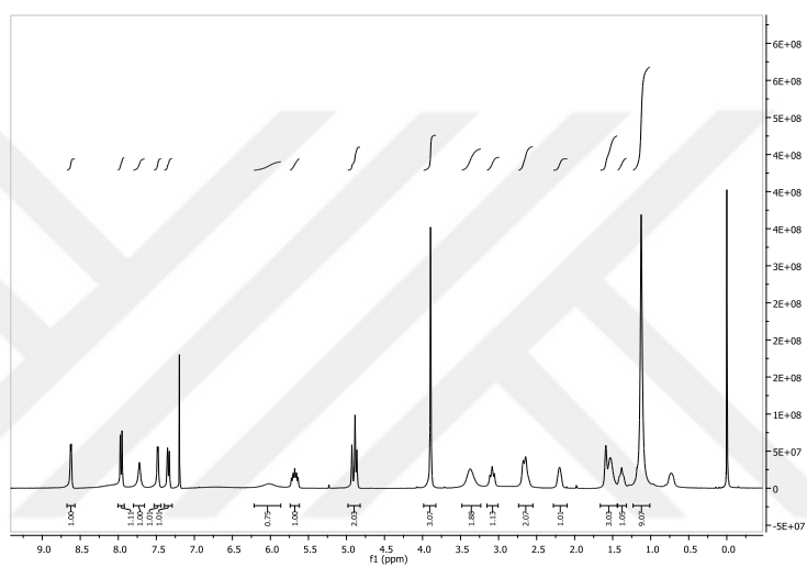
Figure 0.1. ^1\text{H} NMR Spectrum of Quinine / t -butyl Squaramide (20)
