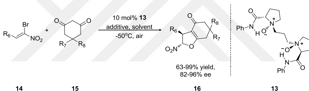
Figure 1.14. Michael-S N 2 Type Alkylation Reaction via N,N' -dioxide Derived Bifunctional Organocatalyst
