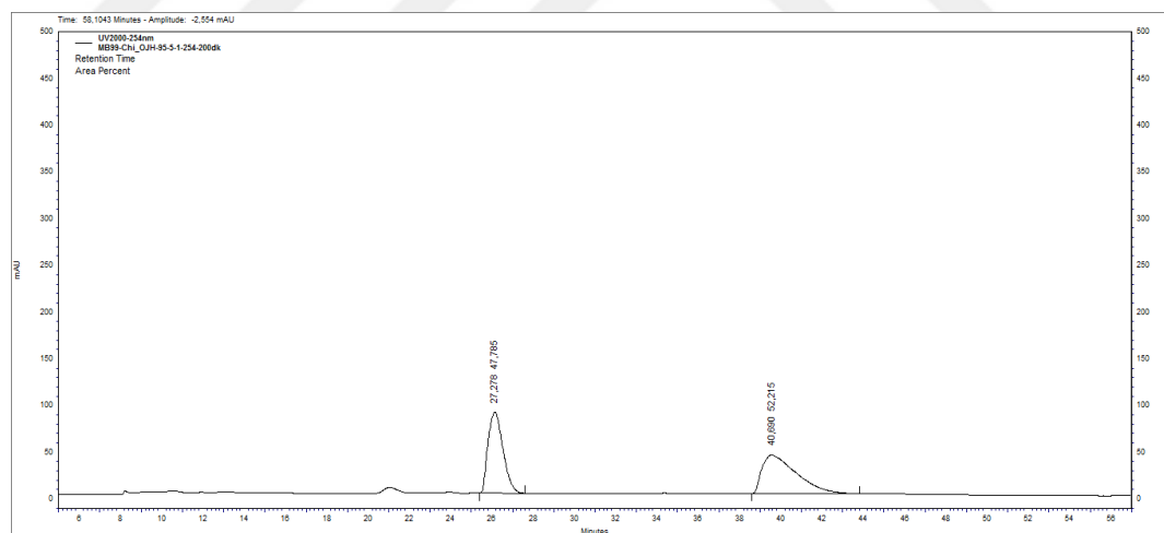
Figure 0.52. HPLC Chromatogram of chiral (36ab)
