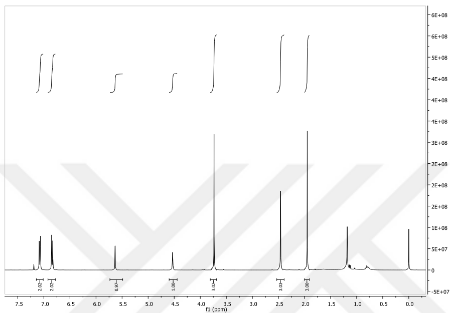
Figure 0.11. ^1\text{H} NMR Spectrum of (36ea)
