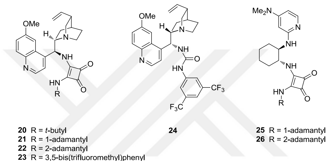
Figure 1.17. Bifunctional Organocatalysts 20 – 26
