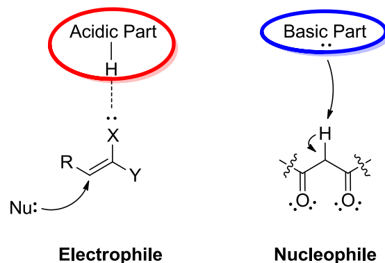
Figure 1.7. Interaction of Bifunctional Organocatalyst and Substrates
