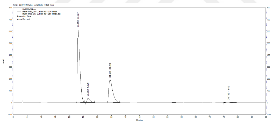
Figure 0.50. HPLC Chromatogram of chiral (36ja)
