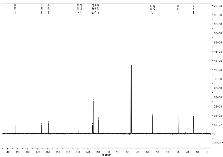
Figure 0.12. ^{13}\text{C} NMR Spectrum of (36ea)
