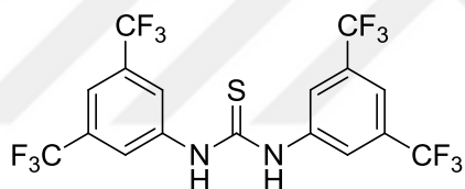
Figure 1.8. Schreiner Thiourea Catalyst
