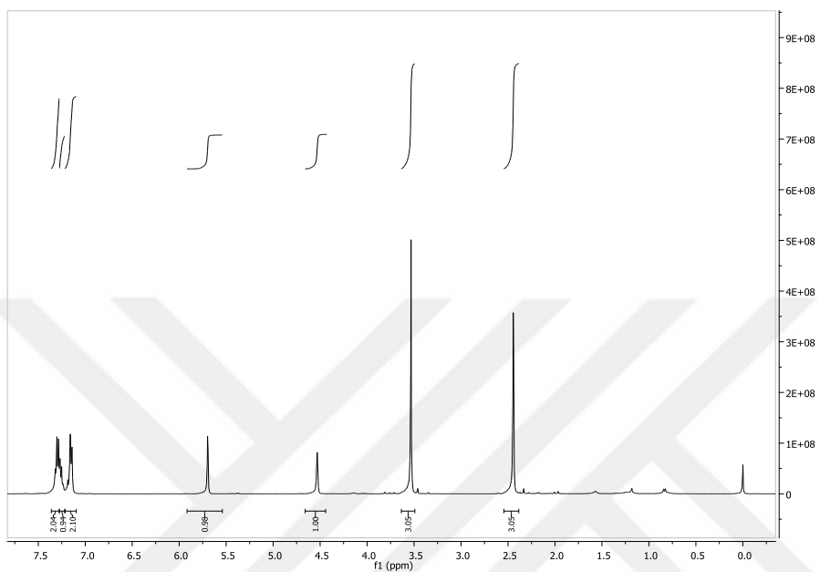
Figure 0.27. 1 H NMR Spectrum of (36ad)
