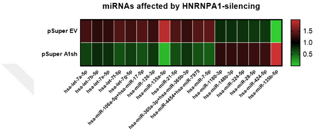
Figure 3.2. Heatmap results of selected miRNAs.
