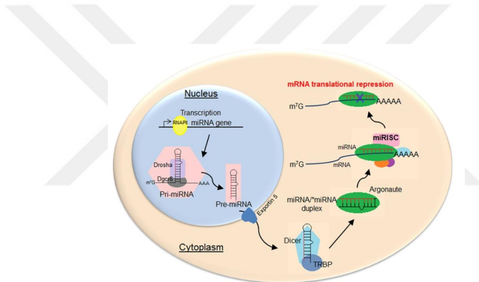
Figure 1.3. Overview of miRNA biogenesis and function.
