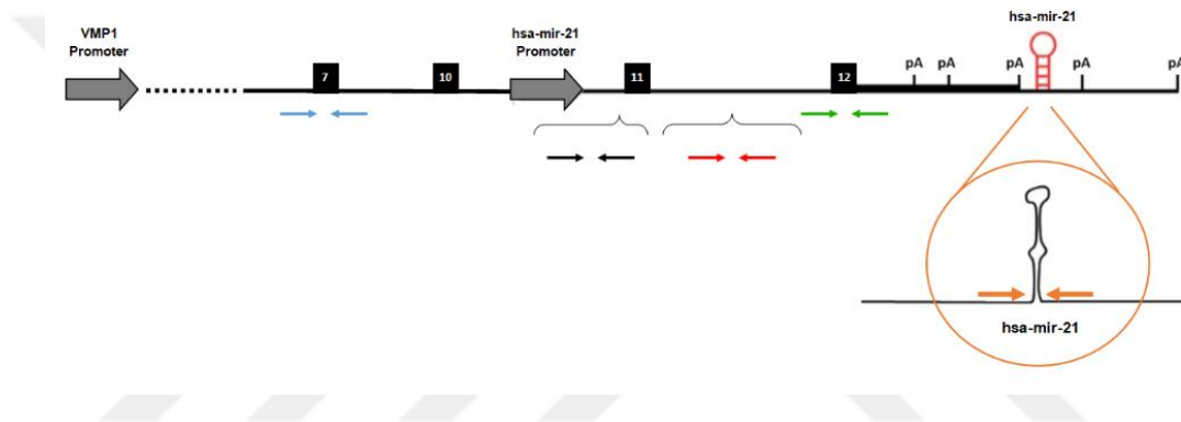
Figure 3.7. Overview of VMP1 and mir-21 locus.
