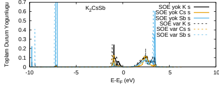
(a) K_2CsSb-s
