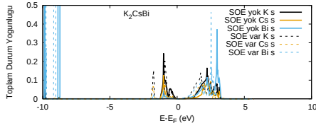
(a) K_2CsBi-s
