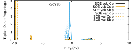
(b) K_2CsSb-p
