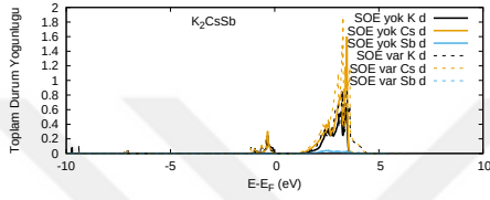
(c) K_2CsSb-d
