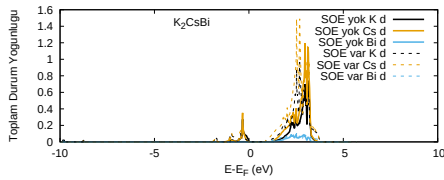
(c) K_2CsBi-d
