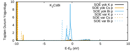
(b) K_2CsBi-p
