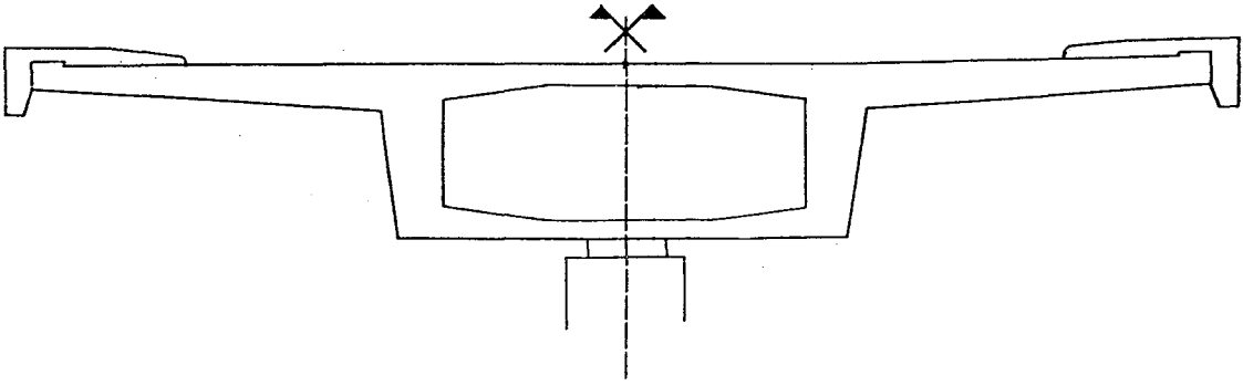
FIGURE 3.2 Typical cross-section of post tensioned continuous plate girder.
