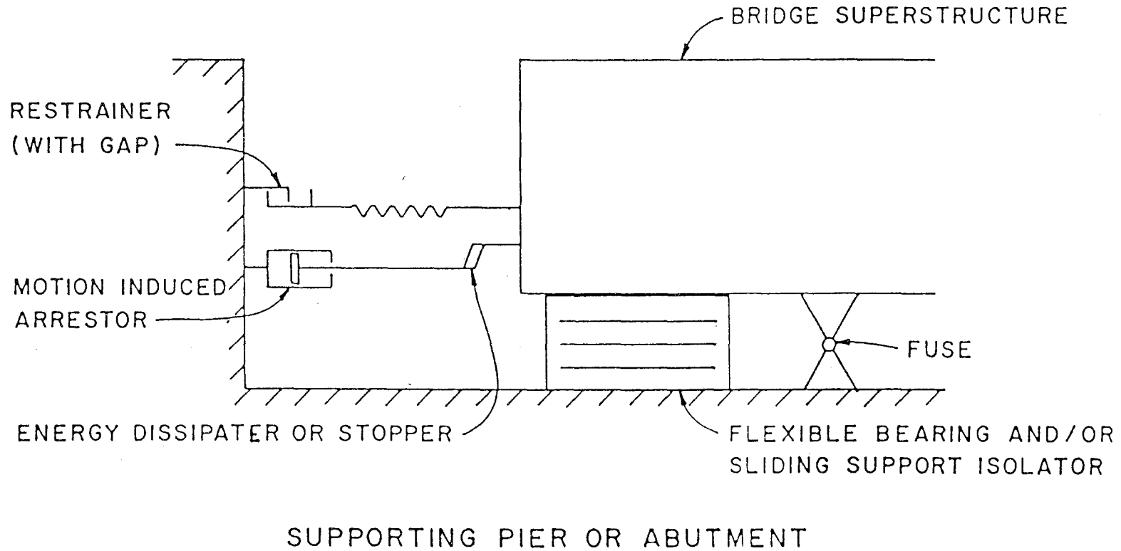
FIGURE G.13 An ideal bearing device (ATC, 1983).
