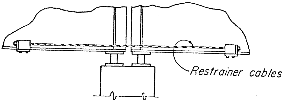
FIGURE G.5 Restrainer at pier-no positive tie to pier (ATC, 1983).
