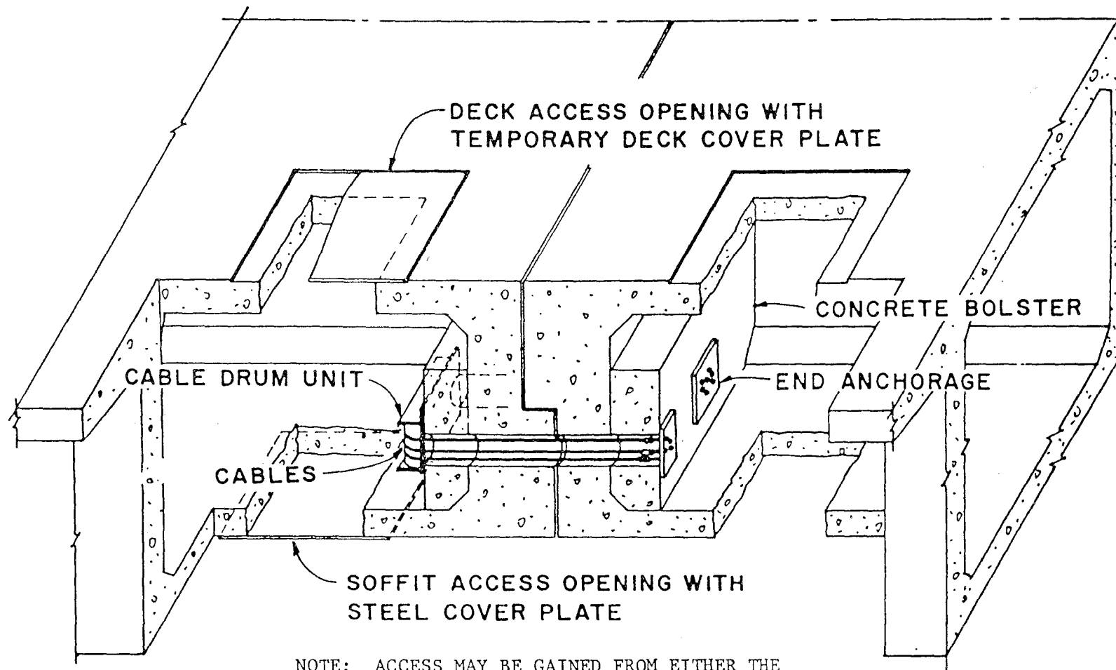
FIGURE G.6 Longitudinal joint restrainer for concrete box girder (ATC, 1983).
