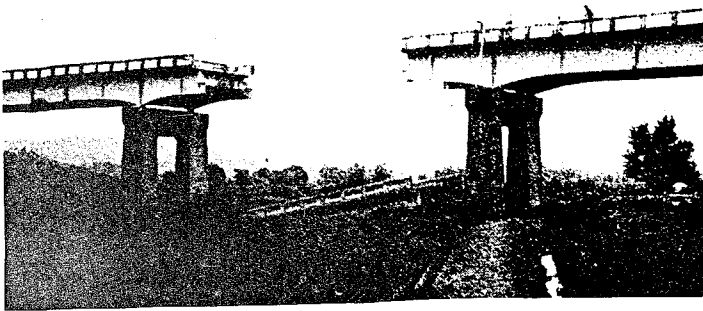
PHOTO B.4 Kin-noh Bridge, fall of suspended girder beam. (Miyagi-ken-oki Earthquake of June 12, 1978), ATC (1979).
