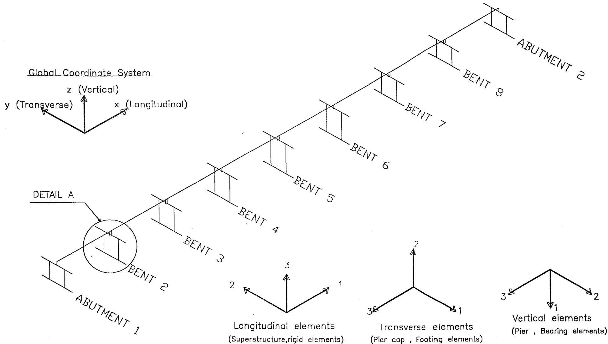
FIGURE 3.15(contd.) The frame element model of the K1 bridge
