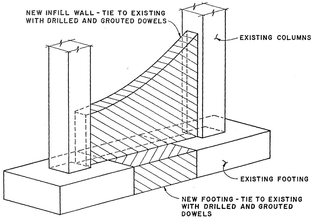
FIGURE G.23 Infill shear wall retrofit (ATC, 1983).
