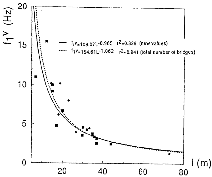
FIGURE 4.7 Experimental values of fundamental vertical frequency ( f_1^v ) versus length of the span, (Karabinis, 1995).
