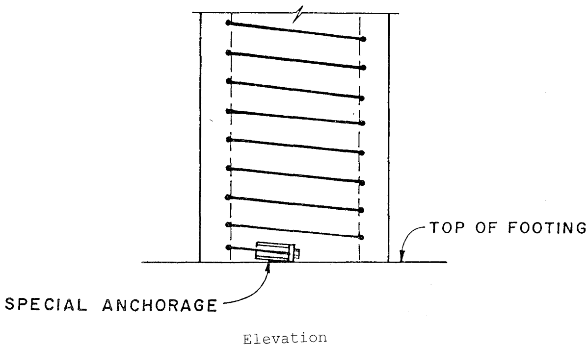
FIGURE G.17 Column retrofit to increase confinement with prestress wire (ATC, 1983).
