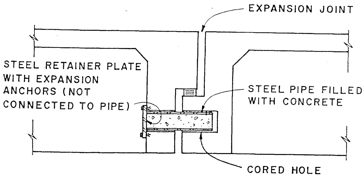
FIGURE G.8 Transverse restrainer retrofit for concrete bridge (ATC, 1983).
