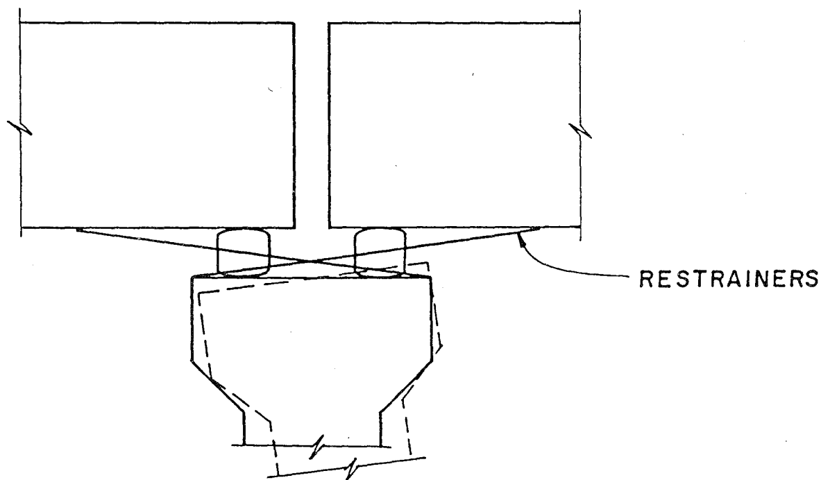
FIGURE G.29 Effects of restrainers at bent during liquefaction failure (ATC, 1983).
