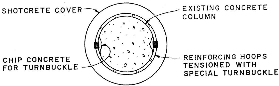
Cross-section
