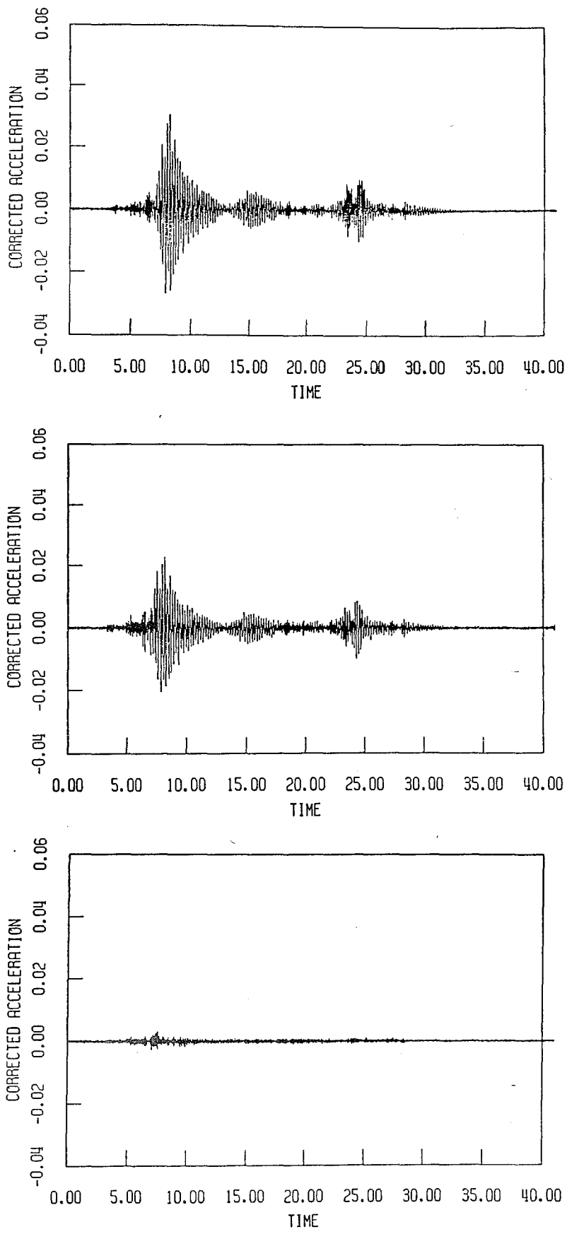
FIGURE 4.3 Corrected acceleration-time histories of test 3 for channel 3, 1 and 5 respectively.
