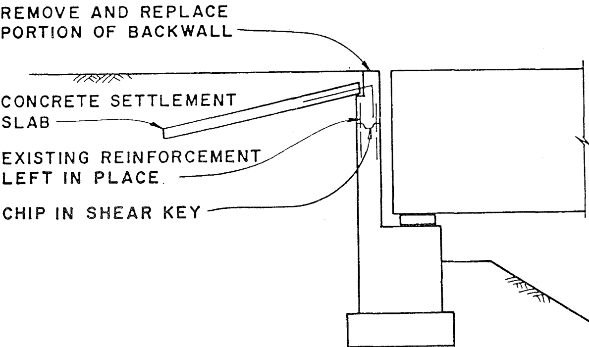
FIGURE G.26 Settlement slab-New Zealand style (ATC, 1983).
