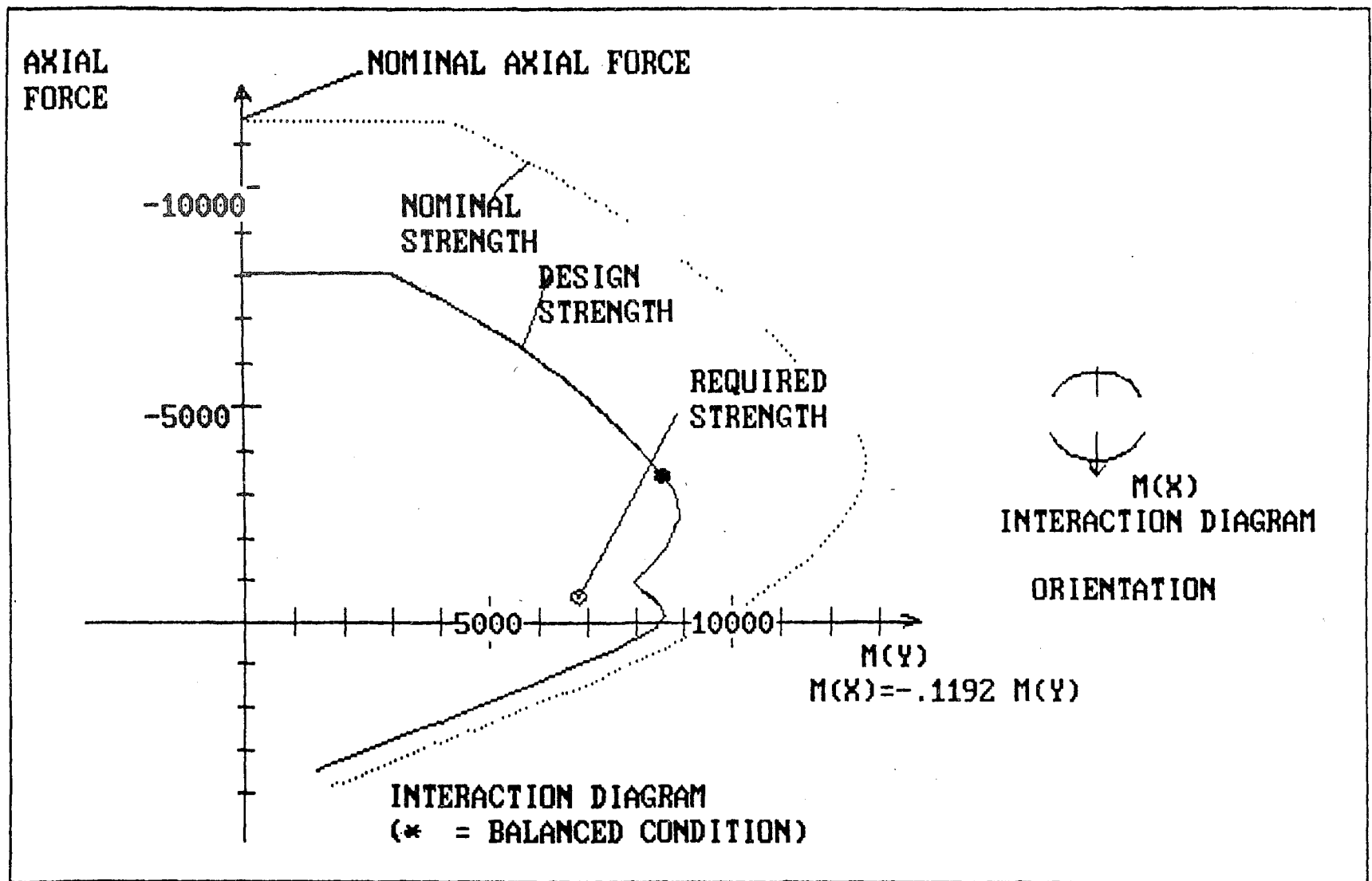
FIGURE 3.19 Interaction diagram of the K1 bridge.
