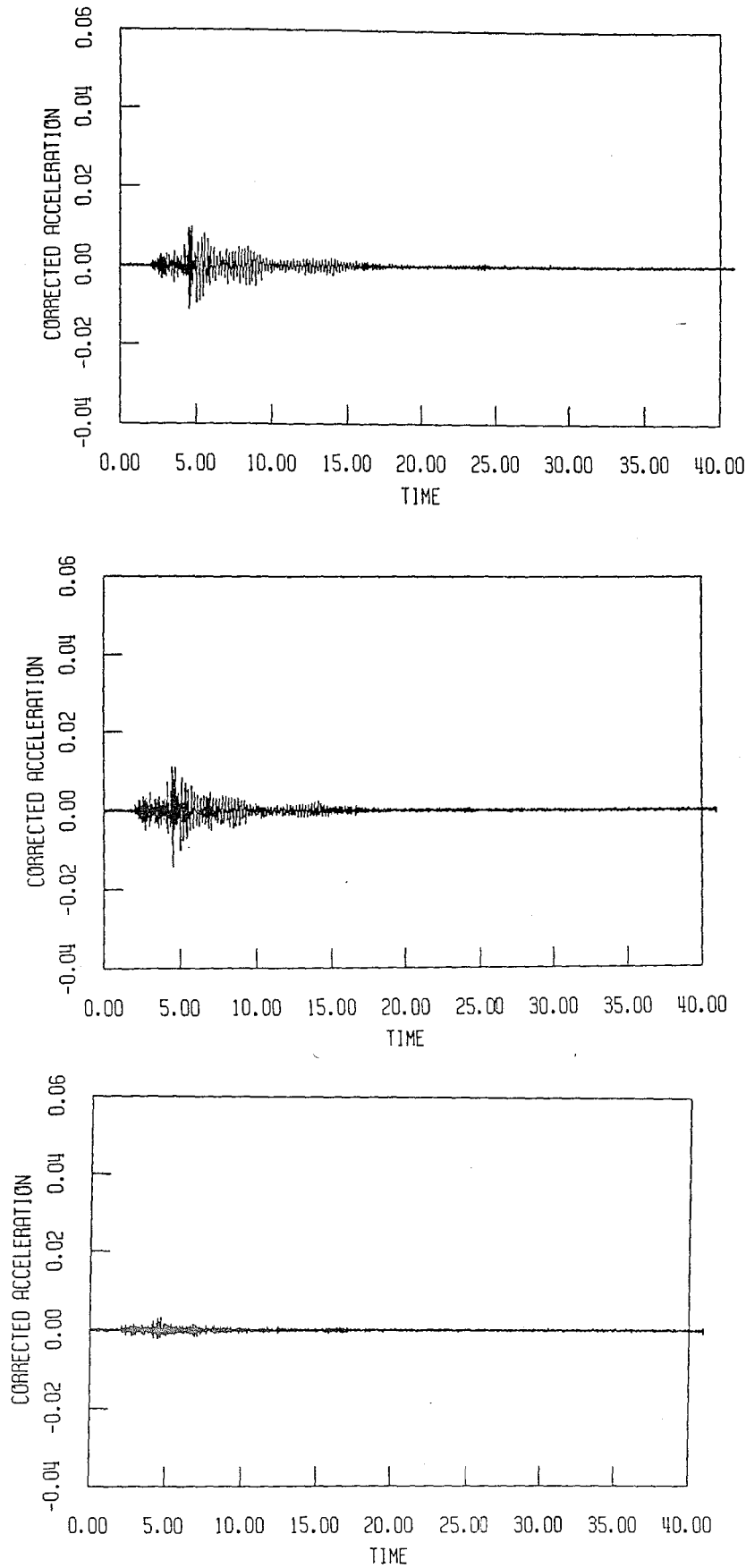
FIGURE 4.4 Corrected acceleration-time histories of test 5 for channel 3, 1 and 5 respectively.
