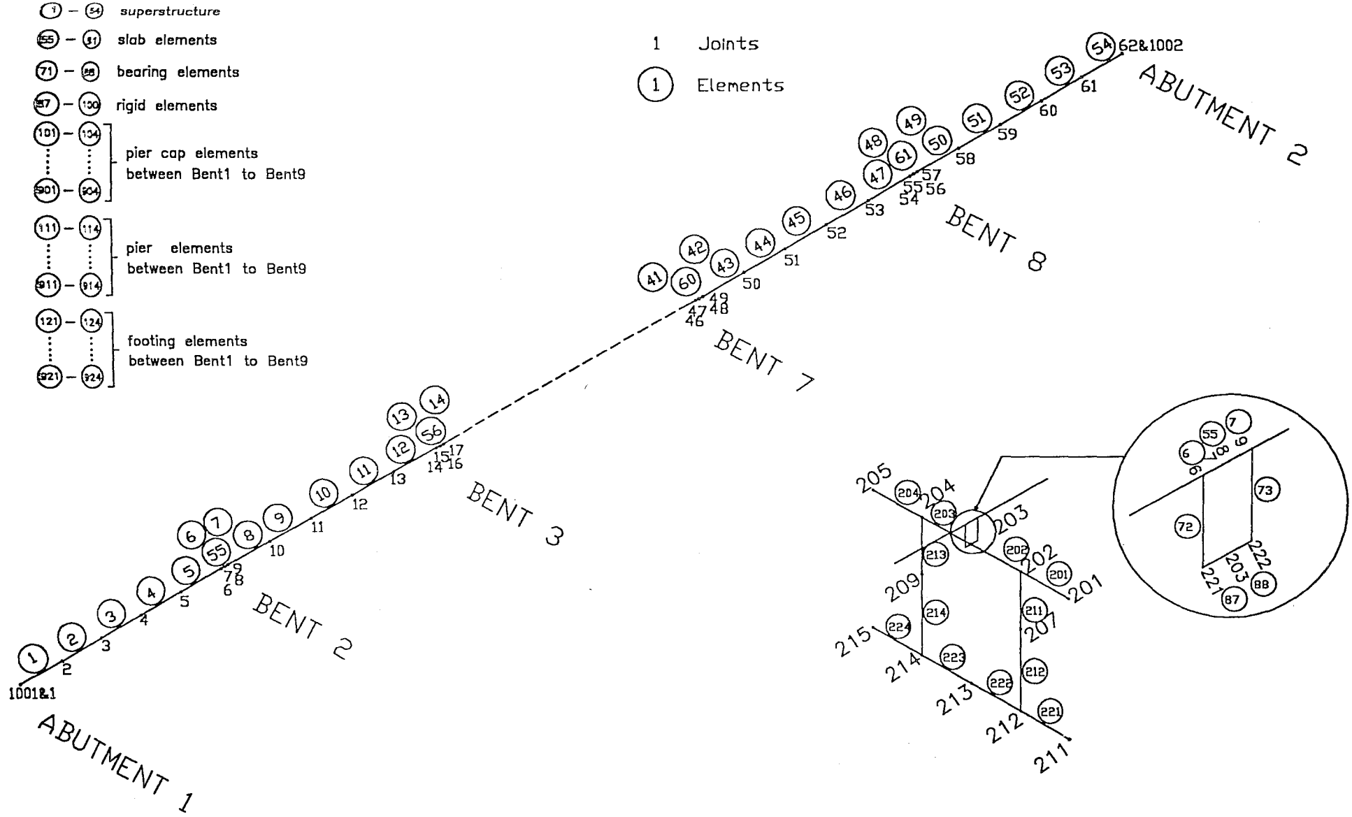
Joint And Element Identification in Superstructure FIGURE 3.15 The frame element model of the K1 bridge. DETAIL A
