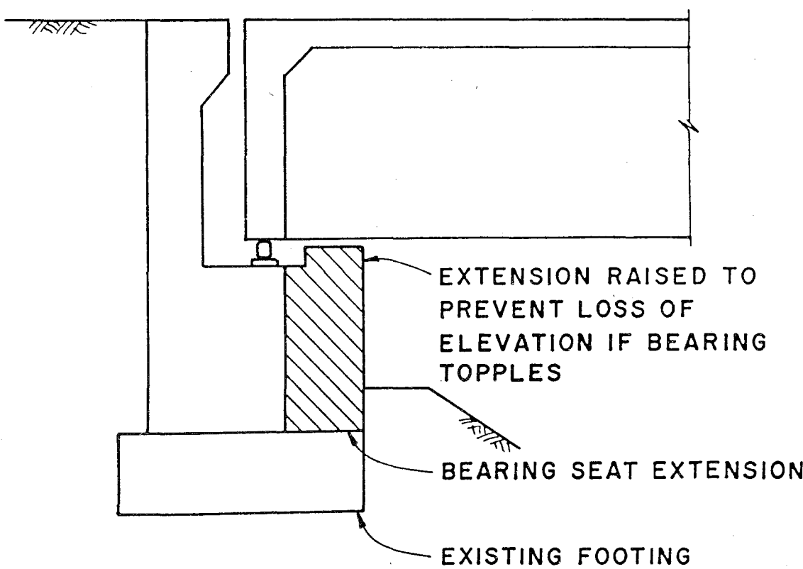
FIGURE G.10 Bearing seat extension at abutment (ATC, 1983).
