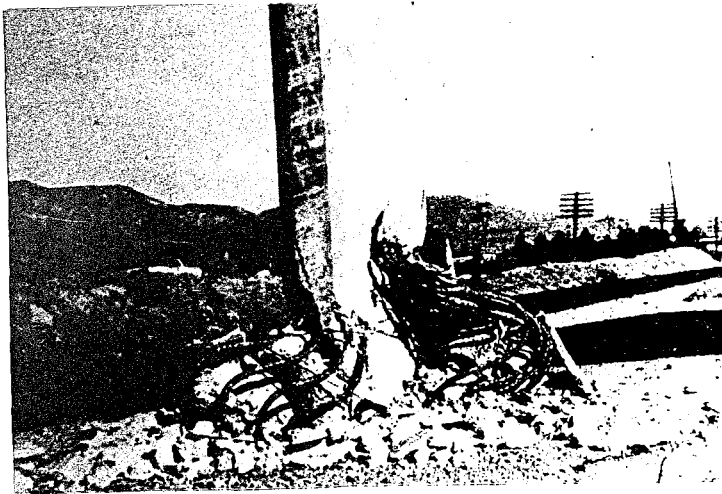
PHOTO B.2 Column Damage. (San Fernando Earthquake of 1971), ATC (1979).
