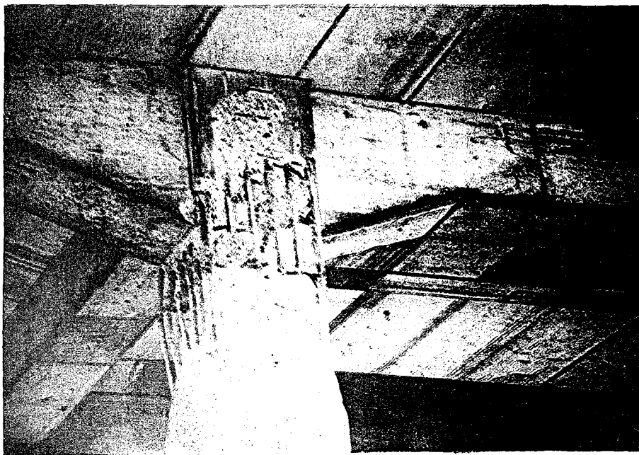
PHOTO B.13 Lack of transverse reinforcement at column-girder joints of Shinkansen Line Bridges.
