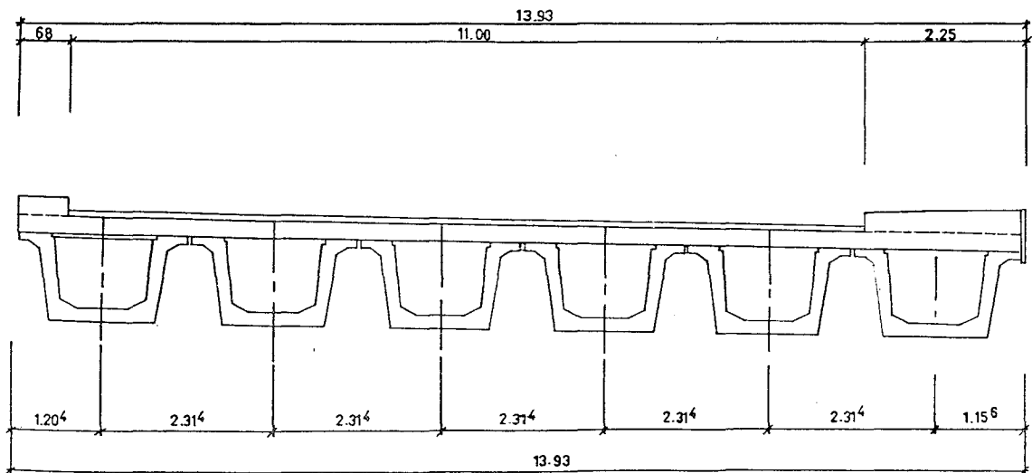
FIGURE 3.3 Typical cross-section of precast prestressed simple supported box beam.
