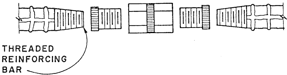
Turnbuckle detail
