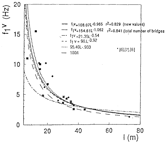
FIGURE 4.8 Correlation with experimental formulas from other researches, (Karabinis, 1995).
