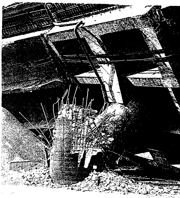
PHOTO B.8 Close view of a broken pier of Hanshin Expressway. (Kobe Earthquake of January 17, 1995), (Aydinoğlu N., 1995).
