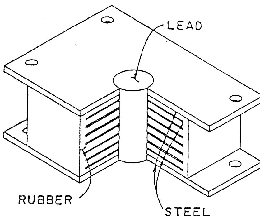
FIGURE G.15 Elastomeric bearing pad with a lead core (ATC, 1983).
