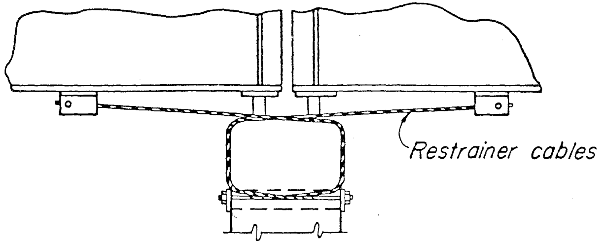
FIGURE G.4 Restrainer at pier-positive tie to pier (ATC, 1983).
