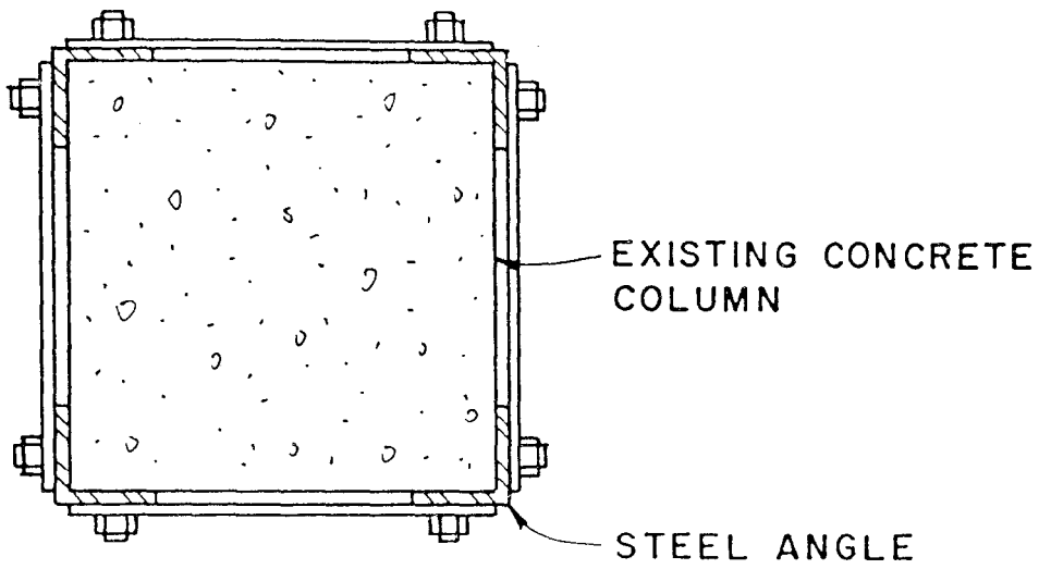
Cross-section
