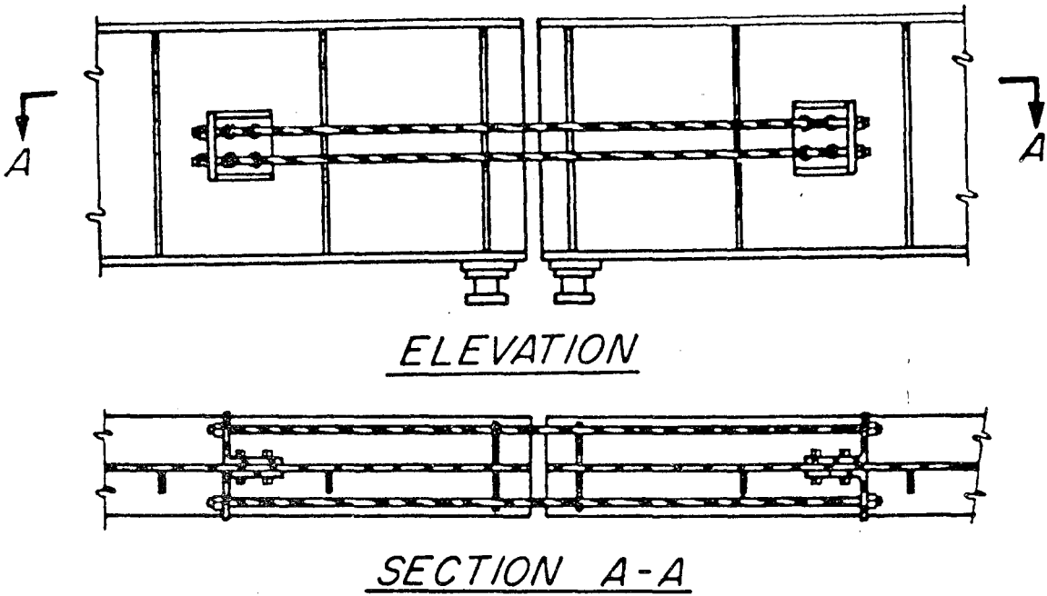
FIGURE G.1 Undesirable restrainer detail (ATC, 1983).
