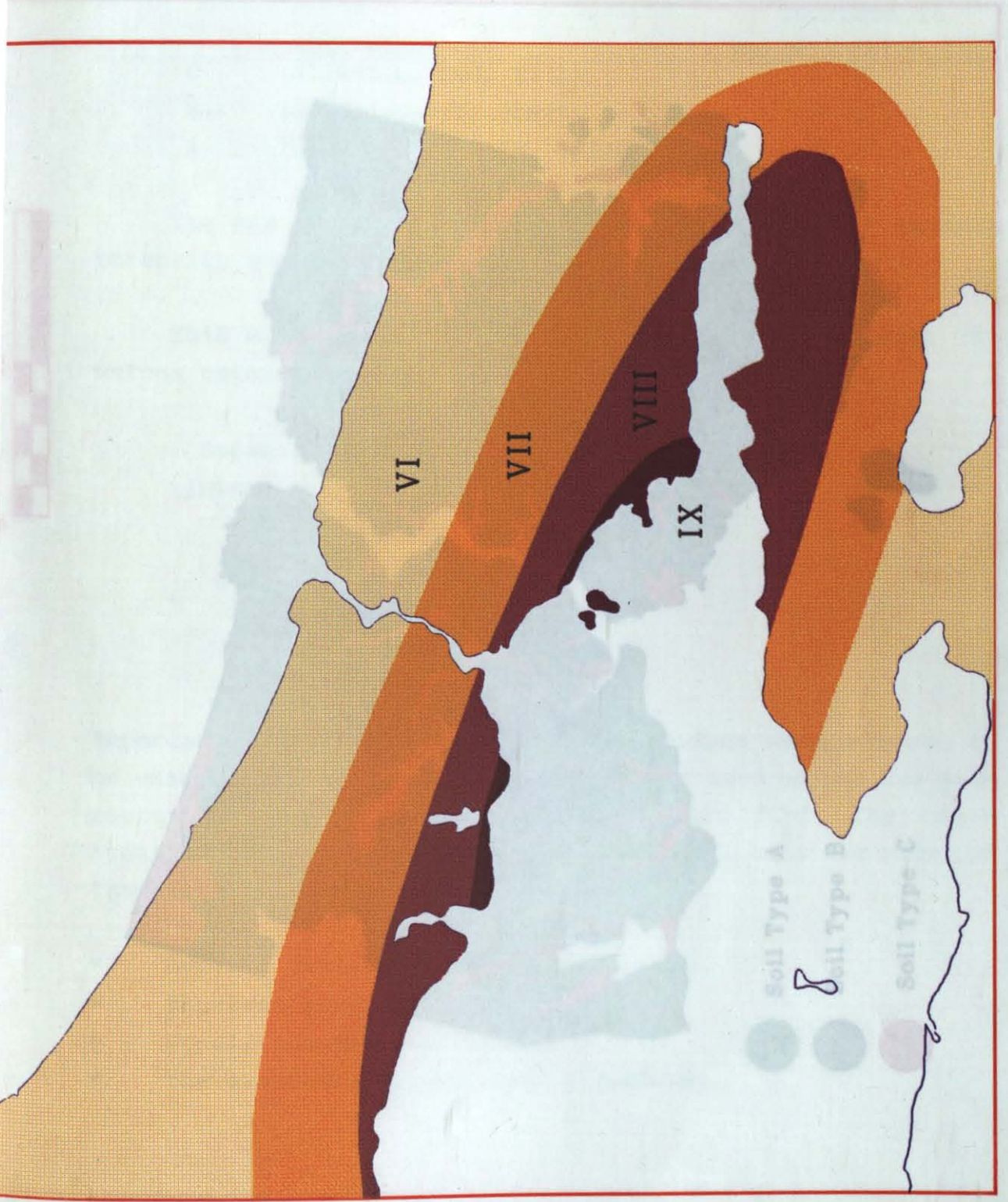
FIGURE 3.10 Seismic intensity map of Istanbul
