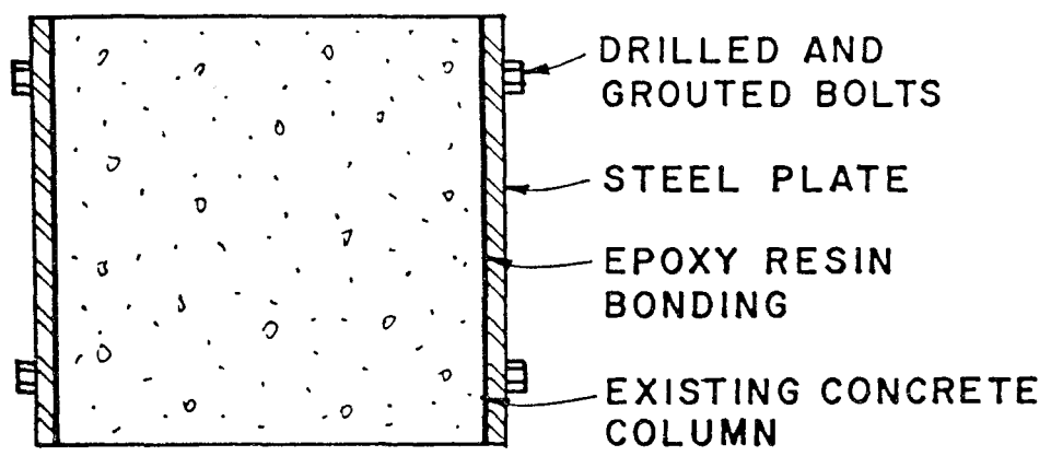
Cross-section
