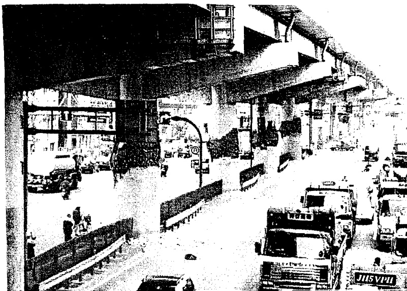
PHOTO B.10 A group of piers on Hanshin Expressway with mid-height damage.
