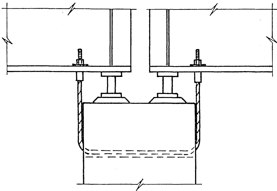
FIGURE G.9 Vertical motion restrainer retrofit (ATC, 1983).
