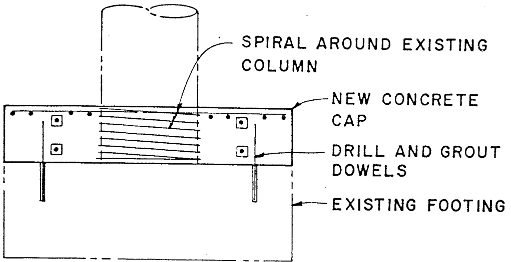
Cross-section
