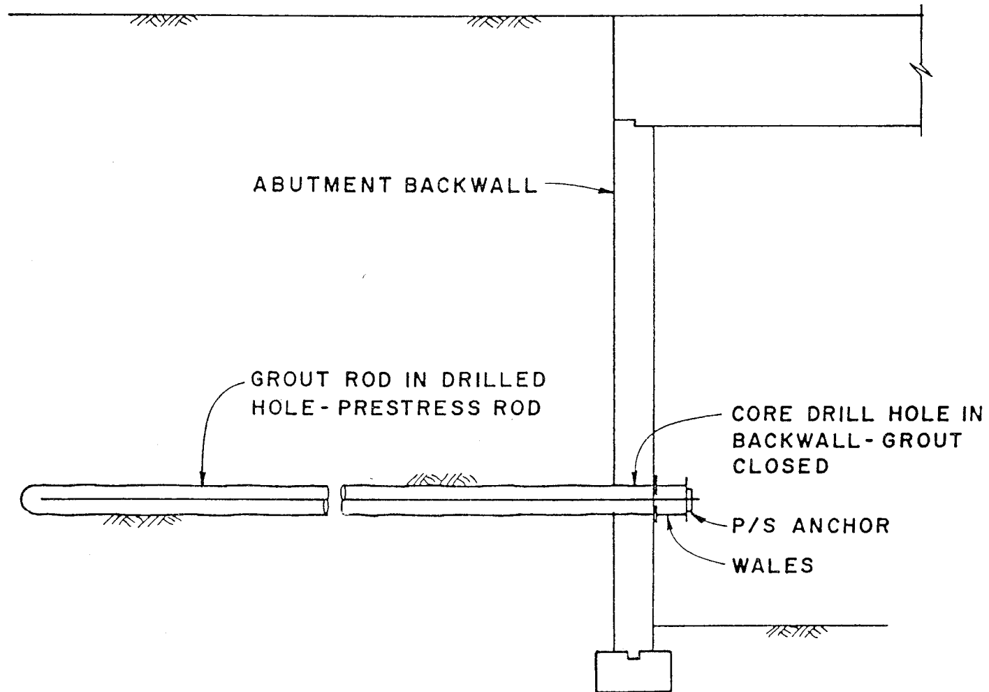
FIGURE G.27 Retrofit of abutment with soil anchors (ATC, 1983).
