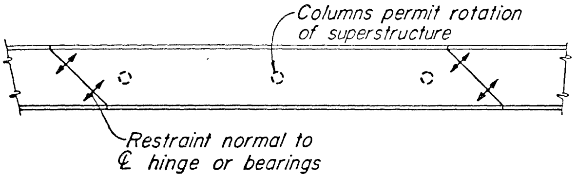
FIGURE G.3 Restrainer orientation-transversely flexible supports (ATC, 1983).
