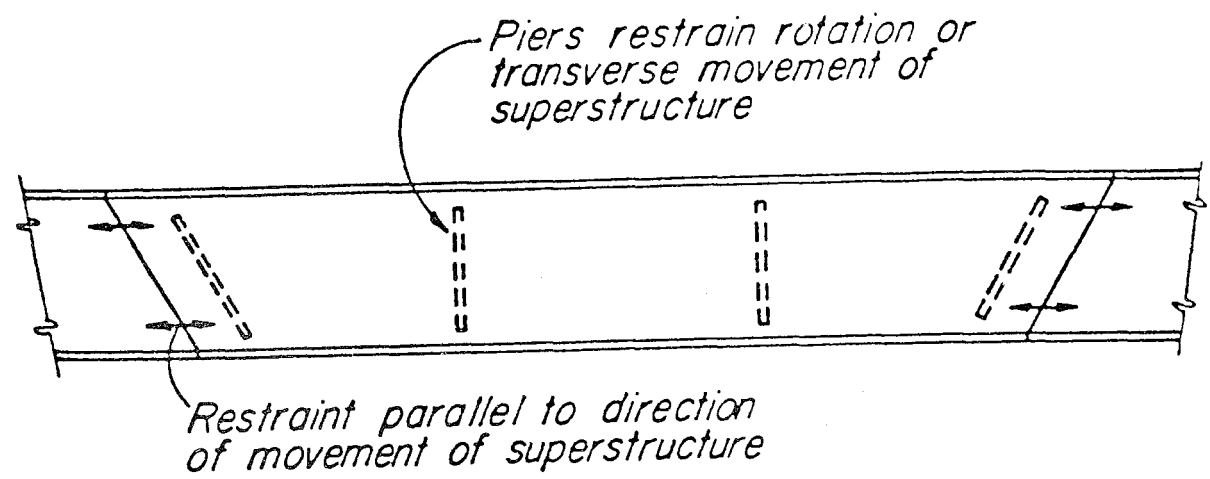
FIGURE G.2 Restrainer orientation-transversely rigid supports (ATC, 1983).
