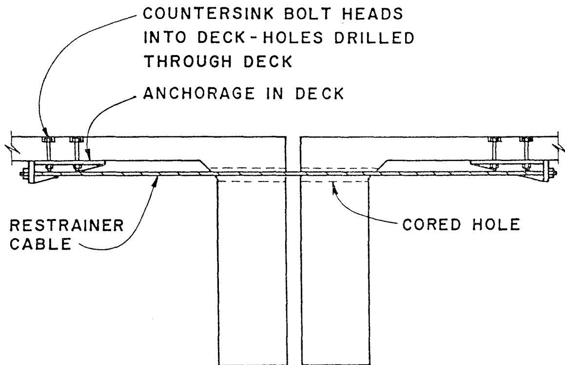
FIGURE G.7 Expansion joint restrainers tied to the concrete deck (ATC, 1983).
