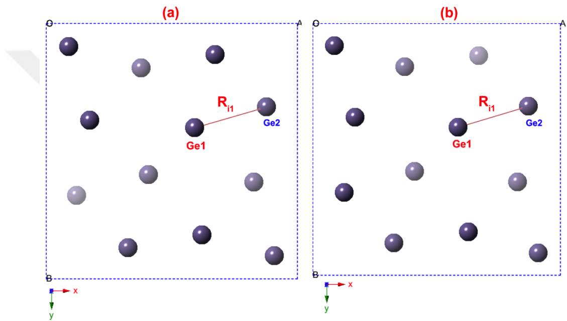
Figure 1.1.2.2 ST-12 structures constructed using ICSD cards (a) ICDS-16570 and (a) ICDS-419380 are observed in the view direction of z-axis. For (a) and (b), the nearest interatomic distance, R_{i1} were found to be 2.4793 \pm 0.0383 \text{ \AA} and 2.4802 \pm 0.0008 \text{ \AA} . The unit cells of the (a) and (b) are a=b=5.930 \text{ \AA} , c=6.980 \text{ \AA} and a=b=5.928 \text{ \AA} , c=6.980 \text{ \AA} respectively.
