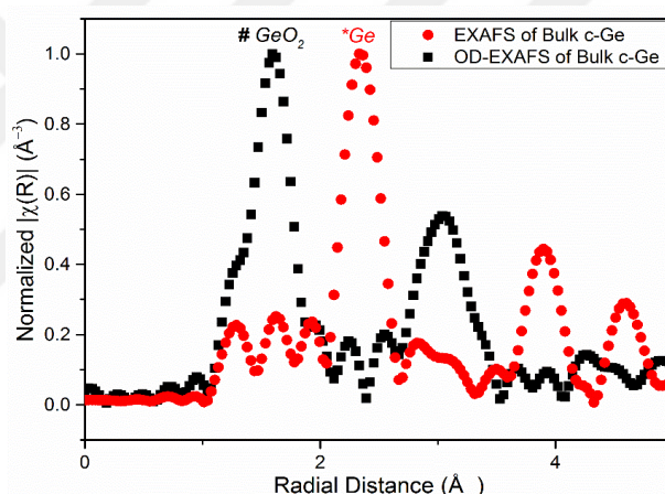
Figure 3.1.3.5 EXAFS and OD-EXFAS of bulk c-Ge in r -space.
