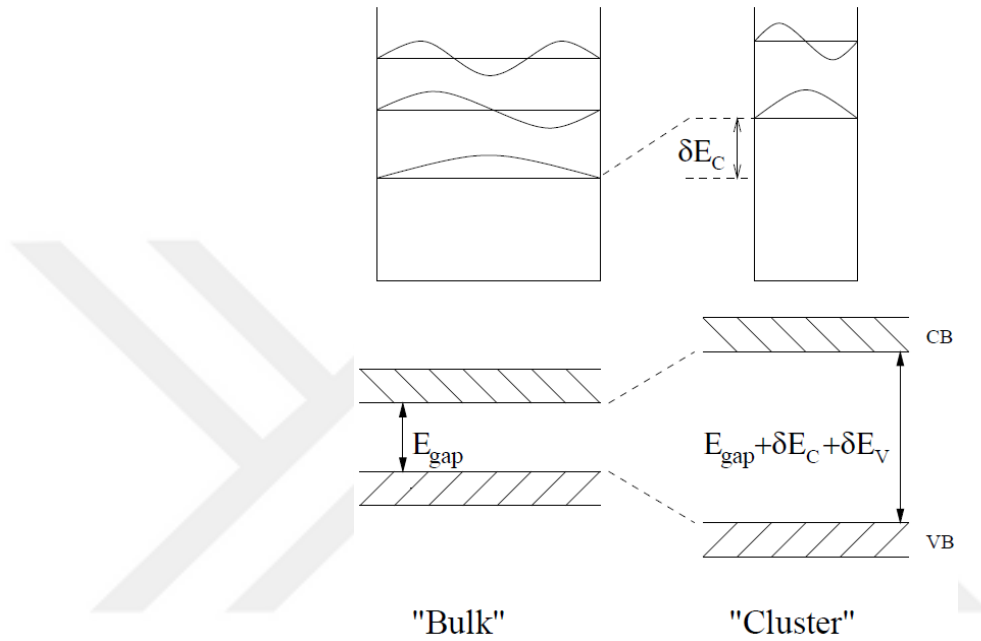
Figure 1.2.1.3 Schematic diagram of quantum confinement model. Due to decrease in size, nanoparticle can be considered as a quantum well resulting in an increase in the ground state energies. Band gap energy increases, which showed a shift of conduction and valence bands, represented as \delta E_C and \delta E_V respectively. (Extracted from reference (Bostedt, 2002).)
