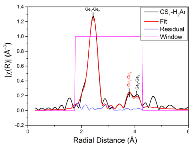
Figure 3.4.2.17 The FT modulus of EXAFS of \text{CS}_1\text{-H}_2\text{Ar} at Ge K-edge, the fit, the residual between the fit and the data and the window. The diamond cubic type of Ge and the ST-12 phases were used.
