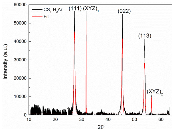
Figure 3.4.2.15 XRD of Ge qdots (CS 1 -H 2 Ar) annealed in H 2 /Ar medium at 450 °C. The reflections show growth and crystallisation of Ge qdots due to the annealing process.
