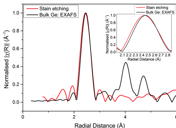
Figure 3.1.3.8 The normalised FT modulus of OD-EXAFS of stain etched Ge nanocrystals is shown in red and compared with the FT of EXAFS of bulk c-Ge. Disordered Ge atoms centered at 2.44 \pm 0.01 Å. The inset shows 0.006 Å difference between the FT modulus of EXAFS of the bulk Ge and The FT modulus of OD-EXAFS of stain etched Ge nanocrystals.
