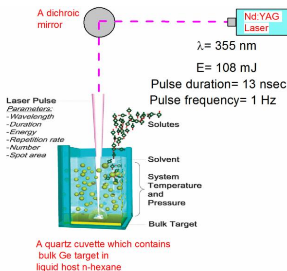
Figure 2.2.2.1 The schematic of the experimental configuration of liquid phase pulsed-laser ablation (LP-PLA) conducted in this section. The Nd:YAG laser with a wavelength of 355 nm, an energy of 108 mJ, a pulse duration of 13 ns and a pulse frequency of 1 Hz was focused on bulk Ge target in liquid host n-hexane using a dichroic mirror. (The scheme of the cuvette was taken from reference (Amendola & Meneghetti, 2013)).
