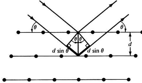
Figure 2.1.4.1 The scheme of Bragg reflection from a crystalline sample. The reflection occurs from a certain plane depending on the angle of the incident of the X-ray and its wavelength. (Taken from reference (Bostedt, 2002))
