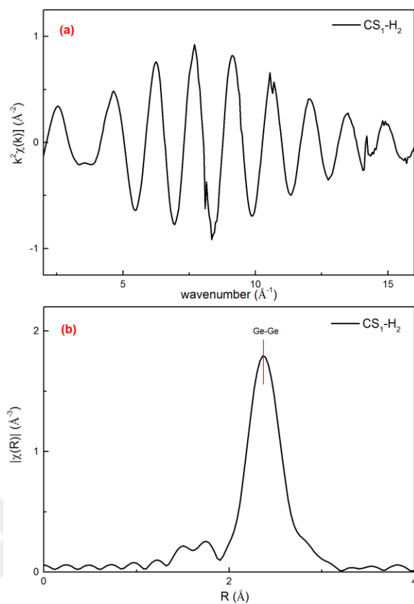
Figure 3.4.2.12 EXAFS of Ge qdots (CS 1 -H 2 ) at Ge K-edge (a) in k -space and (b) the FT modulus of EXAFS of CS 1 -H 2 in r -space.
