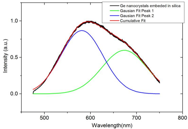
Figure 3.3.1.3 Photoluminescence of nc-Ge after H 2 (5 %)/Ar(95 %) heating treatment at 700 °C. A multi-peak Gaussian fit shows two main peaks at 595 nm (2.08 eV) and 670 nm (1.85 eV).
