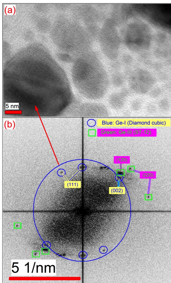
Figure 3.4.3.5 (a) TEM micrograph of \text{Ca}_1 in higher magnification. (b) The fast Fourier transform (FFT) from the whole area of (a) shows spots which matches with Ge-I (diamond cubic type) and Ge-III (ST-12) phases.
