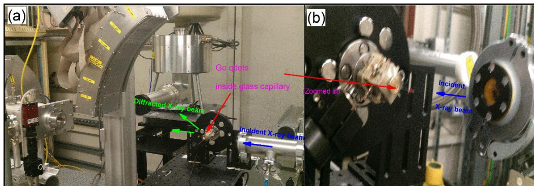
Figure 2.1.4.2 Picture of X-ray Diffraction measurement conducted at station B18, Diamond Light Source, UK. X-ray beam ( \lambda=1.54409 Å, E=8047 eV) is focused onto Ge qdots inside the glass capillary, which is attached to a rotating stage.
