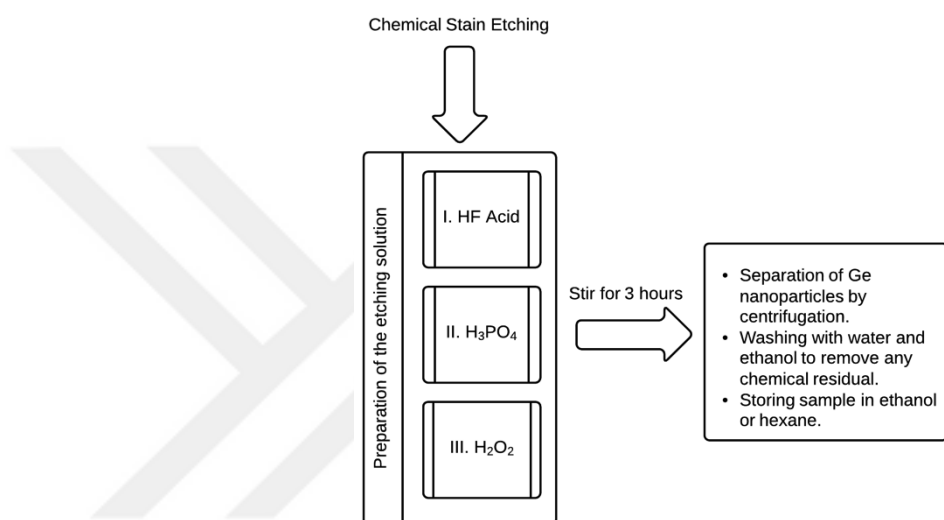
Figure 2.2.1.1 The schematic of the stain etching process. Ge nanocrystals were formed via etching using a solution of HF, phosphoric acid and hydrogen peroxide for 3 hours.
