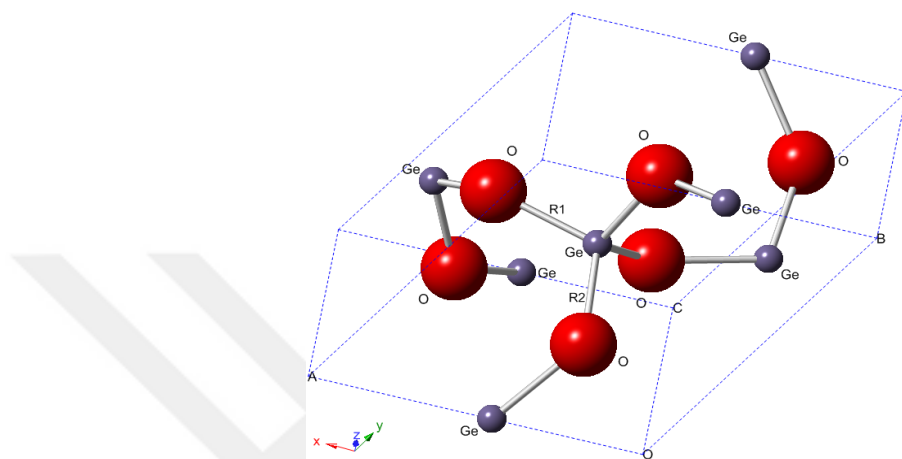
Figure 1.1.2.3 The unit cell of the alpha-quartz (trigonal) type \text{GeO}_2 shows two independent Ge-O bond distances as R1 and R2. Ge atoms and O atoms are represented by violet and red spheres respectively.
