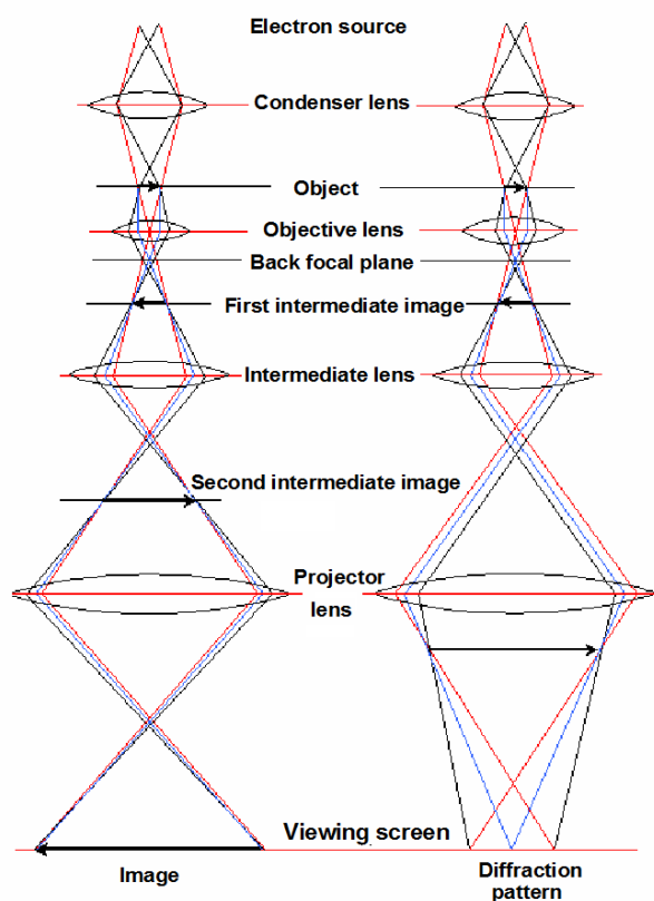
Figure 2.1.3.1 Scheme of transmission electron microscope (TEM) with selective area electron diffraction (SAED) mode. (Taken from reference (“Transmission electron microscopy scheme,” 2010))
