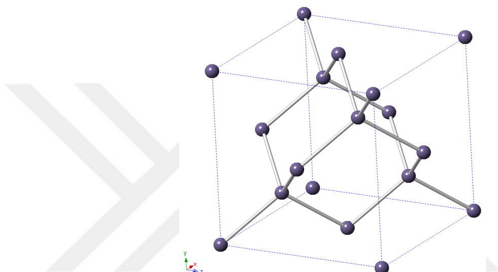
Figure 1.1.1.1 The unit cell of the diamond cubic crystal structure. The unit cell was constructed using a commercially available software called CrystalMaker (“Crystal Maker,” 2013). 1
