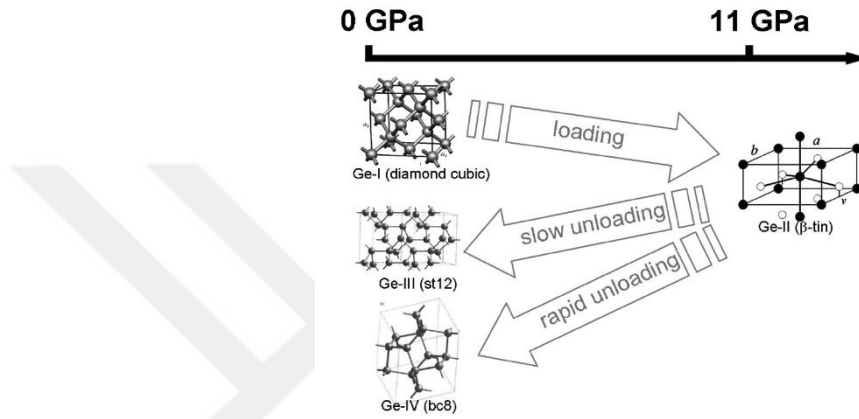
Figure 1.1.2.1 Schematic of phase transformations in case of slow and fast unloading of crystalline cubic Ge. (Extracted from reference (Oliver, 2008)).
