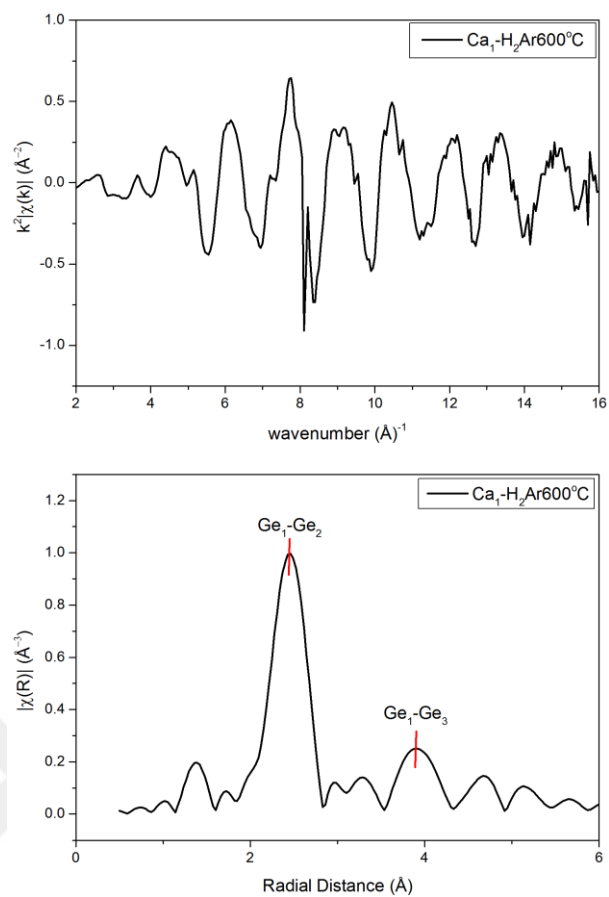
Figure 3.4.3.15 EXAFS of Ge qdots (Ca 1 -H 2 Ar600°C) at Ge K-edge (a) in k -space and (b) the FT modulus of EXAFS in r -space.
