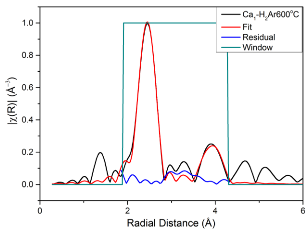
Figure 3.4.3.16 The FT modulus of EXAFS of Ca 1 -H 2 Ar600°C, the fit, the residual between the fit and the data and the window of the fit. The diamond cubic structure of Ge is used for the fit.
