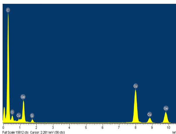
Figure 3.2.2.2 EDX of Ge nanocrystals formed by LP-PLA in n-hexane at the end of 7 hours.
