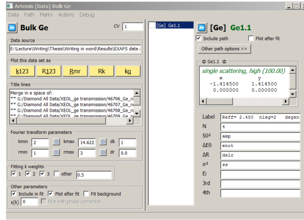
Figure A-5 The Data window in ARTEMIS used to include the scattering paths and their relevant parameters. As given in the bottom right hand side of the figure, the parameters N_i , S_0^2 , \Delta E0 , R_i are obtained using N , S_0^2 , \Delta E0 , \Delta R respectively.
