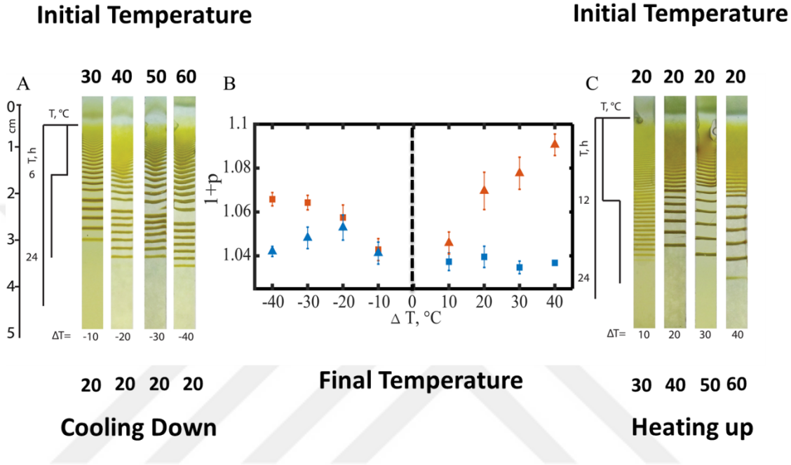
Figure 26: The effect of transition to different temperatures (transitions with different ( \Delta T values) at a particular time of transition is shown. \Delta T indicates the difference in temperature between pre- and post-transition times. (A) The samples are placed at higher temperatures (30, 40, 50, or 60°C) for 6 hours (pre-transition time) and then cooled down to 20°C. (B) Trend in spacing coefficient with respect to change in temperature: orange indicating higher temperatures, blue indicates 20°C for both A and C. Triangle represents l+p after transition and square represents l+p before transition. (C) The samples are placed at 20°C for 12 hours (pre-transition time) and then the sample is heated to higher temperatures (30, 40, 50, or 60°C).
