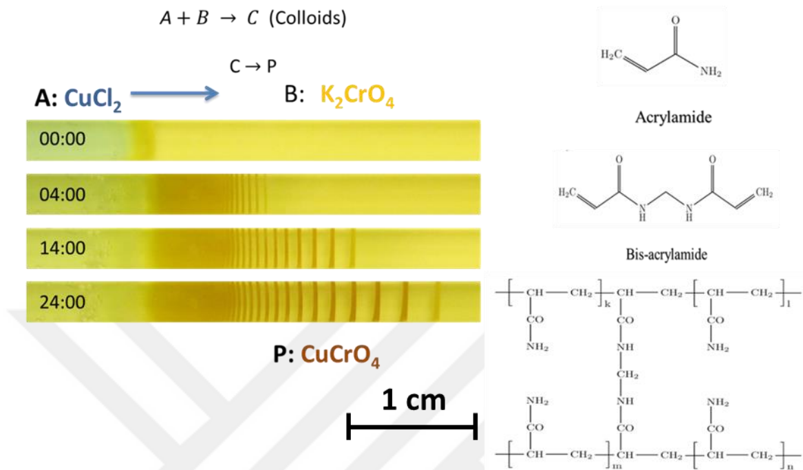
Figure 5: (Left) In our system, outer electrolyte, A, is 1 M copper(II) chloride, and 0.01 M potassium chromate is the inner electrolyte. Over the passage of time, we observe periodic precipitates of copper(II) chromate as dark lines. The diffusion of the outer electrolyte is from left to right in the photos. The time is given in hours. Scale bar is 1 cm. (Right) The hydrogel medium chosen in our experiments is polyacrylamide with bis-acrylamide as the cross-linker.
