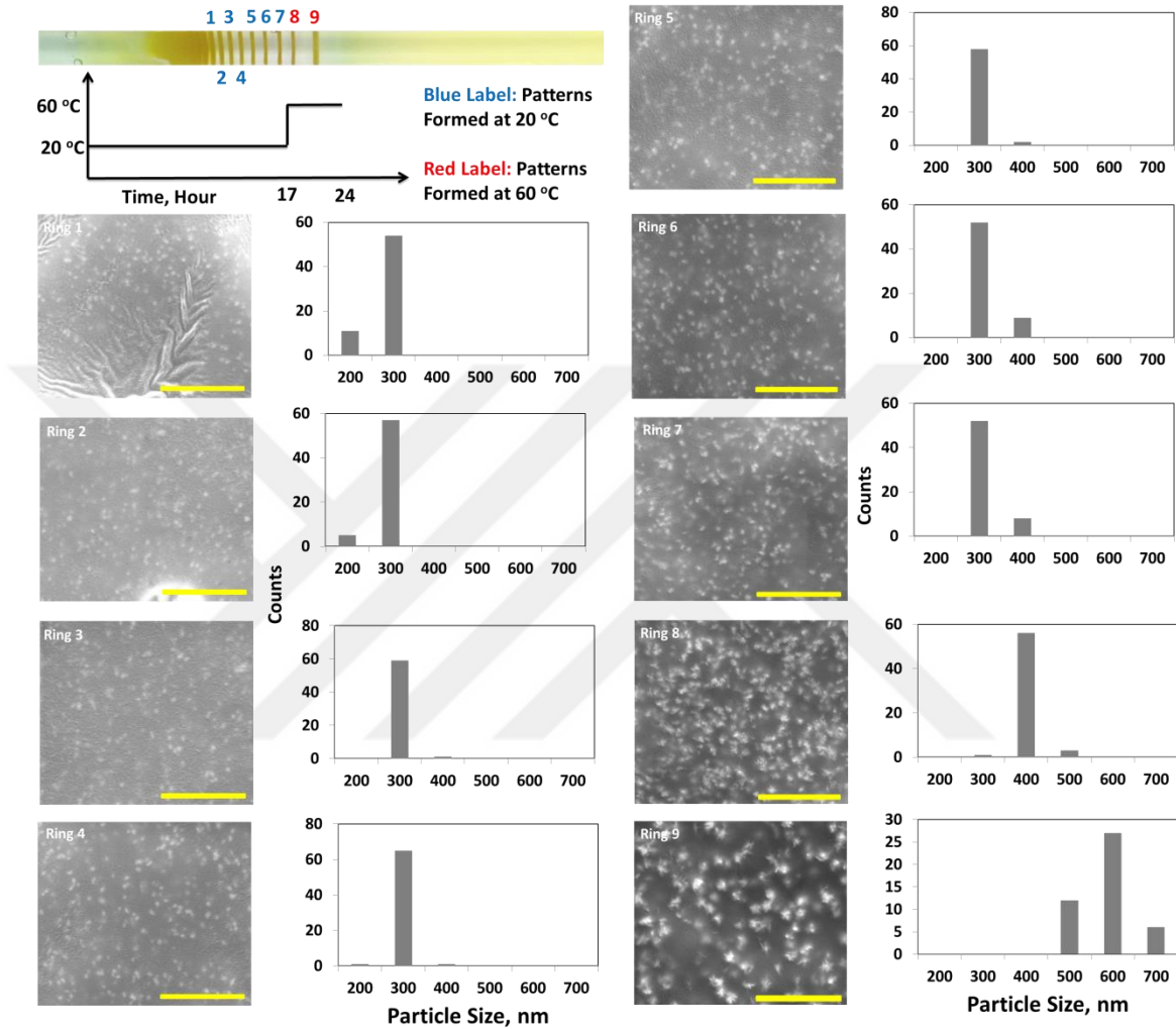
Figure 32: Patterns are formed in a sample with temperature variations from 20 to 60°C. Patterns formed at 20°C are highlighted with blue and patterns formed at 60°C are highlighted with red. The SEM images are for rings 1 to 9 with histograms on their right showing the distribution of particle size. The scale bar (yellow line) represents 5 \mu\text{m} .
