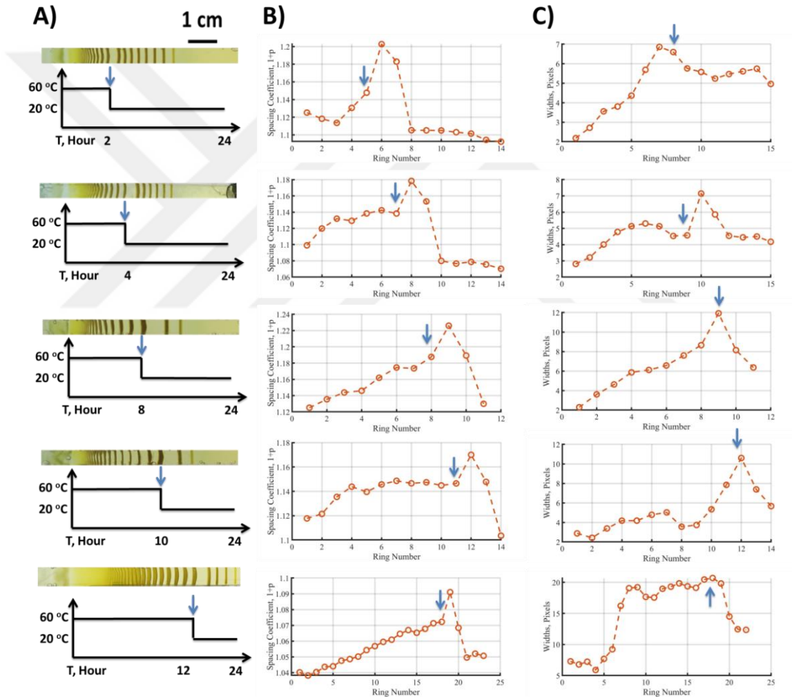
Figure 25: Pattern forming system with different transition times of temperature decrease. (A) From top to bottom, the samples are kept for 2 hours, 4 hours, 8 hours, 10 hours and 12 hours at 60°C during the LP formation, then transferred to 20°C till the 24 th hour. Scale bar is 1 cm. (B) The variation in the spacing coefficient of the patterns for different transition times. (C) The variation in the widths of the patterns. The blue arrow marks the point of transition.
