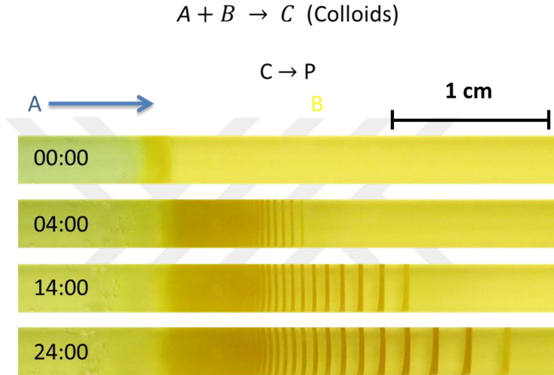
Figure 1: (top) The reaction equation resulting in the formation of LPs. A and B are the counter electrolytes; outer and inner, respectively. C refers to the colloids being produced and the aggregation of the colloids results in the precipitation bands, P (dark bands appearing in the photos below), according to the post-nucleation model. (bottom) The photos of an LP system showing the time evolution of patterns, where A (1 M copper chloride solution) diffuses in to the polyacrylamide hydrogel containing homogeneously distributed B (0.01 M potassium chromate) resulting in the precipitation bands, P , of copper(II) chromate. A is diffusing from left to right in all photos. Scale bar= 1 cm. Time is shown in hours.
