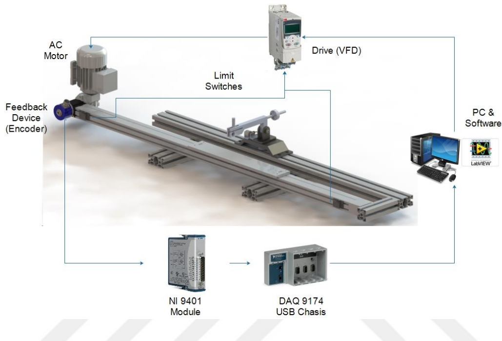
Figure 6.1. Components of a Motion Control System
