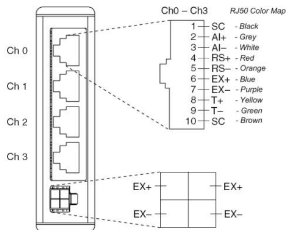
Figure 7.9. NI 9237 Pin assignments and RJ50 Colour Mapping [17]
