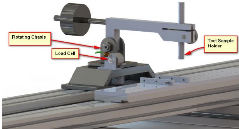
Figure 5.5. Rotational chasis concept
