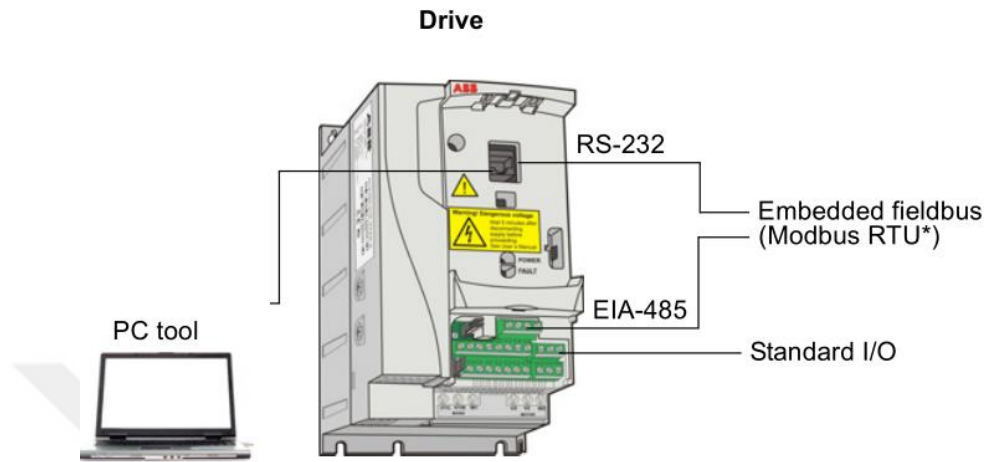
Figure 6.8. ABB ACS310 Variable Frequency Drive communication ports [18]
