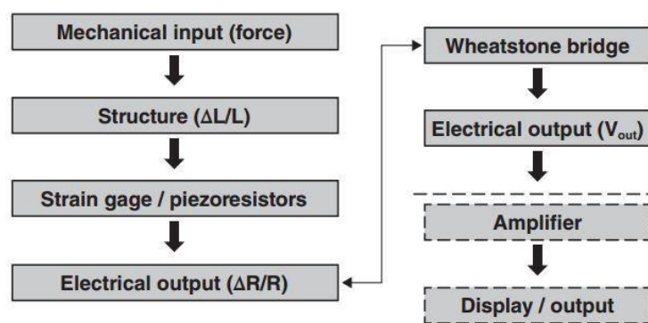
Figure 7.1. Structure of typical load cell [21]
