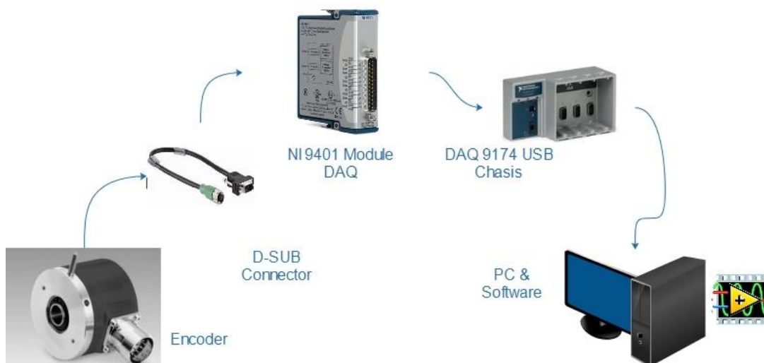
Figure 6.10. Encoder DAQ
