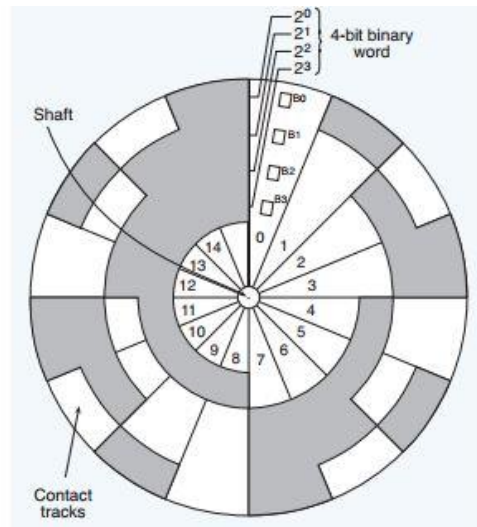
Figure 6.6. Absolute encoder disk
