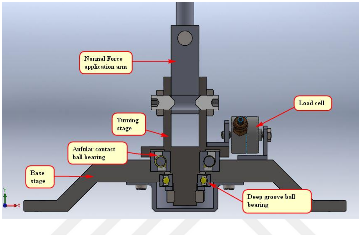
Figure 5.8. Rotational chassis
