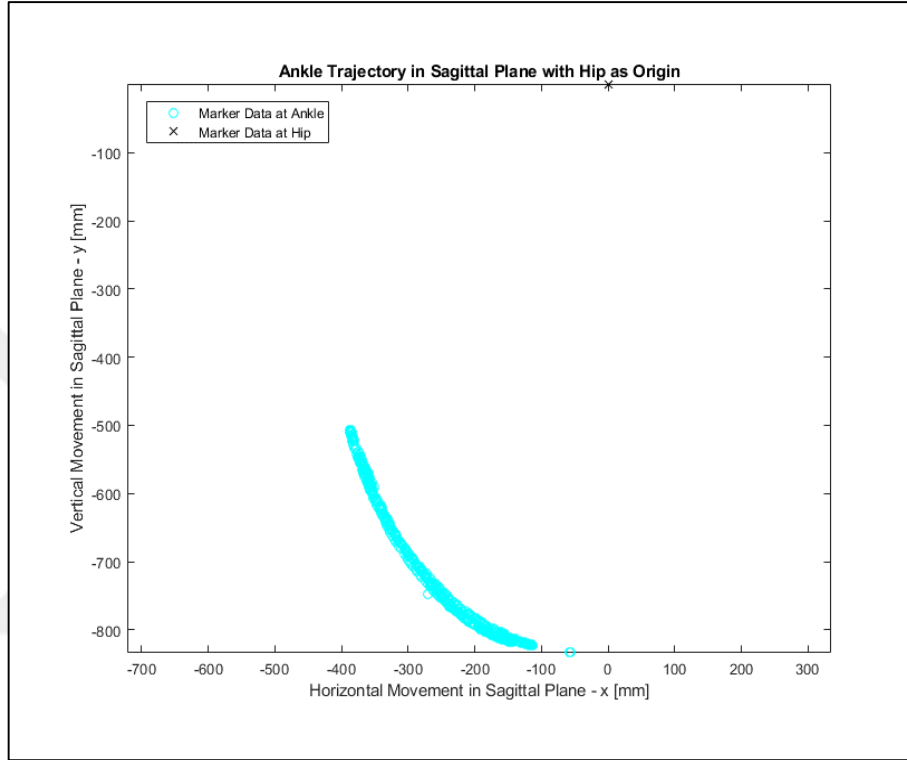
Figure 2.32 Ankle trajectory on sagittal plane with respect to hip joint.
