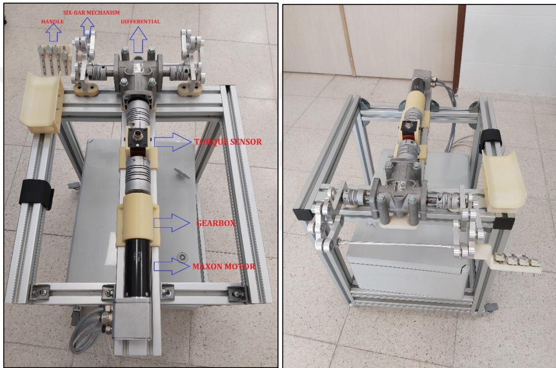
Figure 4.22 Hand Rehabilitation Mechanism.
