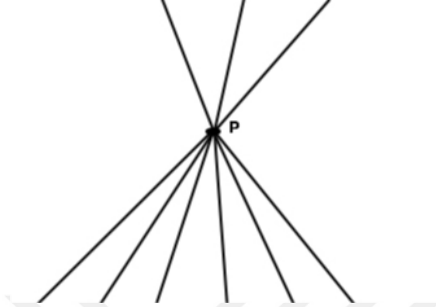
Figure 4.1: A space-time diagram of the sort of radiation source we will consider. [2]
