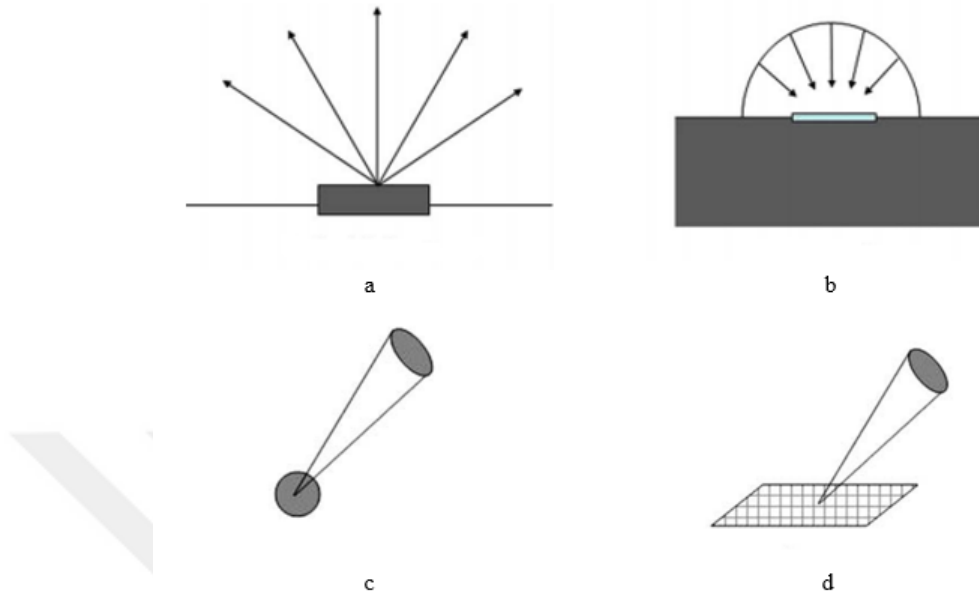
Figure 2.4: Radiometric quantities: a. radiant exitance b. radiant incidence c. radiant intensity d. radiance [22]
