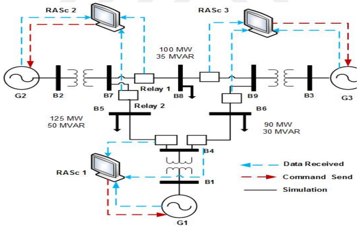
Figure 2. Distributed RAS enabled IEEE 9 bus system [6]
