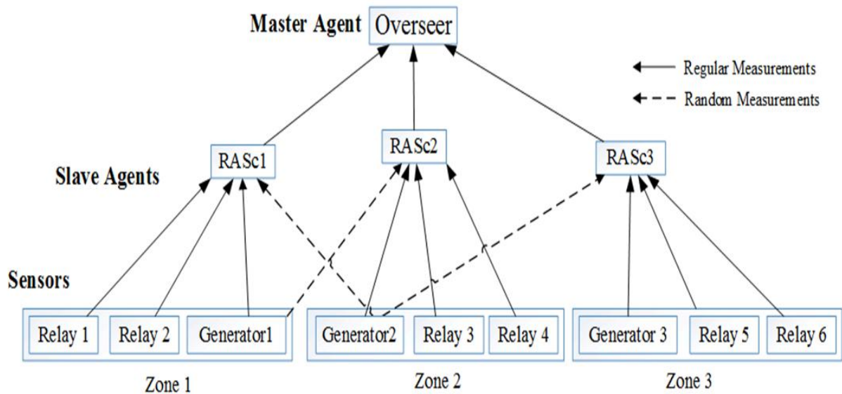
Figure 10. New Scheme Architecture
