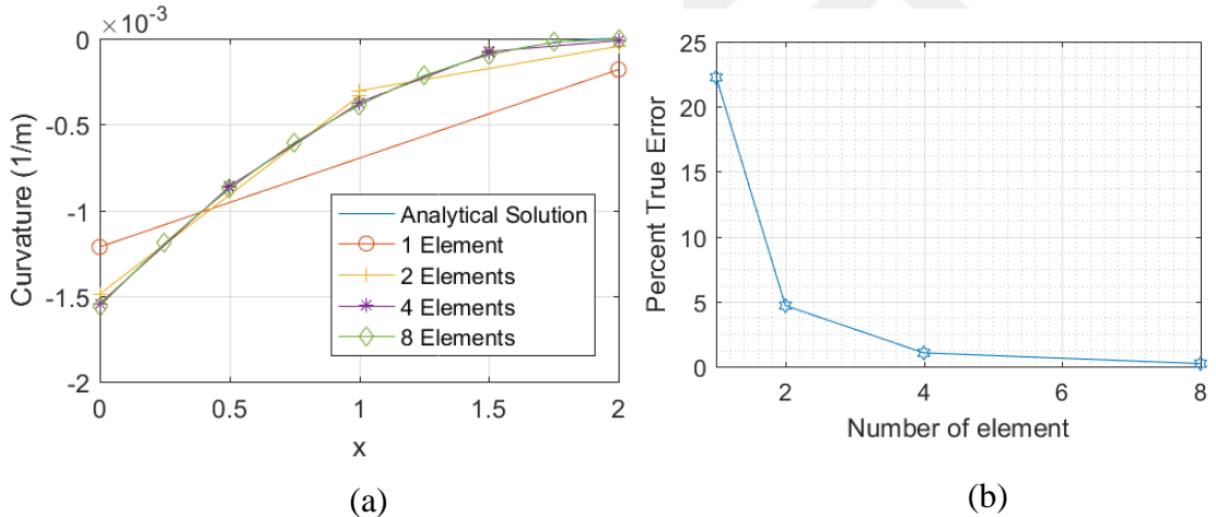
Figure 4.5. (a) Curvature profile of the beam with varying number of elements compared to the analytical solution (b) Percent true error in curvature values at support
