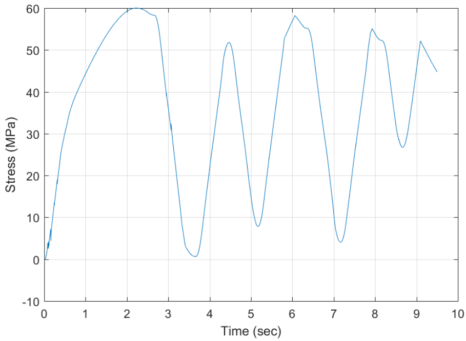
Figure 4.18. Stress history of the fiber located at the most outer of the cross section at the support
