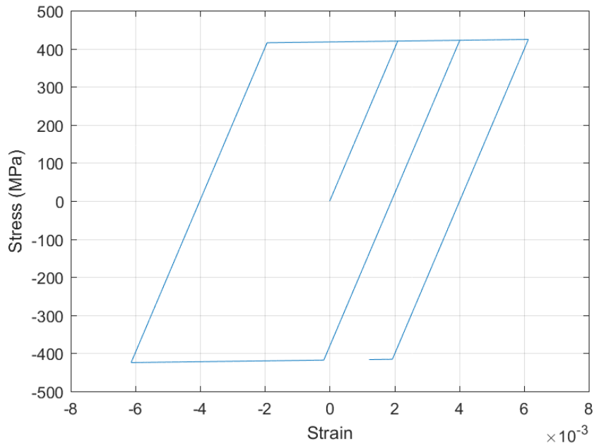
Figure 4.11. Stress-strain history of the steel fiber at the outer most of the cross section at support
