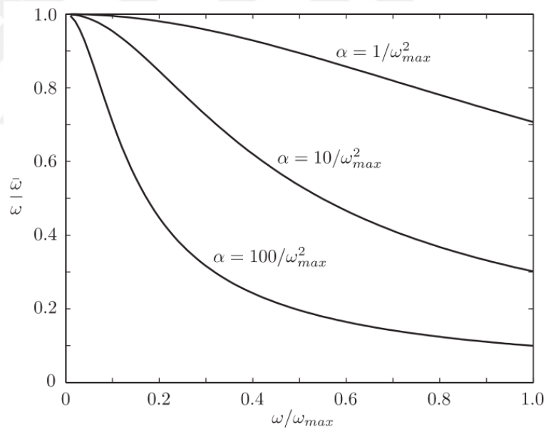
Figure 2.6 Ratio of modified and original frequencies of system with varying \alpha for method I (Olovsson et al. 2005)
