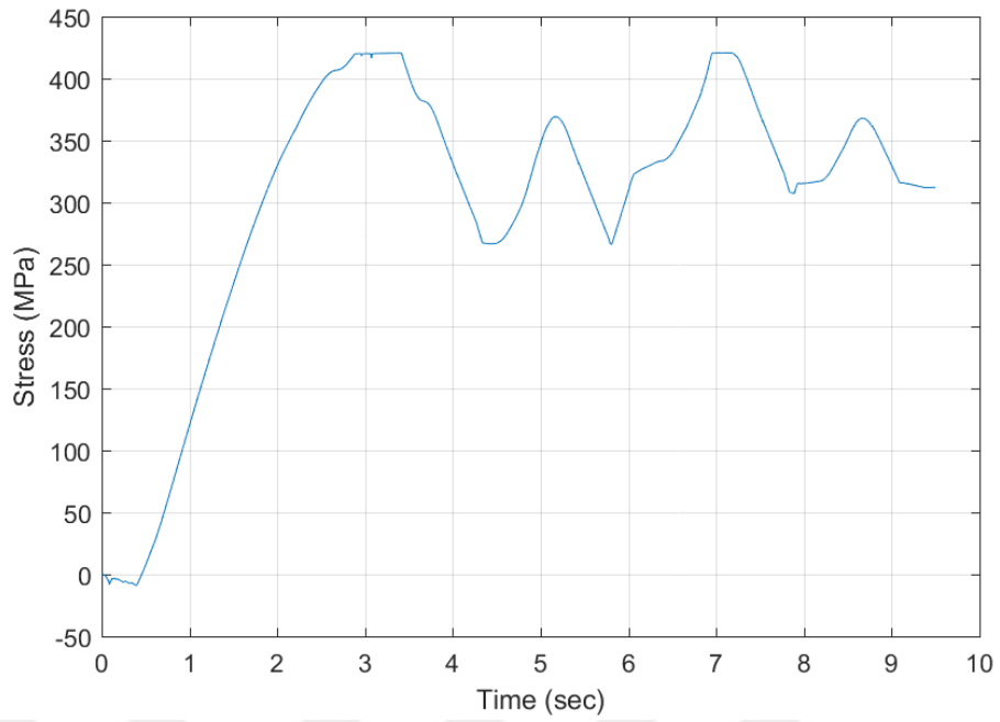
Figure 4.19. Stress history of the steel bar (compression) at the support
