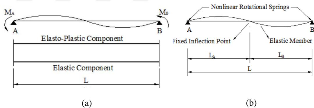
Figure 2.1. Lumped plasticity elements: (a) parallel model (Clough and Johnston 1966); (b) series model (Giberson 1967) (Figure adopted from Taucer et al. (1991))
