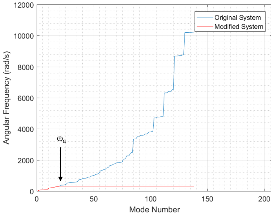
Figure 3.10. Angular frequencies before and after the application of selective mass scaling technique to a system
