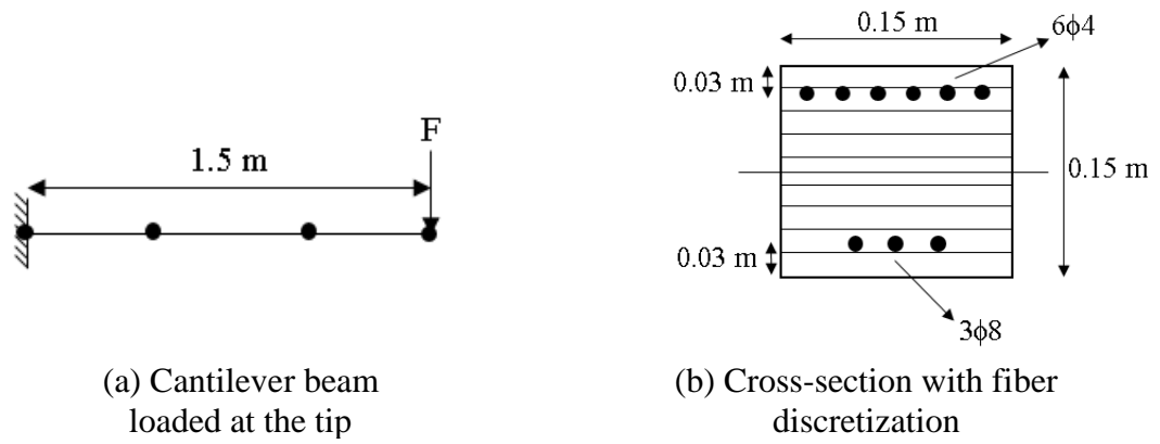
Figure 4.15. Reinforced concrete cantilever beam with tip load
