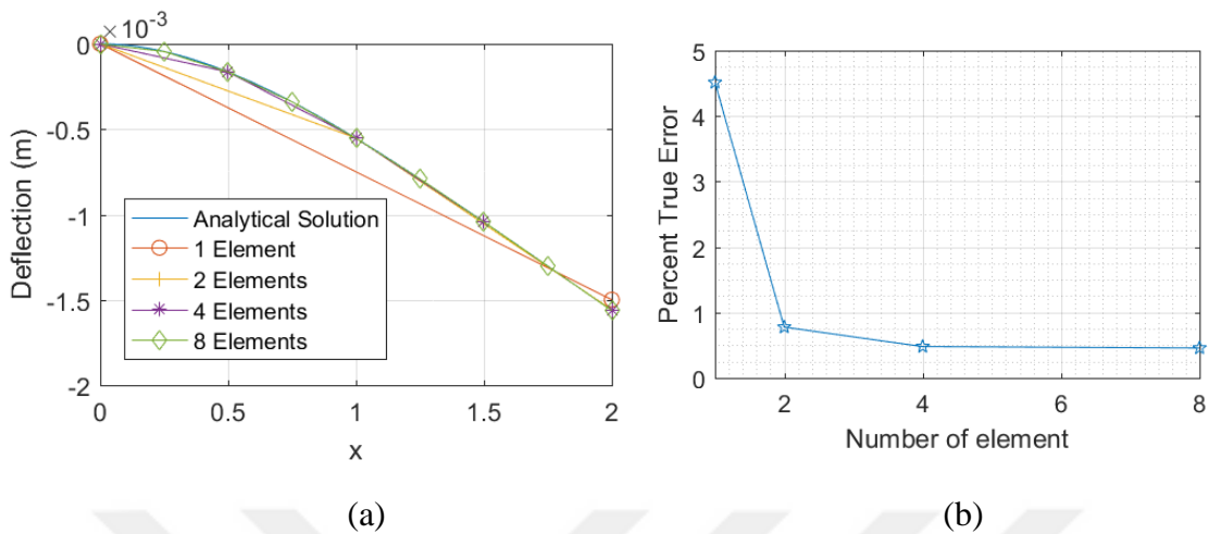
Figure 4.4. (a) Deflection of the beam with varying number of elements compared to the analytical solution (b) Percent true error in the tip displacement
