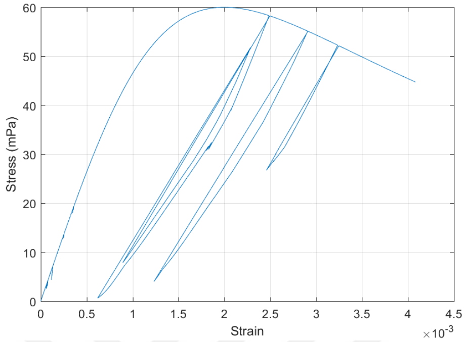
Figure 4.21. Stress-strain history of the concrete fiber at the outermost of the cross section at the fixed end of the beam
