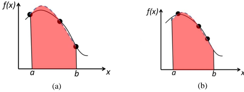
Figure 2.13. Difference in between open and closed Newton-Cotes Formulas (a) Closed (b) Open
