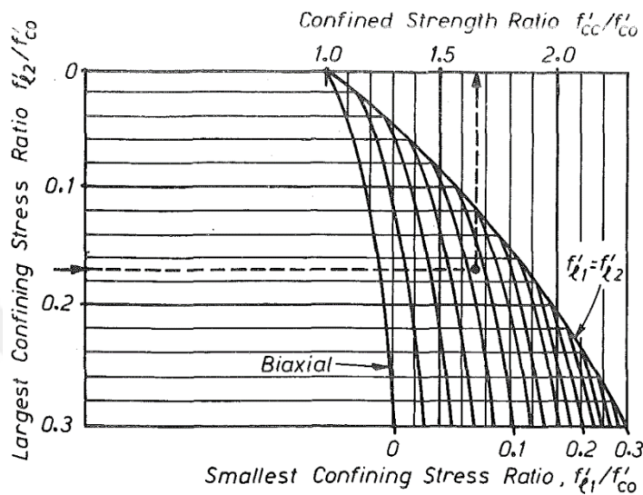
Figure 3.3. Confined peak stress determination from lateral confining stresses for rectangular sections (Mander et al. 1988b)
