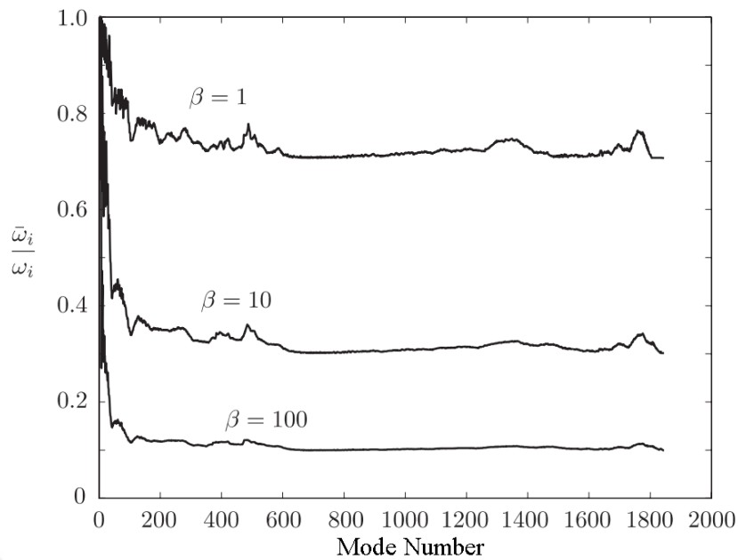
Figure 2.7 Ratio of modified and original frequencies of system with varying \beta for method II (Olovsson et al. 2005)
