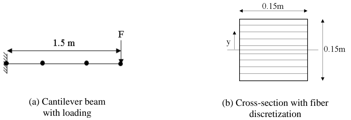
Figure 4.8. Steel cantilever beam with tip load
