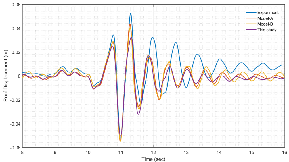
Figure 4.43. Comparison of results for the D2 earthquake (Continuation of D1)
