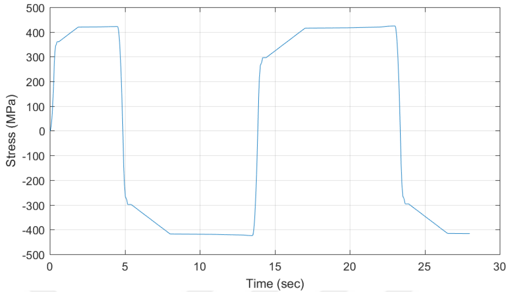
Figure 4.12. Stress history of the steel fiber at the outermost of the cross section at the support
