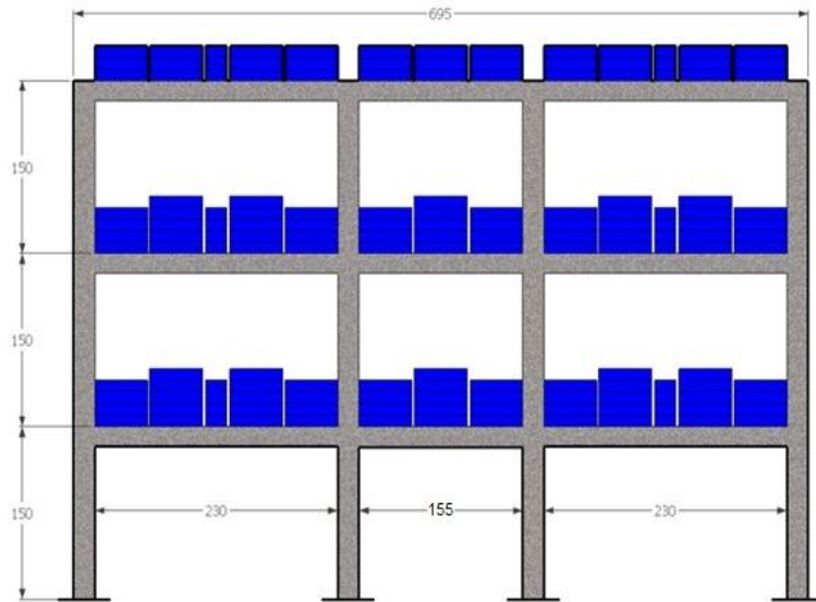
Figure 4.25. Front view of the frame
