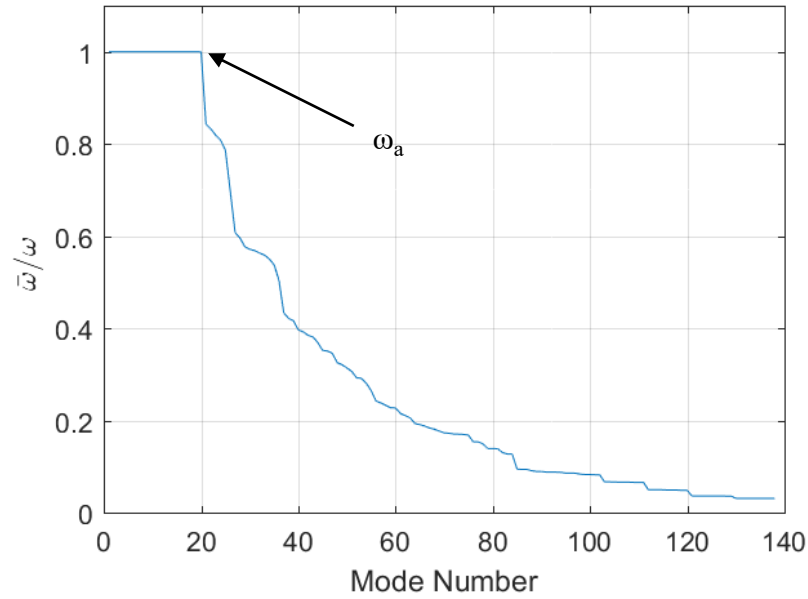
Figure 3.12. Ratio of modified and original angular frequencies of eigenmodes
