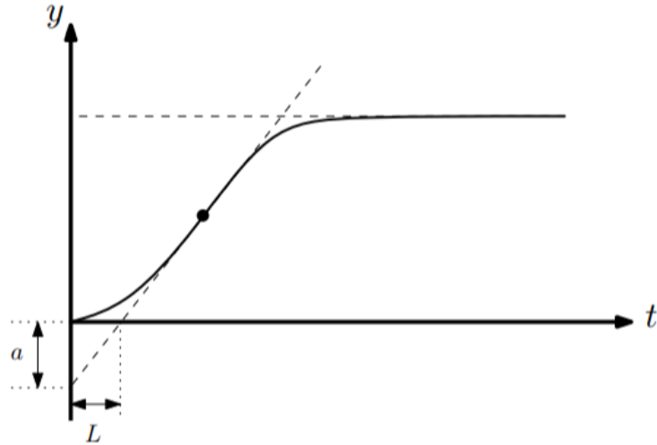
Figure 2.11. Characterization of a step-response in Zeigler-Nichols method (Hang et al. 1991)
