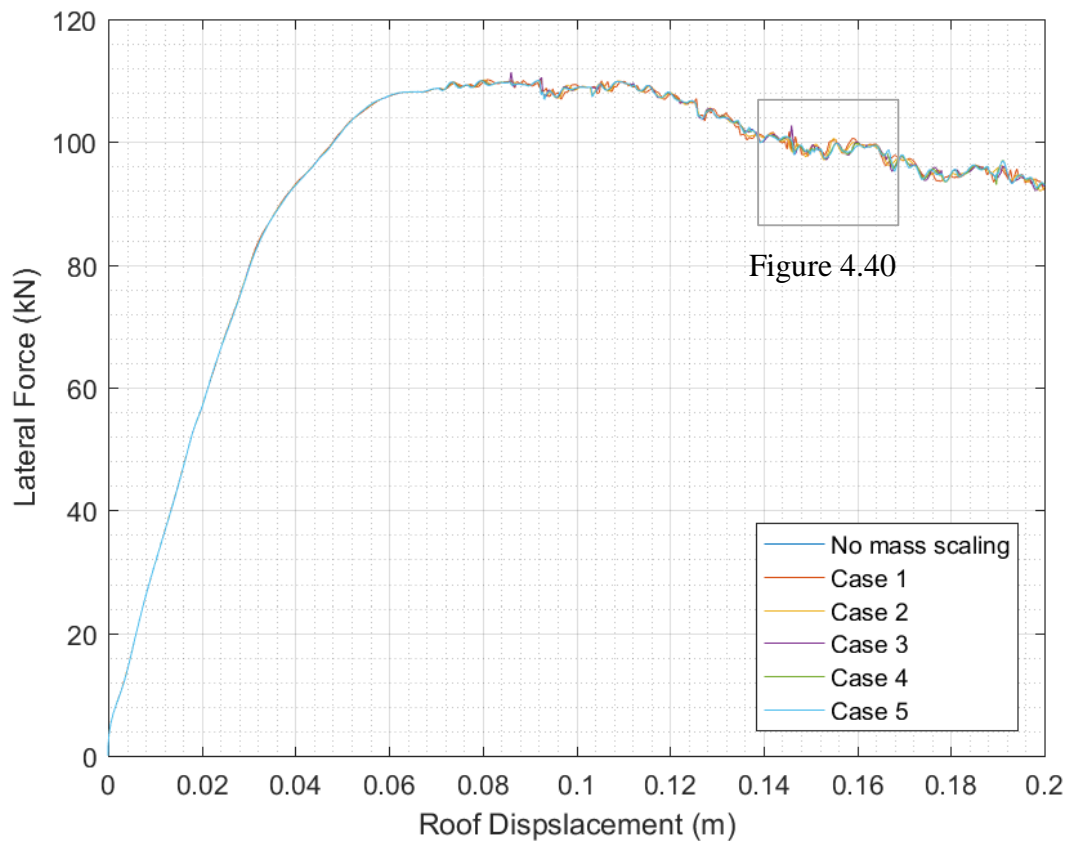
Figure 4.39. Sensitivity of the results on mass scaling.
