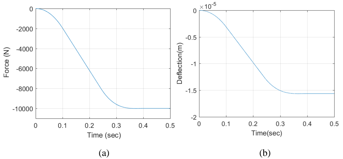
Figure 4.3. Loading pattern of the system (a) and its response (b)
