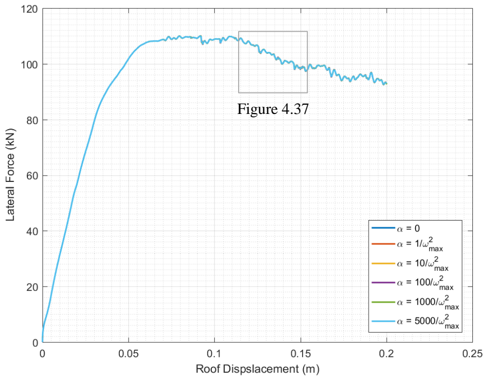
Figure 4.36. Effect of \alpha on the numerical results
