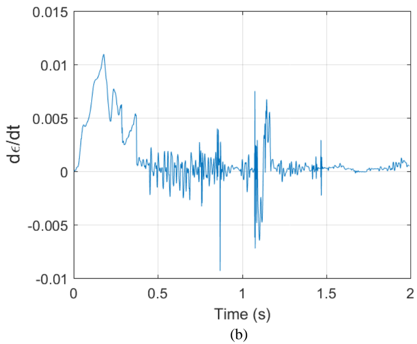
Figure 4.31. Strain response of reinforcing steel at the base (a) strain-time series, (b) rate of strain – time series
