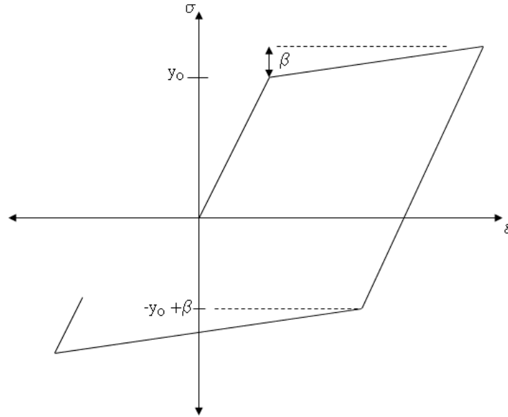
Figure 3.8. The stress-strain relation for elastoplasticity with kinematic hardening
