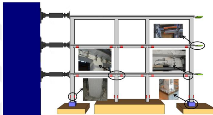
Figure 4.27. Test setup and locations of measurement instruments (Mutlu 2012)
