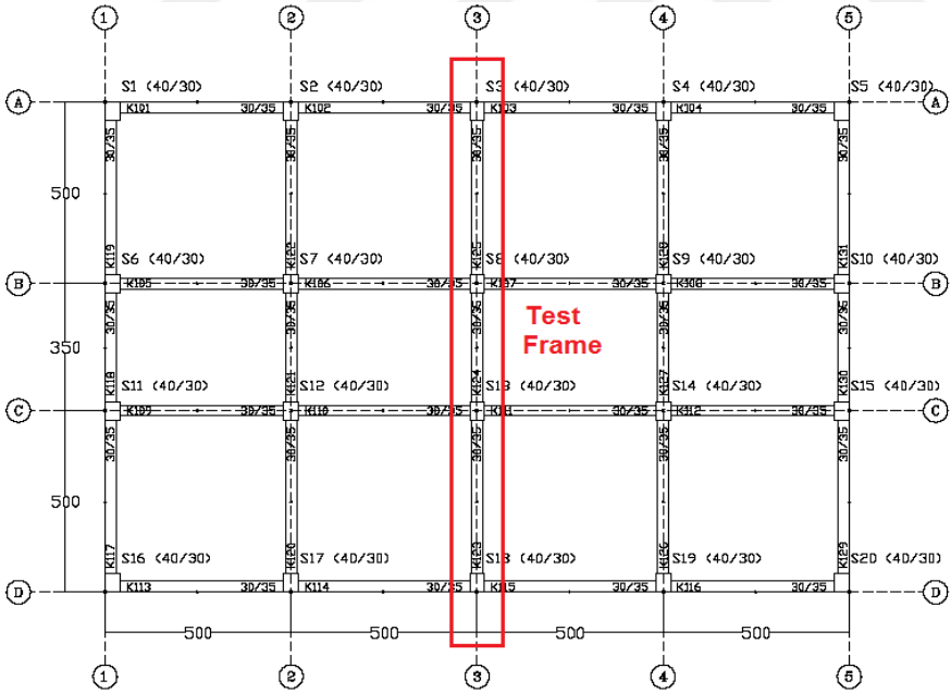
Figure 4.24. Plan view of the prototype building and the selected two-dimensional frame
