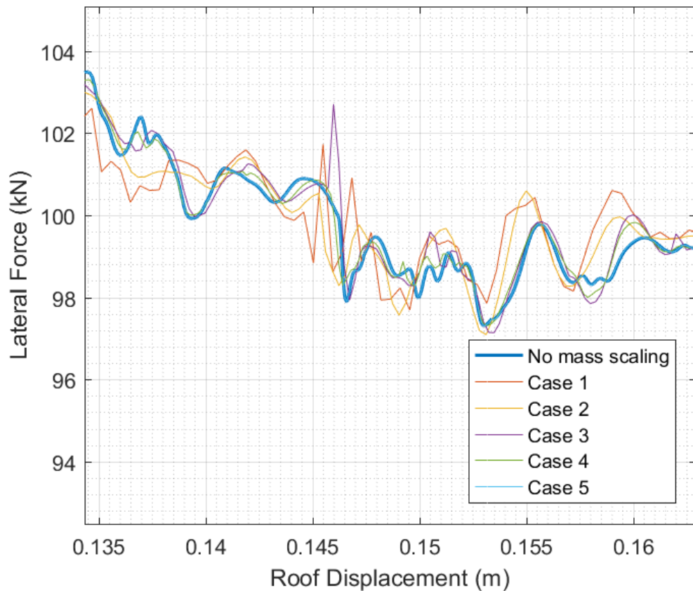
Figure 4.40. Sensitivity of the results on mass scaling (zoomed).
