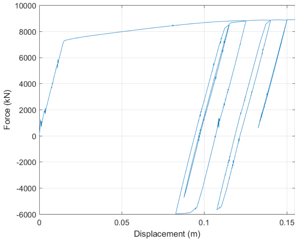
Figure 4.23. Computed external force with PID algorithm versus tip deflection
