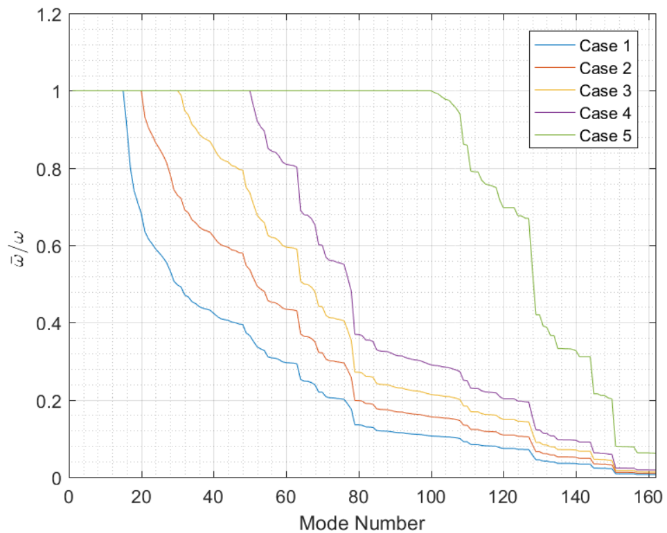
Figure 4.38. Ratio of modified and original angular frequencies of the system with varying selected corner modes
