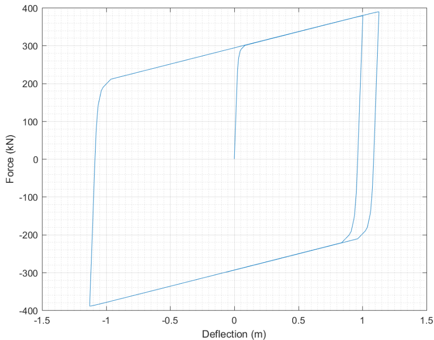
Figure 4.14. Tip deflection vs force
