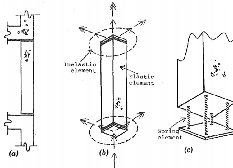
Figure 2.3 Degrading inelastic element for RC beam/columns Lai et al. (1984) (a) member in frame; (b) member model; (c) inelastic element
