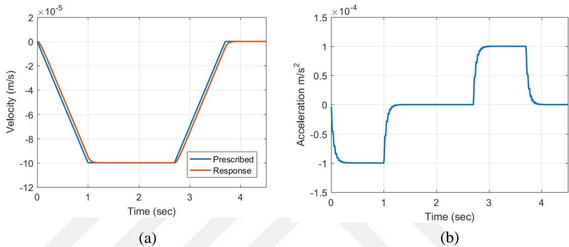
Figure 4.28. Velocity and acceleration at the control point (a) prescribed and response velocity, (b) response acceleration
