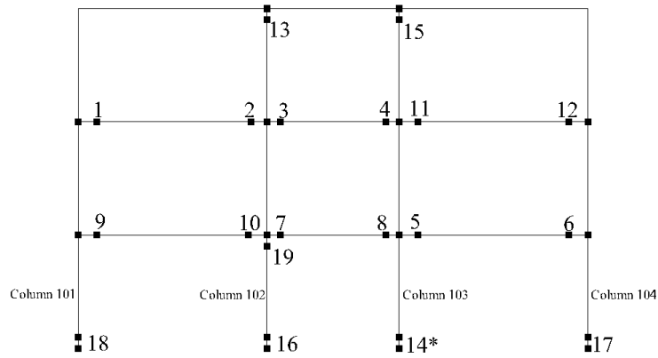
Figure 4.33. Plastic hinge formation sequence predicted by the numerical simulation
