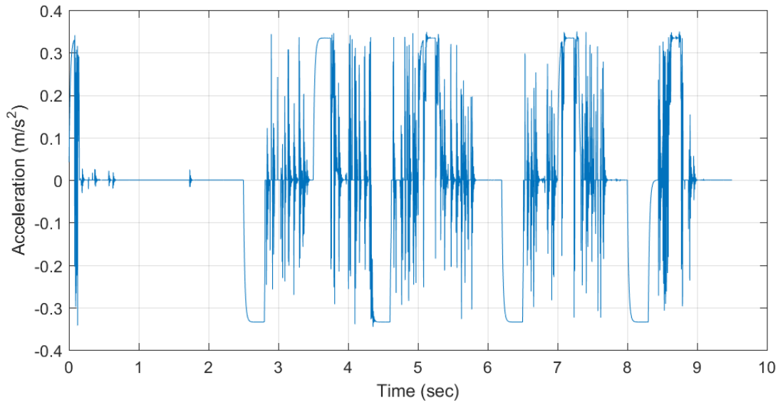
Figure 4.17. Acceleration response in the y-direction at the tip of the beam
