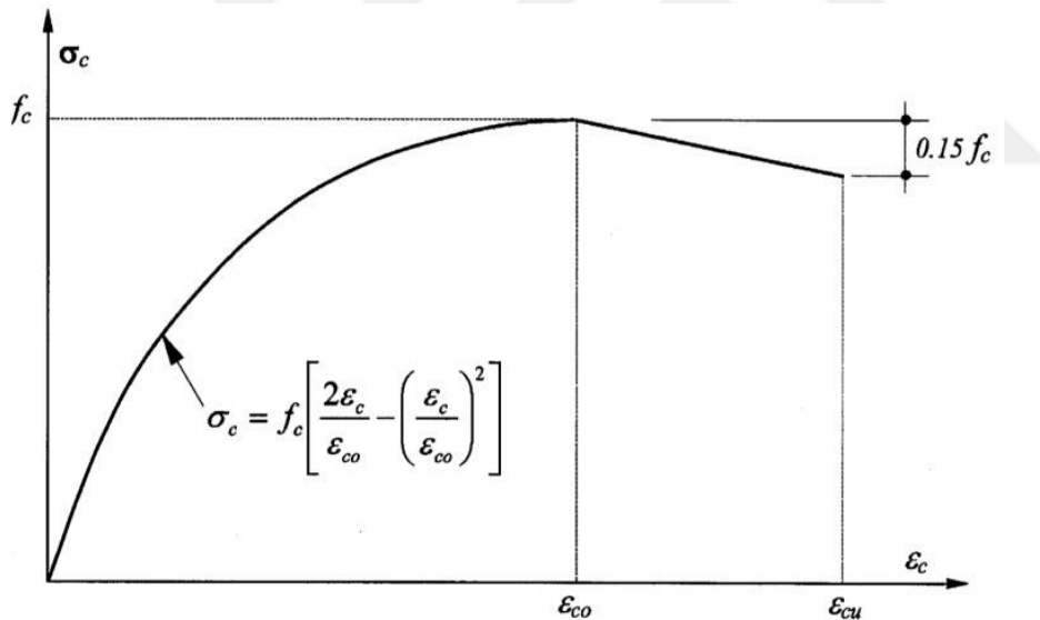
Figure 3.7. Proposed constitutive model for unconfined concrete model (Hognestad 1951)
