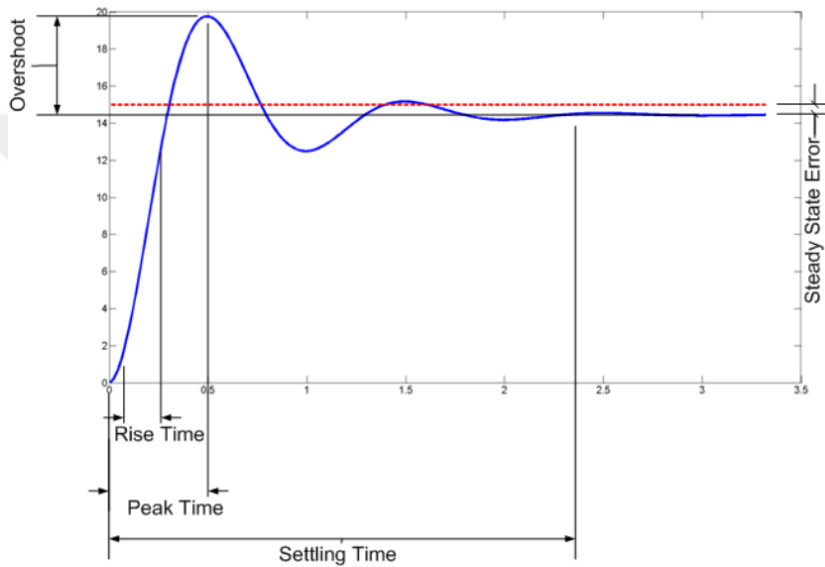
Figure 2.9. An ordinary response of the system under step point defined as step function. (Tehrani and Mpanda, 2012)
