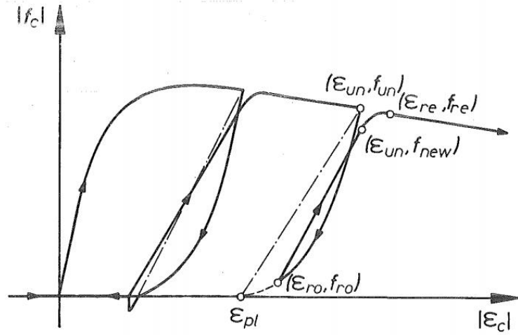
Figure 3.6. Assumed stress-strain curves for reloading branch Mander et al. (1988b)
