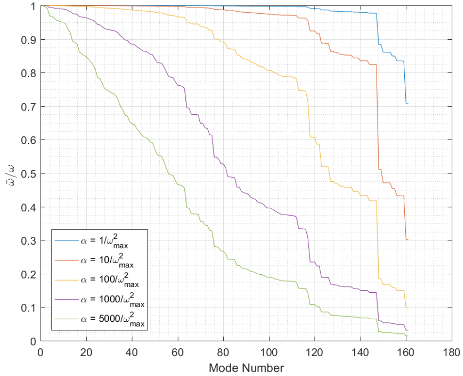
Figure 4.35. Ratio of modified and original angular frequencies of system with varying \alpha
