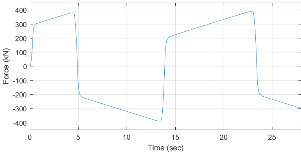
Figure 4.13. External force history calculated by the PID algorithm based on the prescribed velocity time series
