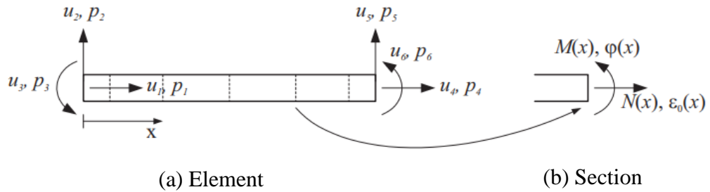
Figure 3.1. Force and deformation variables at the element and section levels (Lee and Mosalam, 2006)
