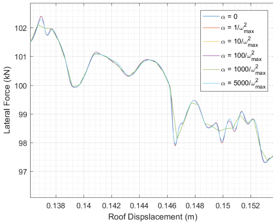
Figure 4.37. Effect of \alpha on the numerical results (zoomed)
