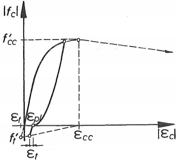
Figure 3.5. Assumed deterioration in tensile strength of concrete due to prior compression loading (Mander et al. 1988b)
