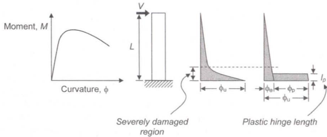
Figure 2.5 Definition of plastic hinge length (Park and Paulay 1975)
