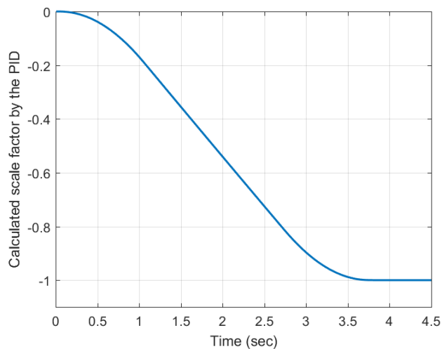
Figure 4.29. Gravity load scale factor calculated by the PID
