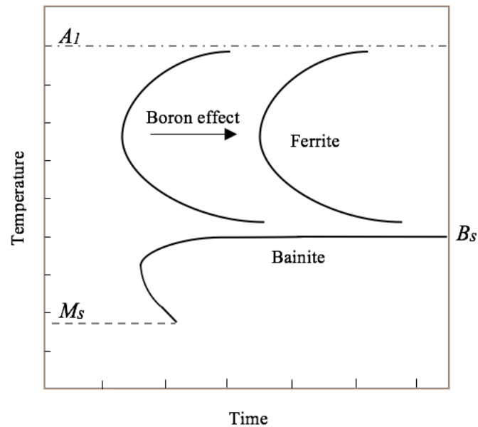
Figure 13. Effect of boron on TTT diagram of a steel.
