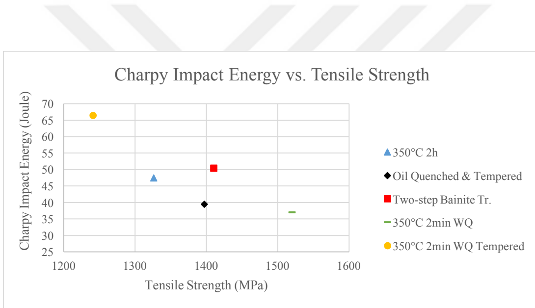
Figure 47. Graph of Charpy impact energy vs. tensile strength of heat treated 32CrB4 steel specimens.
