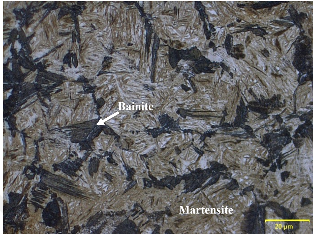
Figure 27. Optical micrograph of R260 steel quenched to 205°C and hold isothermally for 3 hours.
