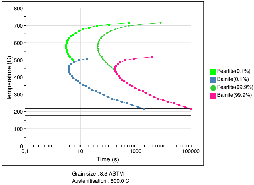
Figure 19. TTT diagram of R260 railway steel constructed by using JMatPro.
