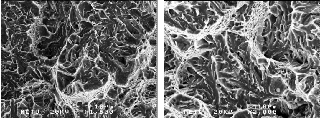
Figure 50. Fracture surface images of 32CrB4 steel that hold isothermally at 350°C for 2 minutes and then water quenched.
