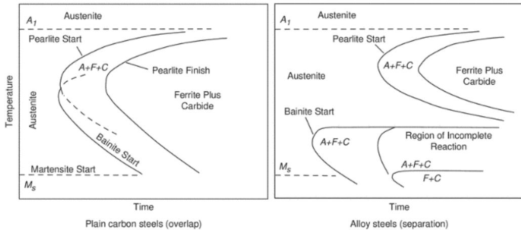
Figure 4. Effect of alloying elements on TTT diagram [6]
