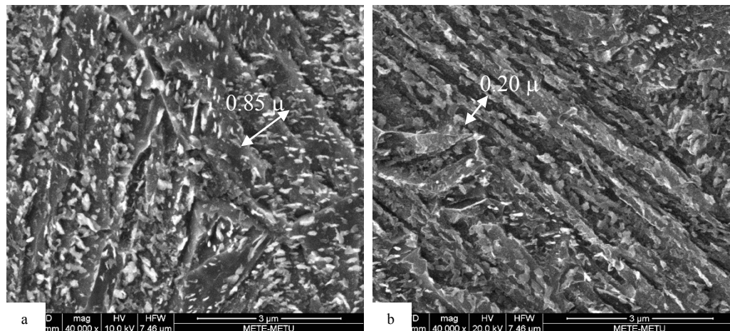
Figure 52. Bainitic structures formed by (a) single step isothermal holding at 350^{\circ}\text{C} for 2 hours (b) two-step quenching and partitioning at 350^{\circ}\text{C} for 2 minutes and 300^{\circ}\text{C} for 5.5 hours.
