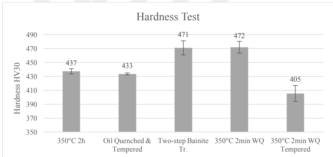
Figure 44. Graph of 32CrB4 steel hardness for selected heat treatments
