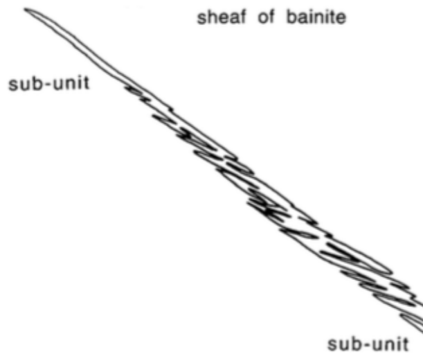
Figure 5. Bainite sheaf illustration [1]
