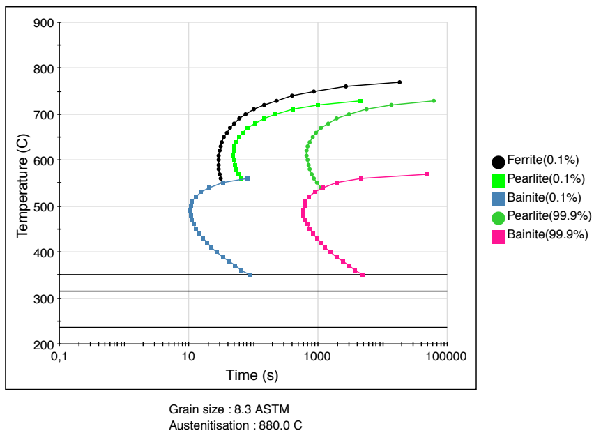
Figure 20. TTT diagram of 32CrB4 steel constructed by using JMatPro.
