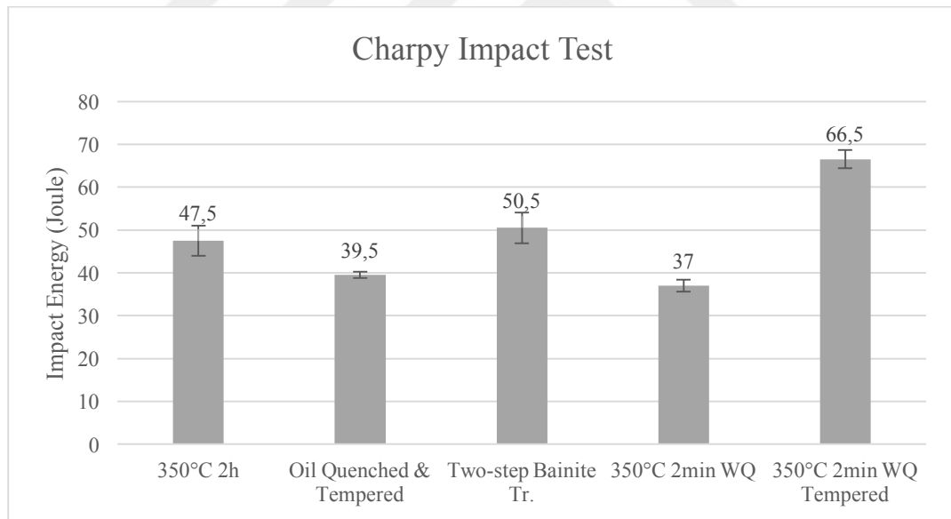
Figure 46. Charpy impact test results of heat treated 32CrB4 steel specimens
