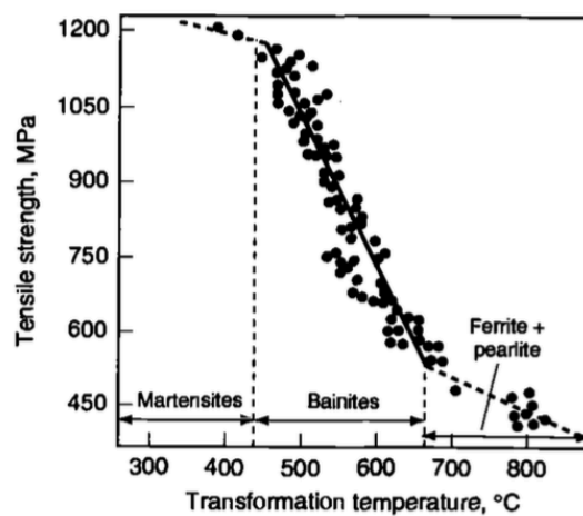
Figure 9. Diagram showing the effect of transformation temperature on tensile strength of low-carbon steel [18]
