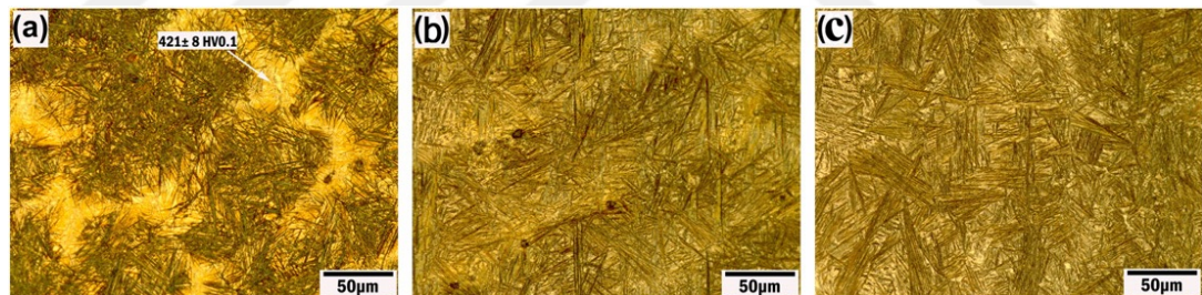
Figure 16. Optical micrographs of samples subjected to isothermal holding at (a) 300°C for 8 h (b) 330°C for 4 h and (c) 360°C for 1 h [36].
