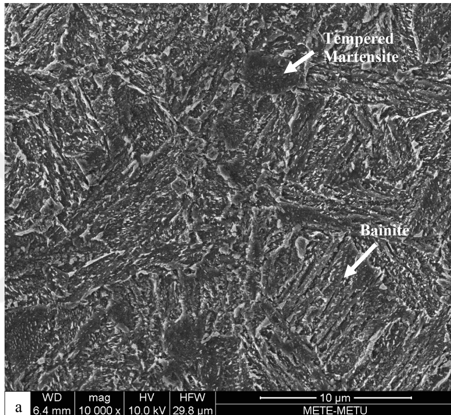
Figure 43. Bainite and tempered martensite phase mixture of 32CrB4 steel obtained by quenching to 350°C and hold isothermally for 2 minutes and water quenching followed by tempering at 450°C for 2 hours.
