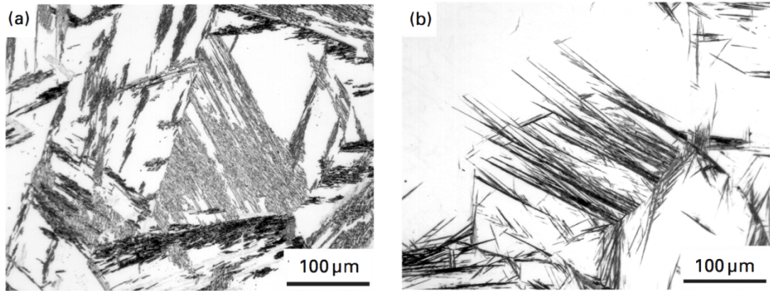
Figure 15. Optical micrographs of (a) upper bainite (b) lower bainite of high-carbon steel [35]
