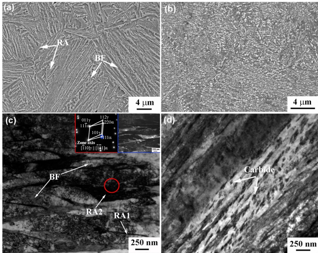
Figure 14. SEM and TEM micrographs of (a)(c) carbide-free bainite structure, (b)(d) carbide-bearing lower bainite structure, studied by Long et al. , by using 0.34C% [33].
