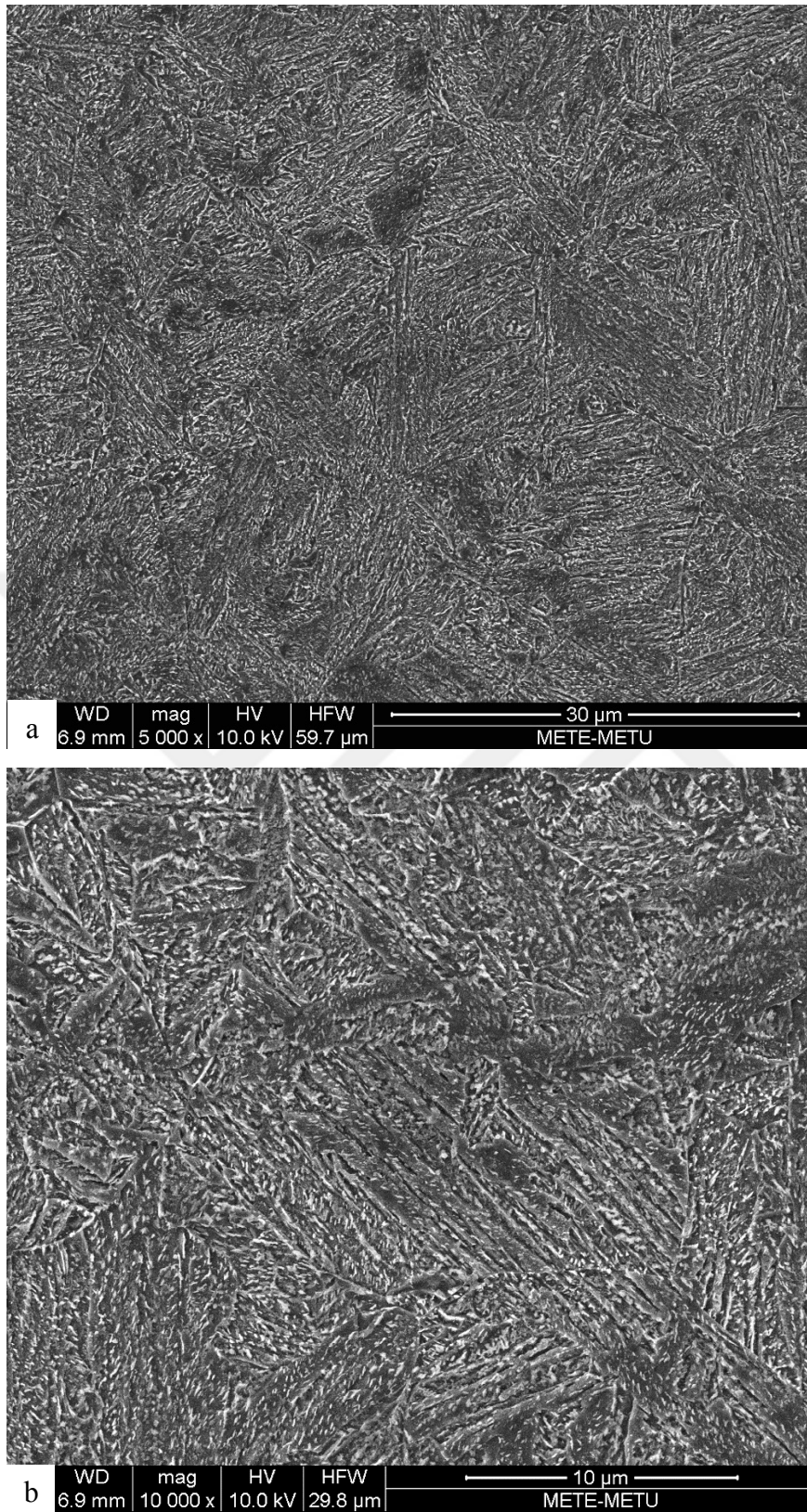
Figure 38. SEM images of 32CrB4 steel quenched to 350°C and hold isothermally for 2 hours. The microstructure is nearly fully bainitic.
