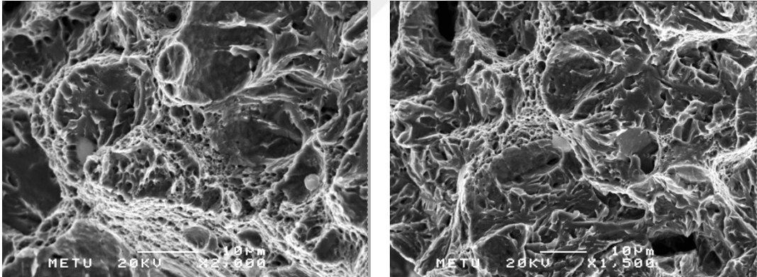
Figure 51. Fracture surface images of 32CrB4 steel that hold isothermally at 350°C for 2 minutes then water quenched and tempered.
