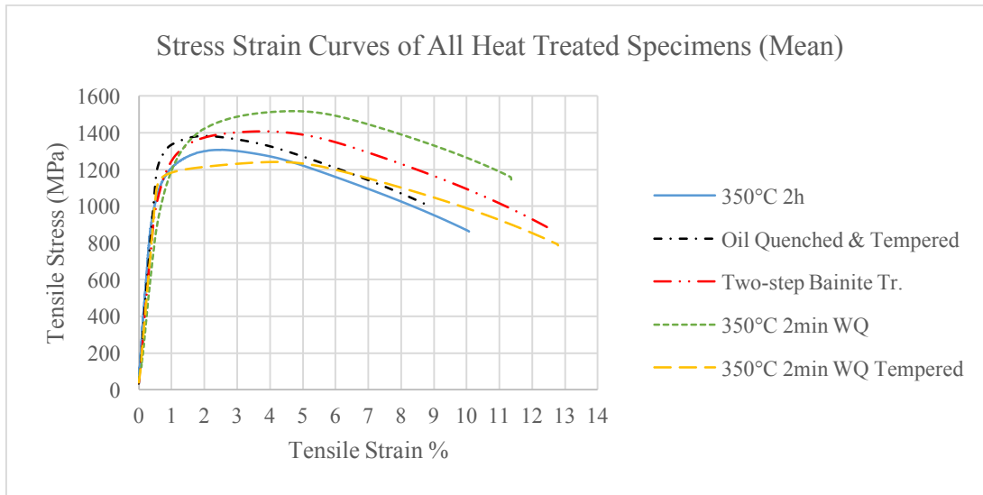
Figure 45. Stress strain curves of heat treated 32CrB4 steel specimens with mean values for each heat treatment process
