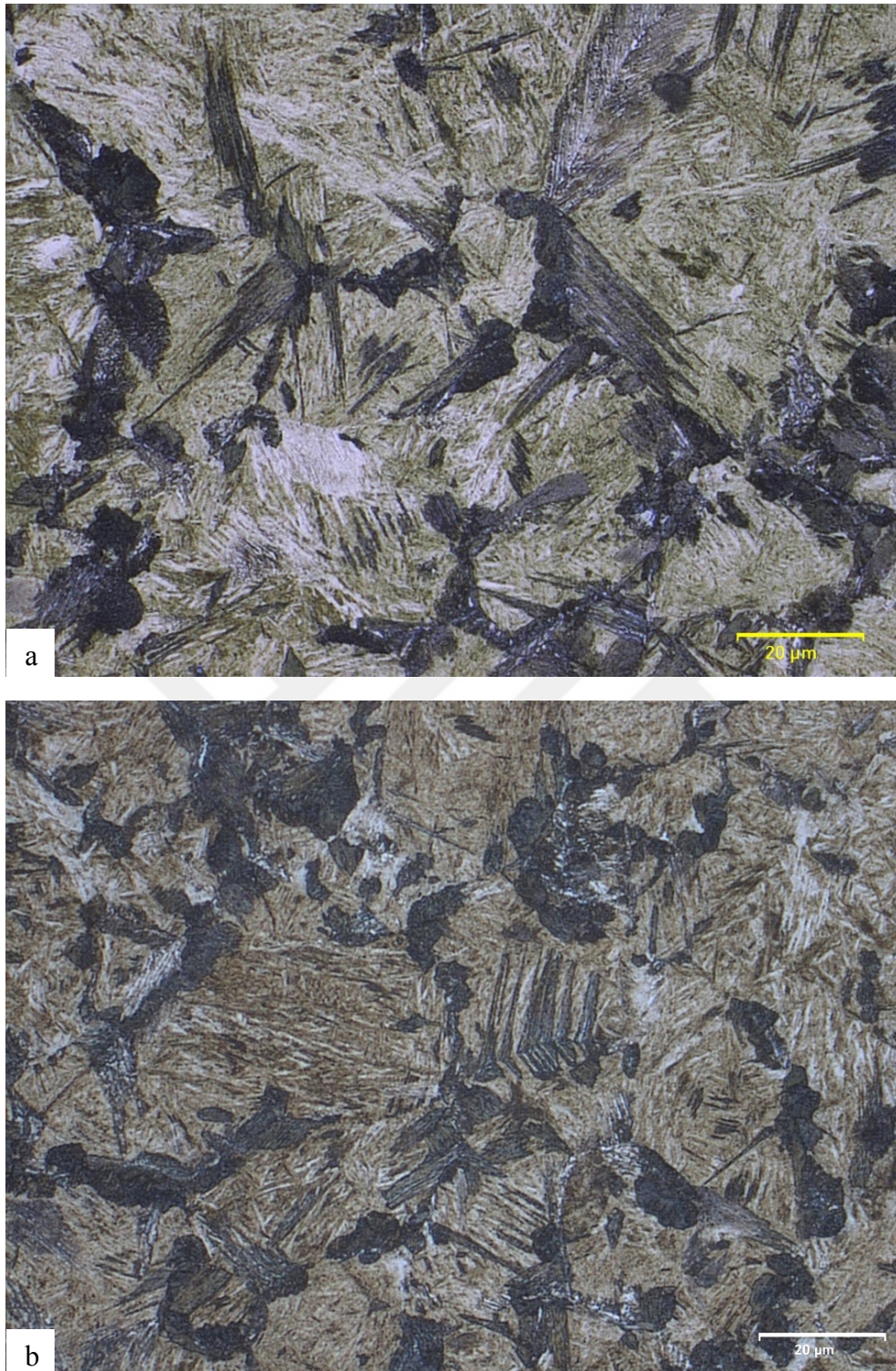
Figure 28. Optical micrographs of R260 steel; (a) quenched to 205°C and hold isothermally for 3 days, (b) quenched to 205°C and hold isothermally for 7 days.
