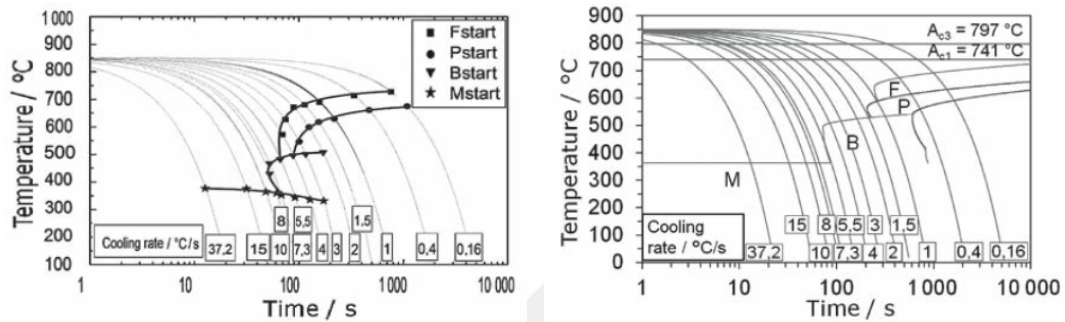
Figure 31. CCT diagram of 32CrB4, (a) drawn by experimental data and (b) drawn by software [26].
