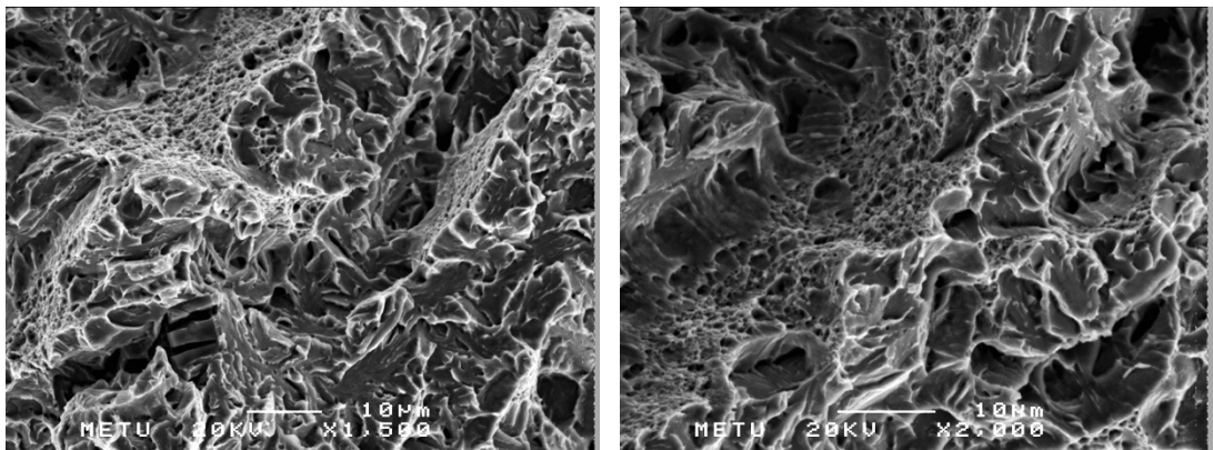
Figure 49. Fracture surface images of 32CrB4 steel that has a two-step bainite transformation
