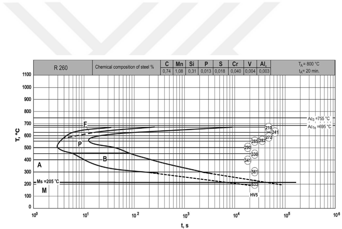
Figure 18. TTT diagram of R260 railway steel [38]
