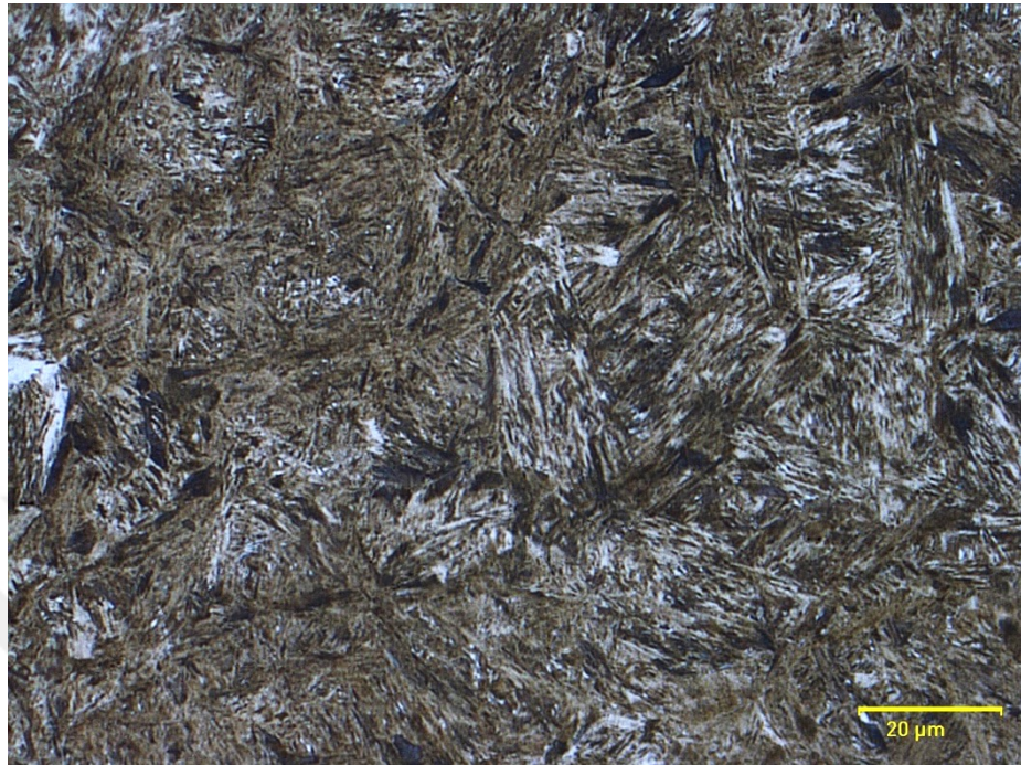
Figure 25. Optical micrograph of martensite phase in R260 steel.
