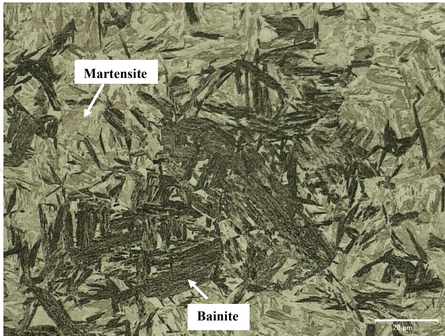
Figure 36. Optical micrograph of 32CrB4 steel, quenched to 350°C and hold for 1 minute and then water quenched. Light contrasted acicular phase is martensite and the dark, feathery constituent is bainite.
