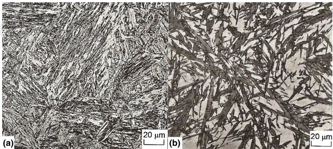
Figure 3. (a) Tempered martensite of 4130 steel, (b) plate martensite of high-carbon steel [8]
