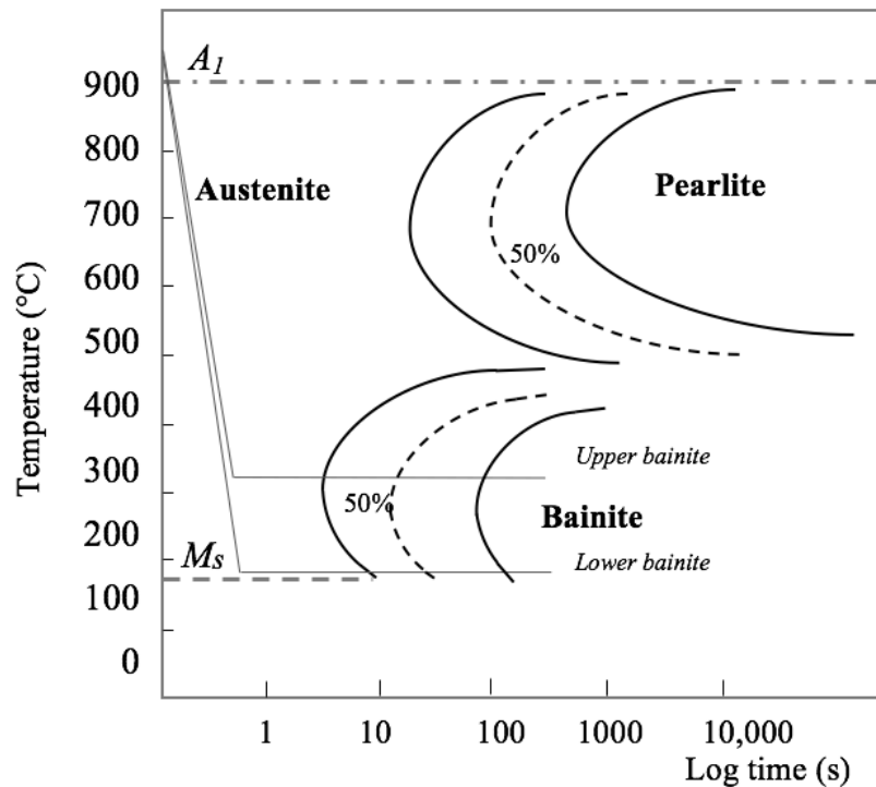
Figure 6. TTT diagram showing upper and lower bainite regions and example of isothermal cooling paths
