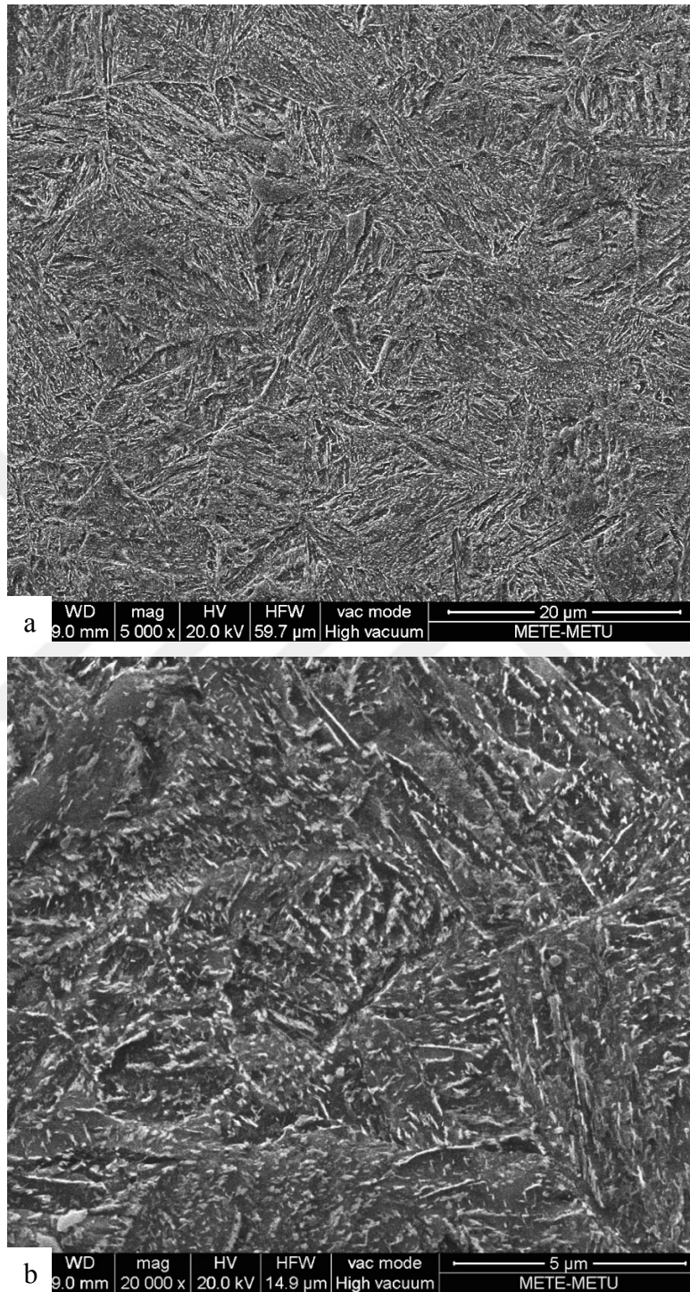
Figure 35. SEM images of 32CrB4 steel, oil quenched and tempered at 450°C for 2 hours. (b) At high magnification, the carbide precipitation can be seen.
