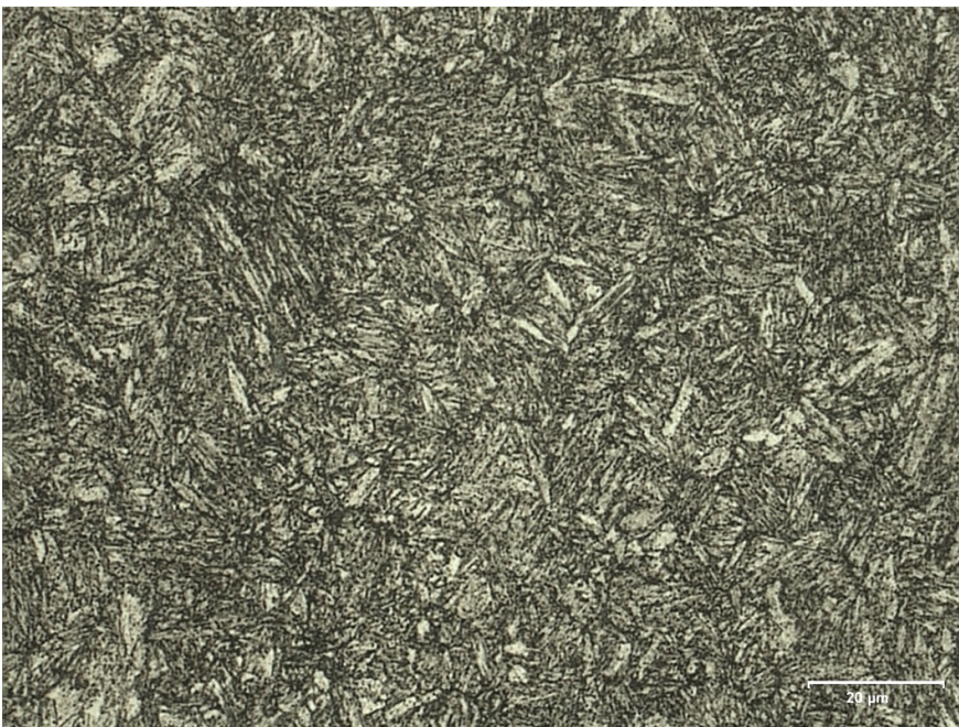
Figure 34. Optical image of tempered martensite of 32CrB4 steel.
