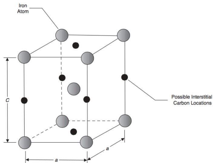
Figure 1. BCT structure of martensite and possible interstitial locations for carbon atom [6]
