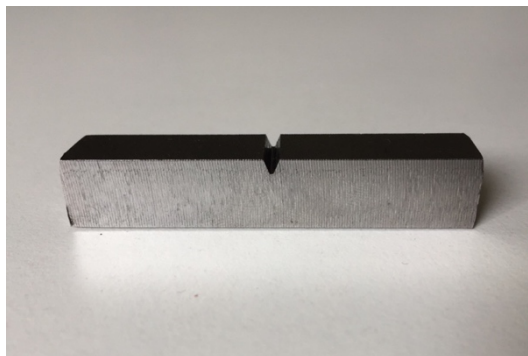
Figure 23. V-notched bar Charpy impact test specimen of 32CrB4 steel
