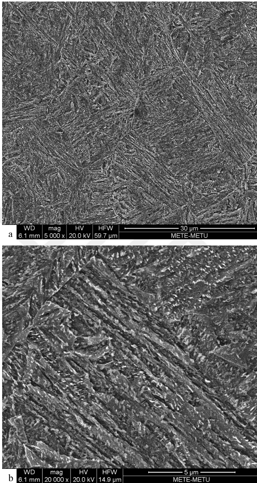
Figure 42. SEM images of two-step quenched specimen (350°C for 2 minutes and 300°C for 5.5 hours). The bainite phase can be seen easily. However, the martensite phase could not be differentiated.
