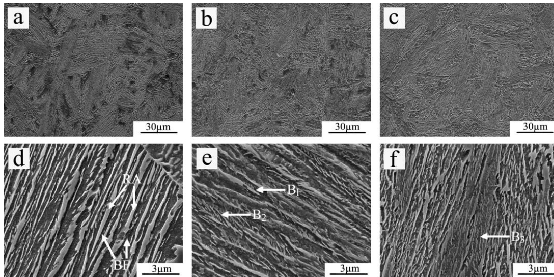
Figure 12. SEM images of (a)(d) conventional bainitic transformation, (b)(e) two-step quenching bainitic transformation, (c)(f) three-step quenching bainitic transformation [5].
