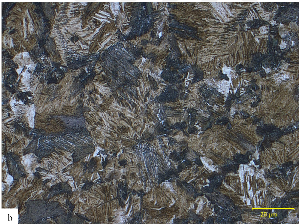
Figure 29. Optical micrographs of R260 steel; isothermally treated for 3 hours after quenched to (a) 220°C, (b) 250°C and (c) quenched to 280°C and transformed isothermally for 1 hour.
