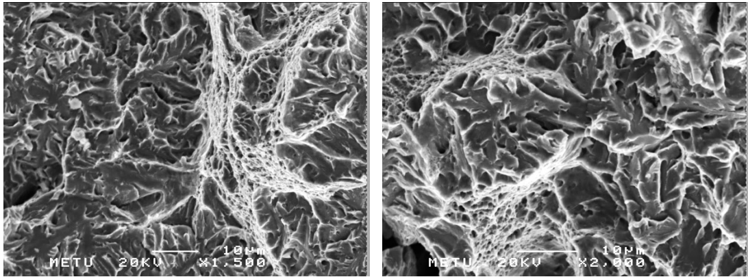
Figure 48. Fracture surface images of 32CrB4 steel quenched to 350°C and hold isothermally for 2 hours.
