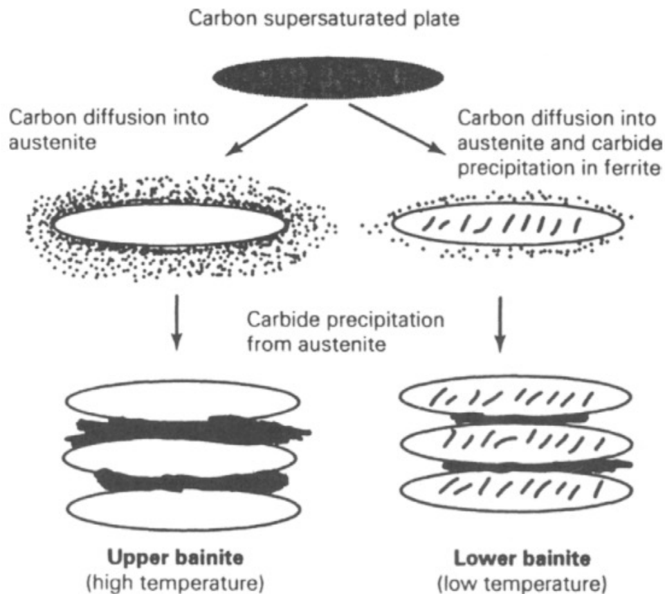
Figure 7. Carbon diffusion and precipitation for upper and lower bainite [14]
