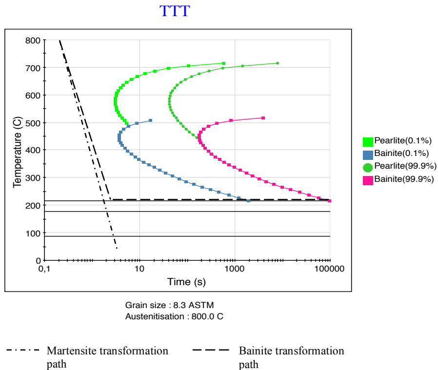
Figure 24. Schematic cooling paths on digital constructed TTT diagram of R260
