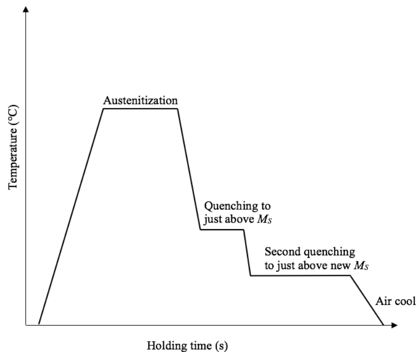
Figure 11. Schematic heat treatment path for two-step quenching process
