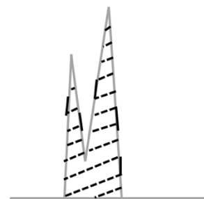
Lower bainite
