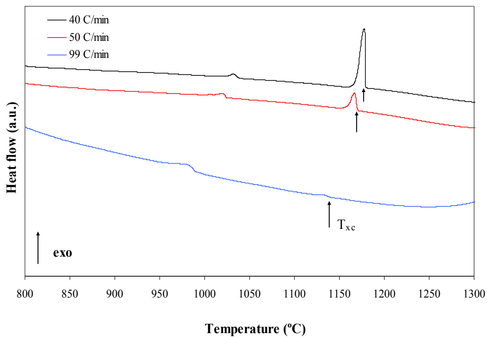
Figure 4.22 DSC cooling curves of Fe 60 Co 8 Zr 10 Mo 5 W 2 B 15 amorphous alloy at various cooling rates.
