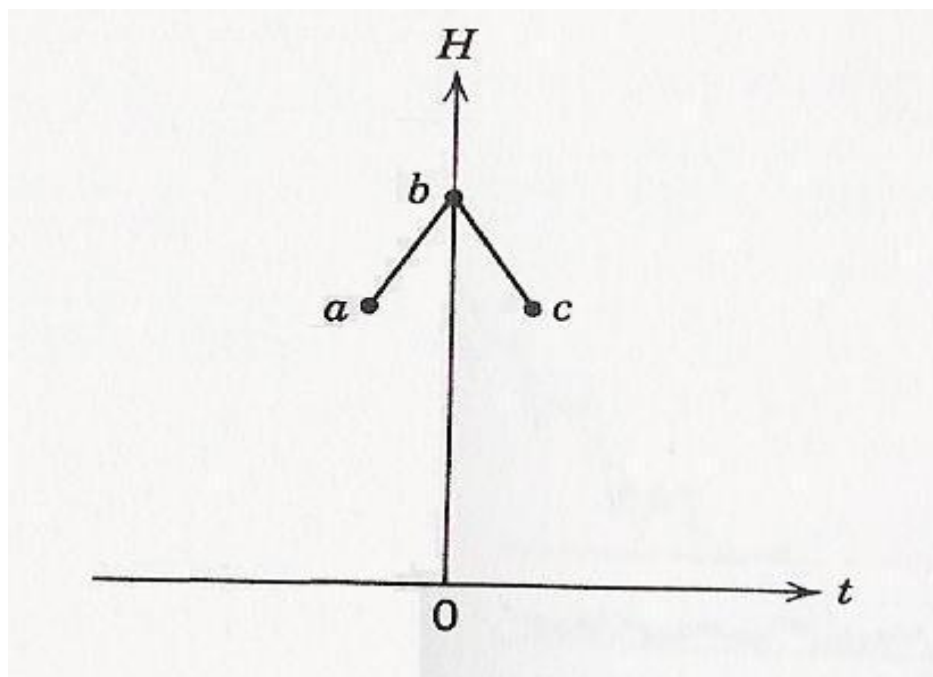
Figure 4.2: H Function and Local Peak
