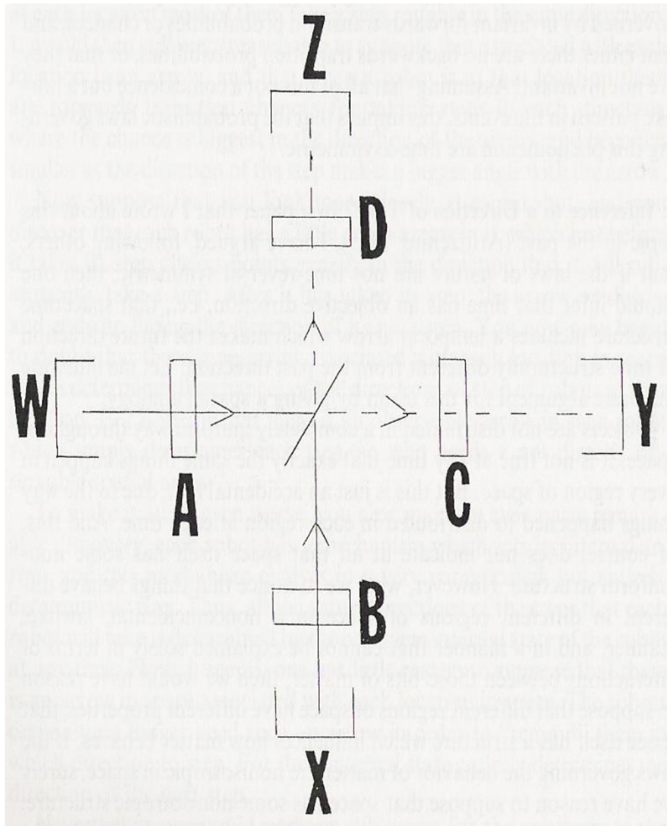
Figure 5.1: Arntzenius Gedanken Experiment
