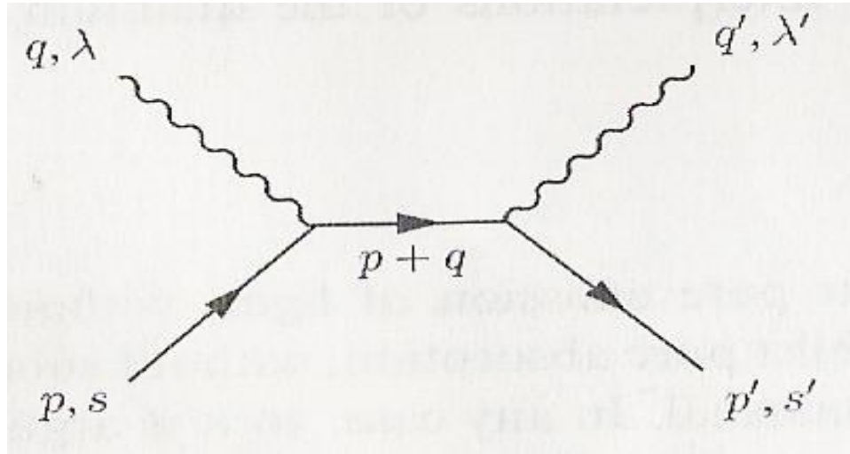
Figure 5.2: Compton Scattering
