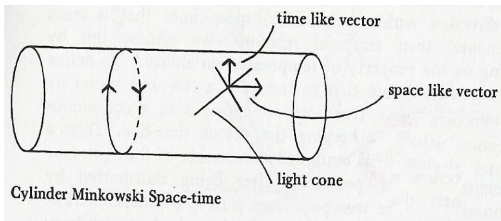
Figure 4.6: Cylinder Minkowski Space-time
