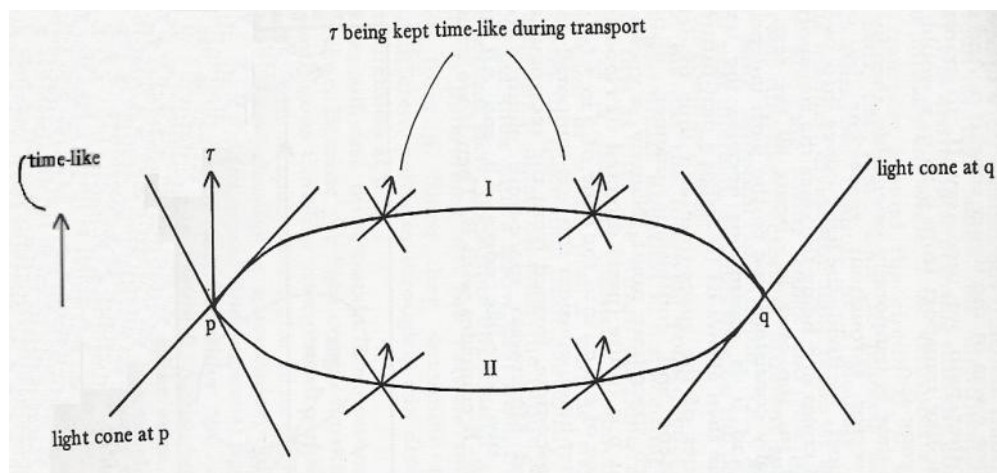
Figure 4.7: Parallel Transport
