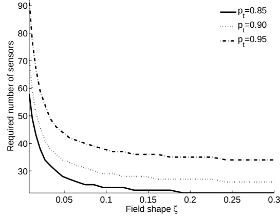
Figure 4.4. The effect of field shape parameter \zeta = D_2/D_1 on the required number of sensors for different threshold detection probabilities where total area is 3000 m 2 , d_t = 10 meters
