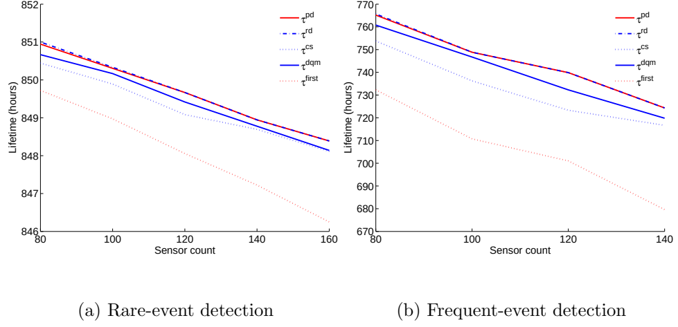
Figure 5.5. The effect of the number of sensors on the network lifetime
