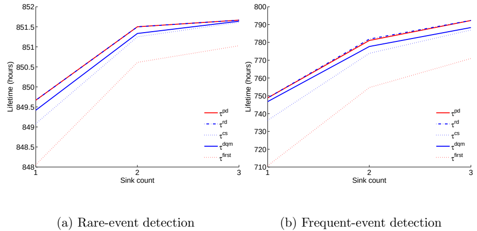
Figure 5.6. The effect of deployed number of sinks on the network lifetime
