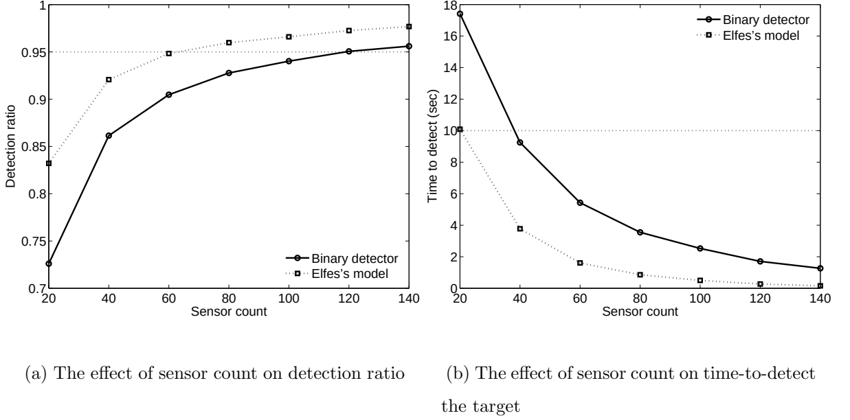
Figure 2.23. The effect of sensor count on the detection ratio and time-to-detect the target when binary or Elfes's detectors are utilized
