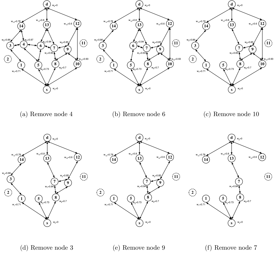
Figure 3.8. Trace of Algorithm in Figure 3.7. This is the auxiliary graph of the watershed contours in Figure 3.4 produced using Algorithm in Figure 3.5
