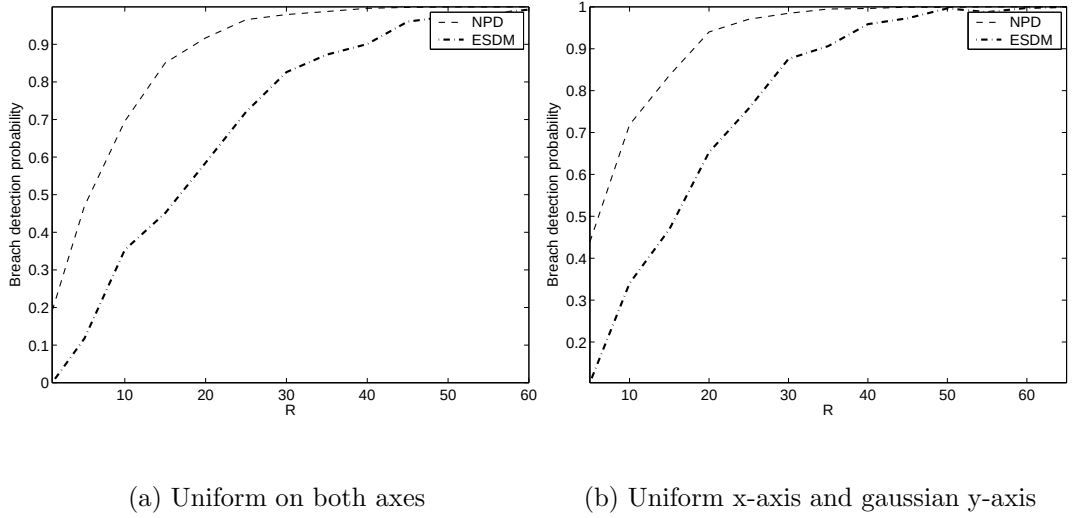
Figure 2.7. The effect of the number of sensors, R , on the breach detection probability
