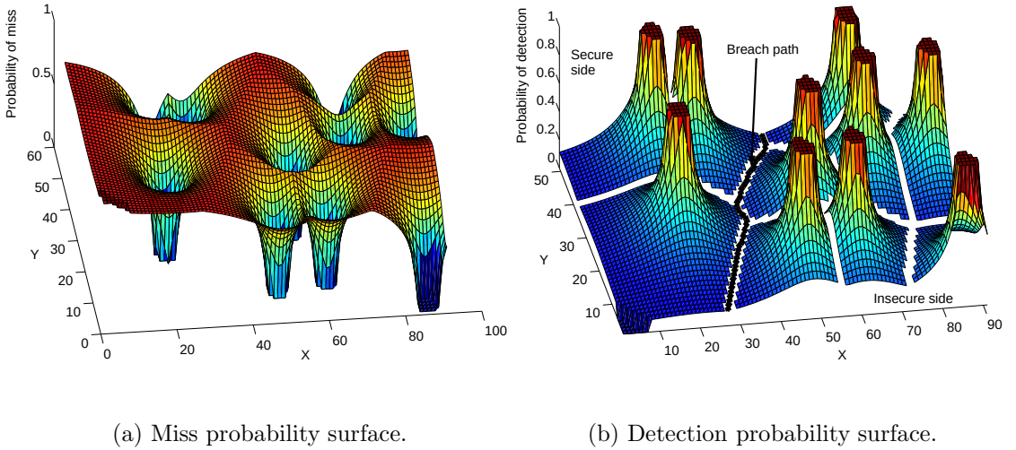
Figure 2.17. Miss probability surface and watershed segmentation shown on the detection probability surface where length=50 m, width=50 m, boundary=20 m., grid size=1 m., R = 10 , r = 15 m., r_e = 12 m., \lambda = 0.5 and \beta = 0.5 .
