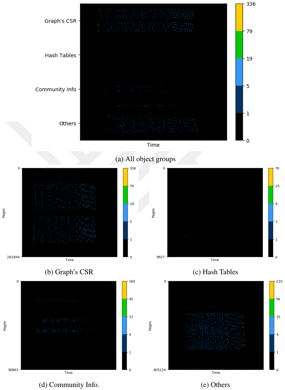
Figure 4.14. Page fault charts of Long_Coup_dt6 dataset at 30% oversubscription.
