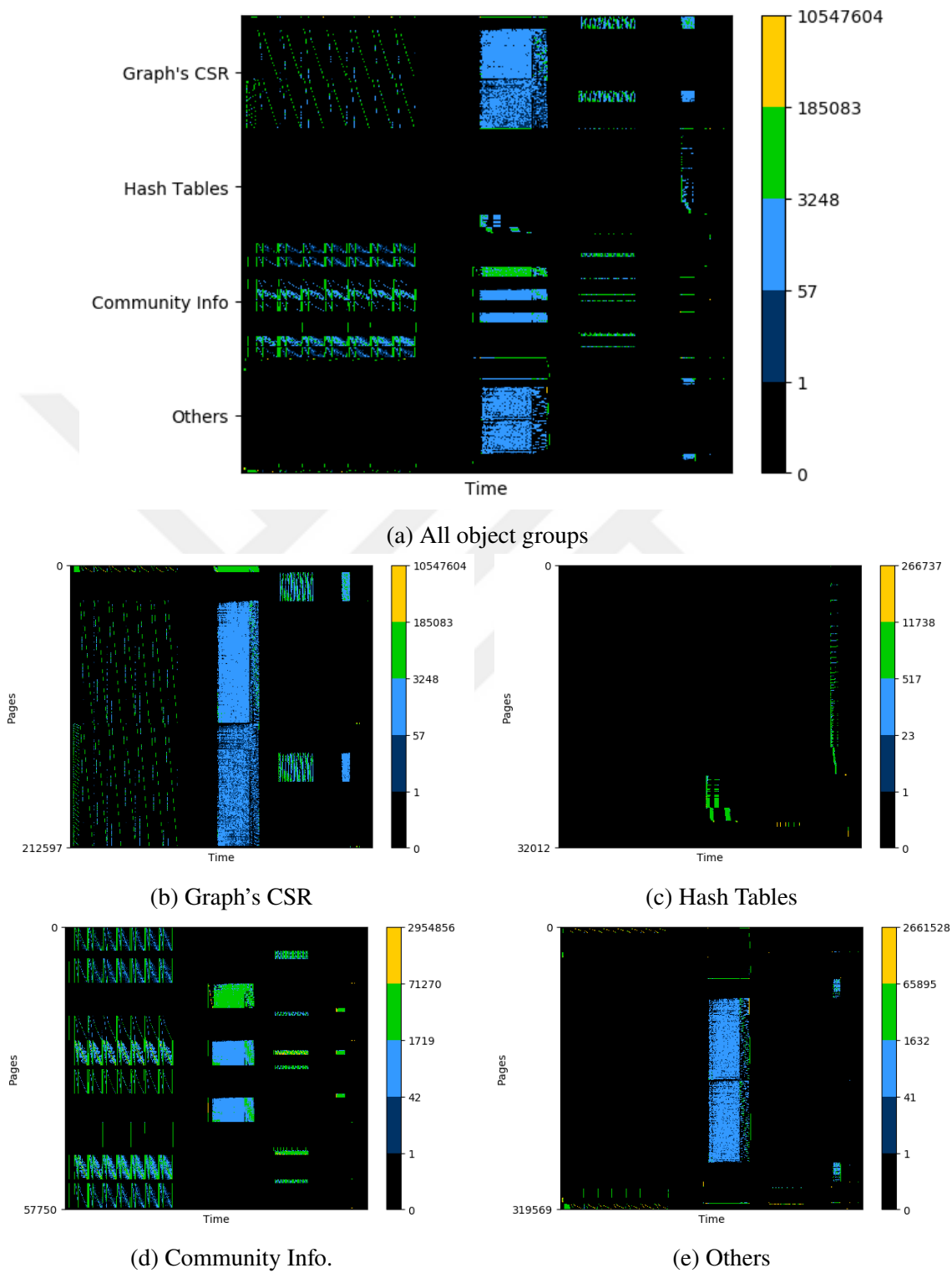
Figure 4.6. Memory accesses of each object group for cage15 dataset.
