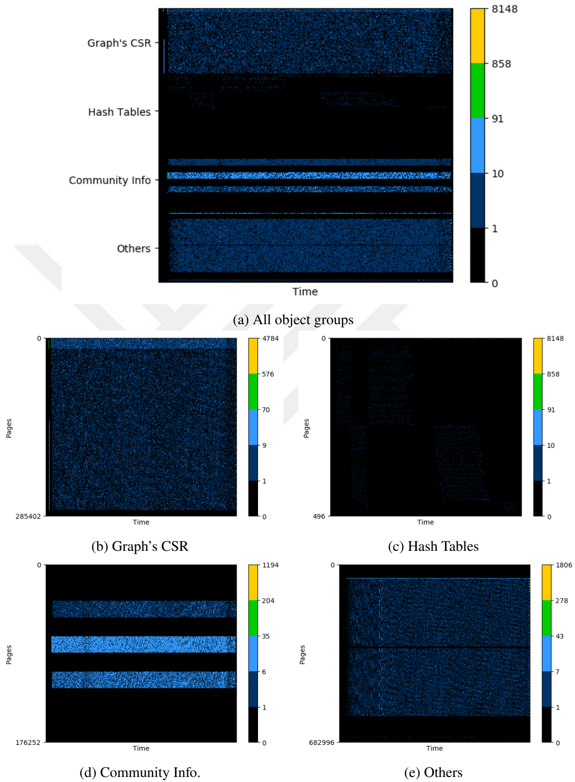
Figure 4.17. Page fault charts of rgg_n_2_24_s0 dataset at 30% oversubscription.
