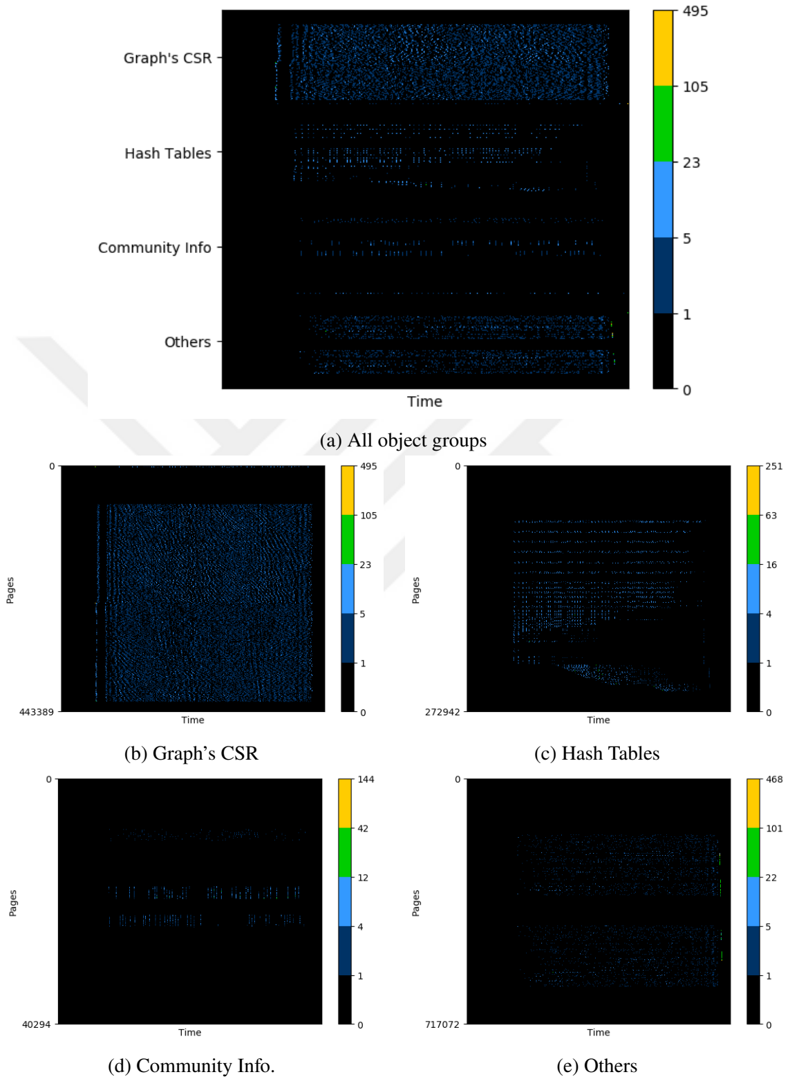
Figure 4.18. Page fault charts of kron_g500-logn21 dataset at 30% oversubscription.
