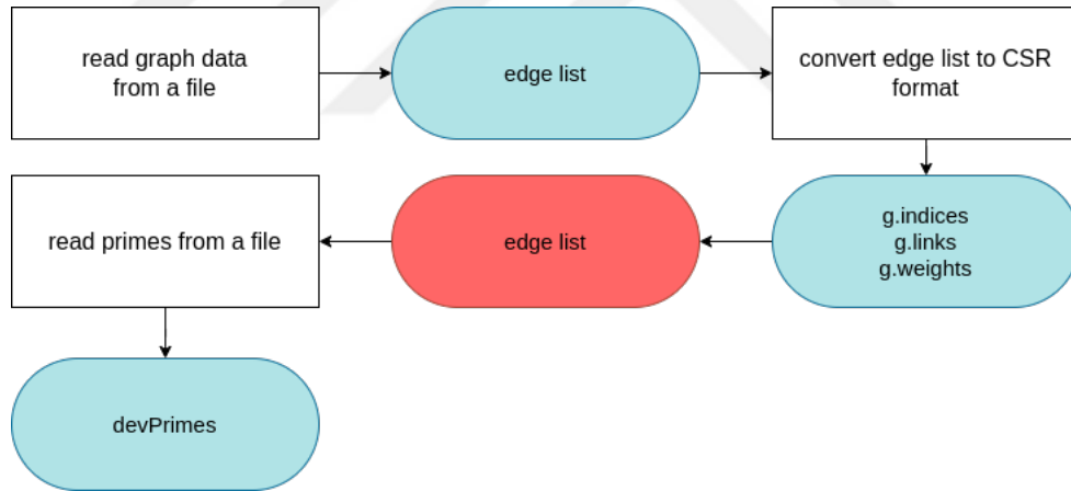
Figure 3.1. Initialization phase's flow chart.
