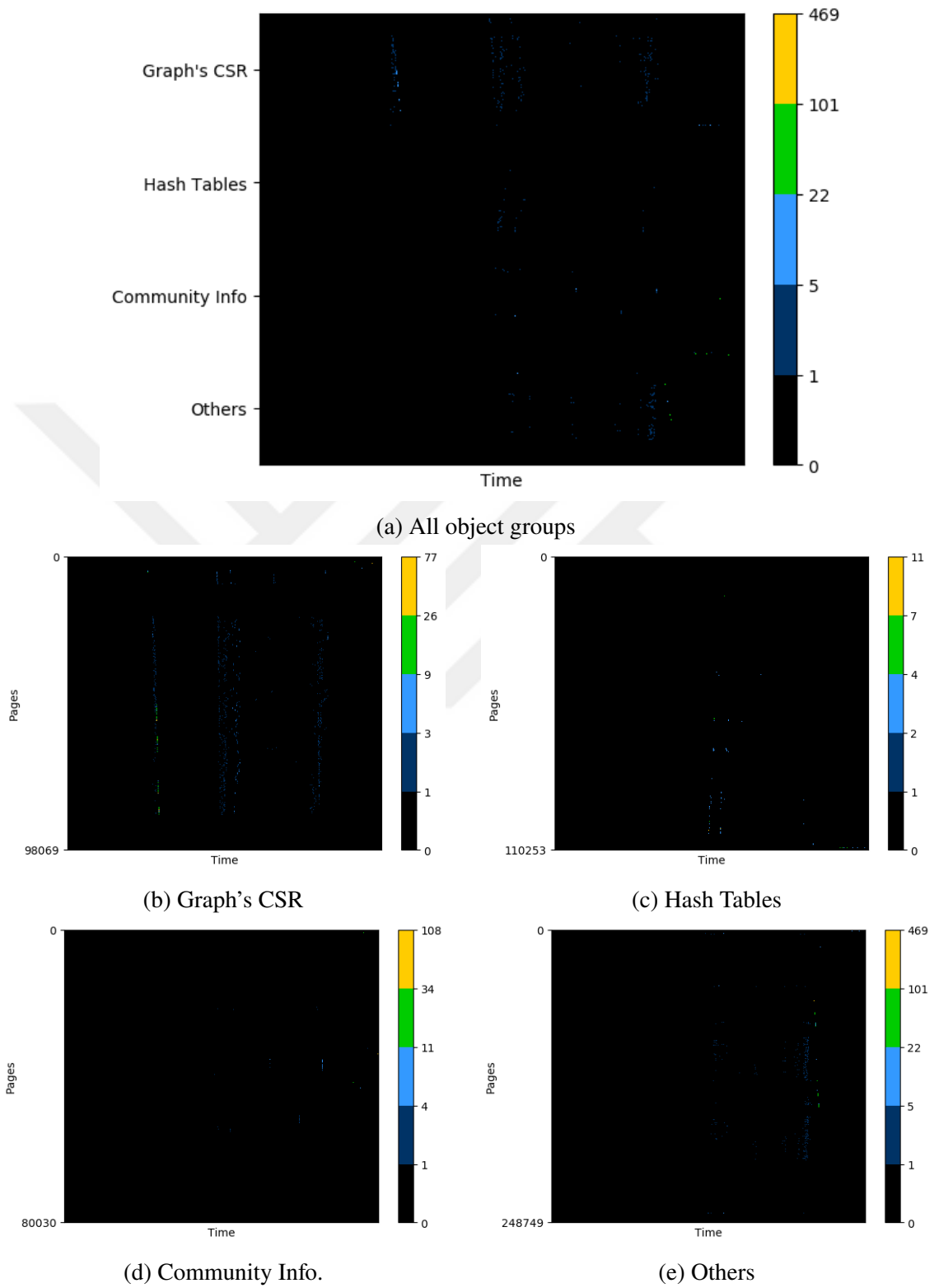
Figure 4.13. Page fault charts of soc-LiveJournal1 dataset at 30% oversubscription.
