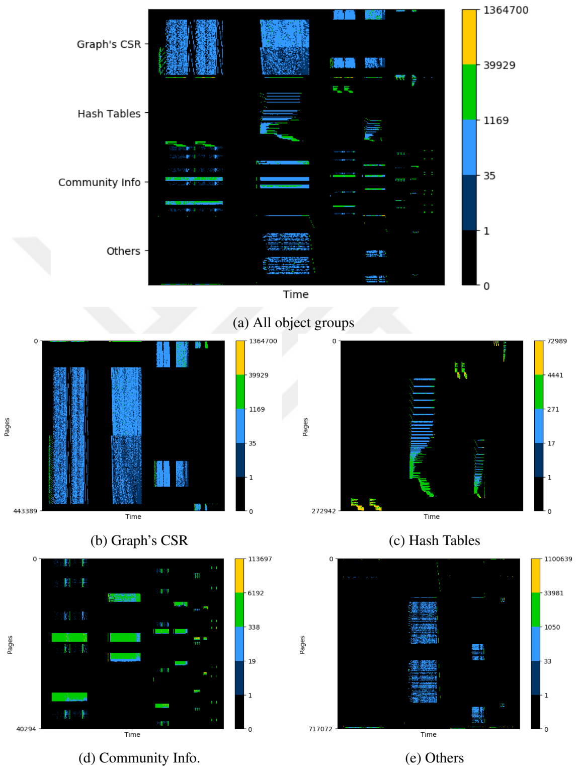
Figure 4.8. Memory accesses of each object group for kron_g500-logn21 dataset.
