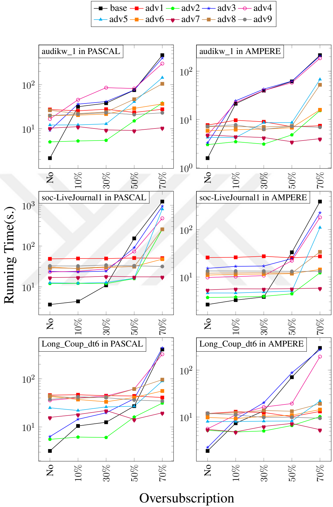
Figure 4.20. The running times of Rundemanen for several datasets with memory advises at different oversubscription rates (I).
