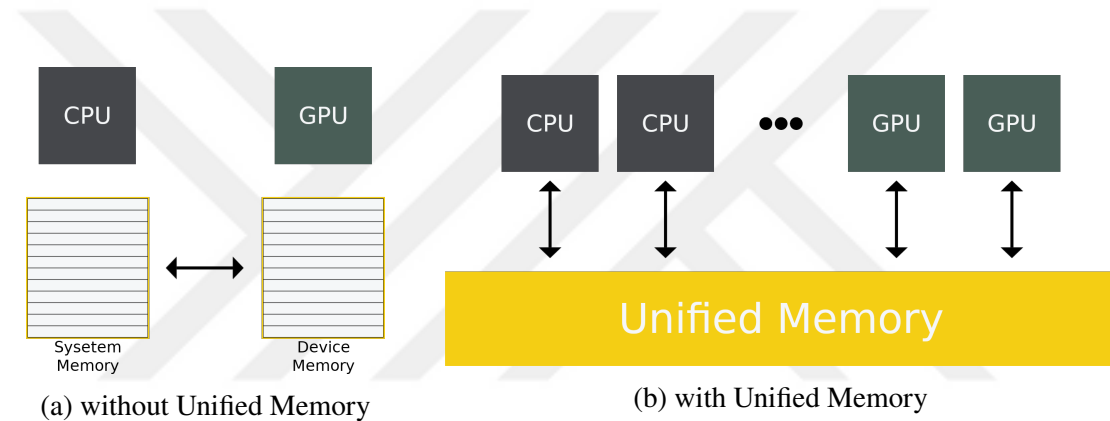
Figure 2.4. Pictorial view of Unified Memory.
