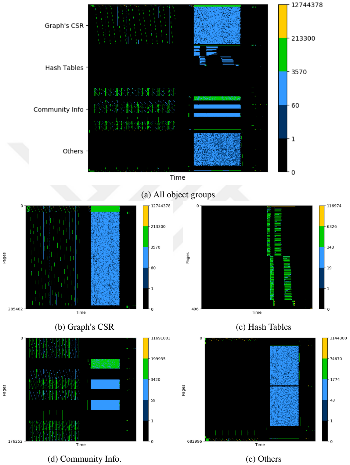
Figure 4.7. Memory accesses of each object group for rgg_n_2_24_s0 dataset.
