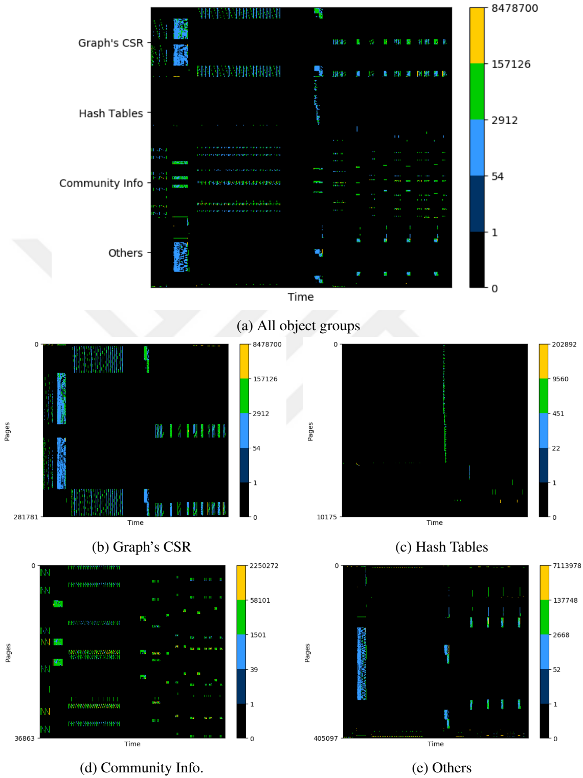
Figure 4.4. Memory accesses of each object group for Long_Coup_dt6 dataset.
