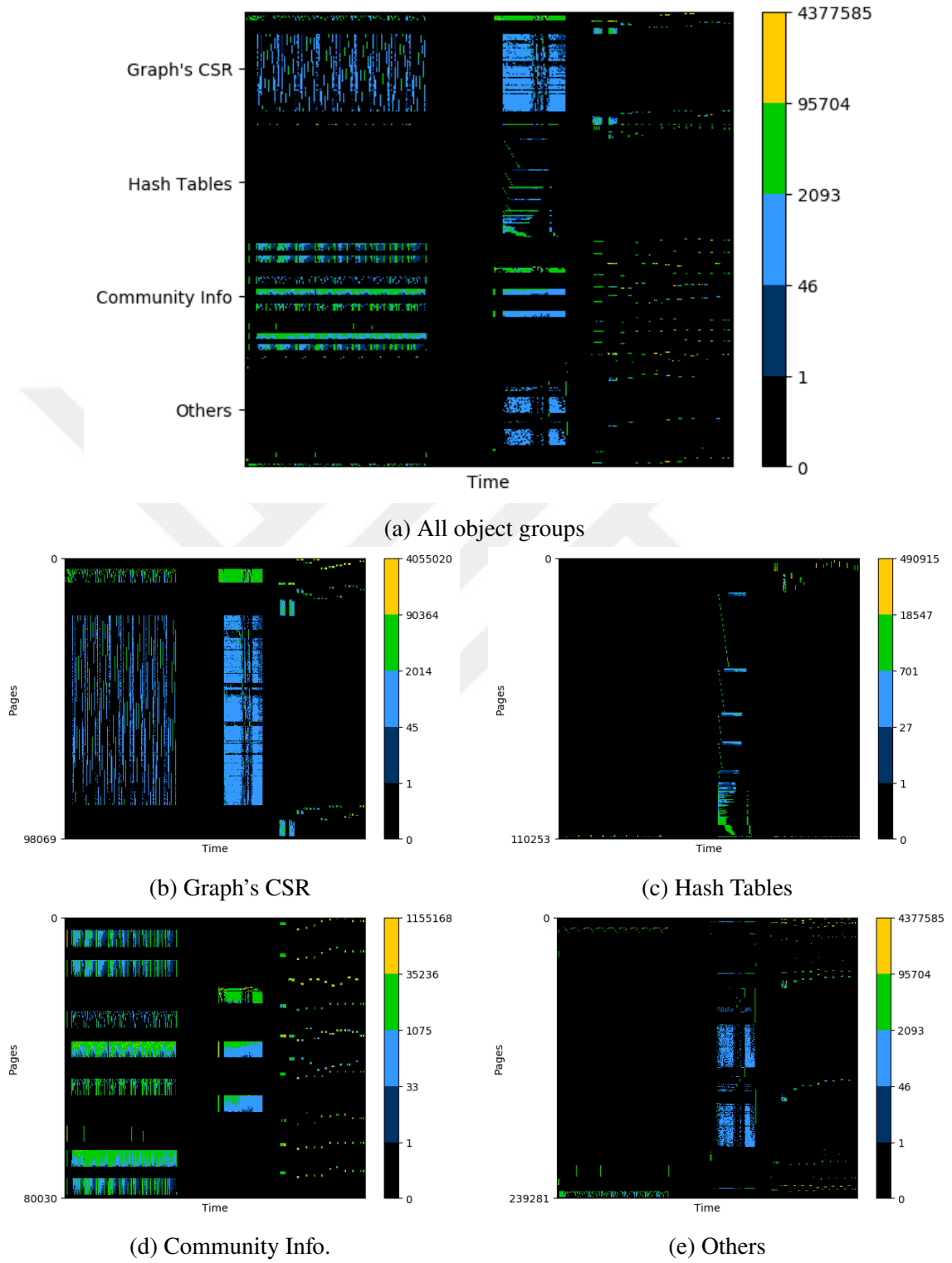
Figure 4.3. Memory accesses of each object group for soc-LiveJournal1 dataset.
