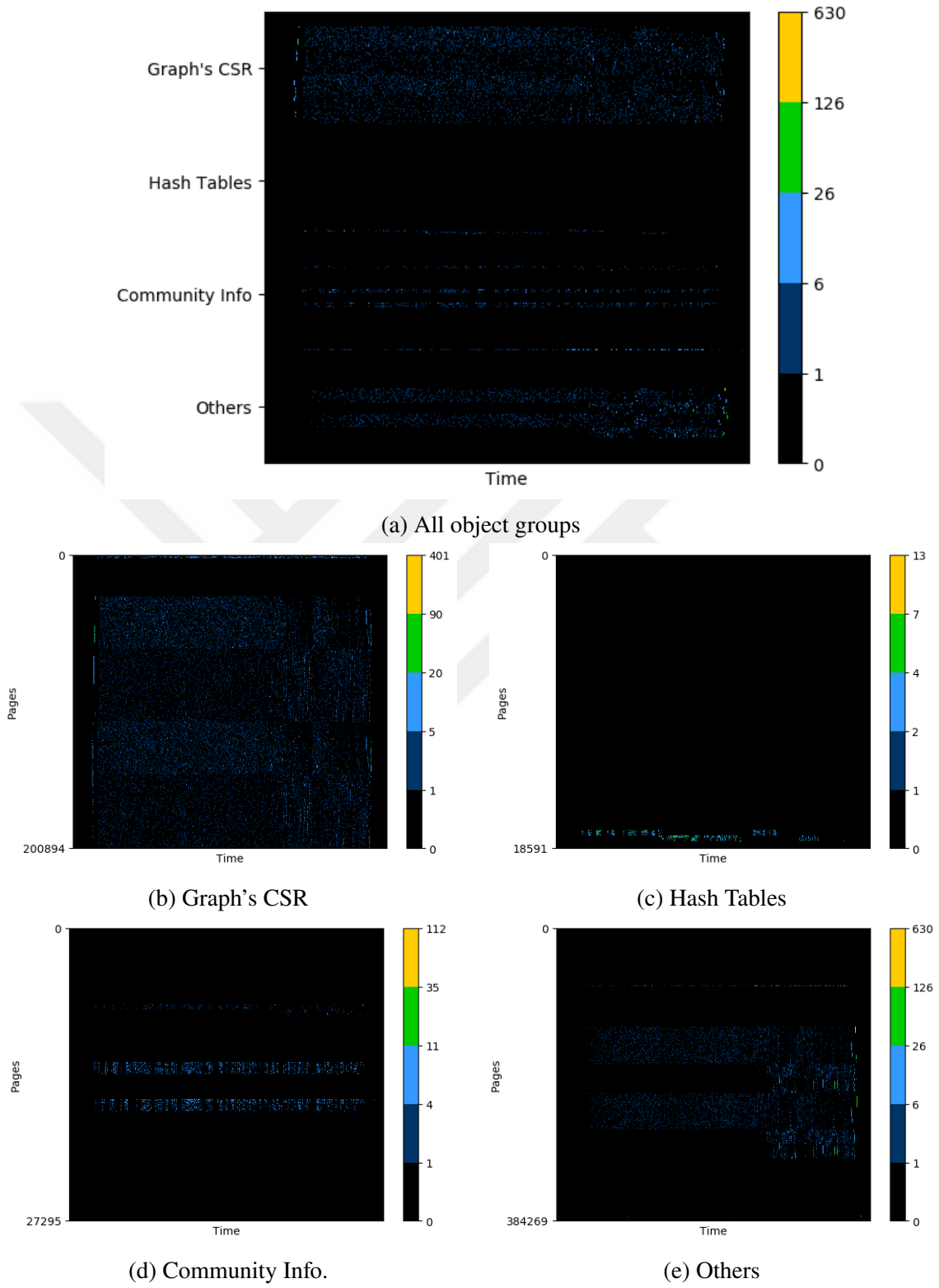
Figure 4.15. Page fault charts of dielFilterV3real dataset at 30% oversubscription.
