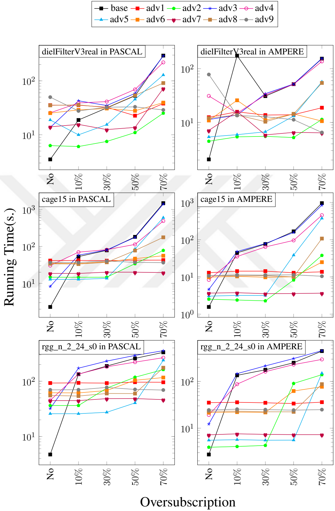
Figure 4.21. The running times of Rundemanen for several datasets with memory advises at different oversubscription rates (II).
