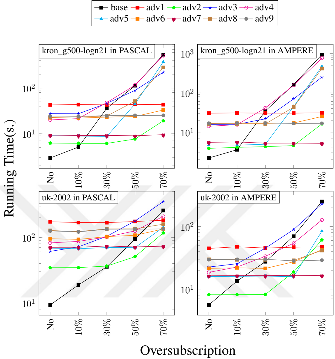
Figure 4.22. The running times of Rundemanen for several datasets with memory advises at different oversubscription rates (III).
