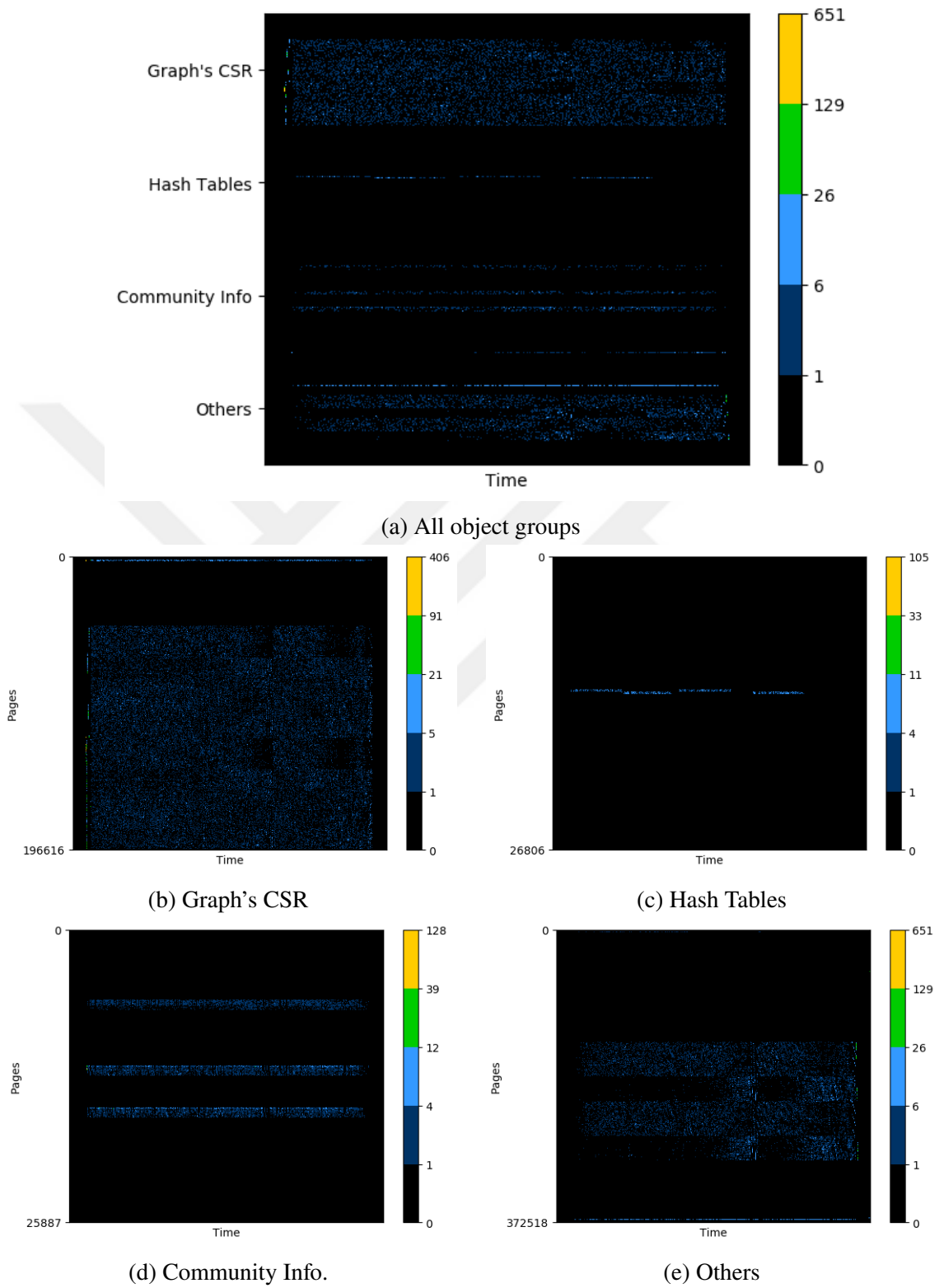
Figure 4.12. Page fault charts of audikw_1 dataset at 30% oversubscription.
