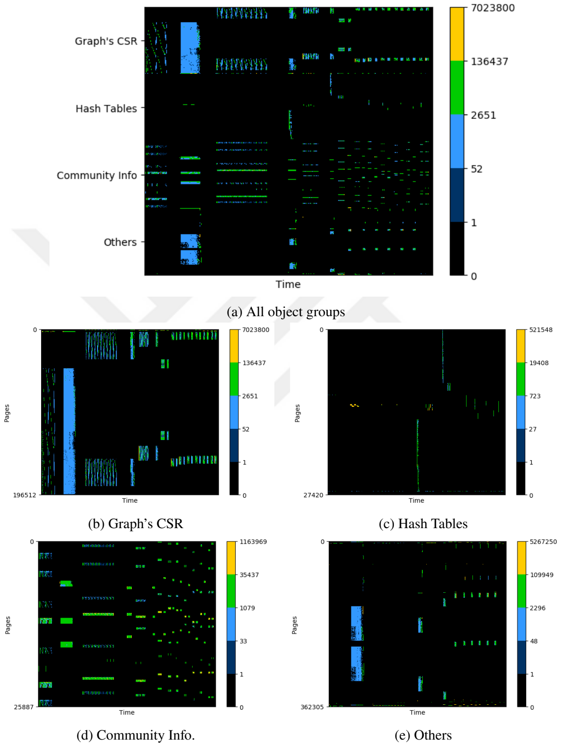
Figure 4.2. Memory accesses of each object group for audikw_1 dataset.
