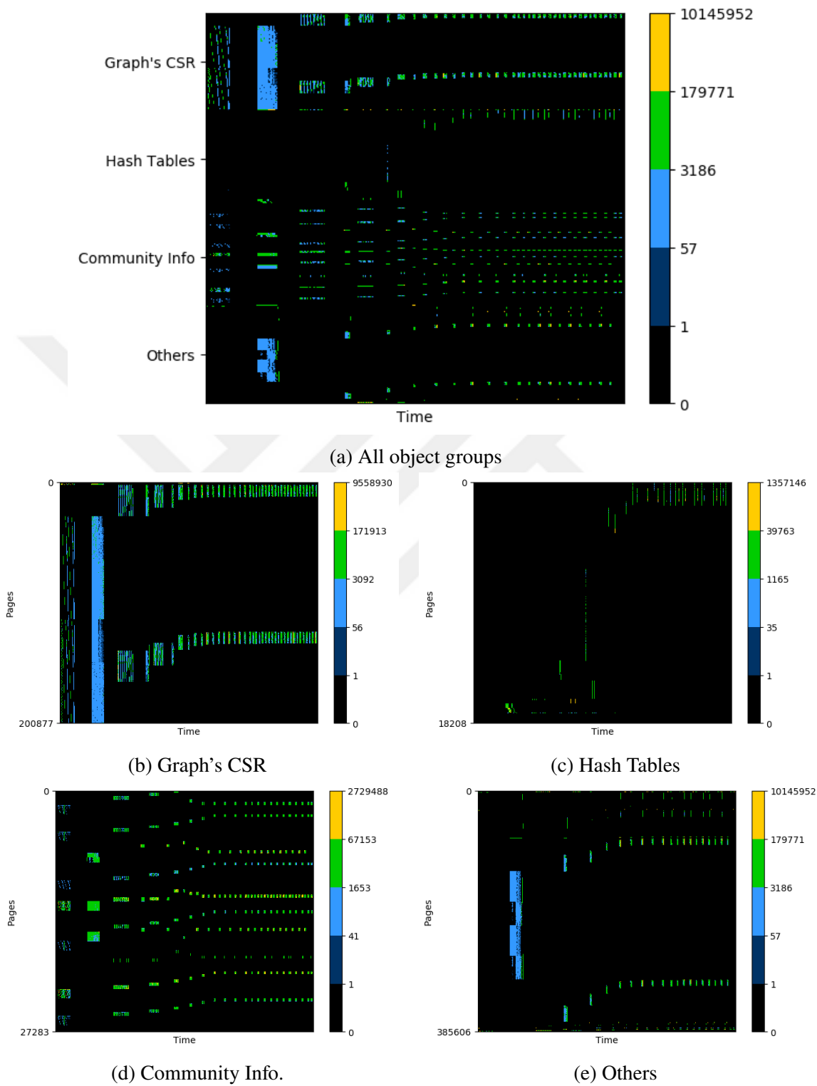
Figure 4.5. Memory accesses of each object group for dielFilterV3real dataset.
