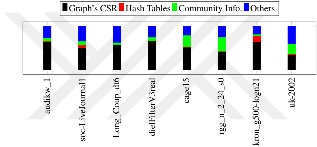
Figure 4.10. Page fault ratios of each object group for all datasets at 30% oversubscription collected in the PASCAL environment.
