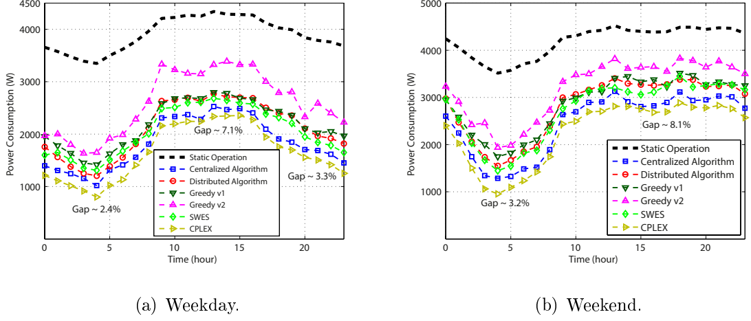
Figure 5.15. Comparative power consumption throughout a day.
