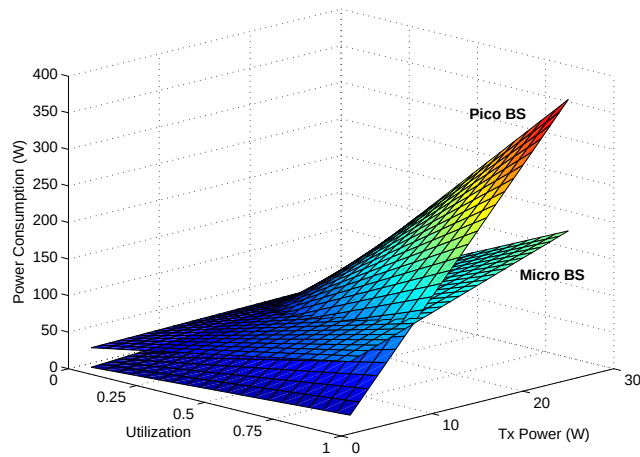
Figure 5.9. Change of micro and pico BS power consumption with utilization and tx power.
