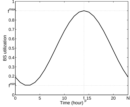
Figure 3.2. An example sinusoidal traffic load for 24h with f^{\min} = 0.1 , f^{\max} = 0.9 , and t^p = 14 h.
