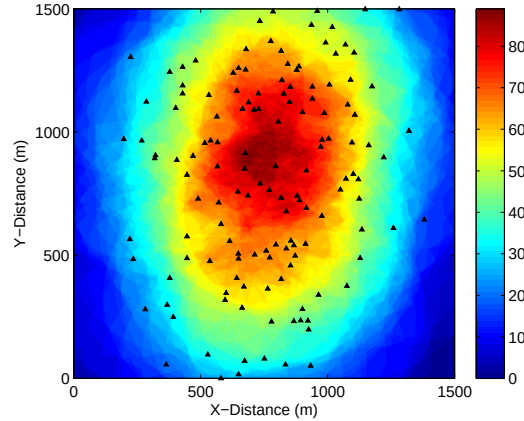
Figure 1.1. Base station location and coverage redundancy of a single operator based on the RSSI value from Sydney Central Business District, Australia.
