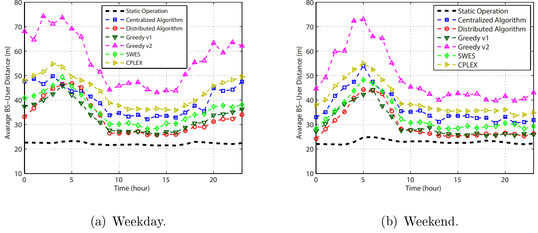
Figure 5.17. Average BS-user distance.
