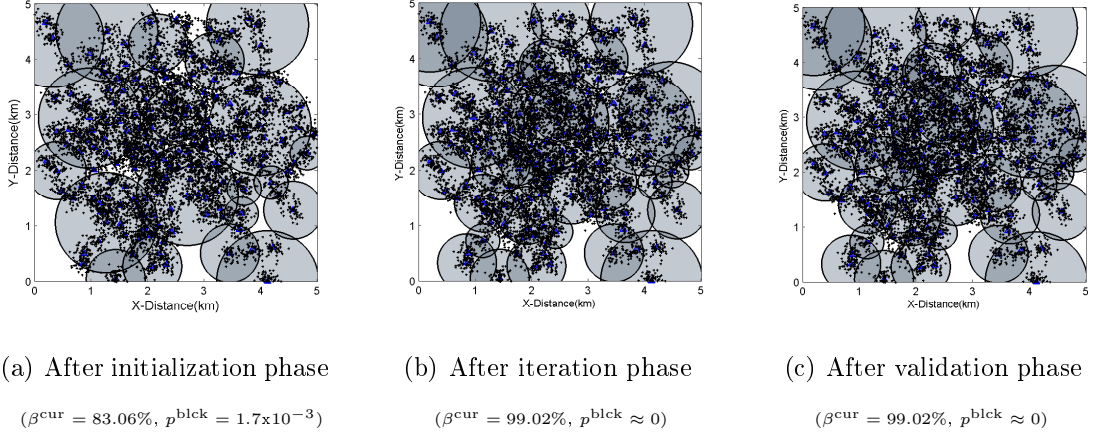
Figure 3.8. Resulting coverage of FastWISE under light traffic load.
