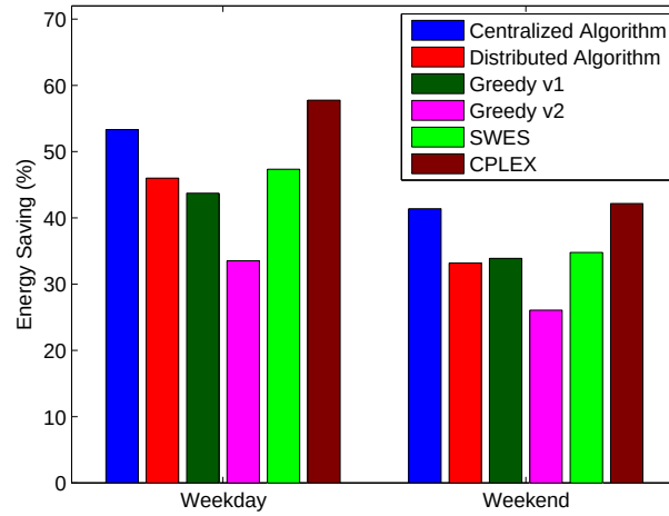
Figure 5.16. Comparative power saving ratio on weekday and weekend.
