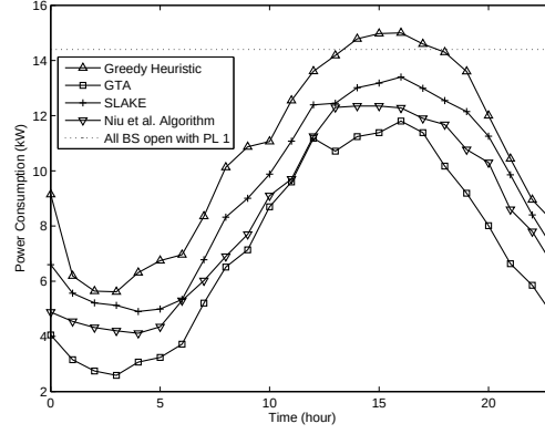
Figure 4.6. Comparative power consumption throughout a day for the large test scenario.
