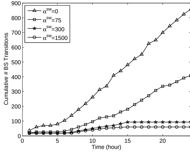
Figure 3.7. Effect of \alpha^{sw} on the cumulative number of BS on/off transitions.
