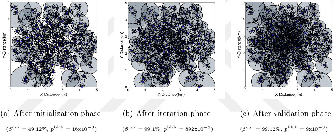
Figure 3.9. Resulting coverage of FastWISE under heavy traffic load.
