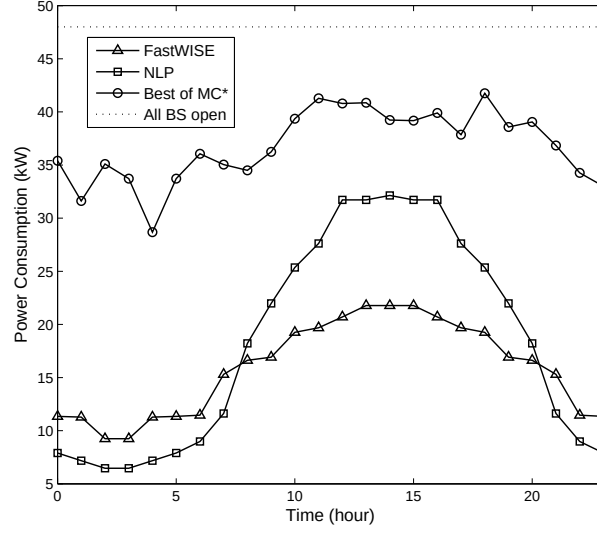
Figure 3.4. Comparative power consumption throughout a day.
