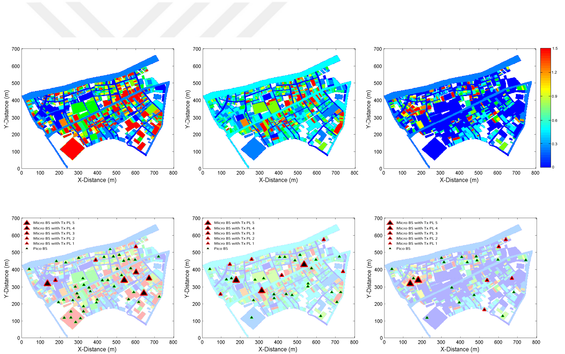
Figure 5.19. User density heat map and corresponding active BS status for time slot 10:00-20:00-02:00 on a weekday.
