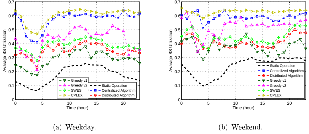
Figure 5.18. Average BS utilization.
