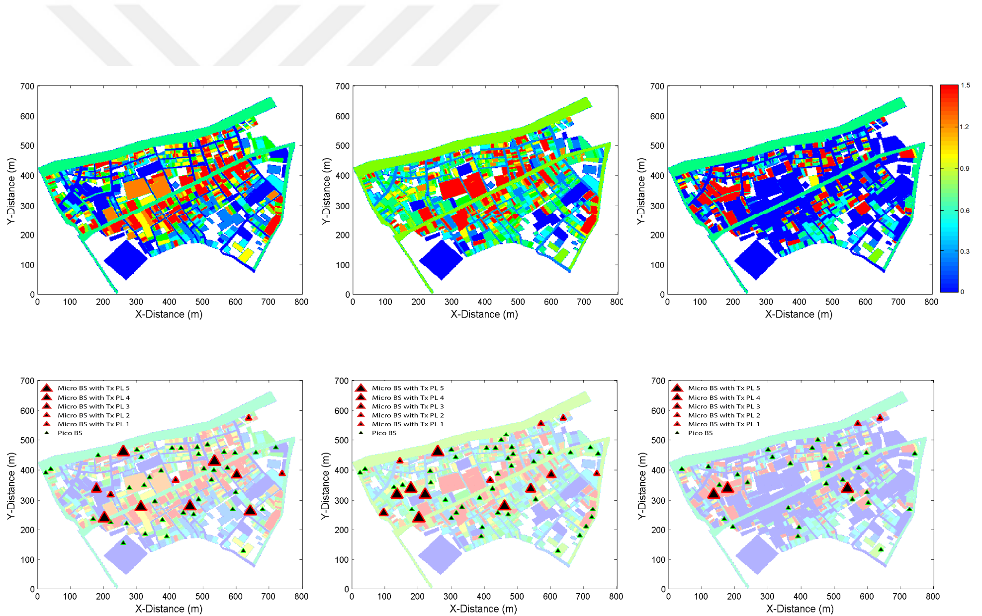
Figure 5.20. User density heat map and corresponding active BS status for time slot 10:00-20:00-02:00 at weekend.
