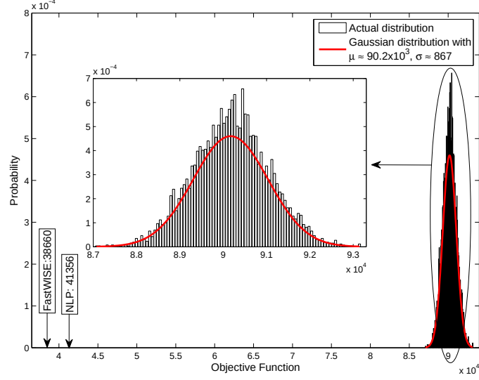
Figure 3.5. Distribution of feasible MC experiments and its comparison with FastWISE and NLP.
