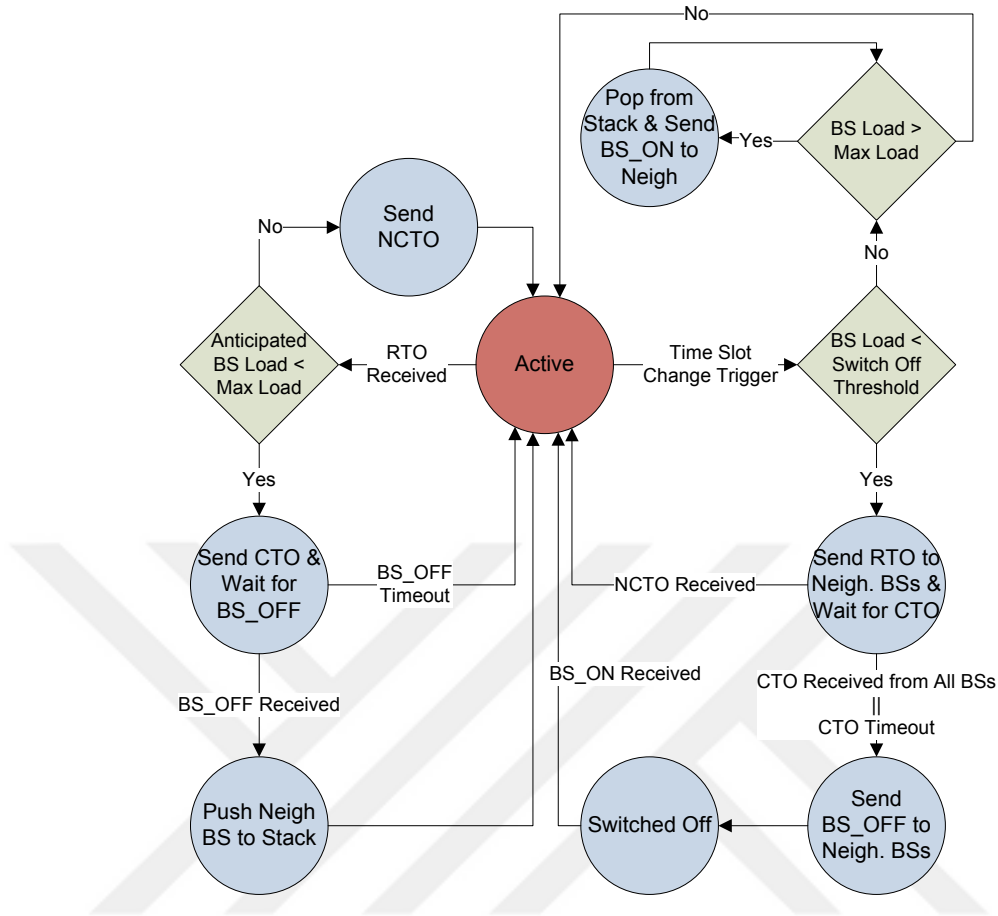
Figure 5.11. Simplified state transition diagram of the online-distributed dynamic BS operation algorithm.
