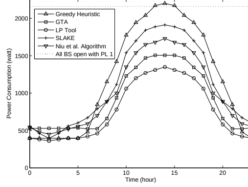
Figure 4.5. Comparative power consumption throughout a day for the small test scenario.
