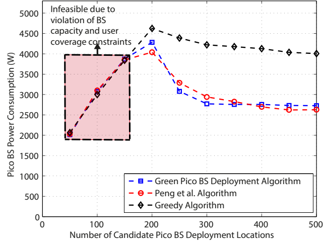
Figure 5.14. Comparative pico BS power consumption during peak traffic
