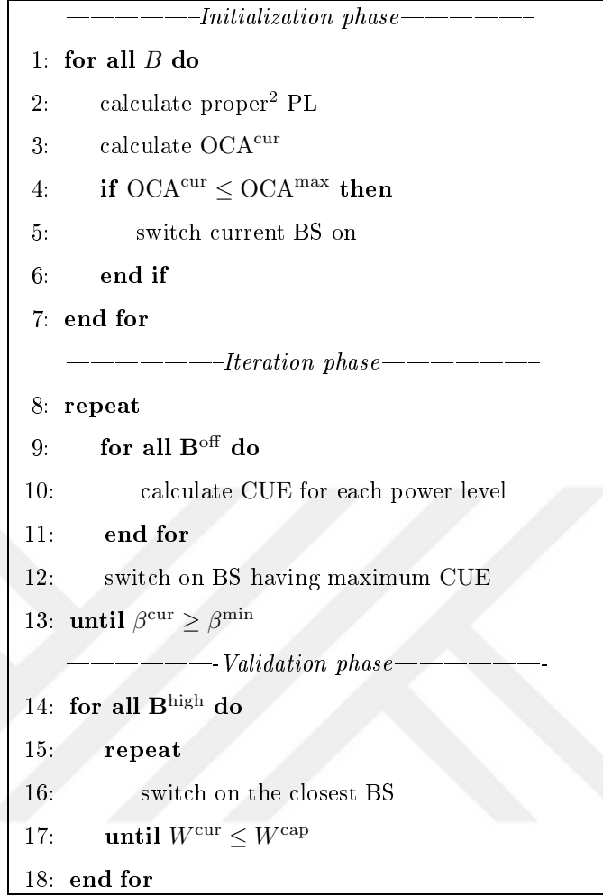
Figure 3.1. FastWISE algorithm.
