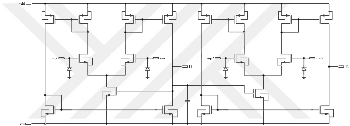
Figure 7.7 : Schematic of adaptive resistive g_m circuit [60]
