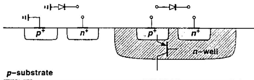
Figure 3.1 : Pn-diode structures.
