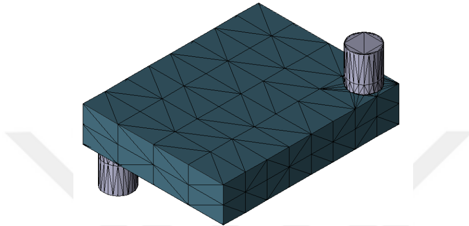
Figure 8.3 : 3D mesh of a metal interconnect (Synopsys TCAD tool).
