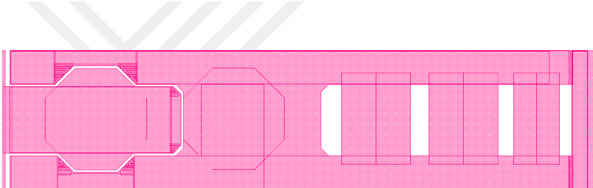
Figure 7.40 : NMOS unit pass device metal 5.
