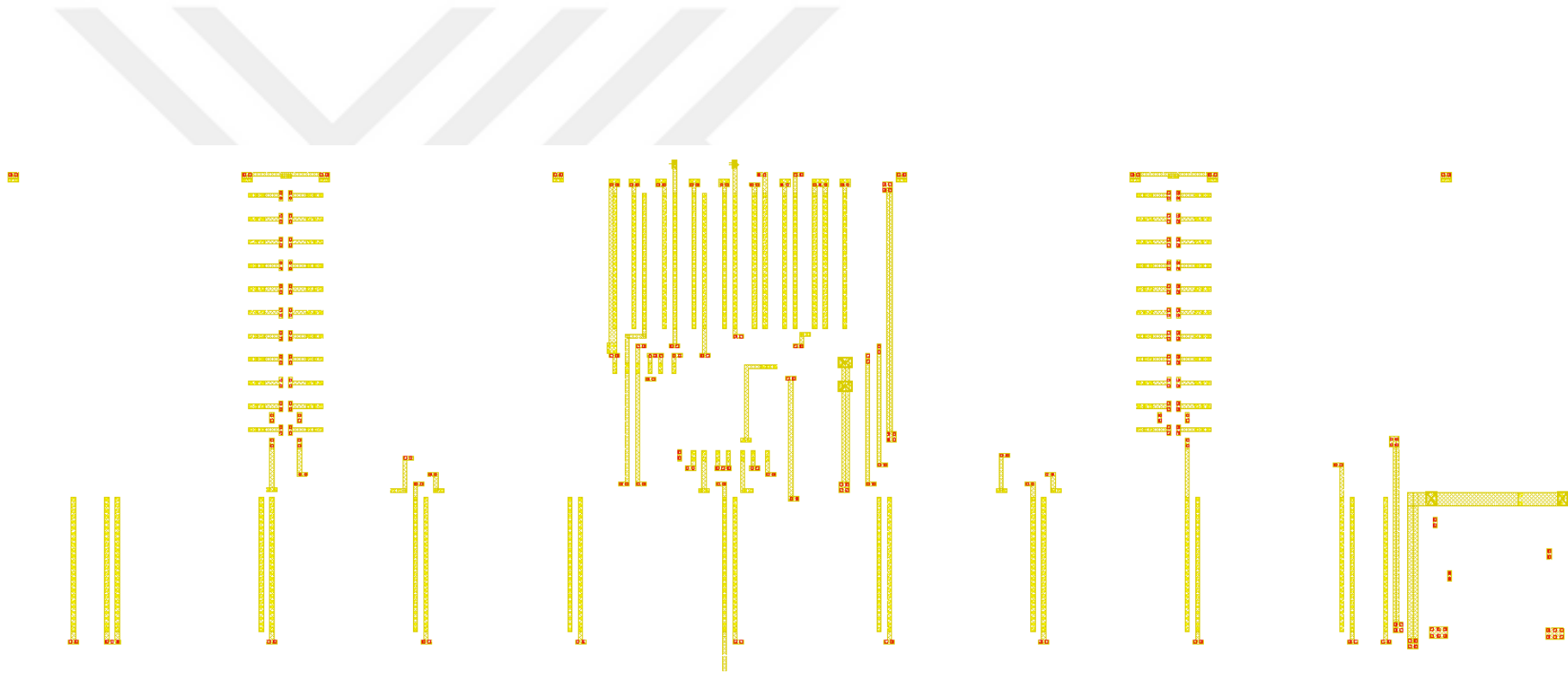
Figure A.2 : Adaptive Capacitive Gm block, metal 2 vertical routings.
