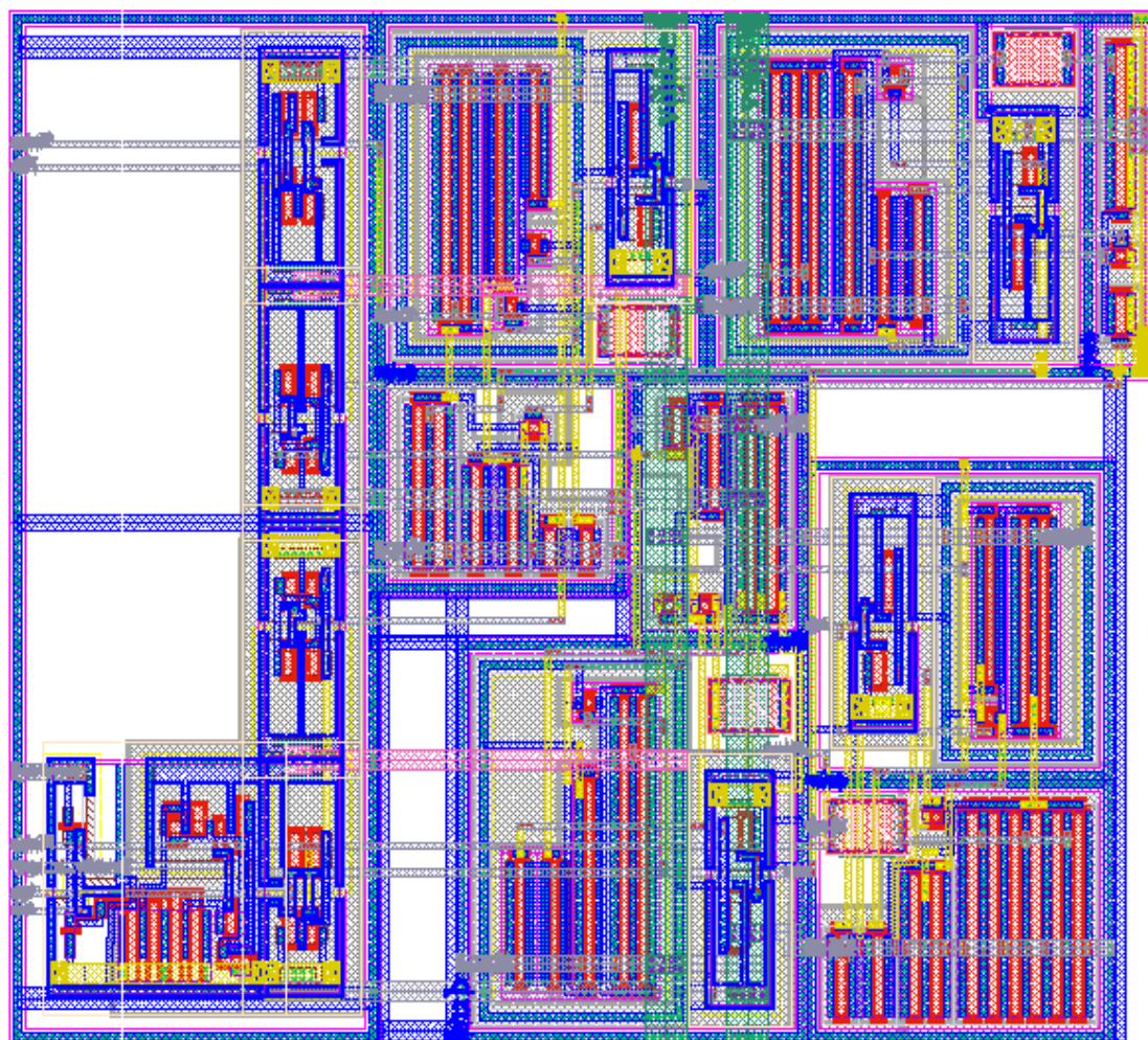
Figure 7.34 : Layout of buck unit drive block.
