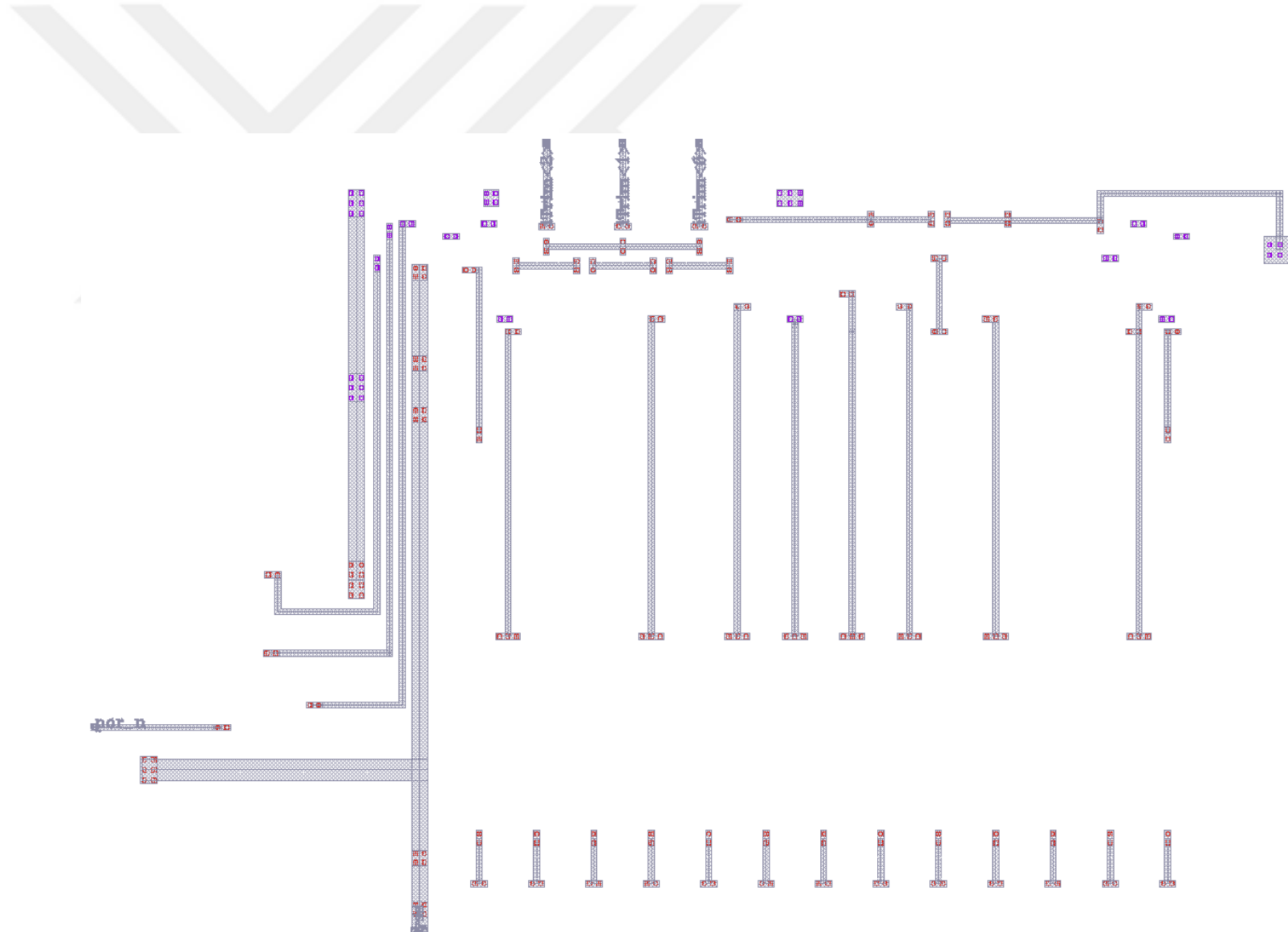
Figure A.15 : Ramp generator, metal 3 vertical routings.
