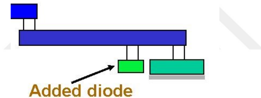
Figure 5.9 : Diode insertion to prevent Antenna effect.
