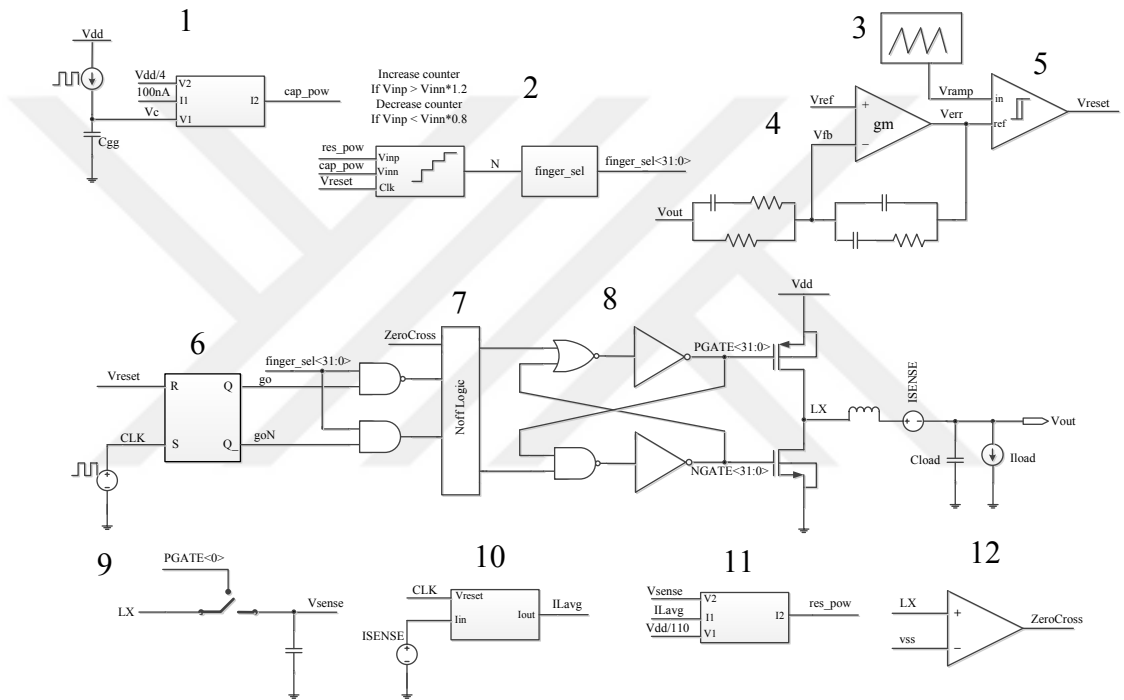
Figure 7.1 : Adaptive output buck converter system model [60].
