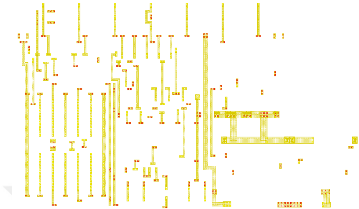
Figure A.12 : PWM comparator, metal 2 vertical routings.
