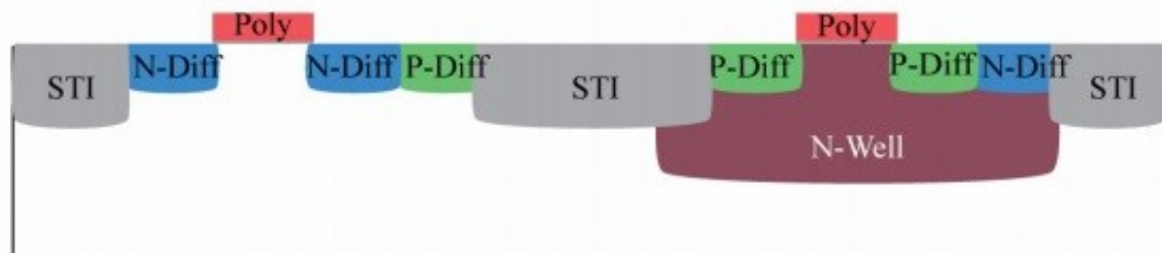
Figure 2.6 : Shallow trench isolation.
