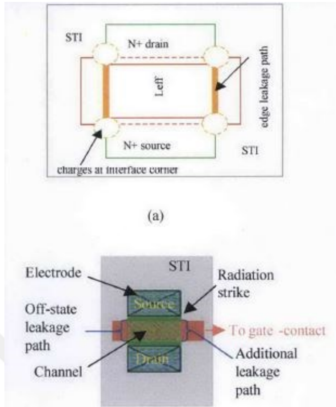
Figure C.1 : (a) Radiation effects mechanism and (b) illustration of off-state leakage path in the 2-edge standard MOSFET [77].
