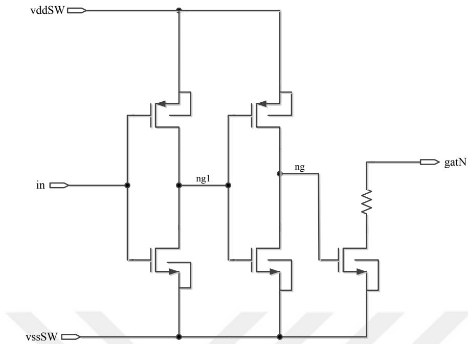
Figure 7.31 : Schematic design of N_{off} logic [60]
