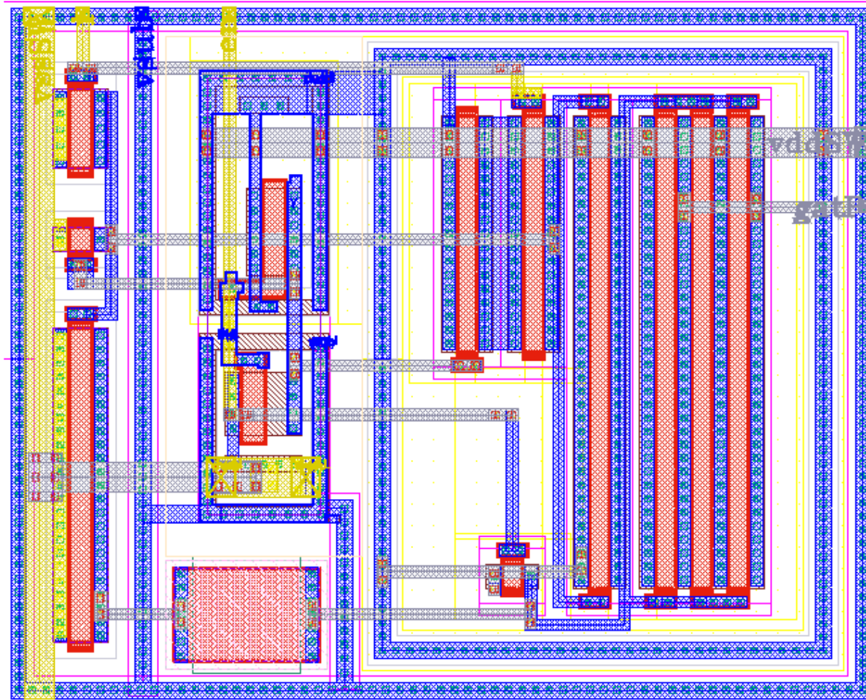
Figure 7.33 : Layout of P_{off} block.
