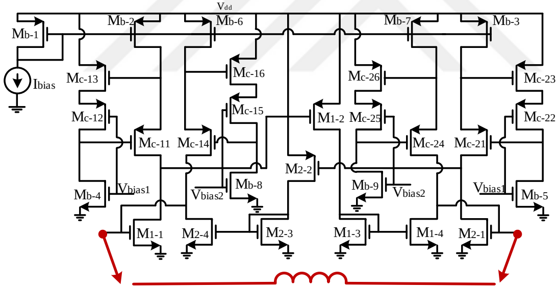
Figure 3.27 : Circuit implementation of the proposed FAI.
