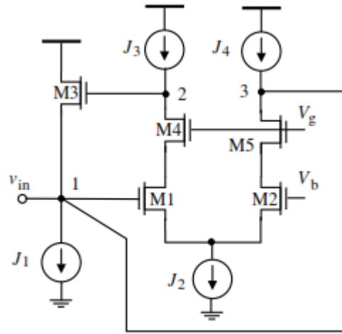
Figure 2.12 : Cascode double-feedback active inductor [40].
