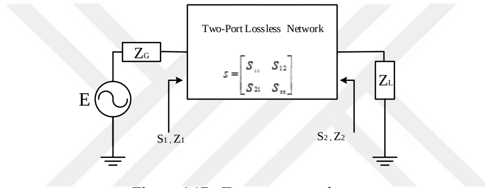
Figure 4.17 : Two port network.
