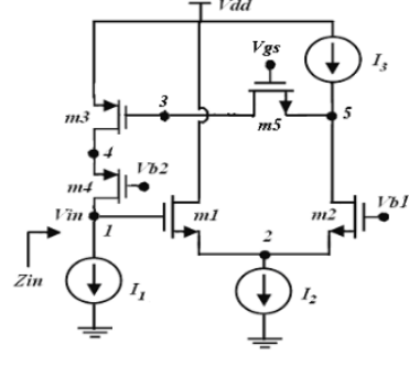
(b) AI with feedback transistor
