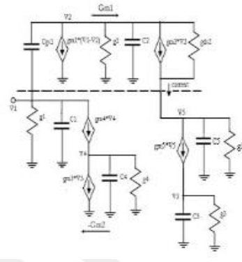
(d) Small signal equivalent circuit of the AI with feedback transistor
