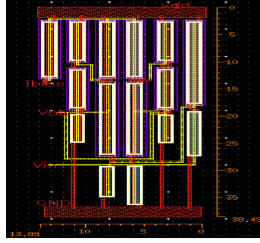
(a) Layout
