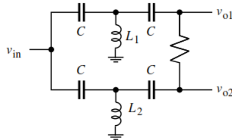
Figure 1.5 : Equivalent circuit of lumped Wilkinson power divider.
