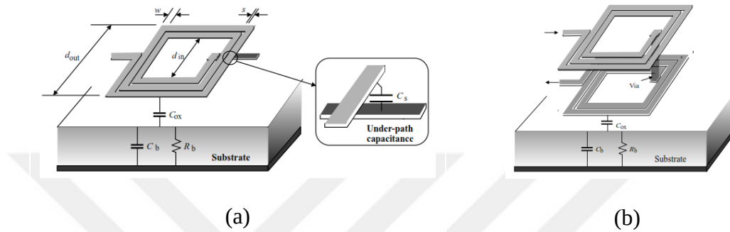
Figure 1.6 : Spiral Inductors (a) planar (b) stacked.
