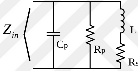
Figure 3.16 : Equivalent RLC model.
