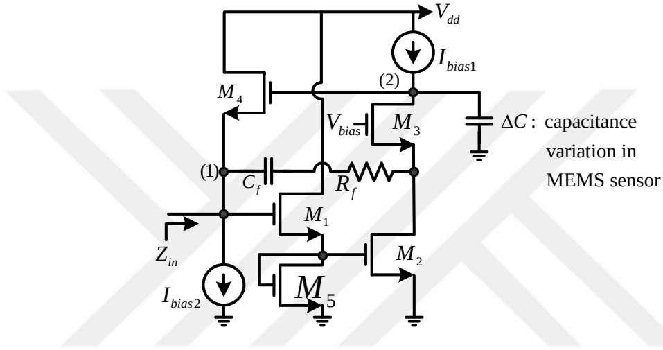
Figure 4.5 : Schematic of the proposed circuit.
