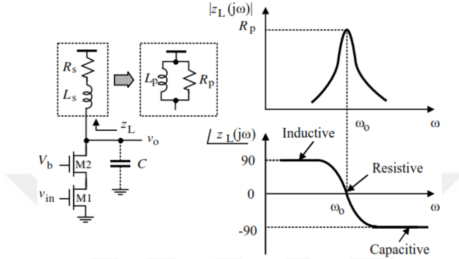
Figure 1.4 : Gain boosting of low noise amplifiers using LC tank load.
