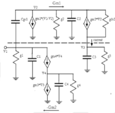
(c) Small signal equivalent circuit of the AI without feedback transistor
