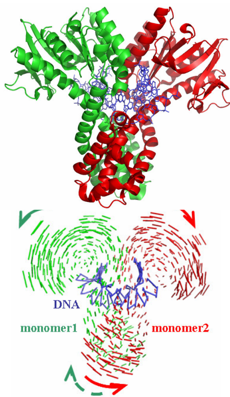
(a) BsoBI-DNA complex, third mode
