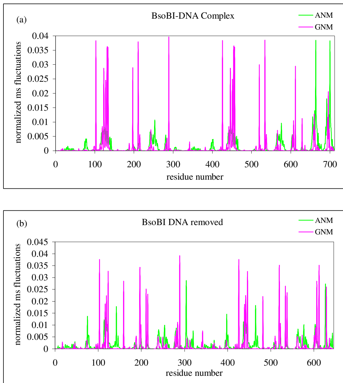
Figure 6.2. Mean-square fluctuations showing cumulative effect of 20 high-frequency modes from ANM ( r_{\text{cut}} : 13 Å) and GNM ( r_{\text{cut}} : 7 Å) for (a) BsoBI-DNA complex, and (b) BsoBI DNA removed form
