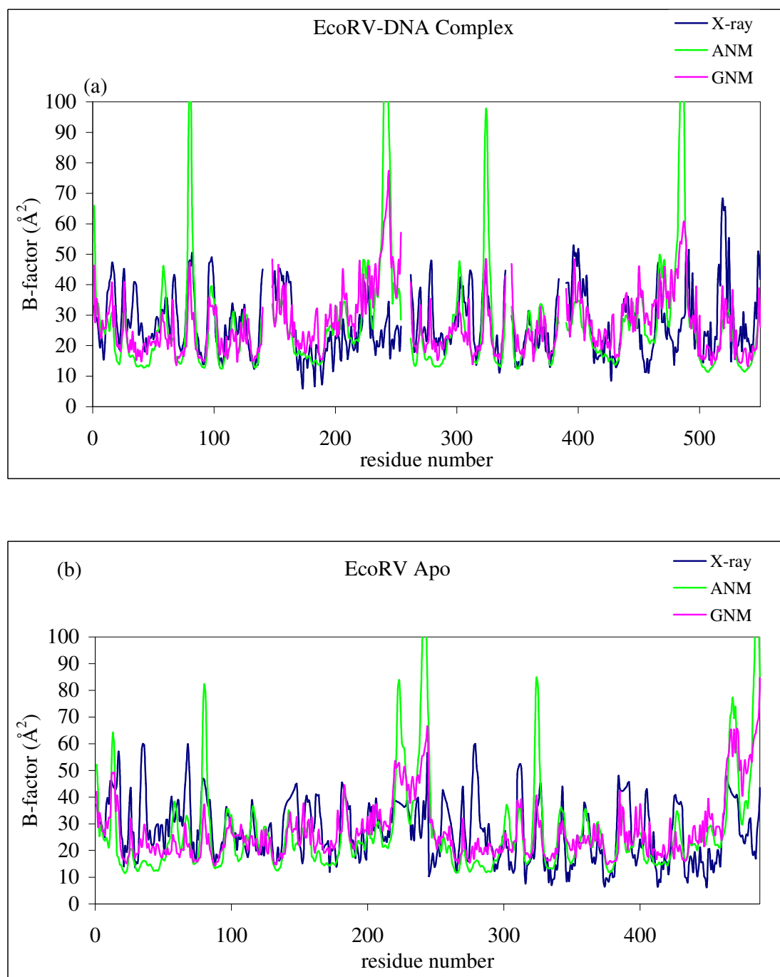
Figure 4.5. B-factors of EcoRV comparing X-ray, ANM and GNM results for (a) complex, and (b) apo forms
