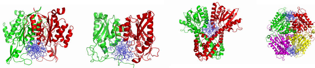
EcoRI-DNA complex
