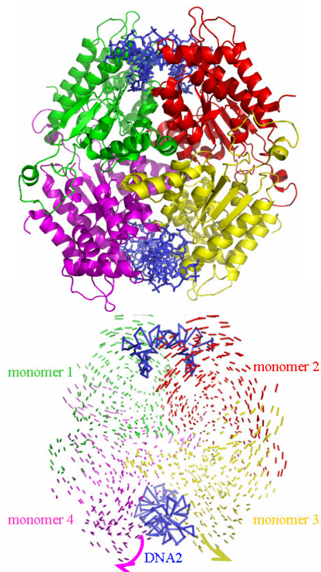
(b) NgoMIV-DNA complex, fourth mode
