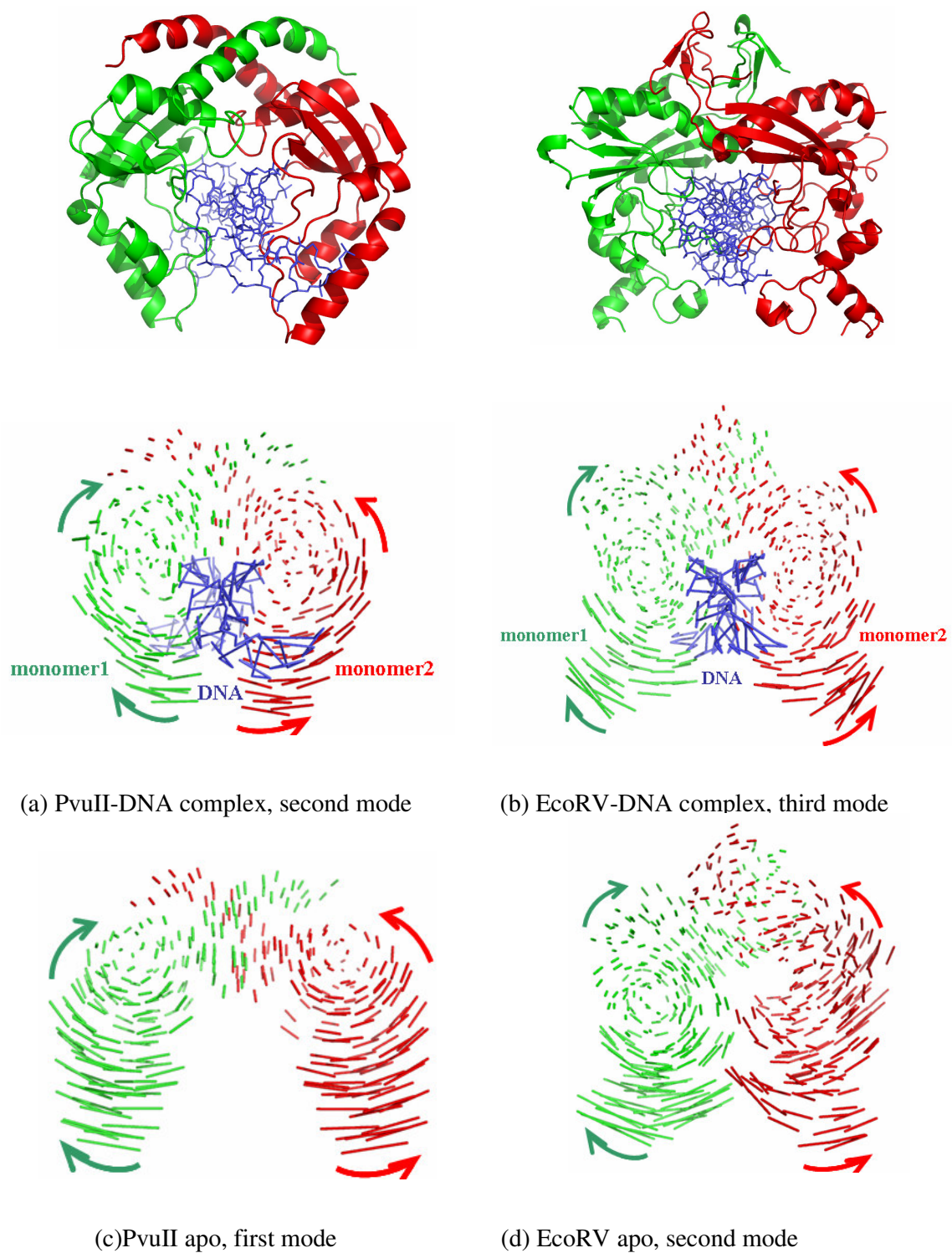
Figure 4.16. Displacement vectors showing twisting motion of PvuII and EcoRV
