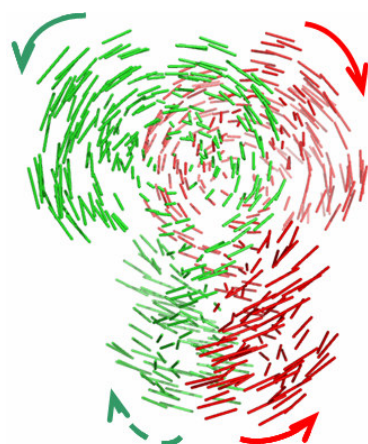
(c) BsoBI DNA removed, first mode
