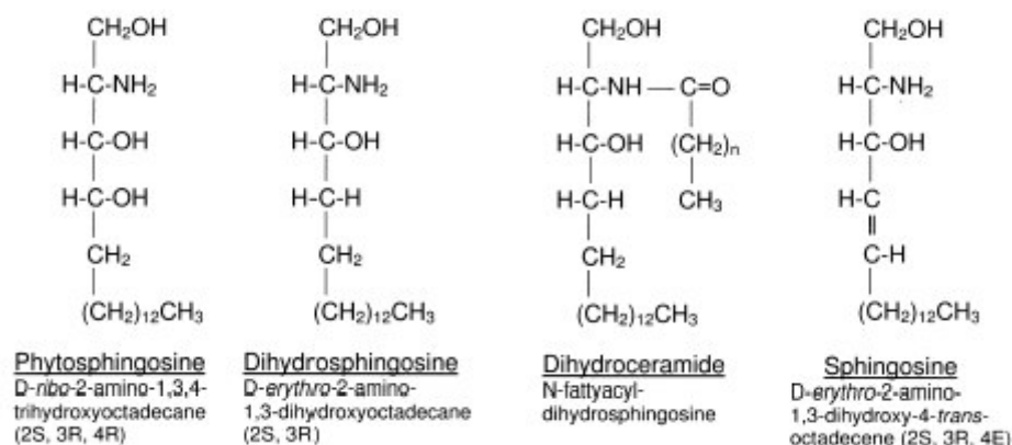
Figure 2.2. Some of the yeast sphingolipids (Dickson and Lester, 1999)
