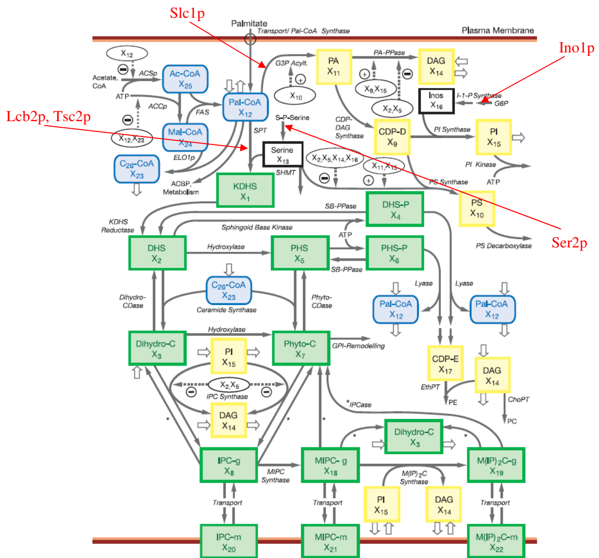
Figure 2.1. Sphingolipid pathway in yeast (Alvarez-Vasquez et al. , 2005)
