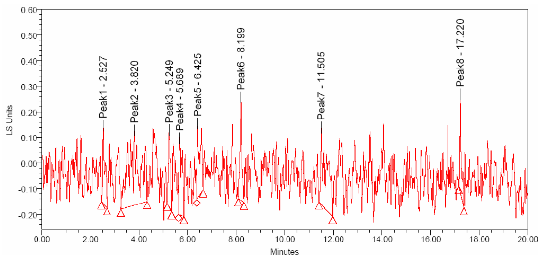
Figure 4.23. Chromatogram of SLC1/slc1Δ mutant grown in YPD
