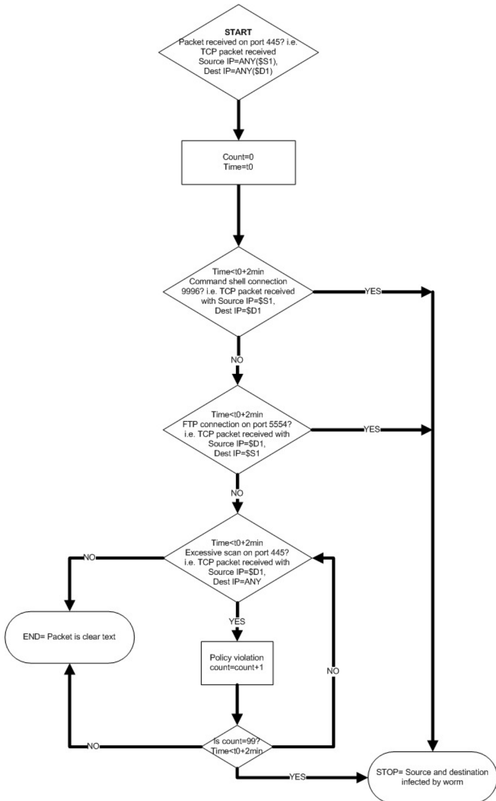
Figure 14 Sample Rule
