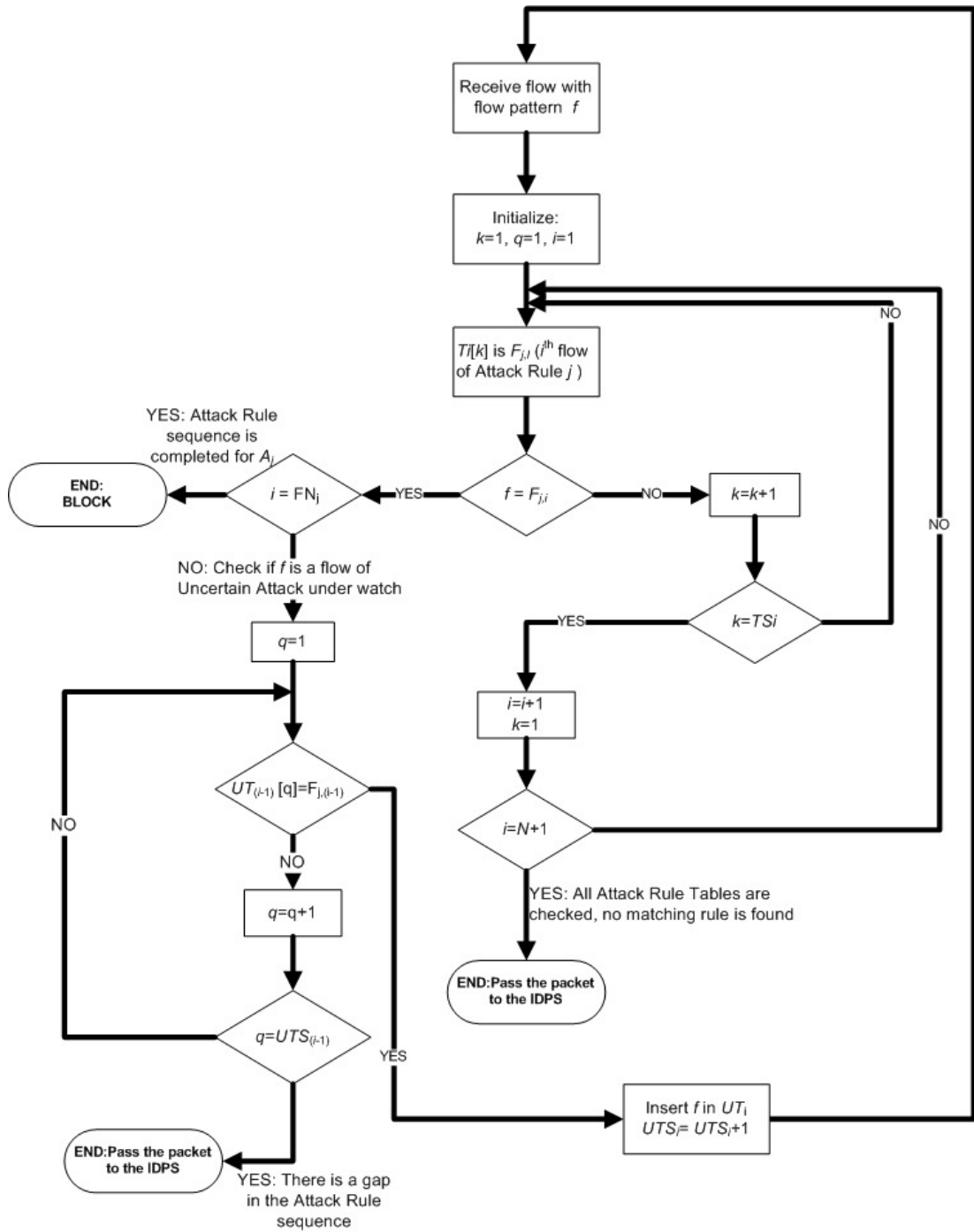
Figure 16 Engine's Flowchart
