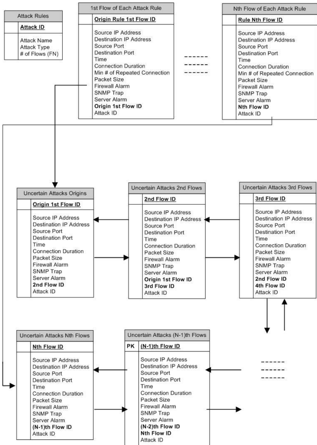
Figure 15 Database Model
