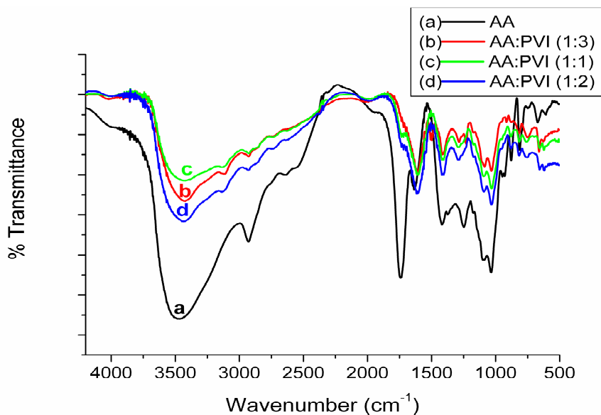
Figure 3.10 FT-IR results of AA and AA/ PVI networks at different x
