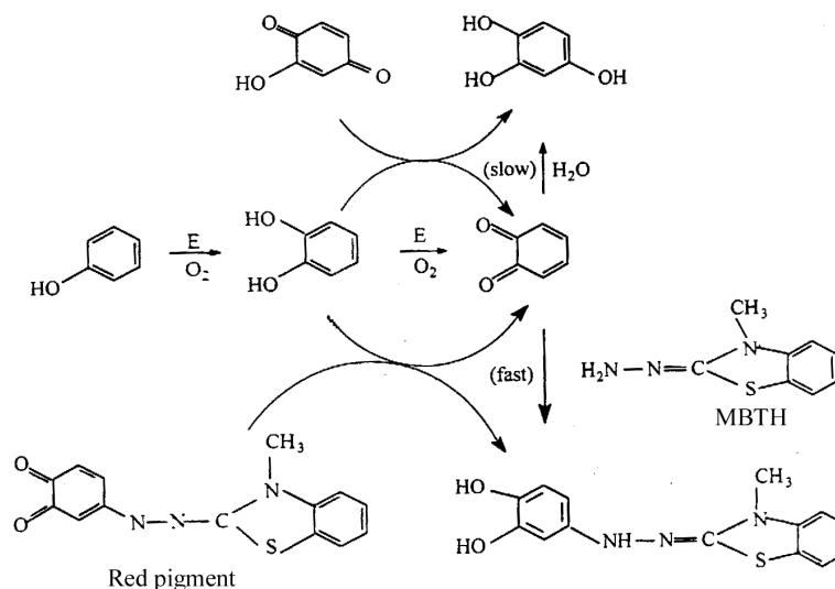
Figure 2.3 Schematic representation of Besthorn's Hydrazone Method
