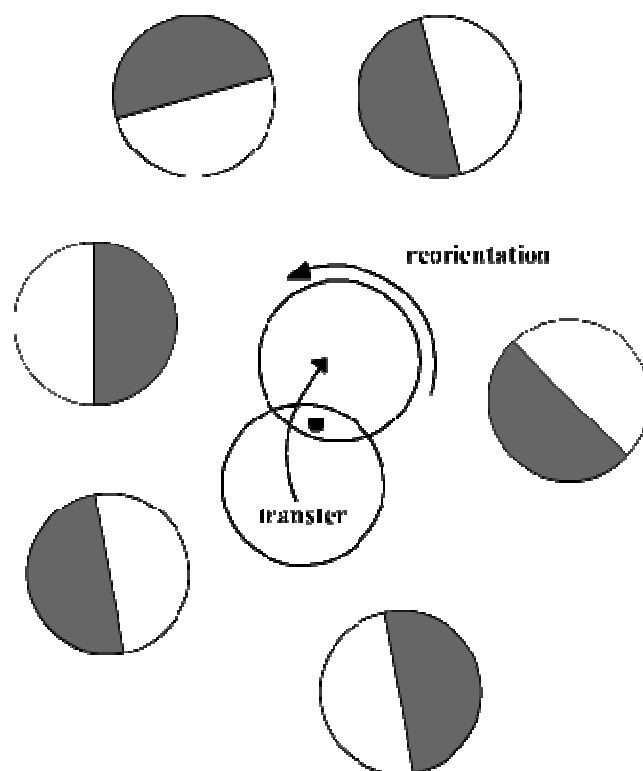
Figure 1.1 Schematic illustration of the two reaction steps involved in most long-range proton transport phenomena.
