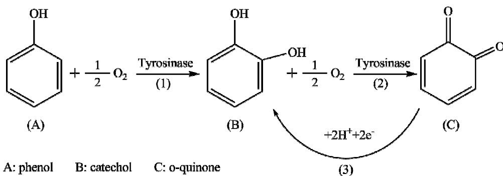
Figure 1. 24 Schematic representation of tyrosinase activity.
