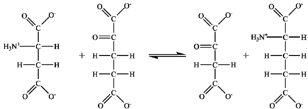
Figure 1.11 Schematic representation of aspartate aminotransferase activity
