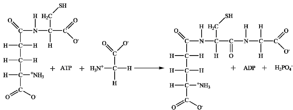
Figure 1.15 Schematic representation of glutathione synthase activity
