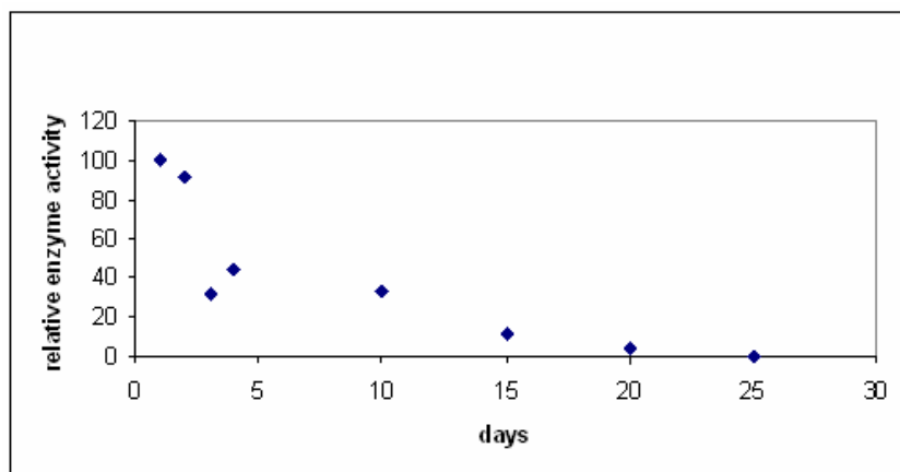
Figure 3.4 Shelf life of the biosensor
