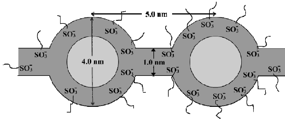
Figure 1.6 The cluster- network model
