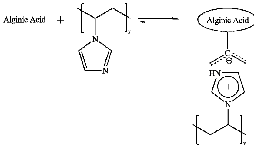
Figure 2.2 The structure of AA/PVI network
