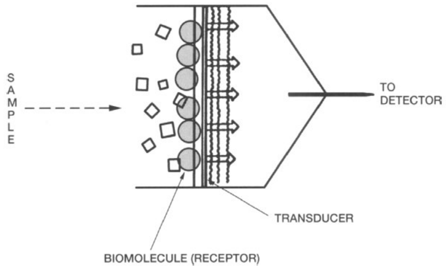
Figure 1.25 Biosensor Construction
