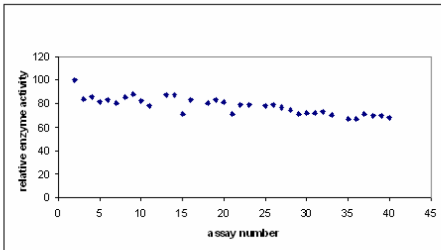
Figure 3.3 Operational stability of enzyme biosensor
