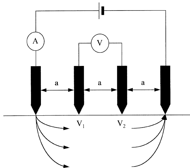
Figure 2.1 Four Probe Conductivity Measurement
