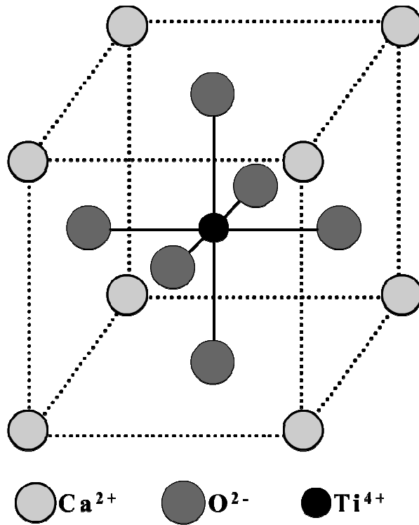
Figure 1.4 Schematic of a perovskite crystal
