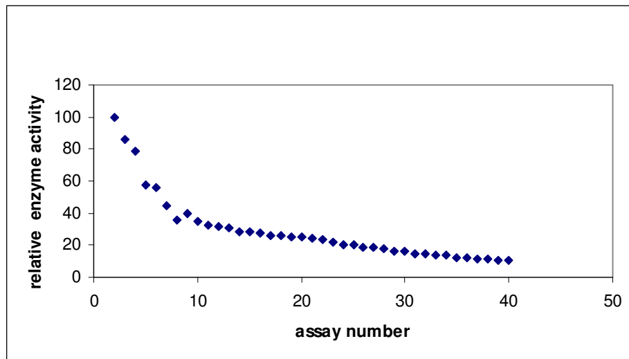
Figure 3.8 Operational Stability of Enzyme Biosensor (pH= 9)
