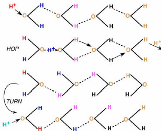
Figure 1.2 A highly schematic representation of a unidimensional chain of four water molecules interconnected via H-bonds (water or proton wire).
