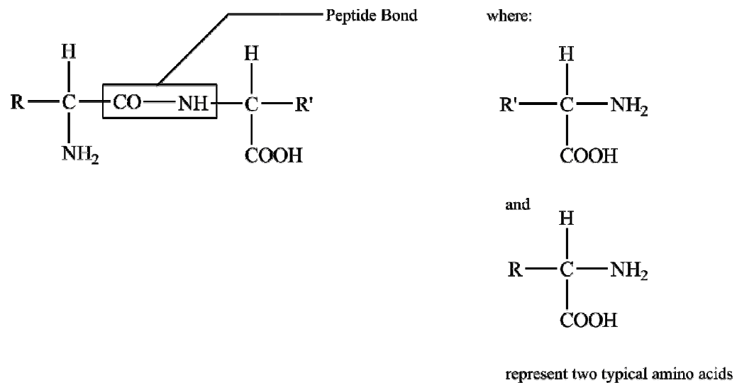
Figure 1.9 Typical Protein structure
