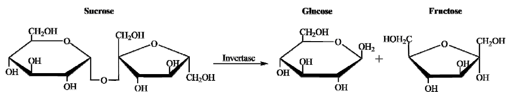
Figure 1.23 Hydrolysis of sucrose
