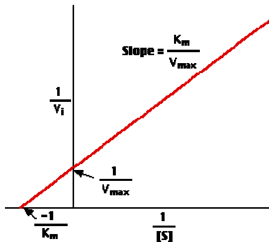
Figure 1.19 Lineweaver- Burk plot
