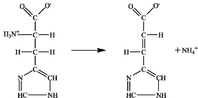
Figure 1.13 Schematic representation of histidine ammonia-lyase activity
