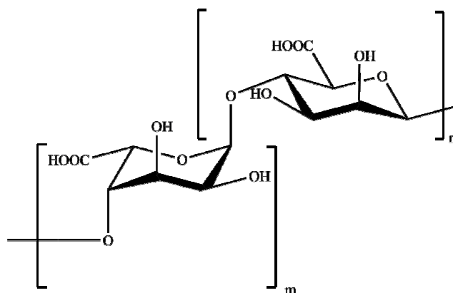
Figure 1.8 The structure of Alginic Acid
