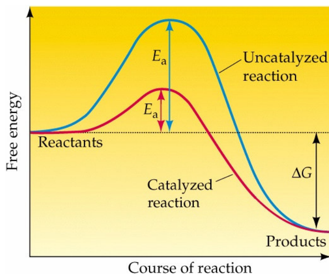
Figure 1.16 Activation energy diagram of enzyme catalyzed reaction
