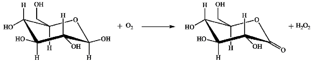
Figure 1.10 Schematic representation of glucose oxidase activity
