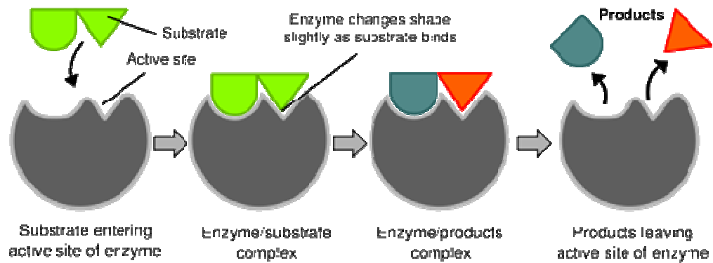
Figure 1.17 Lock and Key Model
