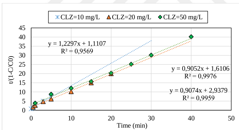
Figure A. 22. BMG kinetic analysis for CLZ degradation at different initial CLZ concentration
