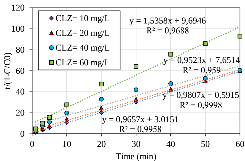
Figure A. 12. BMG kinetic analysis for CLZ degradation by Fenton at different initial CLZ concentration
