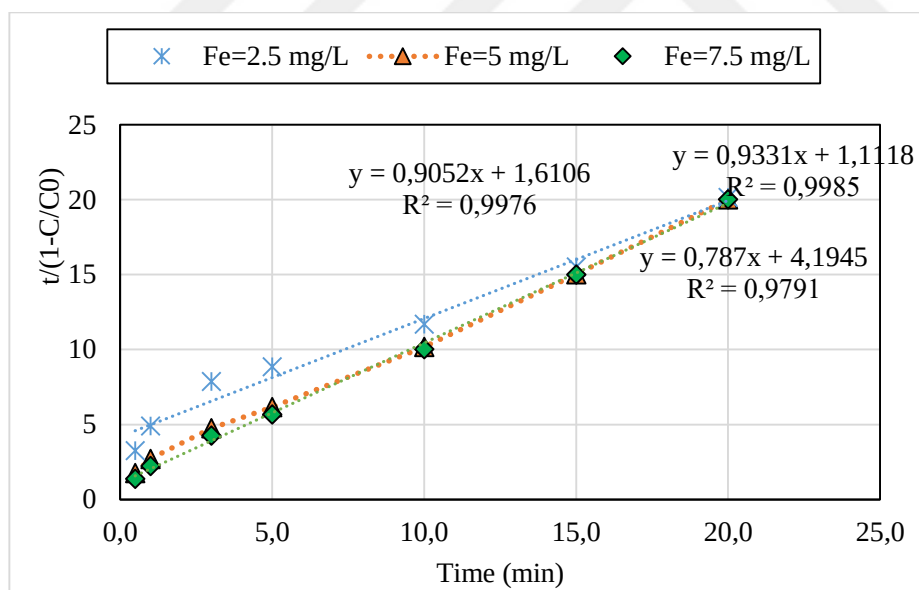
Figure A. 18. BMG kinetic analysis for CLZ degradation by Photo-Fenton at different \text{Fe}^{2+} concentration
