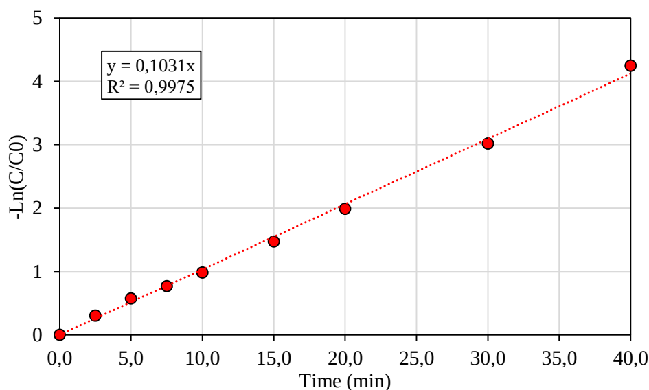
Figure 4.6. Pseudo first order kinetic analysis for CLZ degradation UV/H 2 O 2 processes (T=20°C, H 2 O 2 =20mg/L , pH=3 , CLZ=20mg/L)
