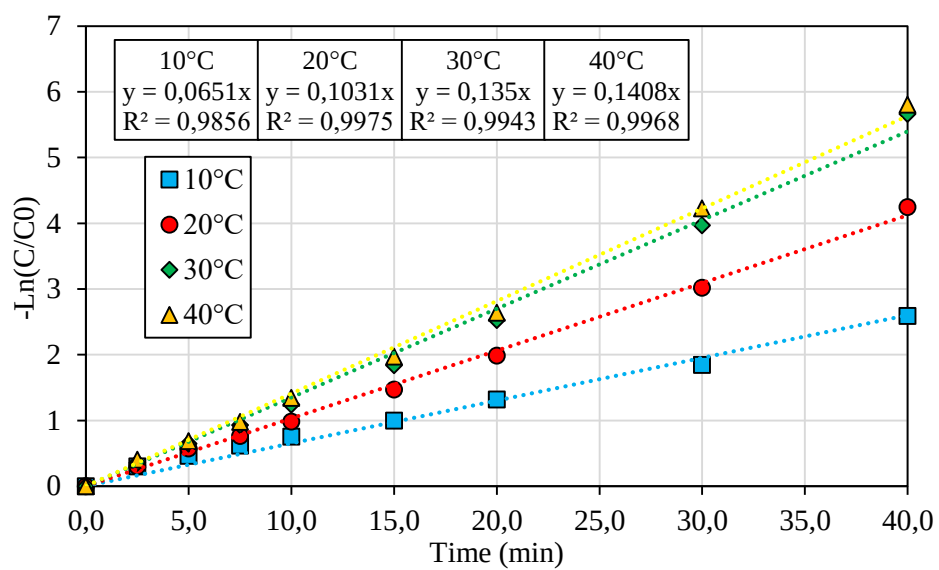
Figure A. 4. Pseudo First Order analysis for CLZ degradation by UV/H 2 O 2 at different Temperature
