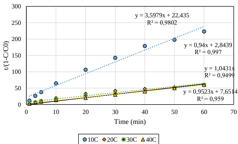
Figure A. 14. BMG kinetic analysis for CLZ degradation by Fenton at different Temperature
