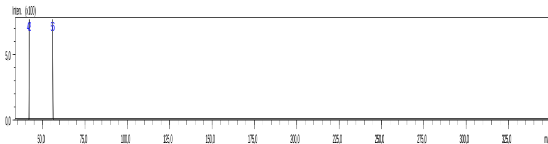
Figure 4.25. LC/MS/MS spectrum of CLZ (a) at the end of Fenton processes ( T=20^{\circ}\text{C} ; \text{CLZ}=40\text{ mg/L} ; \text{H}_2\text{O}_2=50\text{ mg/L} - \text{Fe}^{2+}=5\text{ mg/L} ; \text{pH}=3 ); (b) at the end of Photo-Fenton processes ( \text{CLZ}=60\text{ mg/L} - \text{H}_2\text{O}_2=50\text{ mg/L} - \text{Fe}^{2+}=5\text{ mg/L} - \text{pH}=3 ); (c) Fragment ions of Pyradazine-3,4,5-trione ( m/z 42 and 56).
