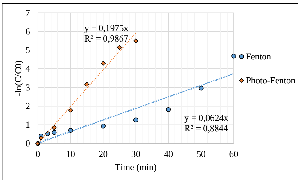
Figure 4.17. Pseudo first order kinetic analysis of CLZ degradation by Fenton and Photo-Fenton processes (pH=3, \text{Fe}^{2+} = 5 mg/L, \text{H}_2\text{O}_2 = 50 mg/L, CLZ=40 mg/L, T=20^\circ\text{C} for Fenton and pH=3, \text{Fe}^{2+} = 5 mg/L, \text{H}_2\text{O}_2 = 50 mg/L, CLZ=60 mg/L, T=20^\circ\text{C} for Photo-Fenton)
