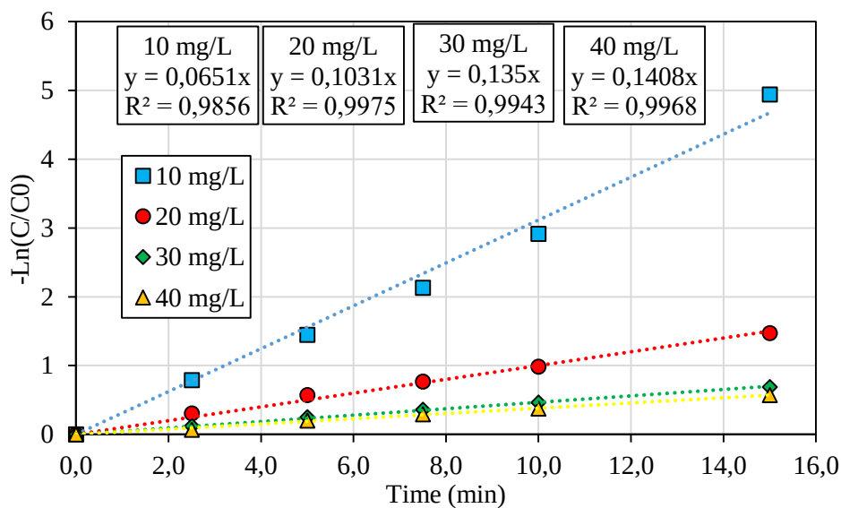
Figure A. 3. Pseudo First Order analysis for CLZ degradation by UV/H 2 O 2 at different initial CLZ concentration
