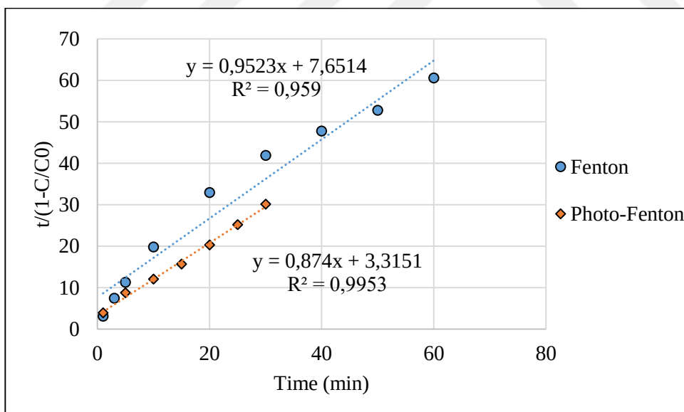
Figure 4.18. BMG kinetic analysis for CLZ degradation by Fenton and Photo-Fenton processes (pH=3, \text{Fe}^{2+} =5 mg/L, \text{H}_2\text{O}_2 =50 mg/L, CLZ=40 mg/L, T=20^\circ\text{C} for Fenton and pH=3, \text{Fe}^{2+} =5 mg/L, \text{H}_2\text{O}_2 =50 mg/L, CLZ=60 mg/L, T=20^\circ\text{C} for Photo-Fenton)
