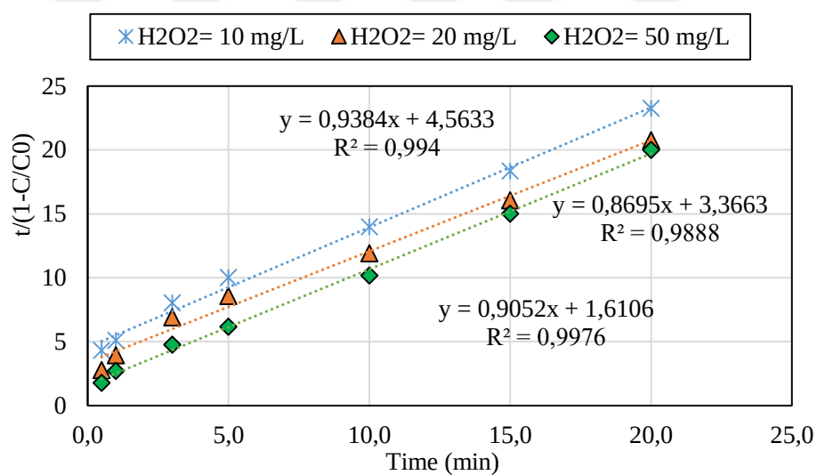
Figure A. 20. BMG kinetic analysis for CLZ degradation by Photo-Fenton at different \text{H}_2\text{O}_2 concentration
