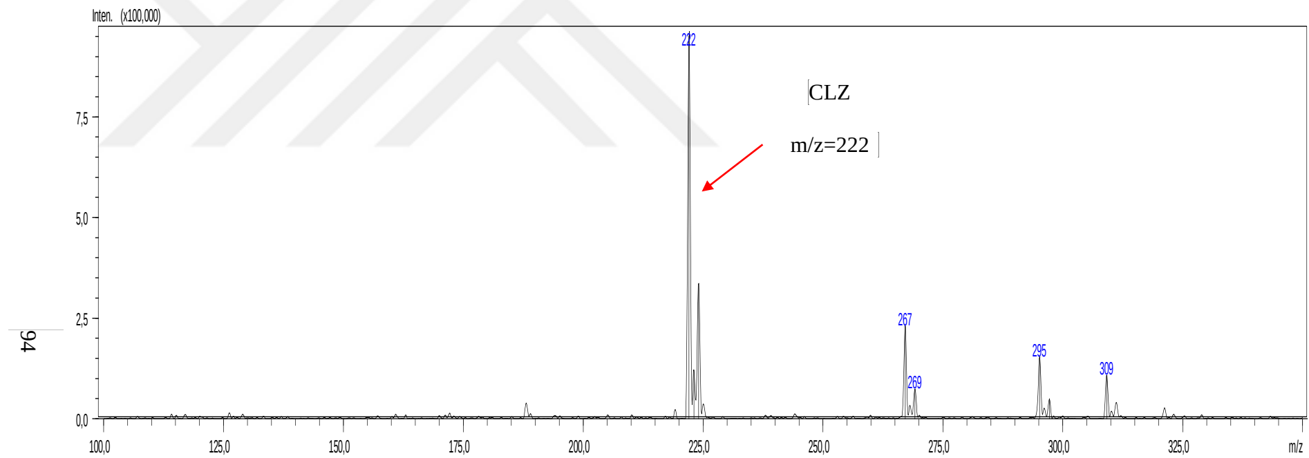
Figure 4.22. LC/MS/MS spectrum of 1 mg/L CLZ (intensity vs m/z)
