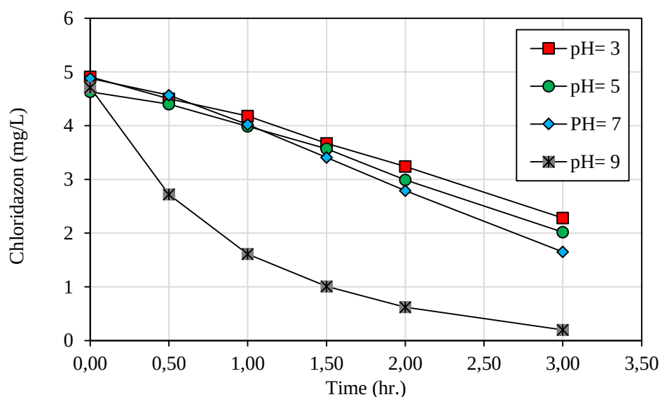
Figure 4.1. CLZ removal at different pH with the presence of UV light
