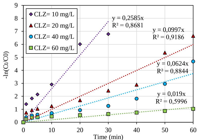
Figure A. 11. Pseudo First Order kinetic analysis for CLZ degradation by Fenton at different initial CLZ concentration
