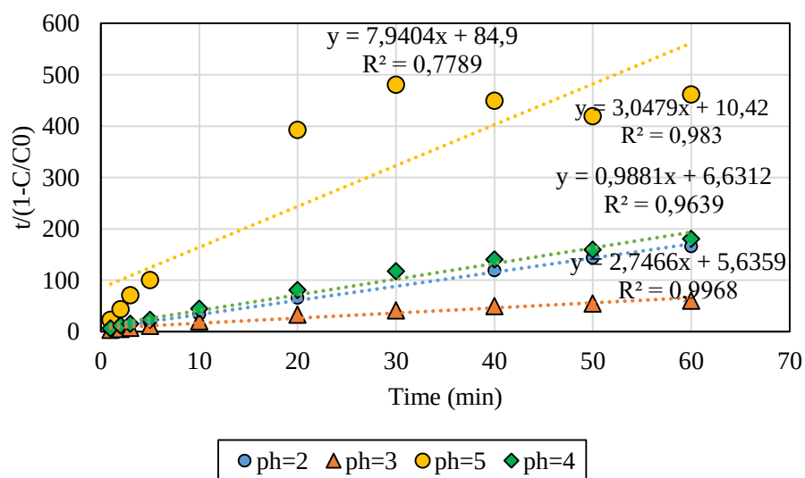
Figure A. 6. BMG kinetic analysis for CLZ degradation by Fenton at different pH
