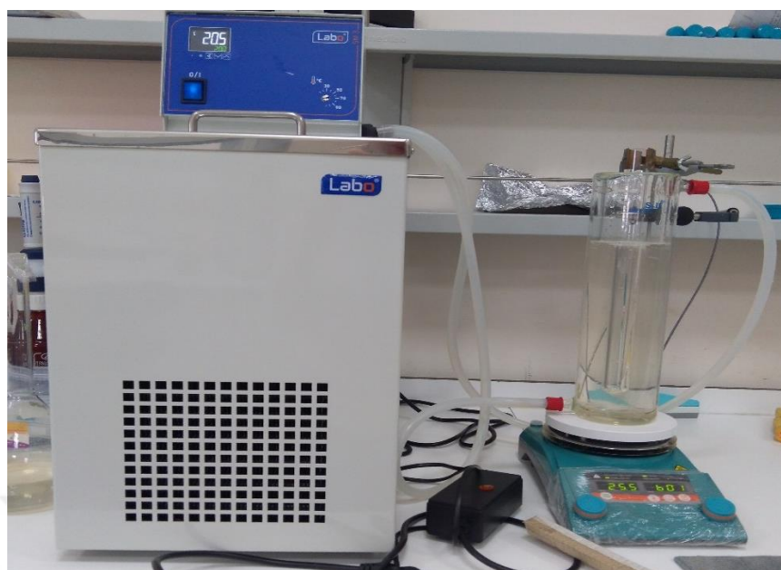
Figure 3.1. Experimental Set-up used for Fenton Oxidation
