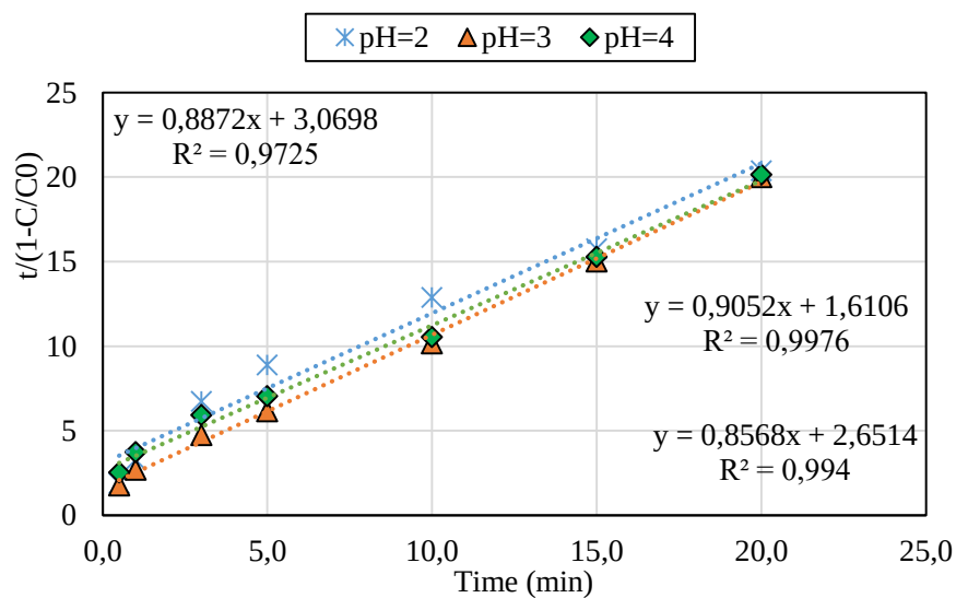
Figure A. 16. BMG kinetic analysis for CLZ degradation by Photo-Fenton at different pH
