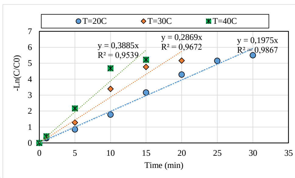
Figure A. 23. Pseudo First Order kinetic analysis for CLZ degradation by Photo-Fenton processes at different Temperature
