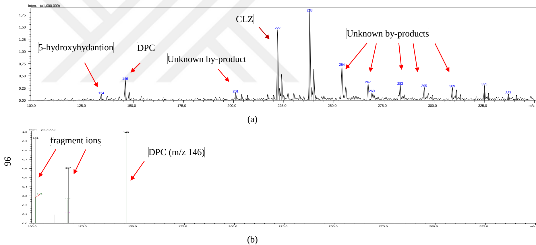
Figure 4.23. (a) LC/MS/MS spectrum of CLZ at the end of UV/H 2 O 2 application (T=20°C; H 2 O 2 =20 mg/L; pH=3; initial CHL=20 mg/L); (b) Fragment ions of DPC (m/z 101 and m/z 117).
