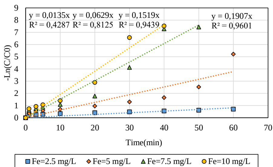
Figure A. 7. Pseudo First Order kinetic analysis for CLZ degradation by Fenton at different \text{Fe}^{2+} concentration
