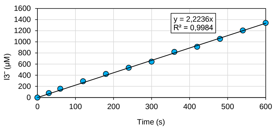
Figure 3.5. Formation of I_3^- in time with KI/ KIO_3 Actinometer
