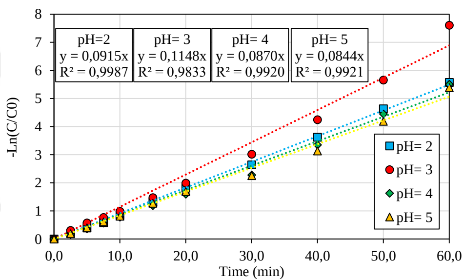
Figure A. 1 .Pseudo First Order analysis for CLZ degradation by UV/H 2 O 2 at different pH
