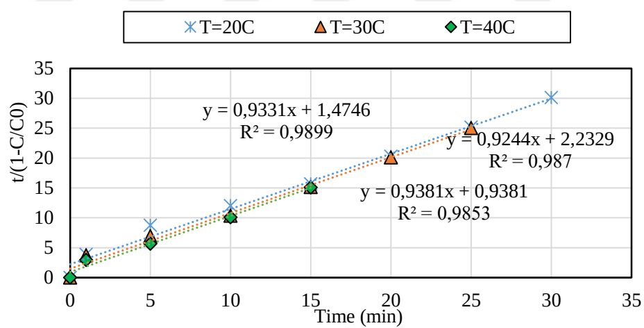
Figure A. 24. BMG kinetic analysis for CLZ degradation by Photo-Fenton at different Temperature
