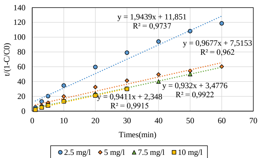
Figure A. 8. BMG kinetic analysis for CLZ degradation by Fenton at different \text{Fe}^{2+} concentration
