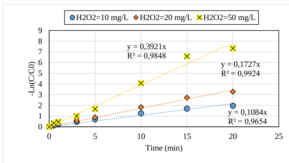
Figure A. 19. Pseudo First Order kinetic analysis for CLZ degradation by Photo-Fenton processes at different \text{H}_2\text{O}_2 concentration
