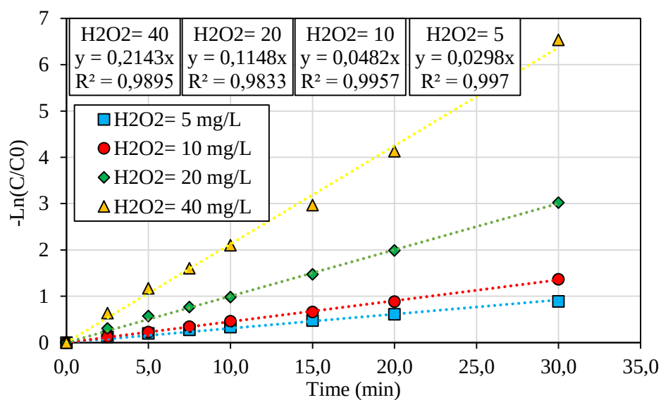
Figure A. 2 .Pseudo First Order analysis for CLZ degradation by UV/H 2 O 2 at different H 2 O 2 concentration
