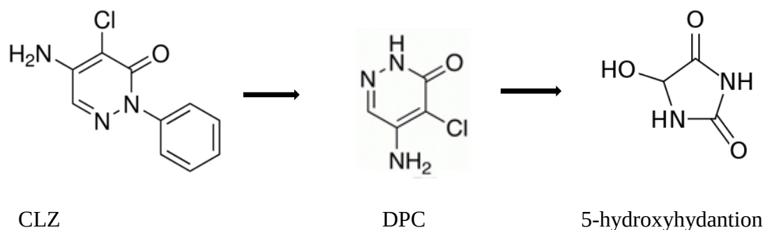
Figure 4.24. Proposed degradation pathway for the formation of 5-hydroxyhydantion (Schatz, 2012)
