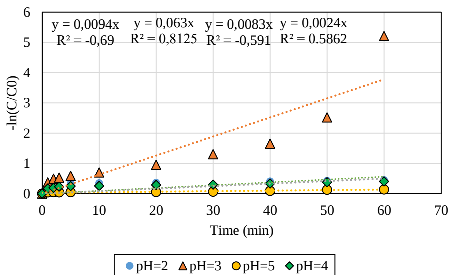
Figure A. 5. Pseudo First Order analysis for CLZ degradation by Fenton at different pH
