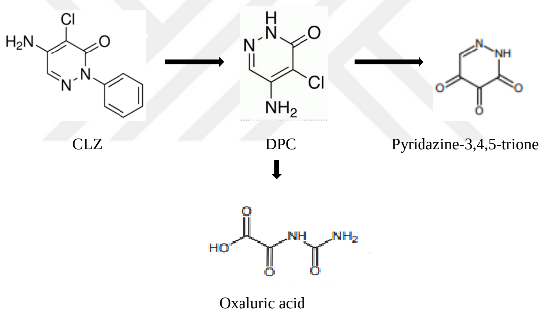
Figure 4.26. Possible degradation pathway for the formation of Pyridazine-3,4,5-trione and Oxaluric acid (Schatz, 2012).
