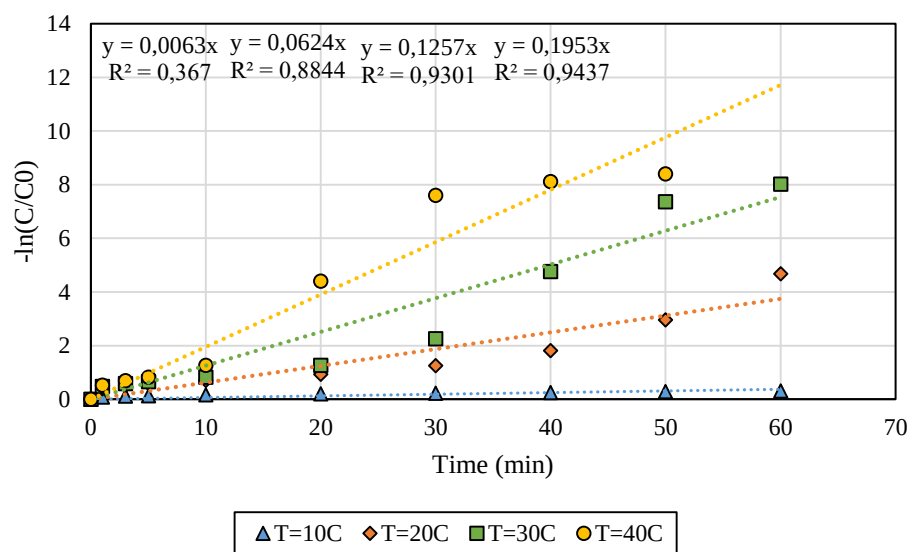
Figure A. 13. Pseudo First Order kinetic analysis for CLZ degradation by Fenton at different Temperature
