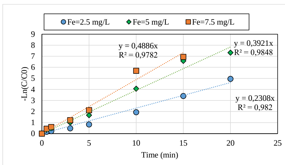
Figure A. 17. Pseudo First Order kinetic analysis for CLZ degradation by Photo-Fenton processes at different \text{Fe}^{2+} concentration
