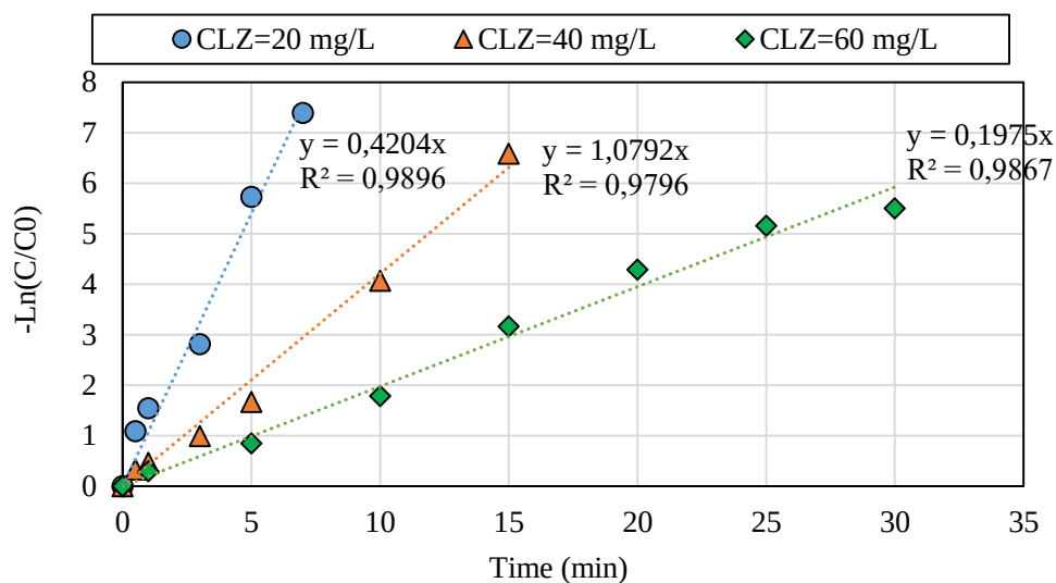
Figure A. 21. Pseudo First Order kinetic analysis for CLZ degradation by Photo-Fenton processes at different initial CLZ concentration
