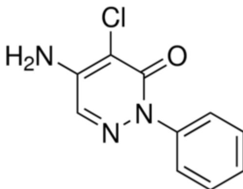
Figure 2.1. Chemical structure of CLZ (URL 2)
