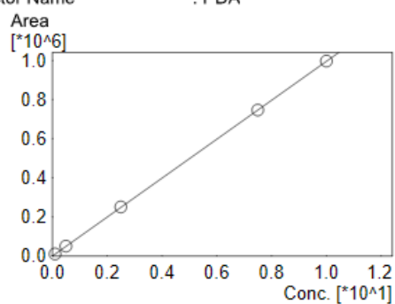
Figure B. 1. Calibration curve in HPLC
