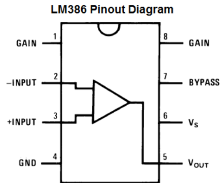
Figure 2.10: LM386 pin diagram [51].
