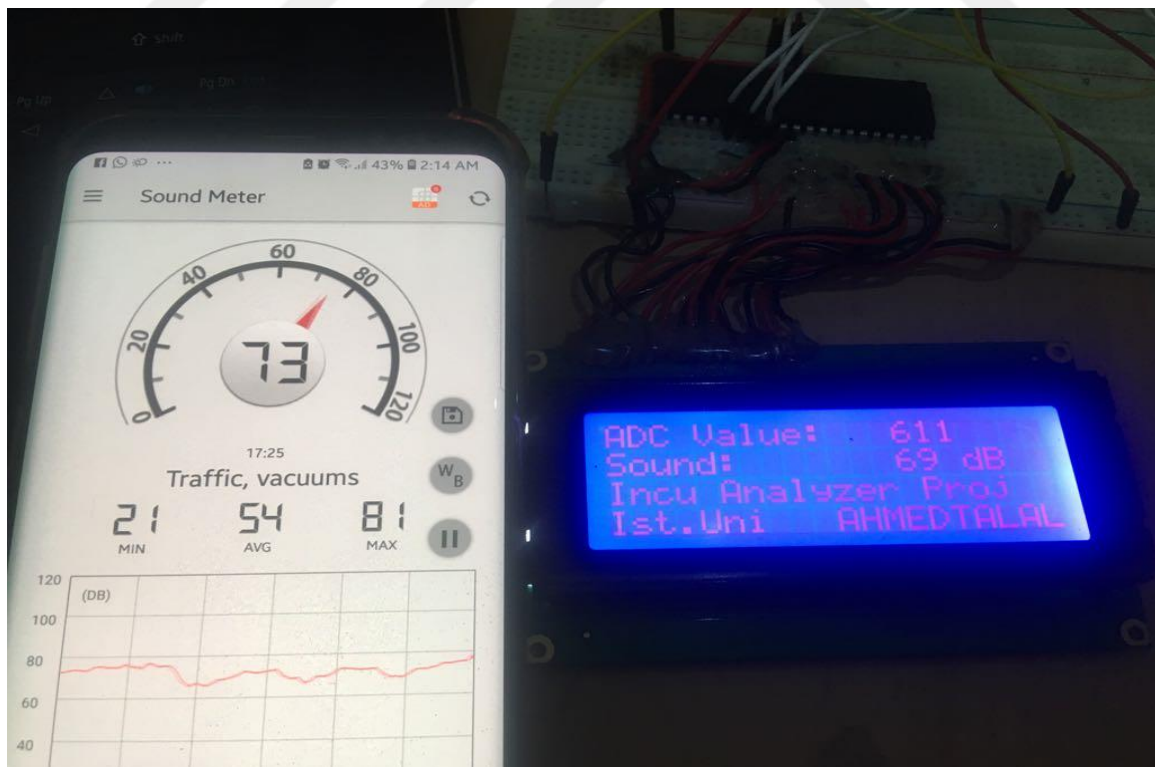
Figure 3.7: Sound sensor obtained result with music turned on.
