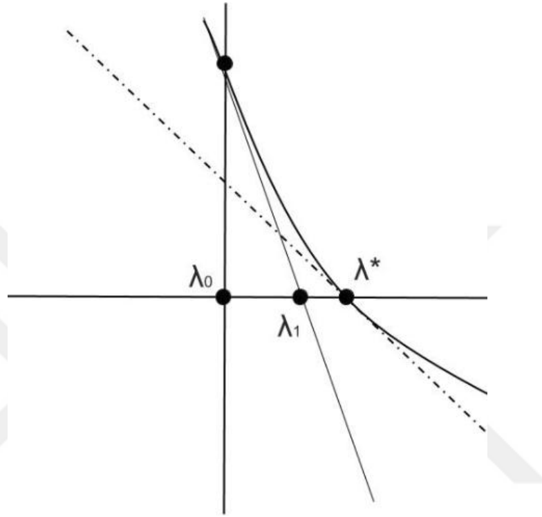
Figure 7.1: Newton Iteration Step
