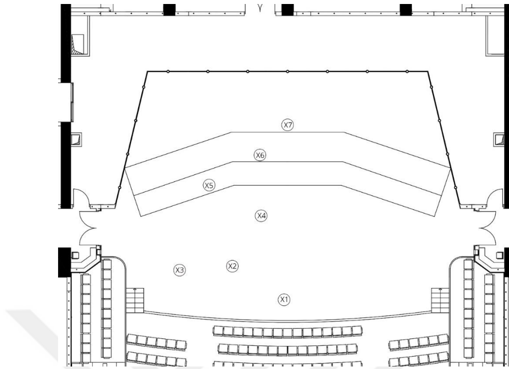
Figure 9. Measurement positions
