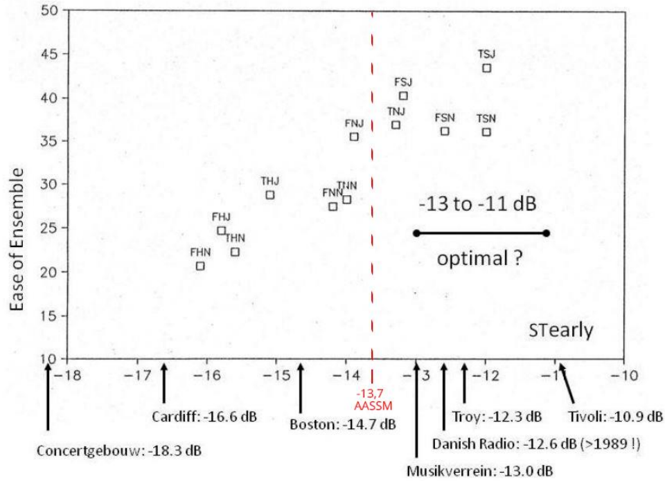
Figure 14. Comparison of this hall with Gade's ST_{early} results
