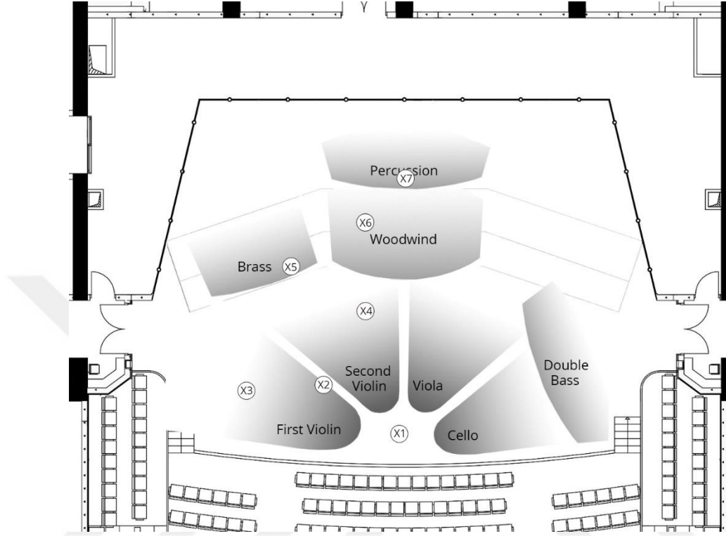
Figure 11. Measurement Positions and Instrument Groups
