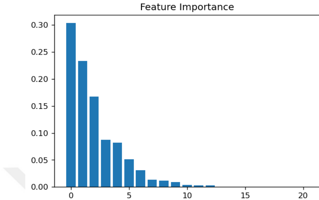
Figure 4.9. Feature importance visualization plot using RandomForestClassifier.
