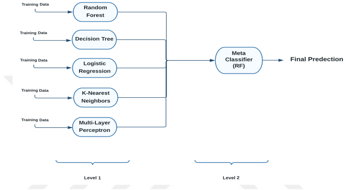
Figure 4.12. Stacking concept diagram.
