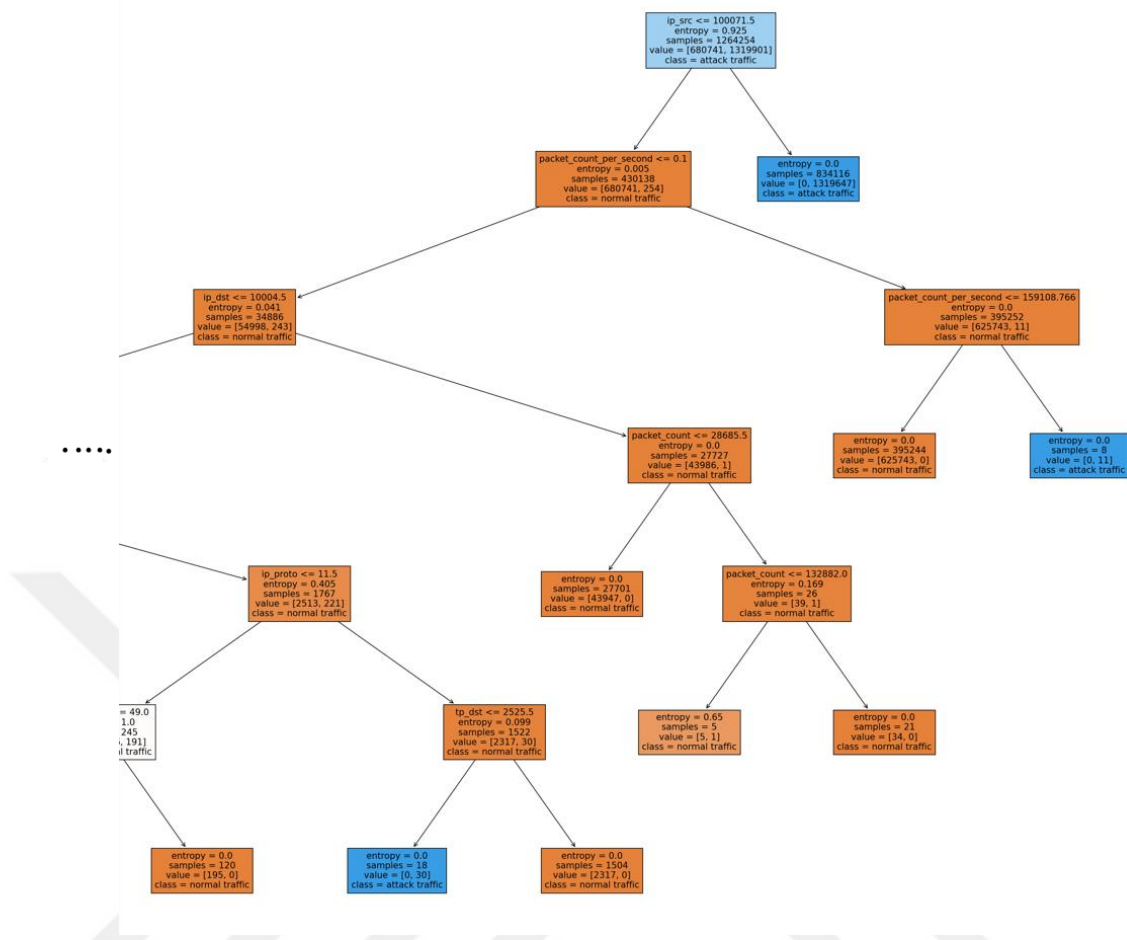
Figure 4.10. An example random forest tree for a network intrusion detection task.
