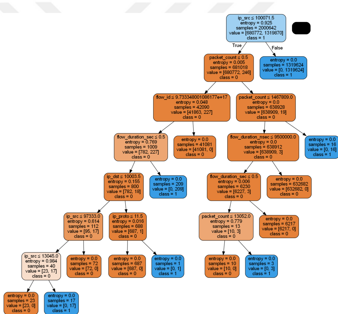
Figure 4.11. Decision tree for a network intrusion detection task
