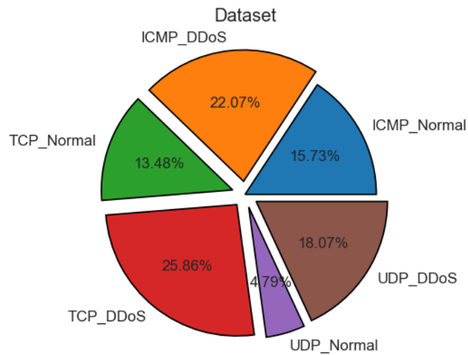
Figure 4.7. Volume of network traffic by type in a six-category dataset.
