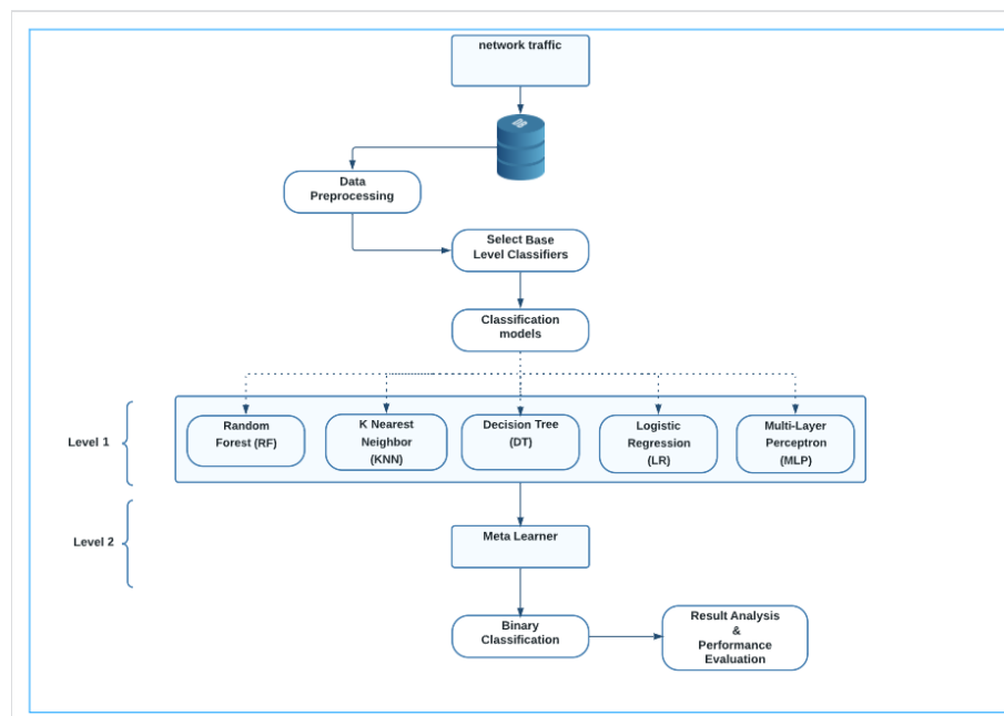
Figure 4.2. Workflow of the model.
