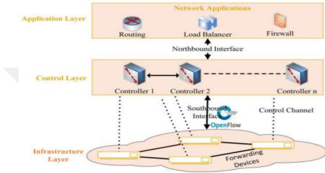
Figure 2.3. SDN structure (Wazirali et al., 2021).
