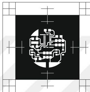
Figure 2.1. Photoresist mask. Each trace has 300 \mu m width. Pads for power supply and I2C (SDA,SCL,INT) have 1.5mm by 1.5mm dimensions
