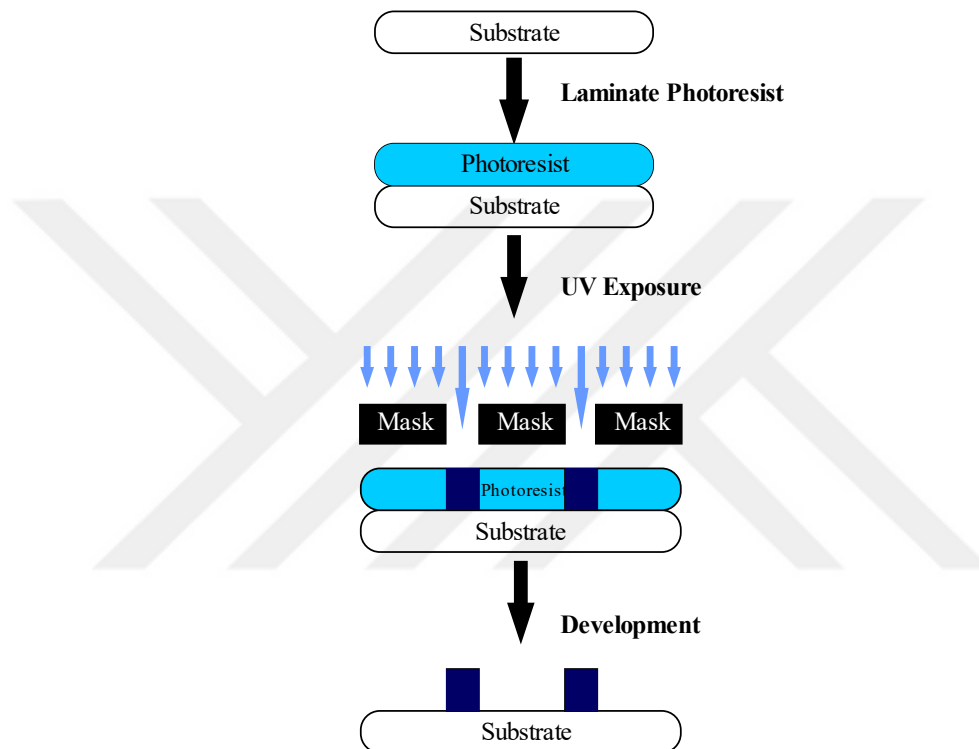
Figure 2.3. Process of Negative Dry Film Photoresist( NDFP) Method.
