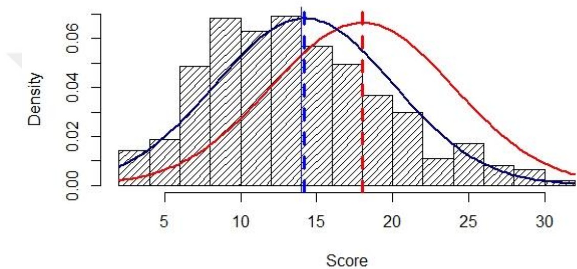
Figure 12. Normal curve of population and sample based on all students' total score
