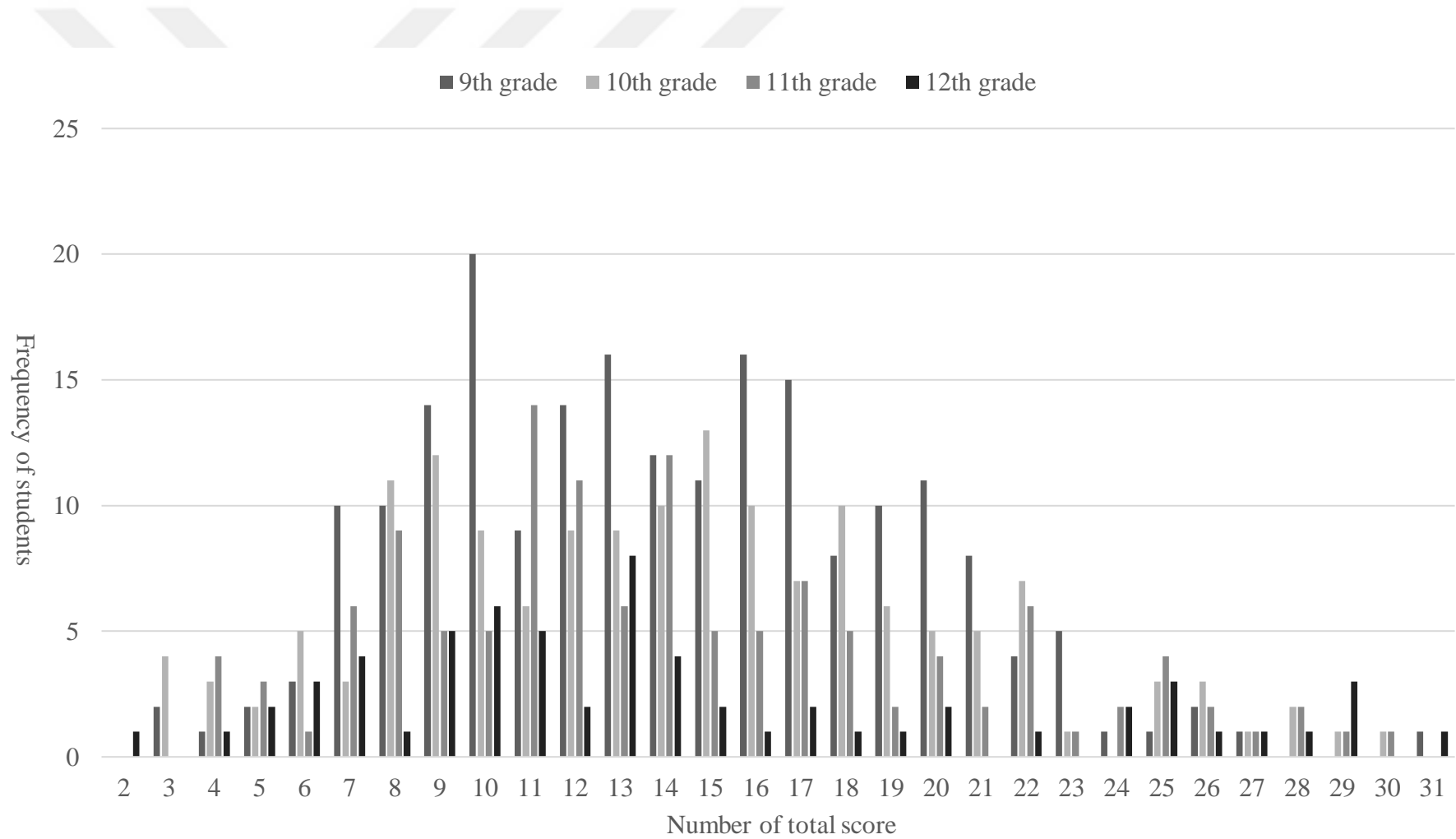
Figure 18. The distribution of students' total scores by grade
