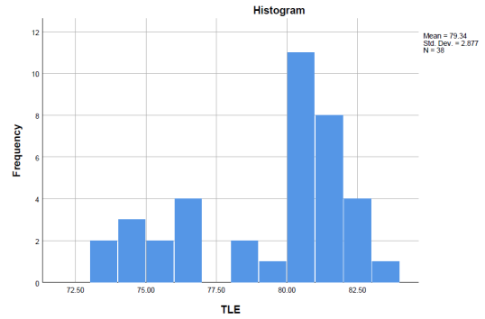
Figure A.16: Histogram-TLE(RECwSH)
