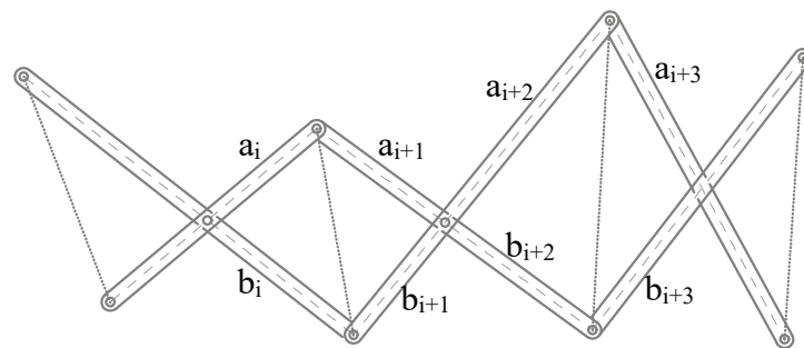
Figure 3.4. Deployability of scissor linkage (Reproduced from: Maden, Korkmaz, and Akgün 2011)
