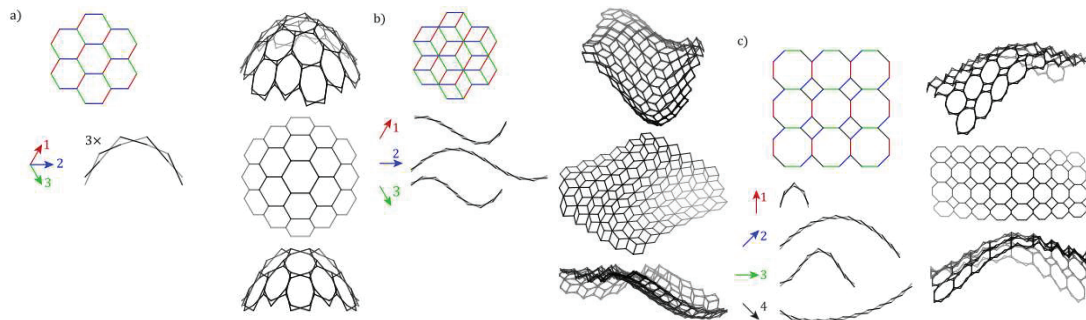
Figure 2.32. Various double-layer grids of translational units generated by tiling the scissor units of multiple planar linkages along a pattern: a) hexagonal tiling; b) rhombille tiling; c) truncated square tiling. (Source: Roovers and Temmerman 2017a)
