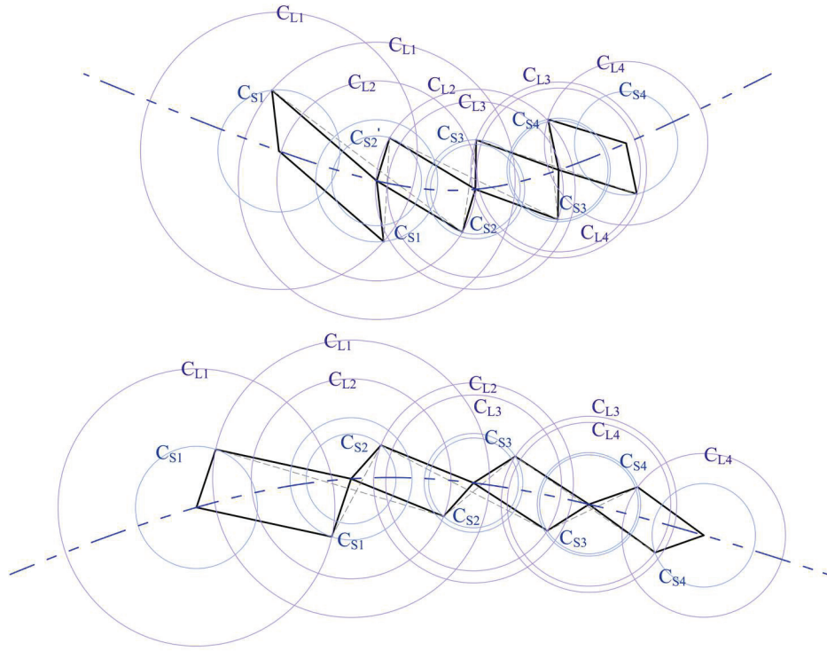
Figure 6.6. Concave and convex forms of planar scissor linkage that are formed with parallelogram loops.
