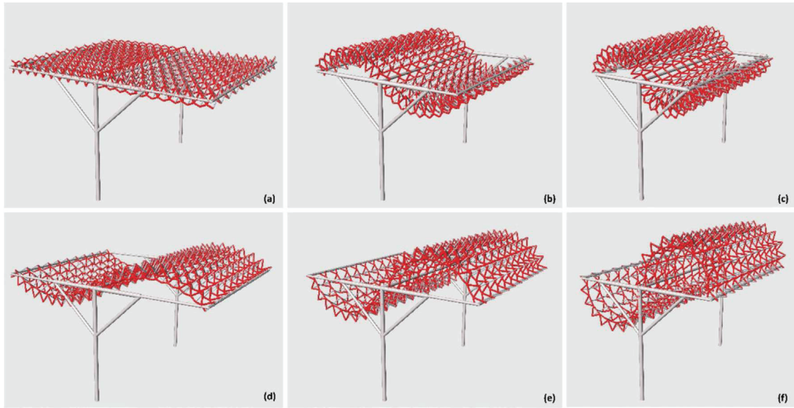
Figure 2.21. The transformation process of dynamic shelter structure. (Source: Maden, Ölmez, et al. 2019)
