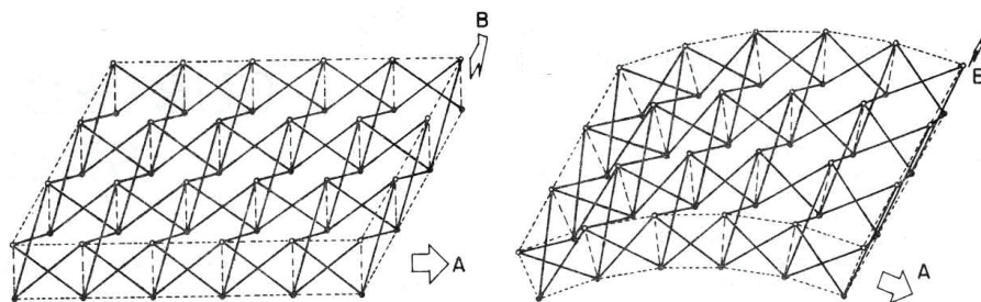
Figure 2.14. Sequence two-way cylindrical grid with translational unit (Escrig and Valcárcel 1987)
