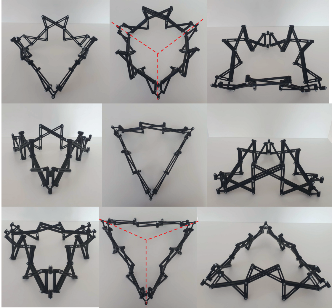
Figure 6.17 3D-printed model of the module with its motion sequence top to bottom concave, flat, and convex.
