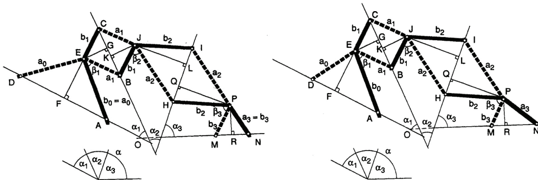
Figure 3.8. Assembly of Type I GAEs left and assembly of Type II GAEs right. (Source: You and Pellegrino 1997)
