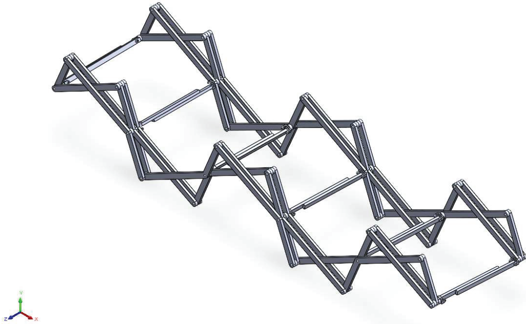
Figure 6.12 A model composed of planar linkages connecting with telescopic middle bars.
