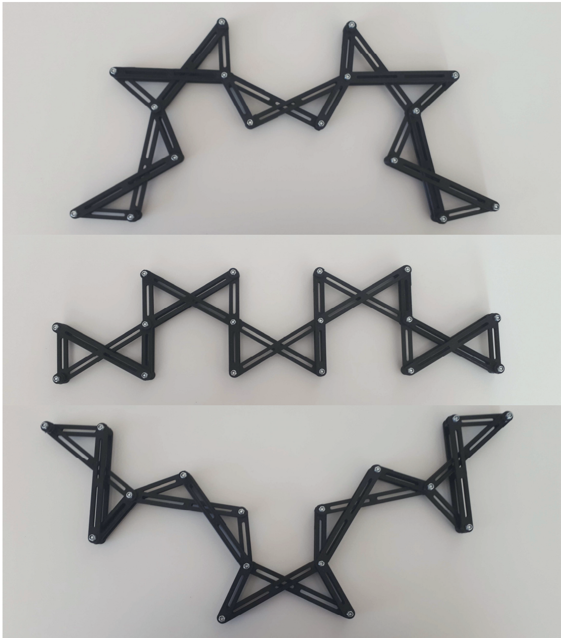
Figure 6.14. 3D Printed model of a scissor linkage with its motion sequence.
