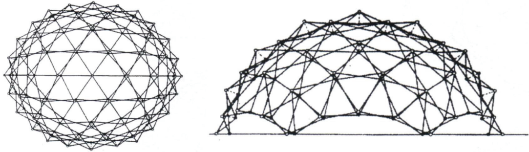
Figure 2.23. Top view and side elevation of a three-way spherical grid with polar units (Source: Escrig and Valcárcel 1987)
