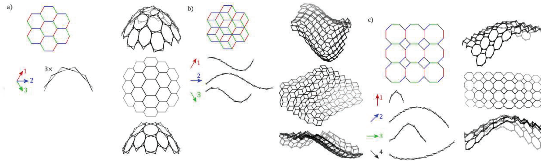
Figure 2.41 Various double-layer grids of translational units generated by tiling the scissor units of multiple planar linkages along a pattern: a) hexagonal tiling; b) rhombille tiling; c) truncated square tiling. (Source: Roovers and Temmerman 2017a)
