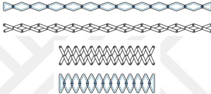
Figure 2.1. Rhombus loop assembly in a direction and resulting scissor linkage (Source: Hoberman, Demaine, and Rus 2013)
