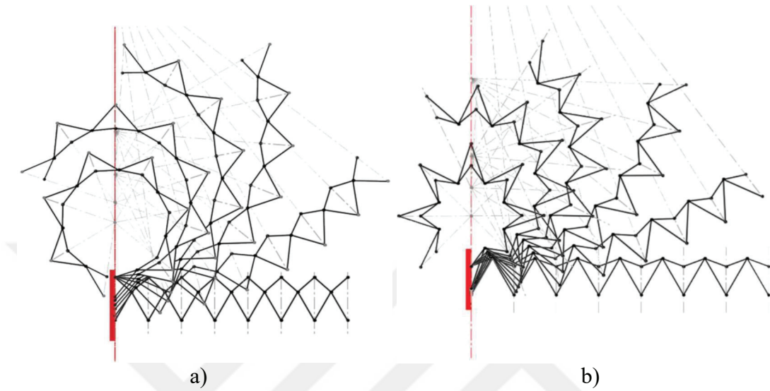
Figure 2.7. Transformable scissor linkages obtained with a) kite and b) dart loops (Source: Yar et al. 2017)
