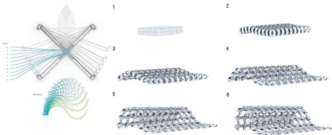
Figure 2.18. Scissor unit with various hinge points and the structure constructed with. (Source: Rippmann 2007)
