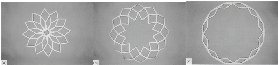
Figure 2.11. Model structure built from 24 identical three-segment, multi-angled rods (Source: You and Pellegrino 1997)
