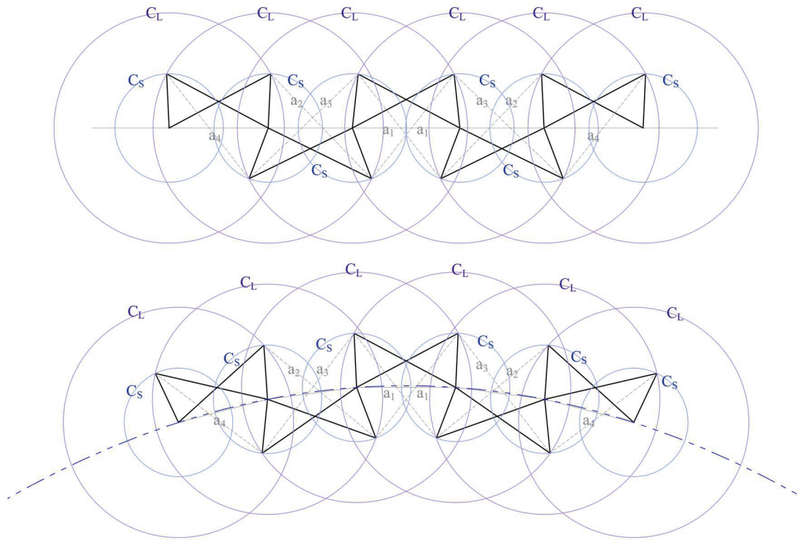
Figure 6.4. Transformation of a planar linkage composed of antiparallelogram loops from linear to parabola.
