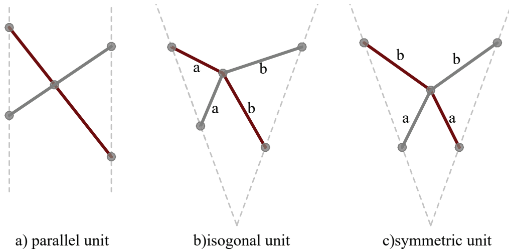
Figure 3.2. Three types of basic scissor units (Reproduced from: Zhang et al. 2016)
