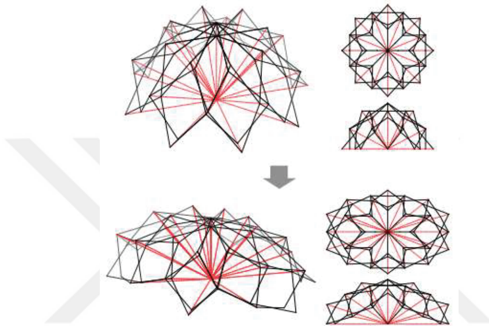
Figure 2.31. An example of the generalization of a spherical foldable scissor grid with a lamella rhomboid pattern, which is translated into an ellipsoidal grid with the same pattern and foldable deployment behavior. (Source: Roovers and Temmerman 2017b)
