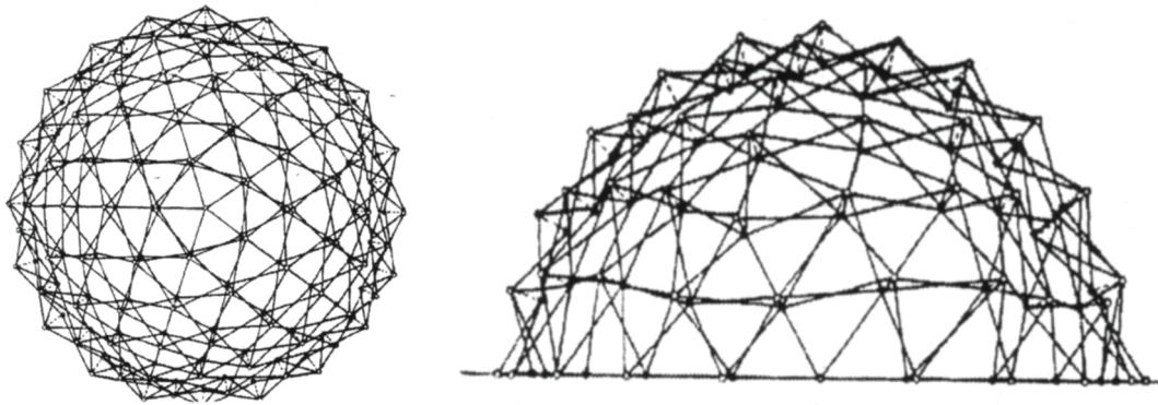
Figure 2.24. Top view and side elevation of a geodesic dome with polar units (Source: Escrig and Valcárcel 1987)
