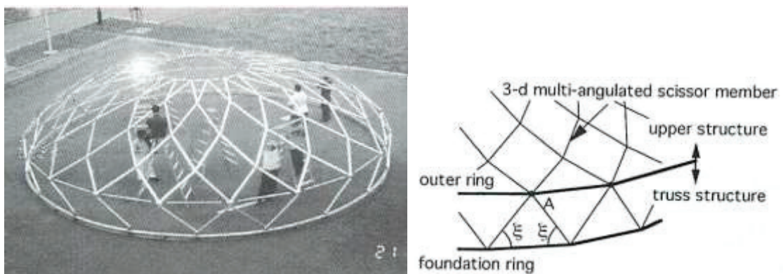
Figure 2.30. Model of retractable loop-dome and its outer and foundation rings (Source: Kokawa 2000)
