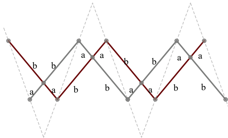
Figure 3.3. Polar scissor units forming a linkage making translational movement (Reproduced from: Maden, Akgün, et al. 2019)
