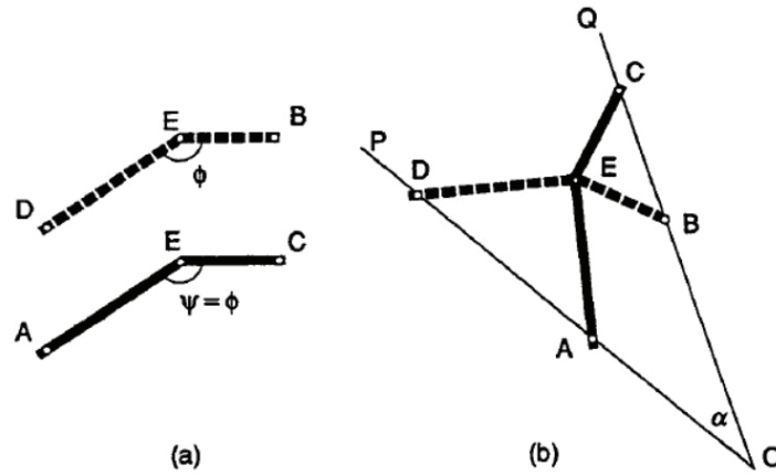
Figure 3.5. General type of Hoberman's element (Source: You and Pellegrino 1997)
