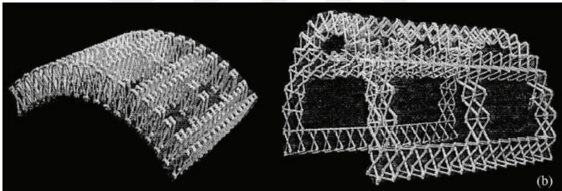
Figure 2.16. Single-curved foldable barrel vault. (Langbecker and Albermani 2000)
