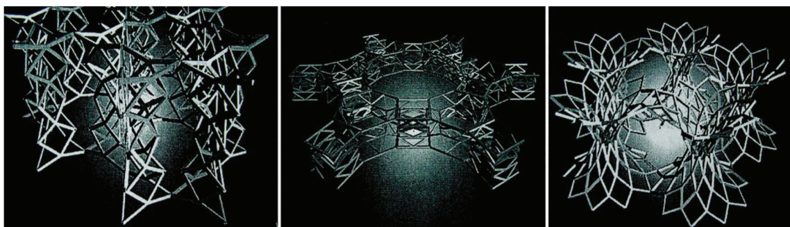
Figure 2.35. Deployable polygonal hyperboloids (Source: Alkhayer 2007)
