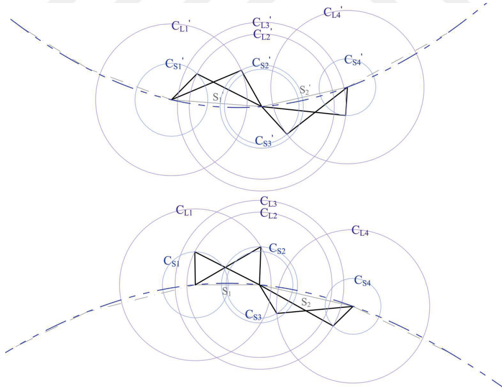
Figure 6.1. Forming antiparallelogram loops by matching the parameters for two cases.
