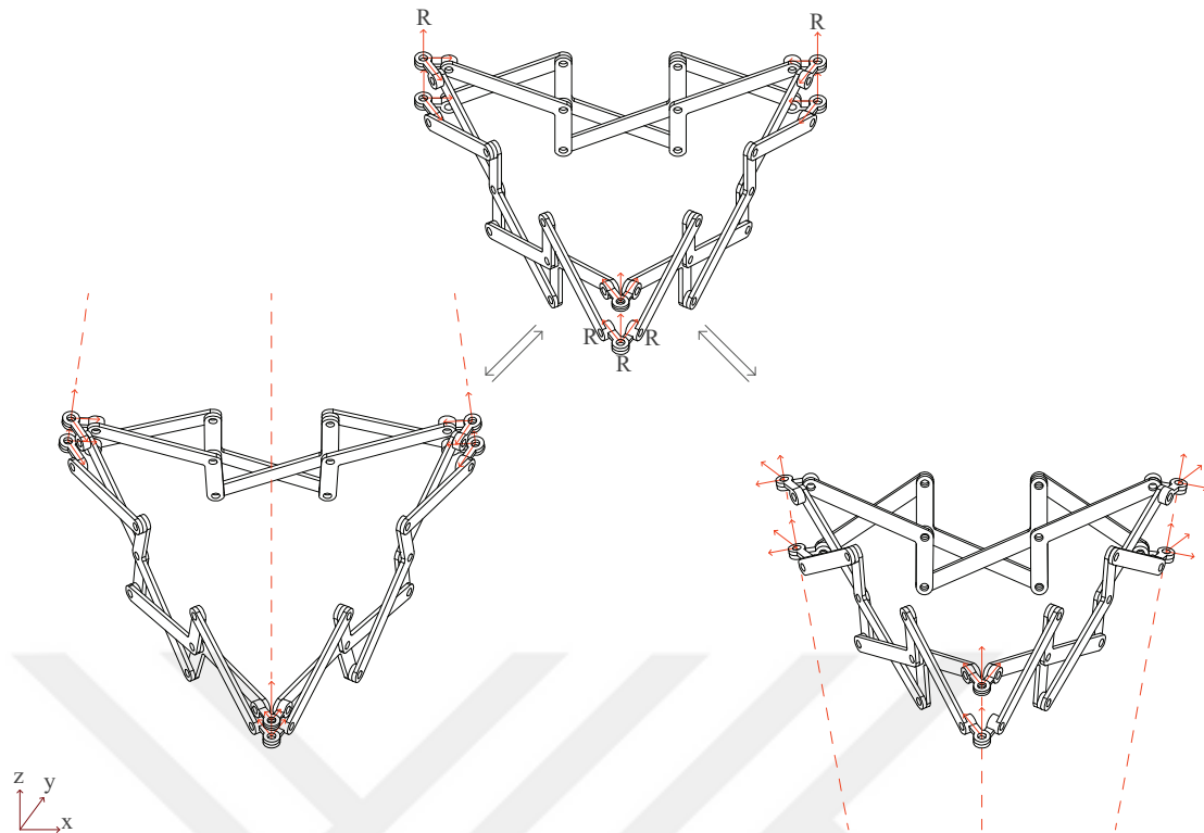
Figure 6.15 A triangular module constructed with antiparallelogram loops can transform concave to convex.
