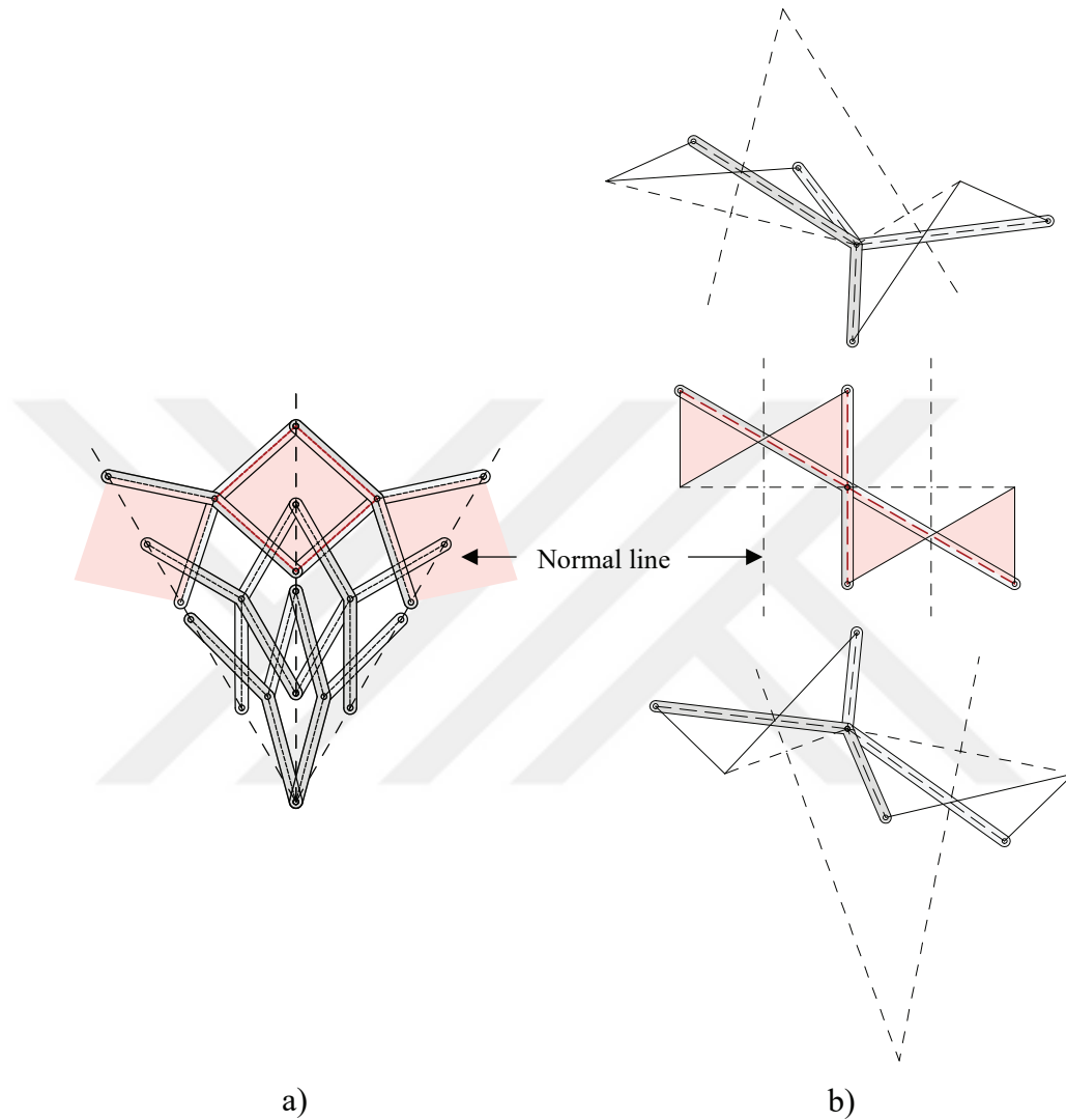
Figure 6.13 Motion sequence comparison of two types of scissor units composed of angulated arms: a) deployable type of scissor unit, b) transformable type of scissor unit.
