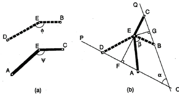
Figure 3.6. Simplest Type I GAE (Source: You and Pellegrino 1997)
