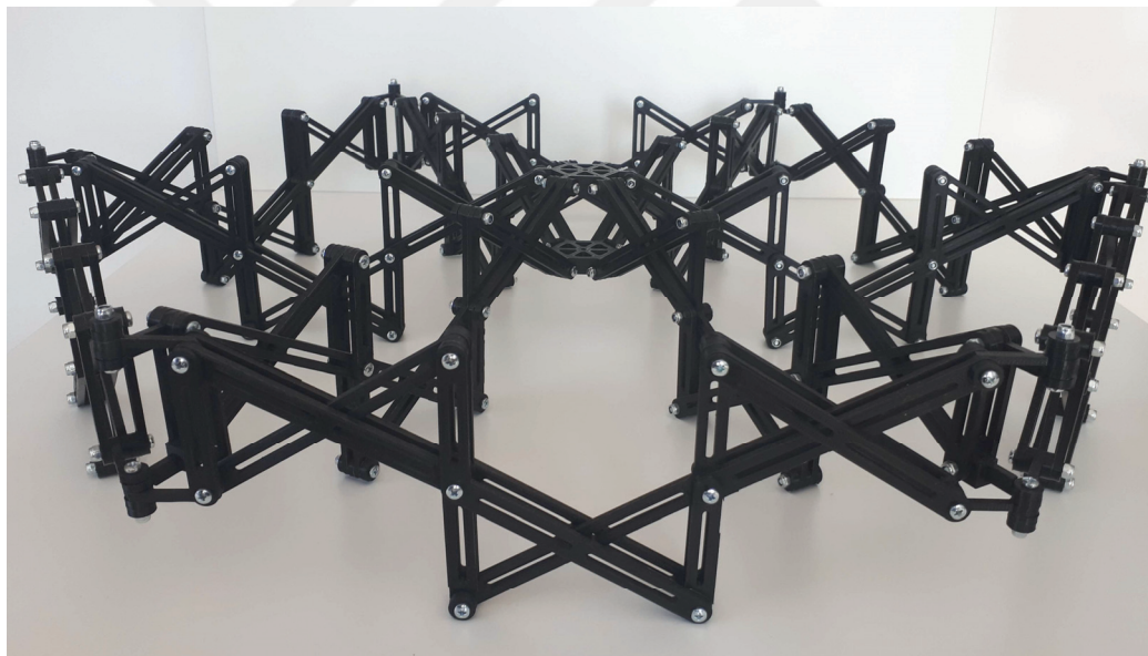
Figure 6.20 3D Printed model of the transformable linkage when it is flat position.
