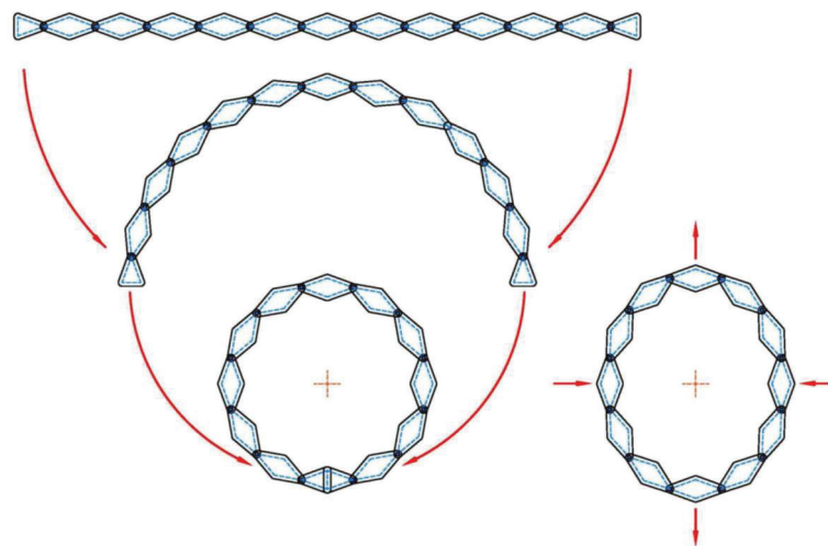
Figure 2.9. Forming hinged rhombi from open to closed chain (Source: Hoberman, Demaine, and Rus 2013)
