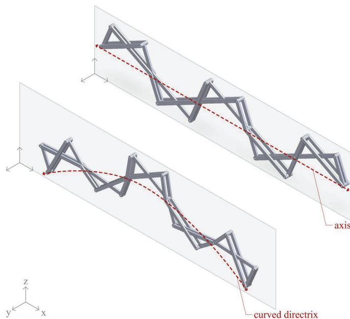
Figure 6.8 Scissor linkages defining a conoid axis and directrix.
