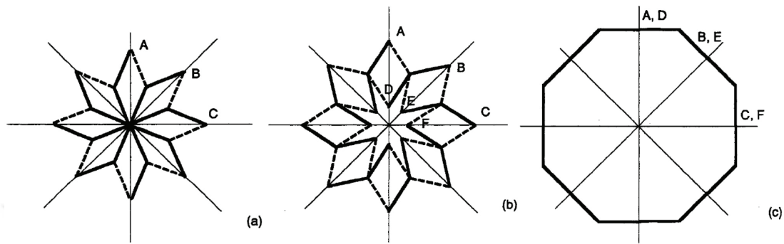
Figure 2.10. Foldable ring linkage formed by identical angulated rods with a kink angle of 135^\circ . (a) "Expanded" and (c) "retracted" configurations (Source: You and Pellegrino 1997)
