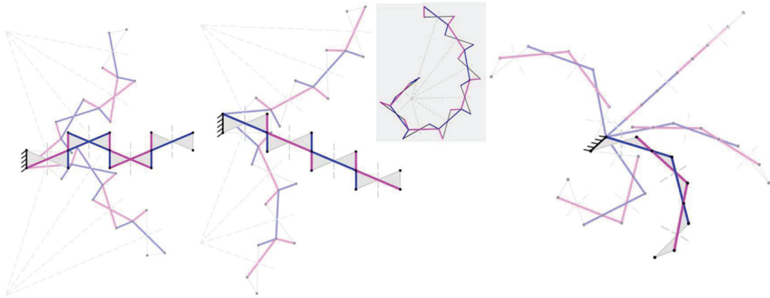
Figure 2.8. a) transformable linkage consists of angulated links, b) transformable linkage consists of ternary and quaternary links, c) transformable linkage consists of polar scissor units (Source: Gür, Korkmaz, and Kiper 2019)
