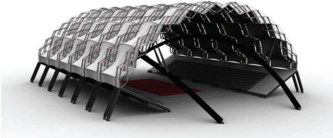
Figure 2.5. A scissor-hinged retractable membrane roof for a tennis arena (Source: Mele et al. 2010)
