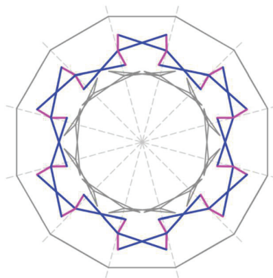
Figure 2.13. Deployable ring-like linkage consists of angulated links. (Source: Gür, Korkmaz, and Kiper 2019)
