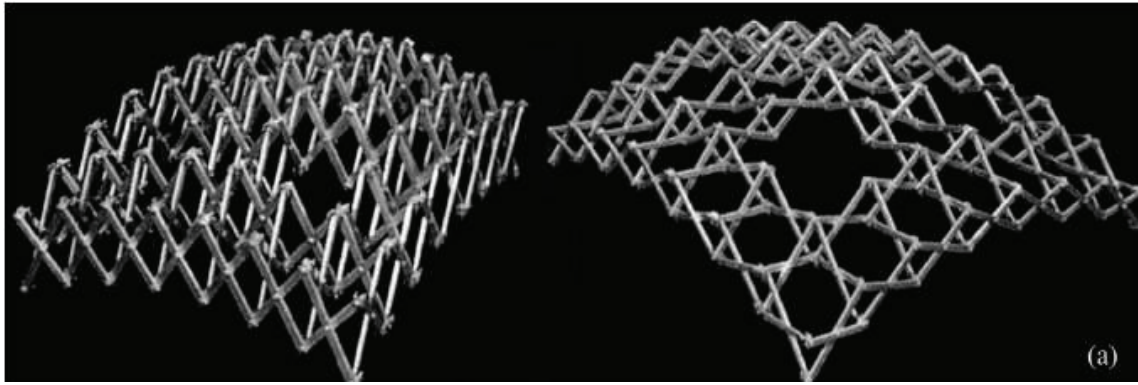
Figure 2.29. Double-curved synclastic scissor structure. (Source: Langbecker and Albermani 2000)
