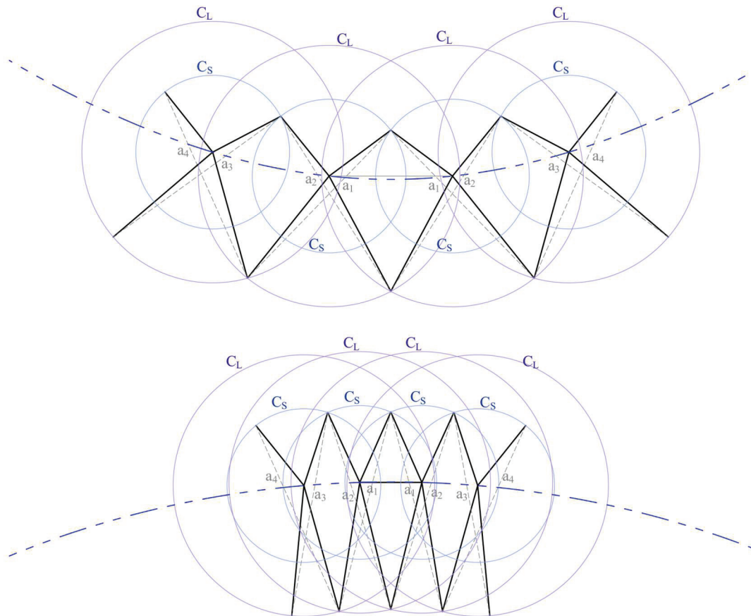
Figure 6.5. Transformation of a planar linkage composed of kite loops concave to convex conic curves.
