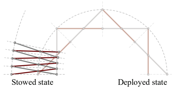
Figure 3.15. Angular deployment.
