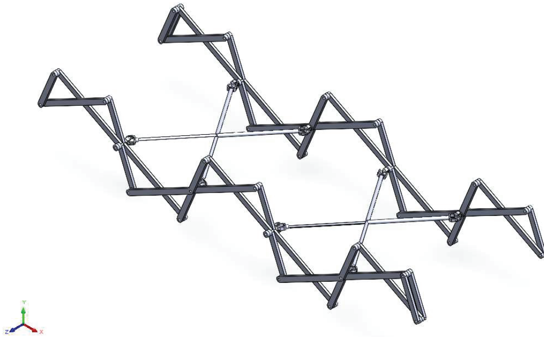
Figure 6.10 A model composed of planar linkages connecting with lazy-tong mechanisms
