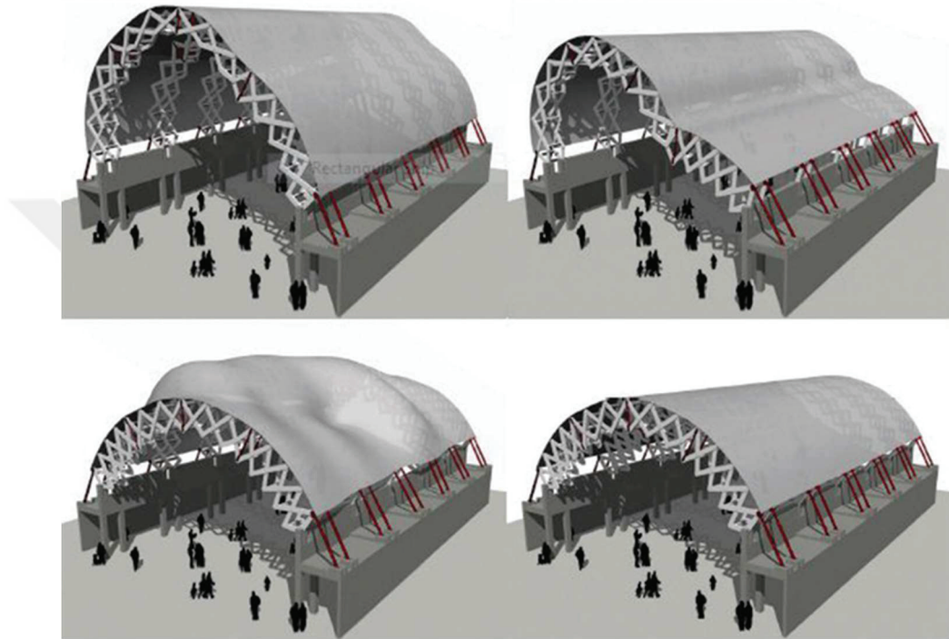
Figure 2.38. Adaptive roof structure composed of scissor arches. (Source: Akgün et al. 2010)
