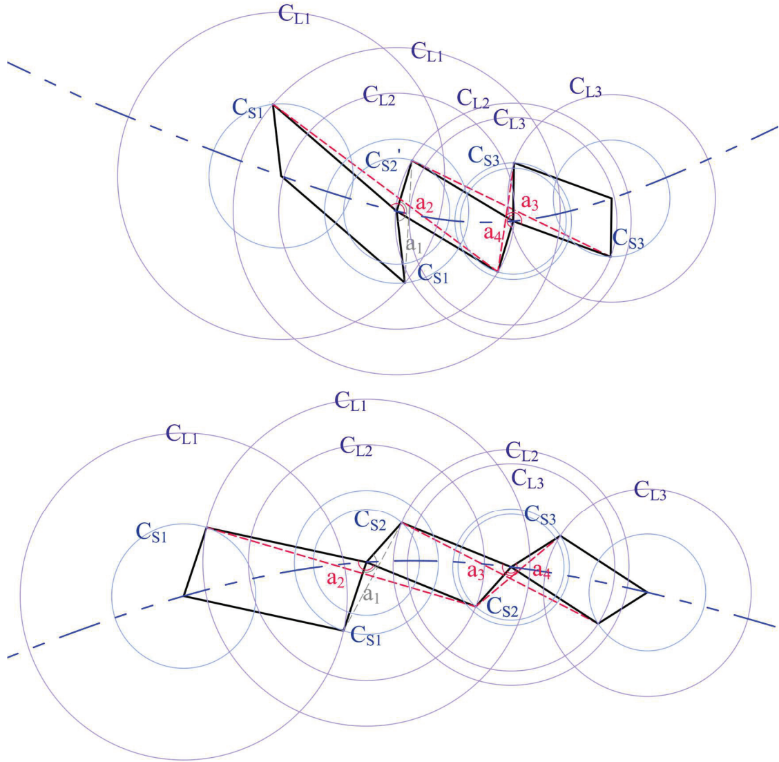
Figure 6.7 Concave and convex forms of parallelogram loop assemblies on a conic curve.
