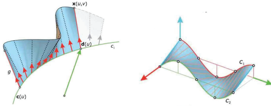
Figure 4.14. Free form ruled surfaces generated by a) moving line segment a long directrix, b) joining two points on parametrized curves. (Source: Pottmann et al. 2007)
