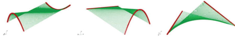
Figure 5.2. Typical examples of Catalan surfaces, respectively from the left to right: a cylindroid, a conoid; a hyperbolic paraboloid (Source: Dzwierzynska 2019)
