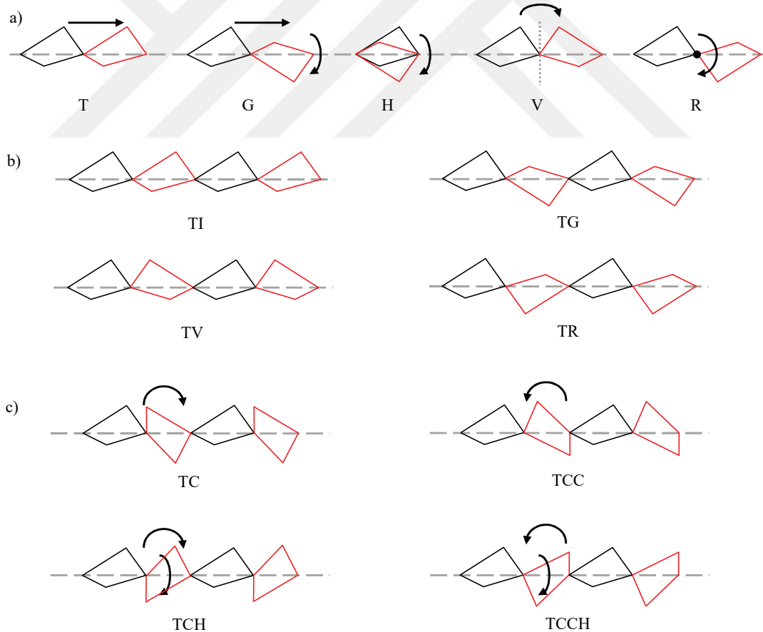
Figure 5.5. a) Basic isometry operations, b) the first four frieze patterns, c) long-short diagonal connections (Source: Kiper et al. 2022)
