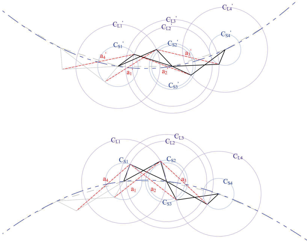
Figure 6.2. Equalization of kink angles of angulated elements.
