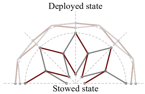
Figure 3.13. Radial deployment.
