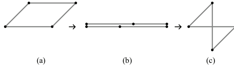
Figure 3.12. Assembly mode change of a parallelogram loop (a) into a antiparallelogram loop (c) through the singular configuration (b) (Reproduced from: Usiskin et al. 2008)
