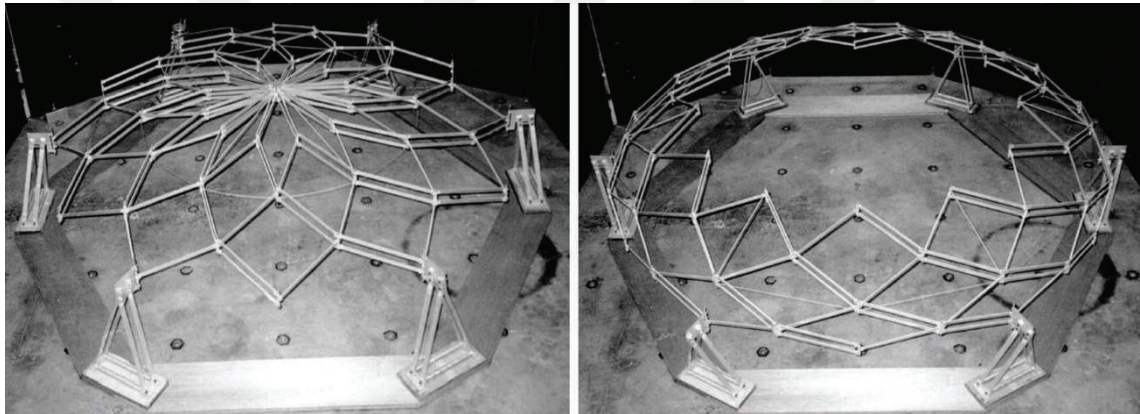
Figure 2.28. Deployable structure composed of multi-angulated elements. (Source: Kassabian, You, and Pellegrino 1999)
