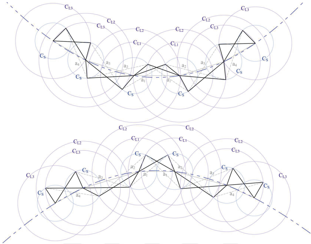
Figure 6.3. Planar scissor linkage is obtained with antiparallelogram loops that can define concave and convex conic curves.
