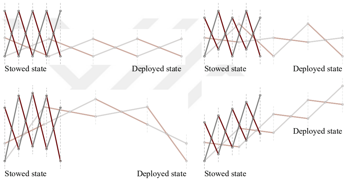
Figure 3.14. Types of linear deployment.
