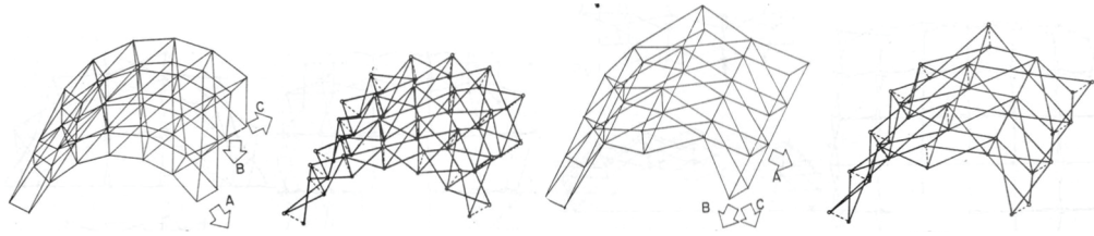
Figure 2.15. Two examples of the three-way spherical grid with translational units (Escrig and Valcárcel 1987)
