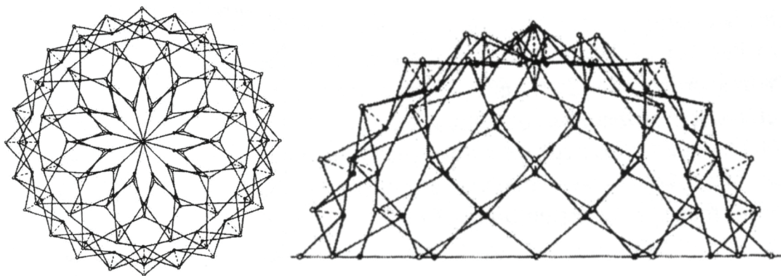
Figure 2.25. Top view and side elevation of a lamella dome with identical polar units (Source: Escrig and Valcárcel 1987)
