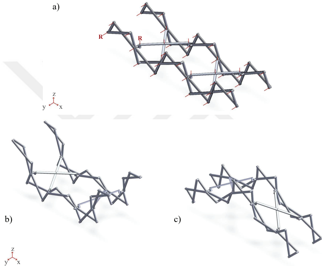
Figure 6.9 A model composed of planar linkages connecting with middle hinged straight bars a) flat position, b) convex vault, c) concave vault.
