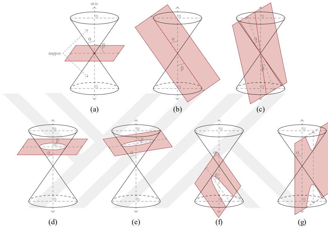
Figure 5.1. Conic sections (Reproduced from: Lastra 2021)
