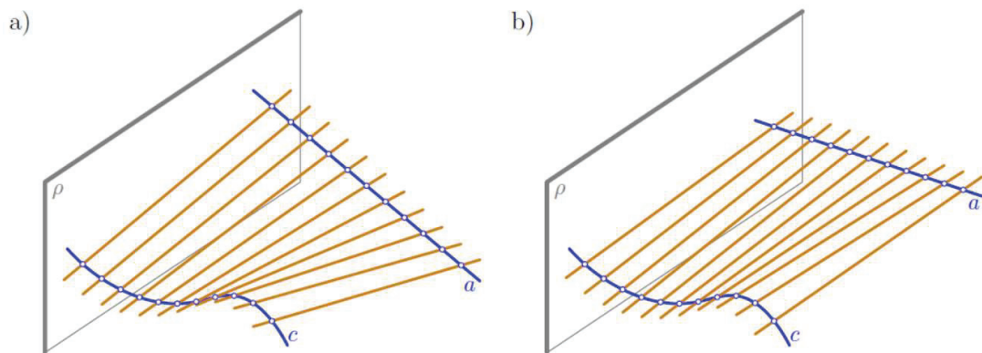
Figure 5.3. Illustration of a) general, and b) right conoid (Source: Dolezal 2011)
