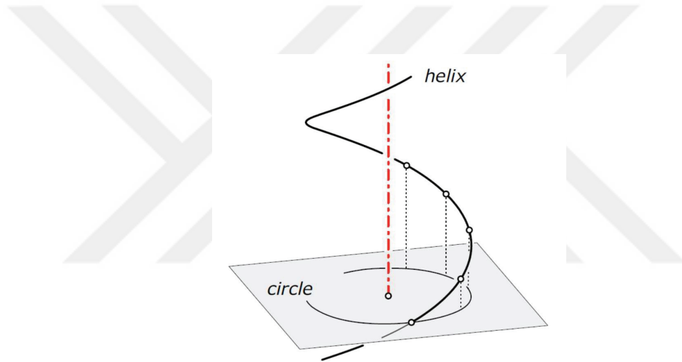
Figure 4.2. Comparison of circle (planar curve) and helix (spatial curve) (Source: Pottmann et al. 2007)
