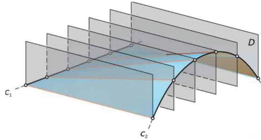
Figure 4.19. All rulings of a conoid are parallel to the director plane (D) and intersect a straight line c_1 and, c_2 are directrices (Source: Pottmann et al. 2007)
