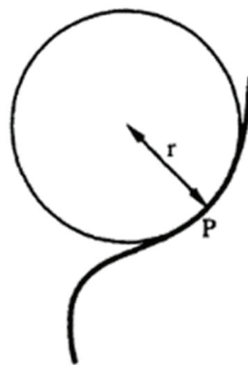
Figure 4.5. The curvature of a planar curve at a point P. (Source: Hyde et al. 1997)
