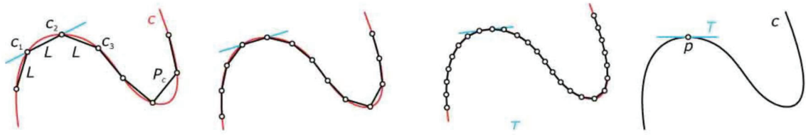
Figure 4.4. Evaluation of a discrete curve. (Source: Pottmann et al. 2007)
