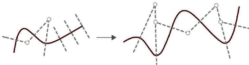
Figure 3.16. Transformation (Source: Maden, Akgün, et al. 2019)
