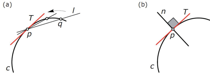
Figure 4.3. a) A tangent T touches a curve c , b) The normal of a planar curve intersects the curve at a right angle. (Source: Pottmann et al. 2007)
