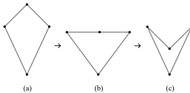
Figure 3.11. Assembly mode change of a kite loop (a) into a dart loop (c) through the singular configuration (b) (Reproduced from: Usiskin et al. 2008)
