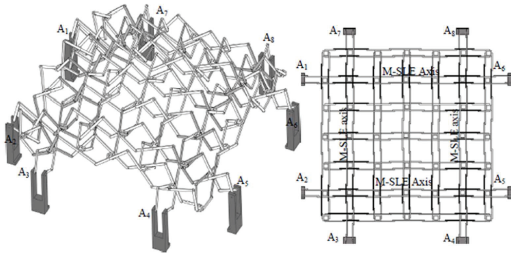
Figure 2.39. Perspective and top view of the proposed scissor-hinge shell structure (Source: Akgün et al. 2011)
