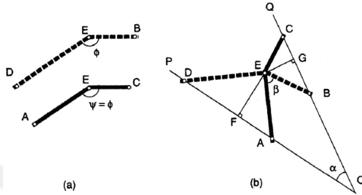
Figure 3.7. Simplest Type II GAE (Source: You and Pellegrino 1997)
