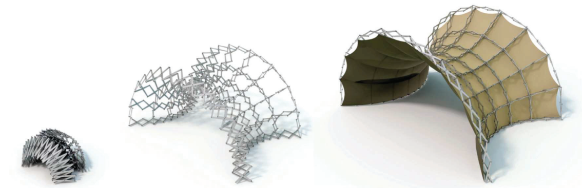
Figure 2.40. Deployable catenoid (Source: Roovers, Alegria Mira, and Temmerman 2013)
