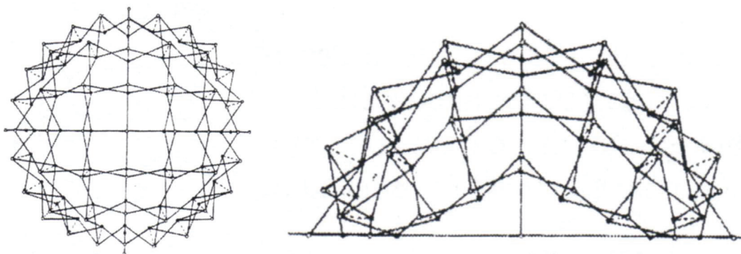
Figure 2.22. Top view and side elevation of a two-way spherical grid with identical polar units (Source: Escrig and Valcárcel 1987)
