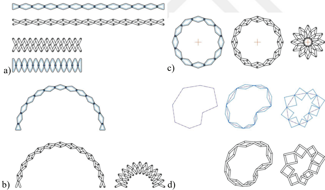
Figure 3.9. a) Rhombi on a line b) rhombi on an arc c) rhombi on a circle d) rhombi on an irregular geometry (Source: Hoberman, Demaine, and Rus 2013)
