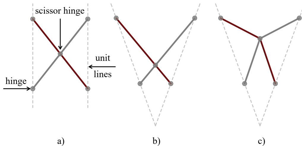
Figure 3.1. Basic scissor unit a) Translational unit b) Polar unit c) Angulated unit (Reproduced from: Maden, Akgün, et al. 2019)
