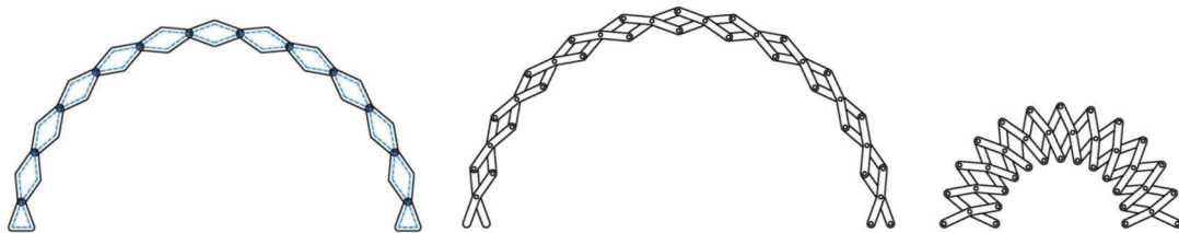
Figure 2.2. a) Hinged rhombs on an arc b) Open and deployed forms of resulting linkage (Source: Hoberman, Demaine, and Rus 2013)
