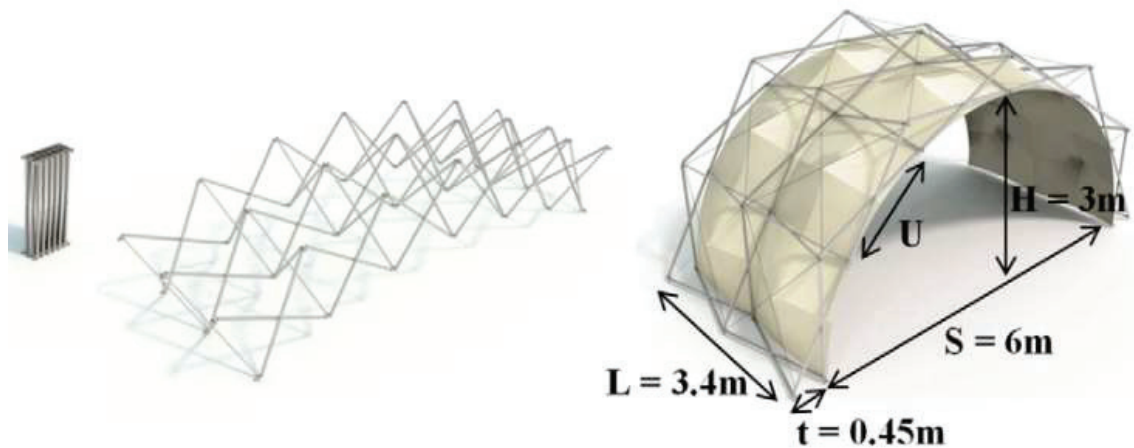
Figure 2.19. The conceptual design for a 4-person shelter comprised of deploying scissor arches with a membrane. (Source: Alegria Mira, Thrall, and Temmerman 2014)
