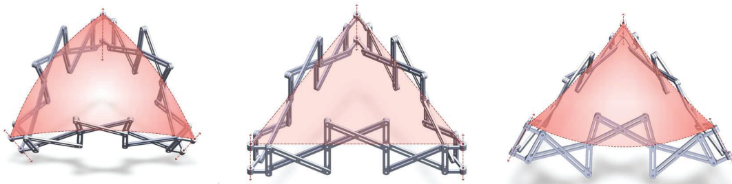
Figure 6.16. The motion sequence of a triangular module transforming concave to convex from left to right.
