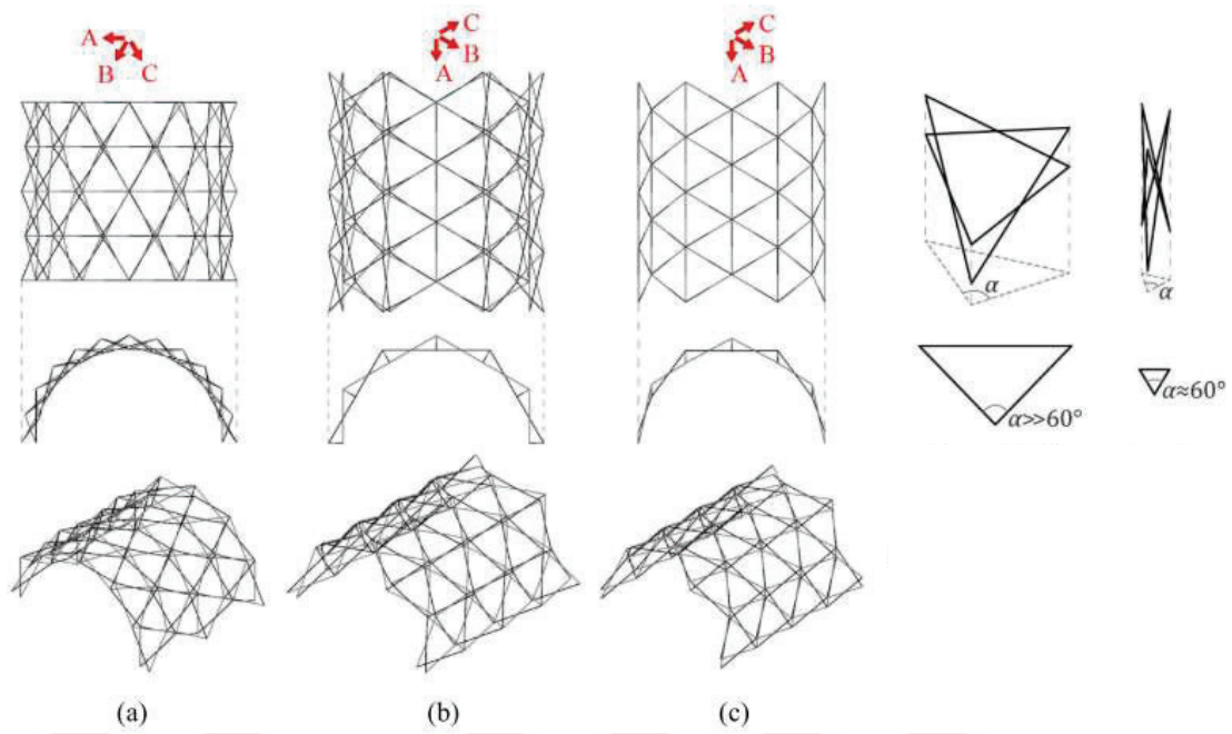
Figure 2.20. Three types of triangulated single curved scissor grids consisting of: a) polar units; b) polar and plane-translational units; c) plane- and curved-translational units Source: Roovers and Temmerman 2014a).
