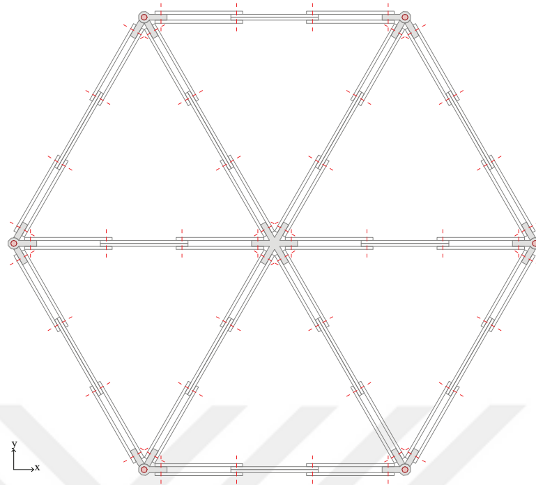
Figure 6.18 Top view of the network constructed scissor linkage.
