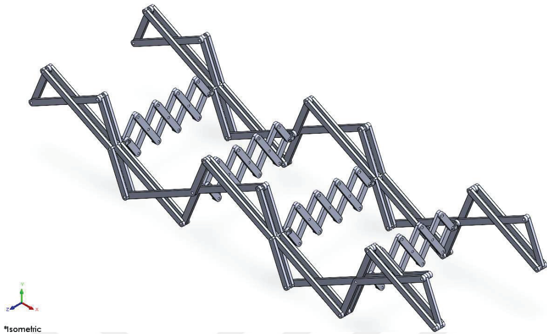
Figure 6.11 A model composed of planar linkages connecting with telescopic middle bars.
