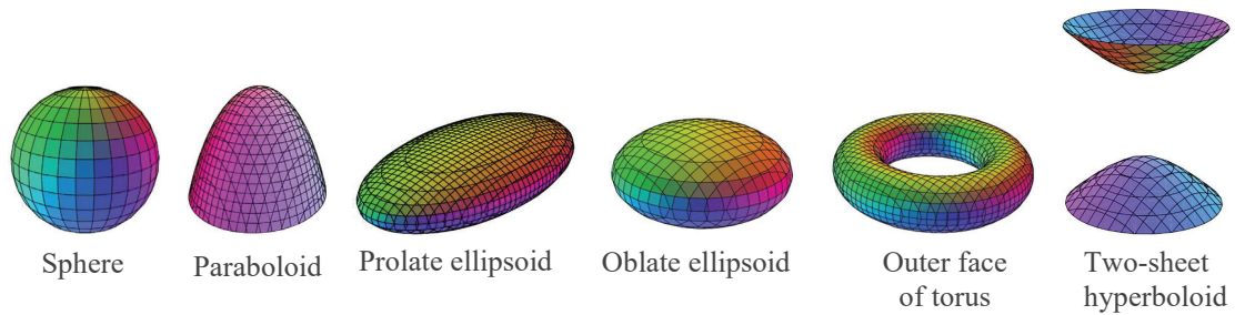
Figure 4.17. Examples of synclastic surfaces (Generated with CalcPlot3D)
