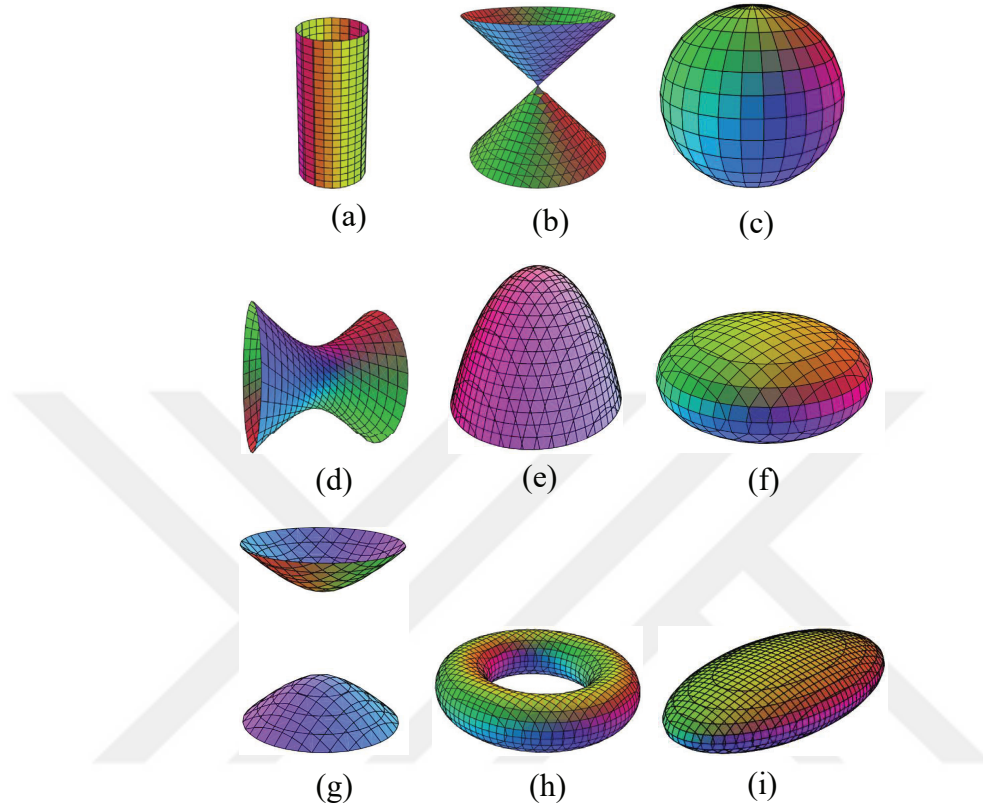
Figure 4.11. Examples of rotational surfaces (a) cylinder, (b) cone, (c) sphere, (d) one-sheet rotational hyperboloid, (e) rotational paraboloid, (f) oblate rotational ellipsoid, (g) two-sheet rotational hyperboloid, (h) torus, (i) prolate rotational ellipsoid. (Generated with CalcPlot3D).
