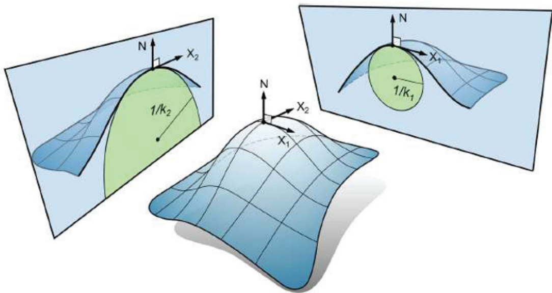
Figure 4.6. Measures of 3D surface curvature represent the greatest and lowest normal curvatures k_1 and k_2 using orthogonal unit vectors X_1 and X_2 (Source: Nabavi and Fossen 2021)
