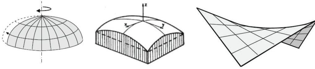
Figure 4.9. Illustrations of rotational surface, translational surface, and ruled surface. (Source: Blaauwendraad and Hoefakker 2014)
