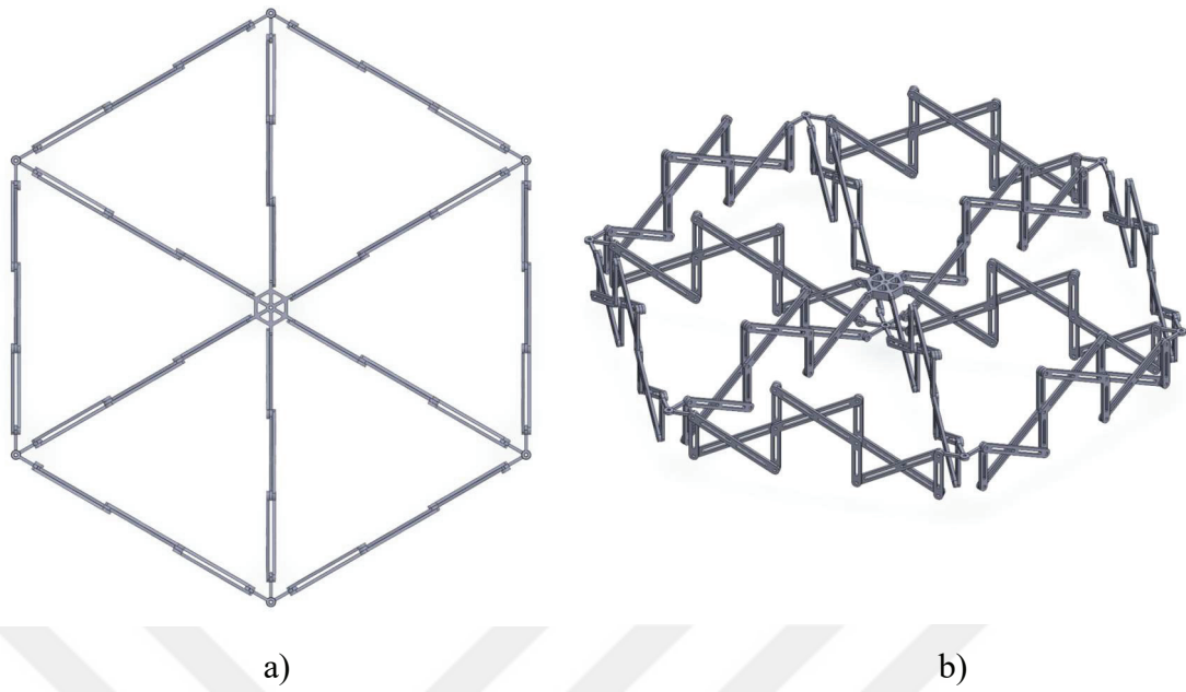
Figure 6.19 a) Top view of the linkage, b) Flat form of the linkage.
