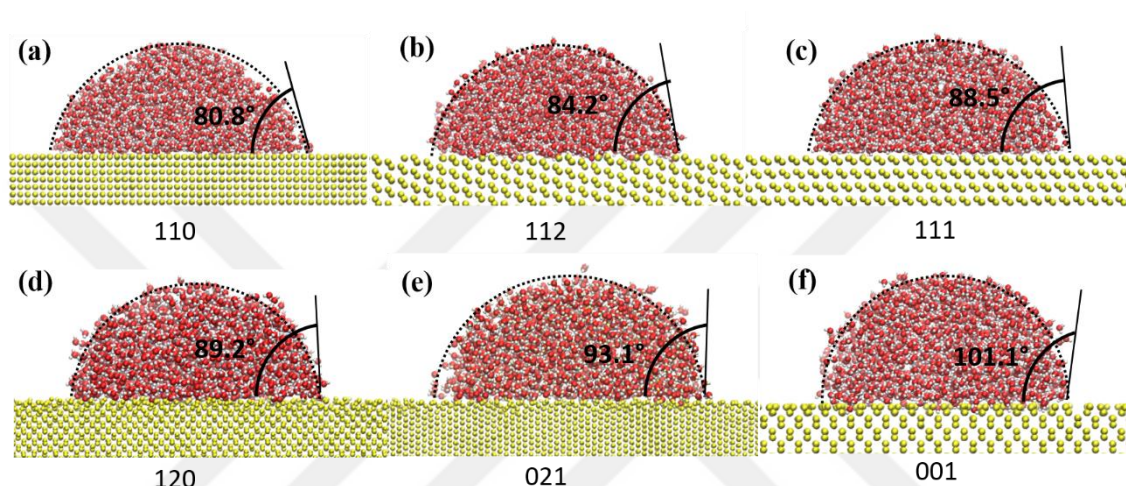
Figure 3.3. Measured of contact angles of crystalline silicon surfaces (a) Si (110), (b) Si (112), (c) Si (111), (d) Si (120), (e) Si (021) and (f) Si (001).
