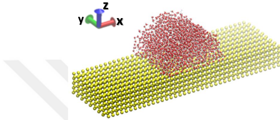
Figure 3.1. Semi cylindrical water nano droplet on the surface. Atoms present as hydrogen- white, oxygen-red and silicon-yellow.
