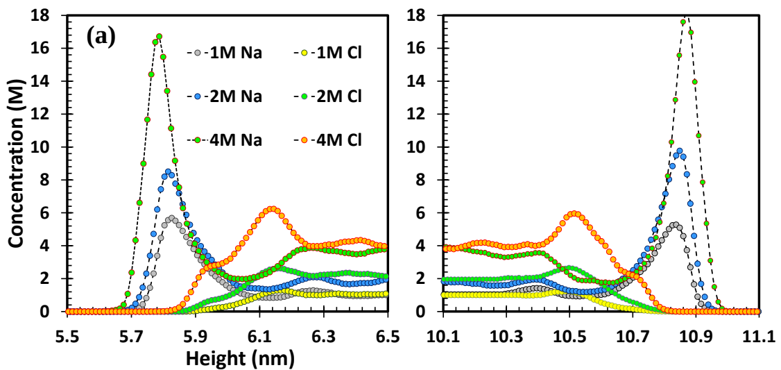
Figure 4.8. Ionic distributions of Na + and Cl - under different concentrations.
