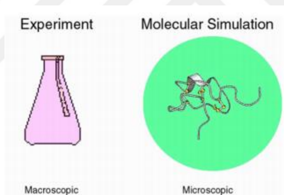
Figure 2.2. Comparison of macroscopic and microscopic results 84 .
