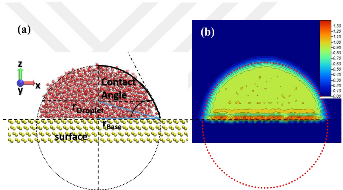
Figure 3.2. (a) Snapshot of measurement technique of contact angles, (b) water density contours.
