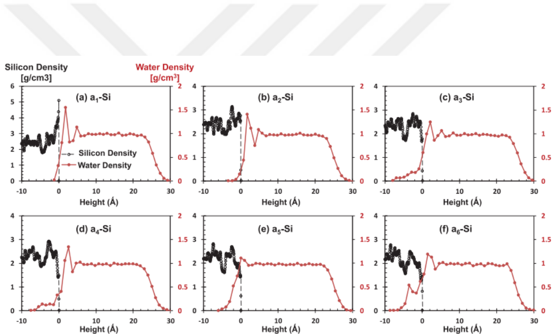
Figure 3.8. Distribution of silicon and water molecules for amorphous silicon structures. Black and red lines are silicon density and water density, respectively.
