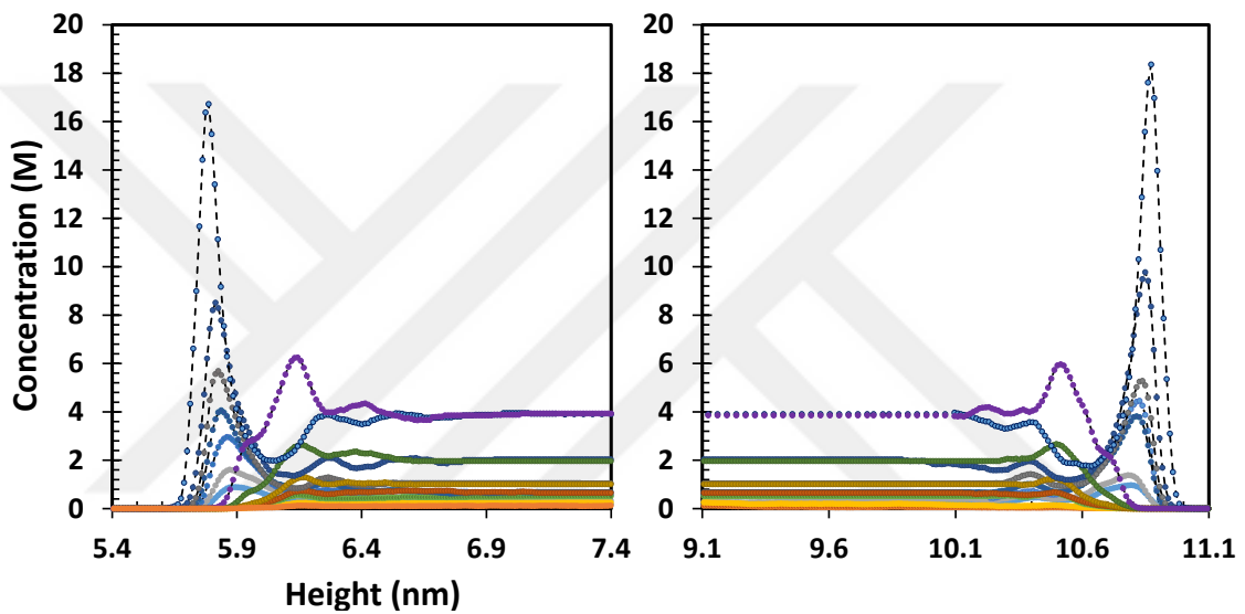
Figure 4.8. Ionic distributions of Na + and Cl - under different concentrations.
