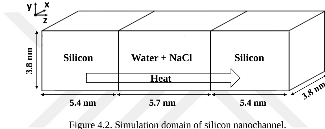
Figure 4.2. Simulation domain of silicon nanochannel.
