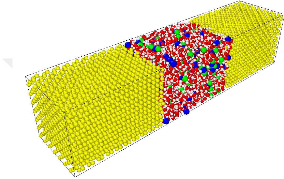
Figure 2.3. Modeling of different numbers and atoms with Molecular Dynamics.
