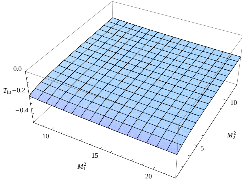
Figure 4.3: The dependence of the form factor T_{1B} on Borel mass parameters M_1^2 and M_2^2 at q^2 = 0 for s_0 = 34GeV^2 and s'_0 = 4GeV^2 .
