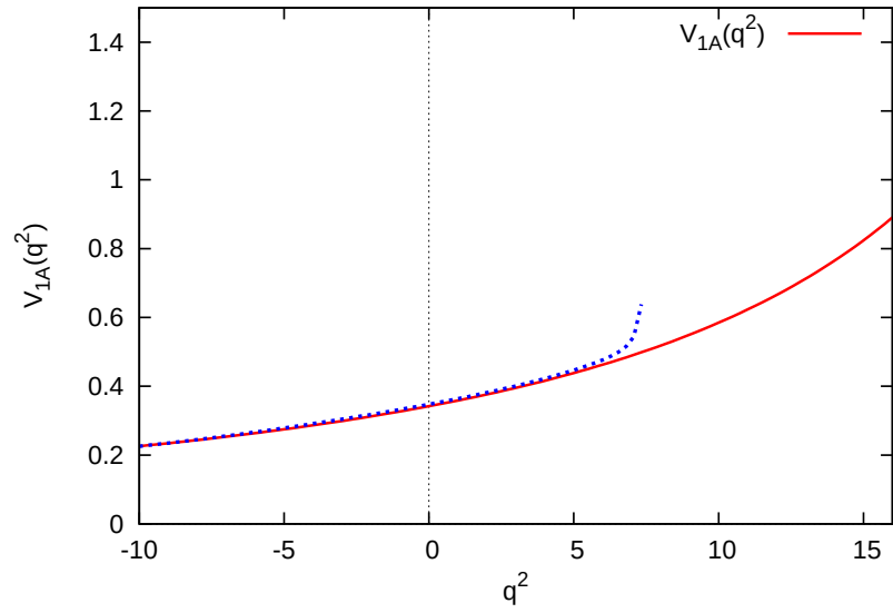
Figure 4.8: The q^2 dependence of the form factor V_{1A} , sum rules prediction(blue-dashed) and fitted(red-solid) for M_1^2 = 16GeV^2 , M_2^2 = 6GeV^2 and s_0 = 34GeV^2 , s'_0 = 4GeV^2 .
