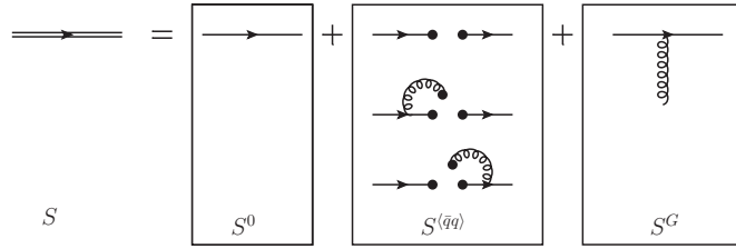
Figure 2.2: Diagrammatic representation of the full quark propagator. For q = b, c, t , the second term S^{(\bar{q}q)} vanish.
