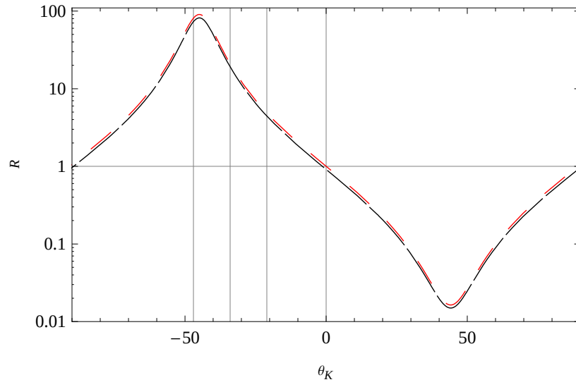
Figure 4.25: The \theta_{K_1} dependance of the ratios(R) of branching fractions R = \frac{\mathcal{B}(B \rightarrow K_1(1270)e^+e^-)}{\mathcal{B}(B \rightarrow K_1(1400)e^+e^-)} (black-dashed) and R = \frac{\mathcal{B}(B \rightarrow K_1(1270)\mu^+\mu^-)}{\mathcal{B}(B \rightarrow K_1(1400)\mu^+\mu^-)} (red-dashed).
