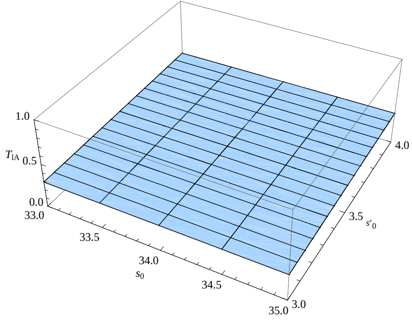
Figure 4.4: The dependence of the form factor T_{1A} on continuum thresholds s_0 and s'_0 at q^2 = 0 for M_1^2 = 16GeV^2 and M_2^2 = 6GeV^2 .
