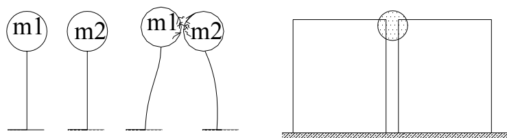
Figure 3.33. Dynamic pounding model for one-storey building
