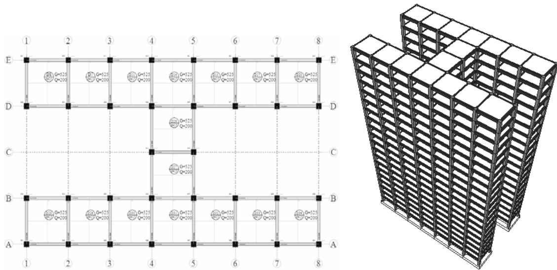
Figure 5.18. Structural plan and 3D view of parametric model IVb
