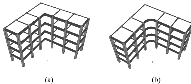
Figure 3.11. Softening Reentrant corners: (a) Before softening, (b) After softening
