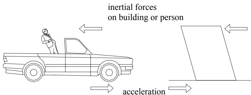
Figure 4.3. Inertia forces
