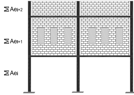
Figure 3.17. Formation mechanism of Weak Storey (B1)
