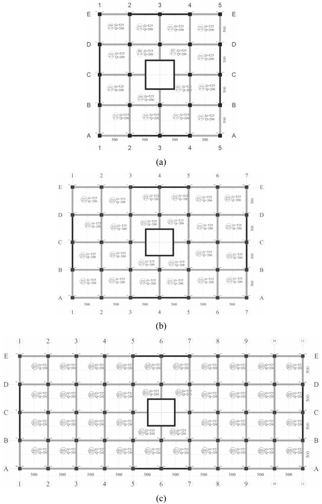
Figure 5.4. Structural plans of parametric model Id a) Id 20x20, b) Id 20x30, c) Id 20x50
