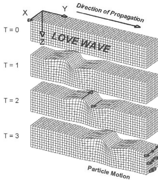
Figure 2.4. Perspective view of L-wave (Source: Braile, 2006)
