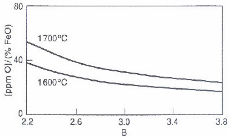
Figure 2.6. Equilibrium Ratio [\text{ppm O}] / (\% \text{ FeO}) Related to Slag Basicity [9]
