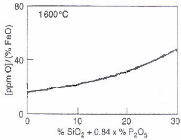
Figure 2.5. Equilibrium Ratio [\text{ppm O}] / (\% \text{ FeO}) Related to \text{SiO}_2 and \text{P}_2\text{O}_5 [9]
