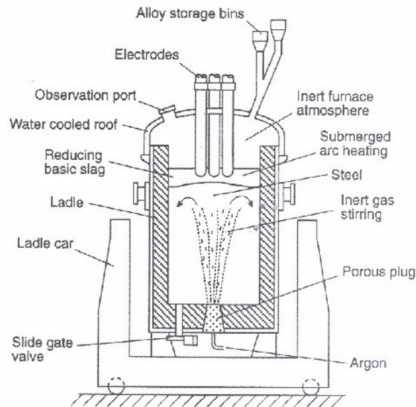
Figure 2.9. Sketch of Ladle Furnace [9]
