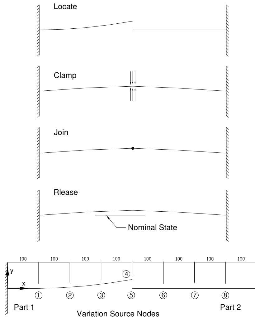
Figure 3.3 Example Problem for Two-Beam Assembly
