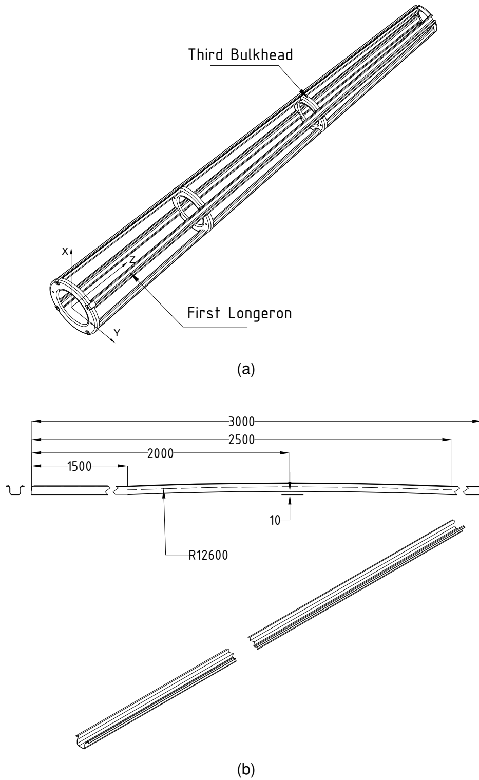
Figure 4.7 Possible Deviations on the Longerons and Bulkhead
