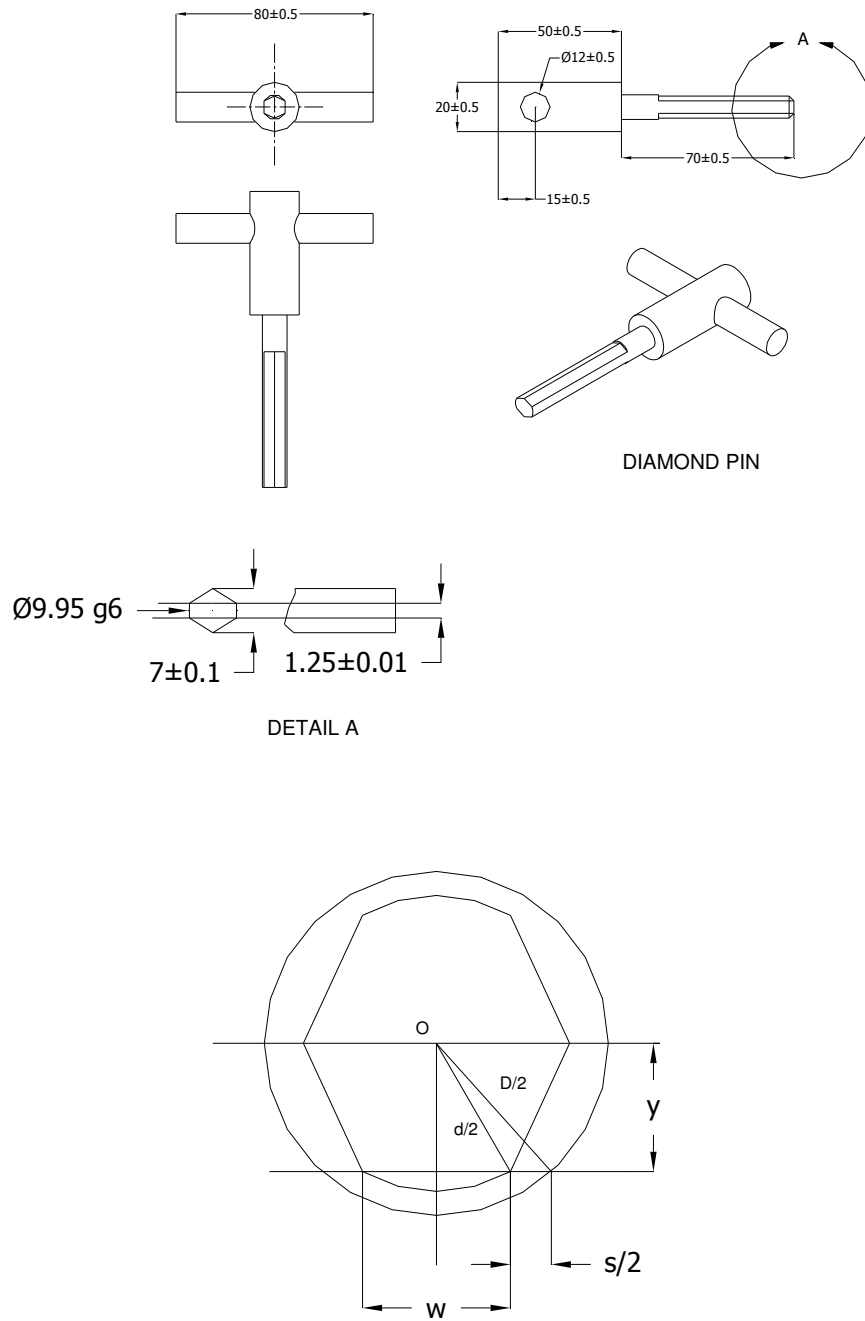
Figure D.2 Assembly Fixture Component Drawings (continued)
