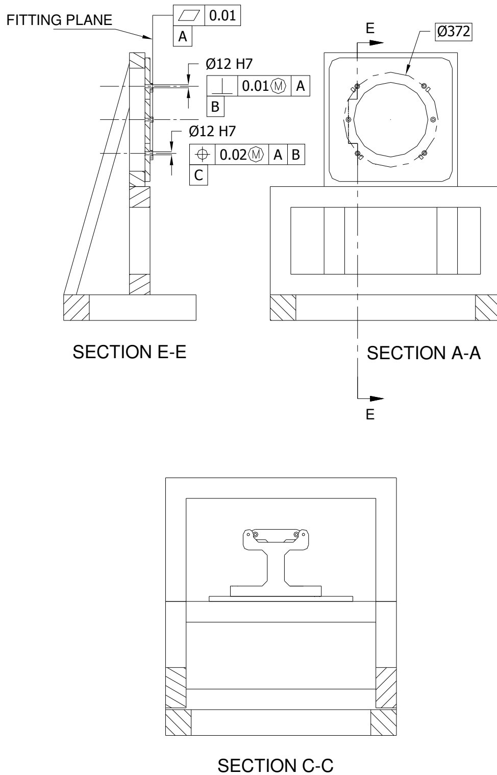
Figure D.1 Tail Cone Assembly Fixture, Assembly Drawings (continued)
