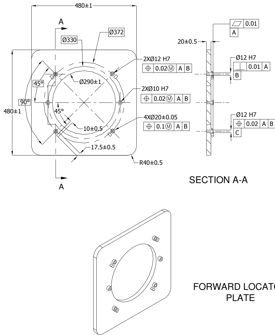
Figure D.2 Assembly Fixture Component Drawings
