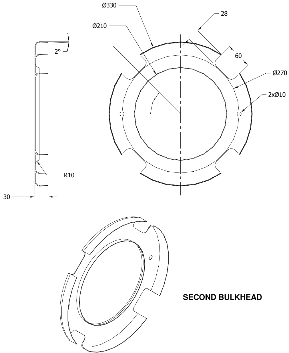
Figure C.2 Tail Cone Component Drawings (continued)
