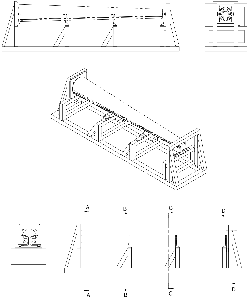
Figure D.1 Tail Cone Assembly Fixture, Assembly Drawings (continued)
