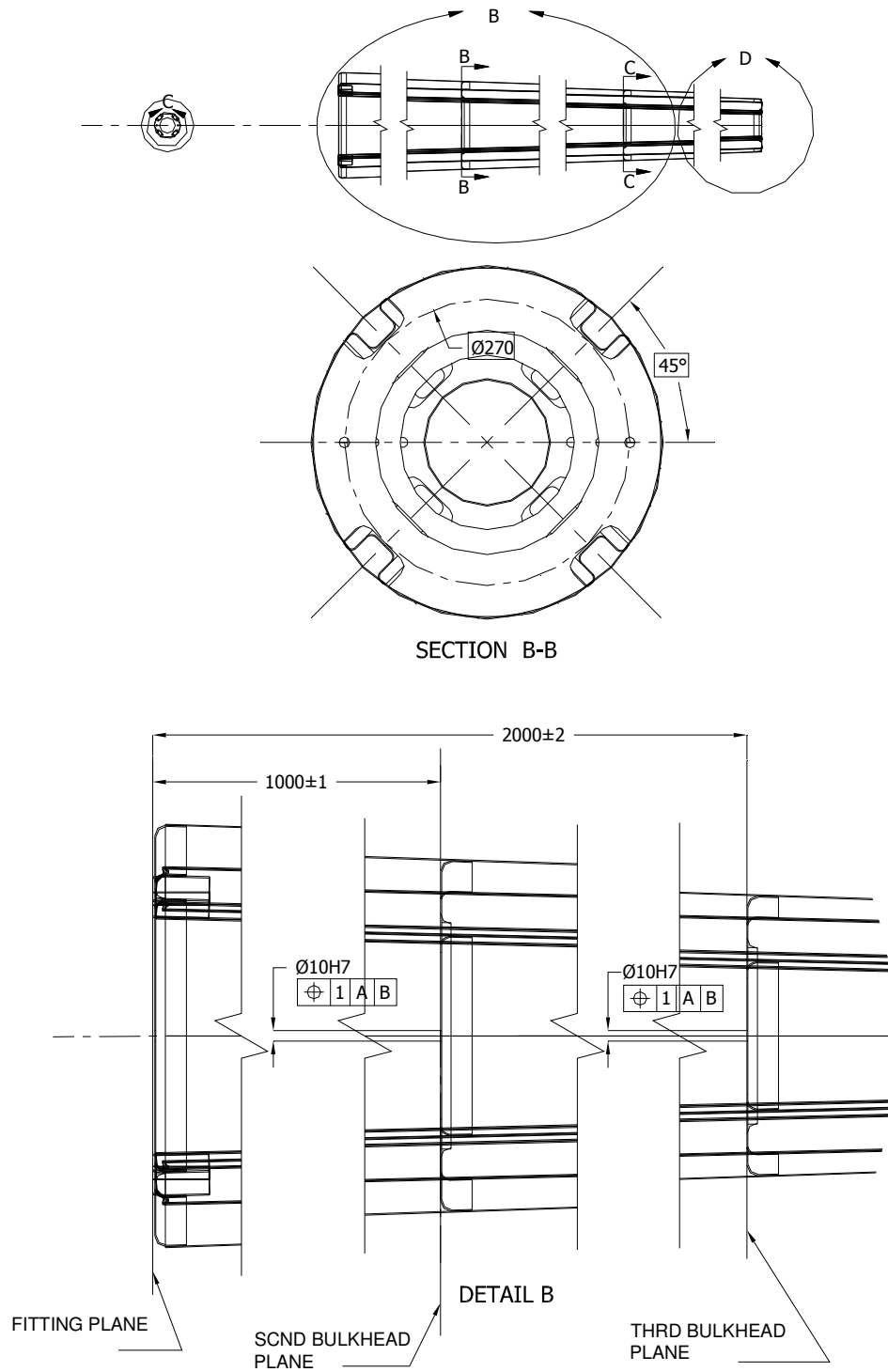
Figure C.1 Tail Cone Assembly Drawings (continued)
