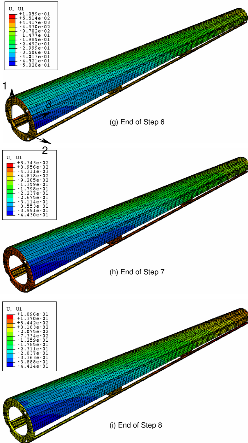
Figure 4.16 Deformations in X direction at the end of each Steps (continued)
