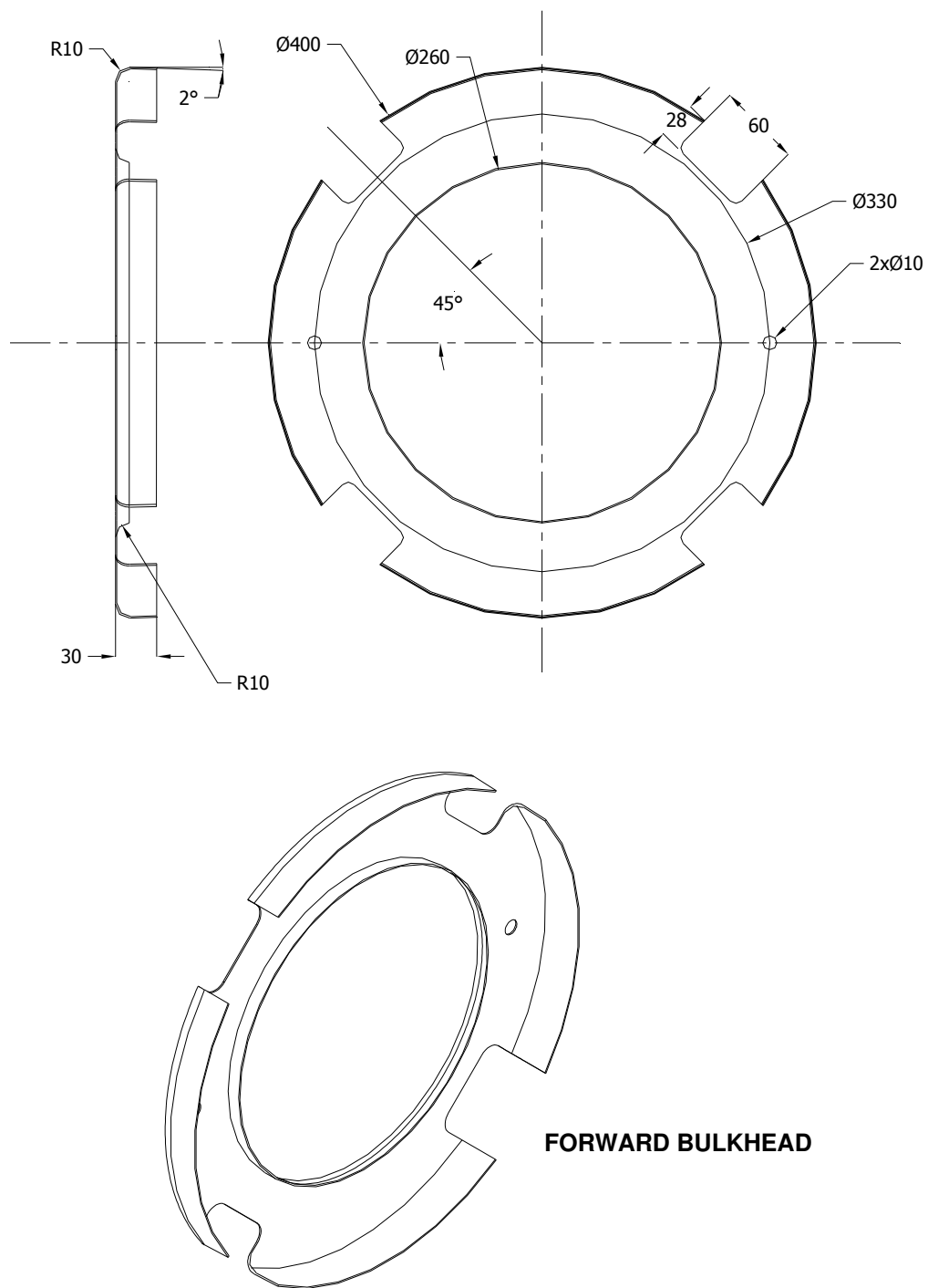
Figure C.2 Tail Cone Component Drawings
