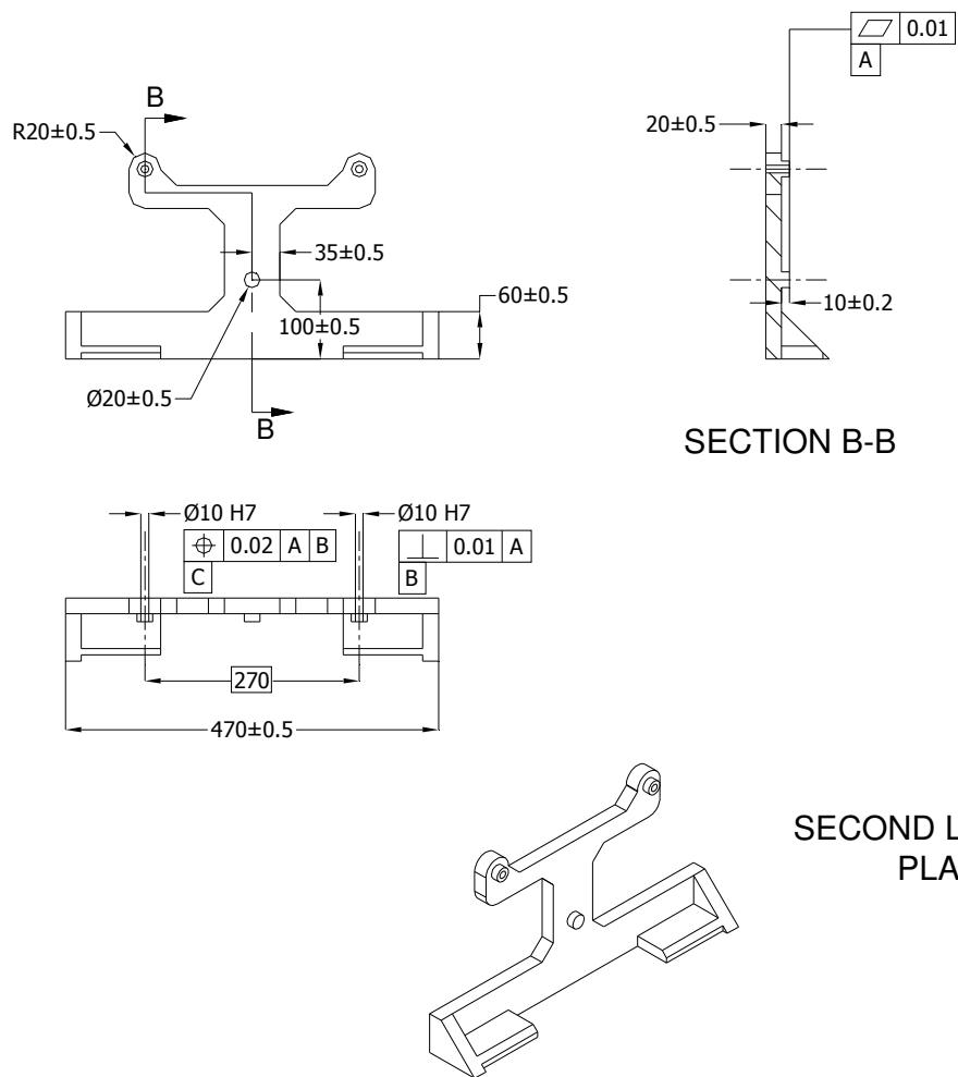
Figure D.2 Assembly Fixture Component Drawings (continued)
