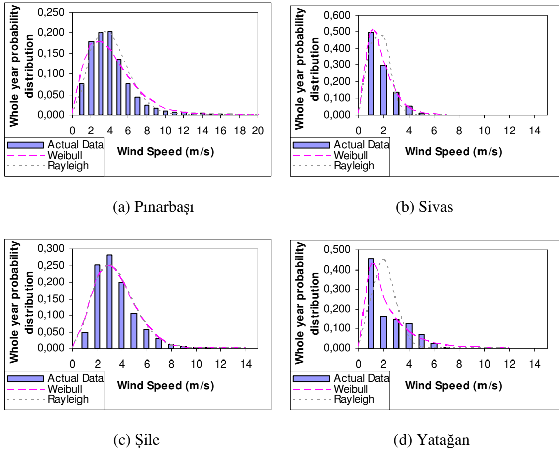
Figure 5.4. Fitted Weibull and Rayleigh distributions for Pınarbaşı, Sivas, Şile and Yatağan
