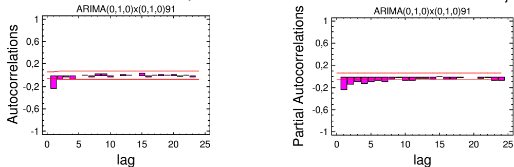
Residual Autocorrelations for adjusted Load Residual Partial Autocorrelations for adjusted Load
