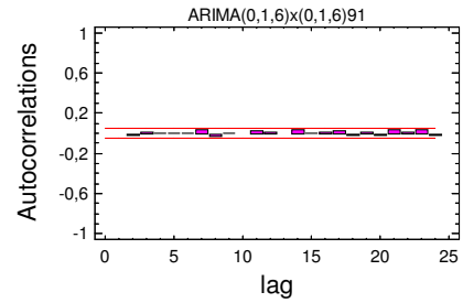
Residual Autocorrelations for adjusted Load
