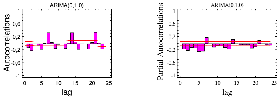
Residual Autocorrelations for adjusted Loac Residual Partial Autocorrelations for adjusted Load
