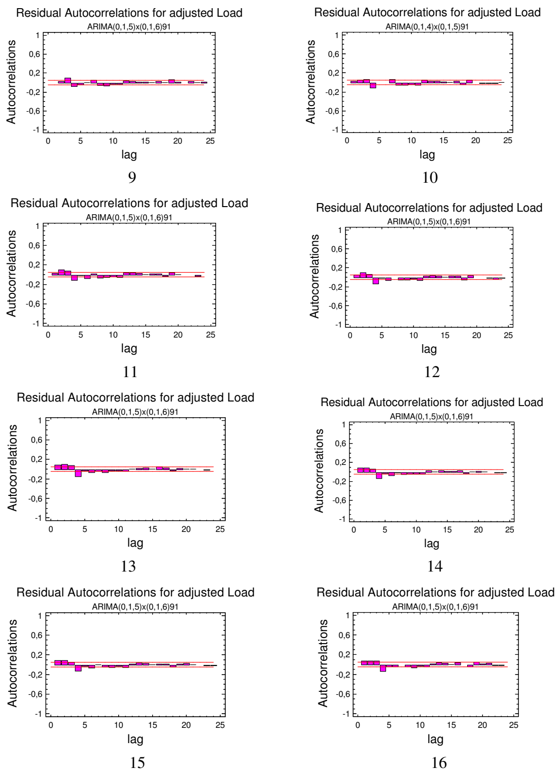
Figure B.4. Autocorrelation functions for region 4 (Continued)
