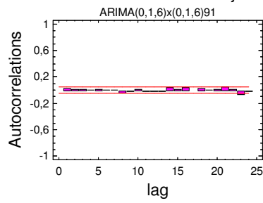
Residual Autocorrelations for adjusted Load
