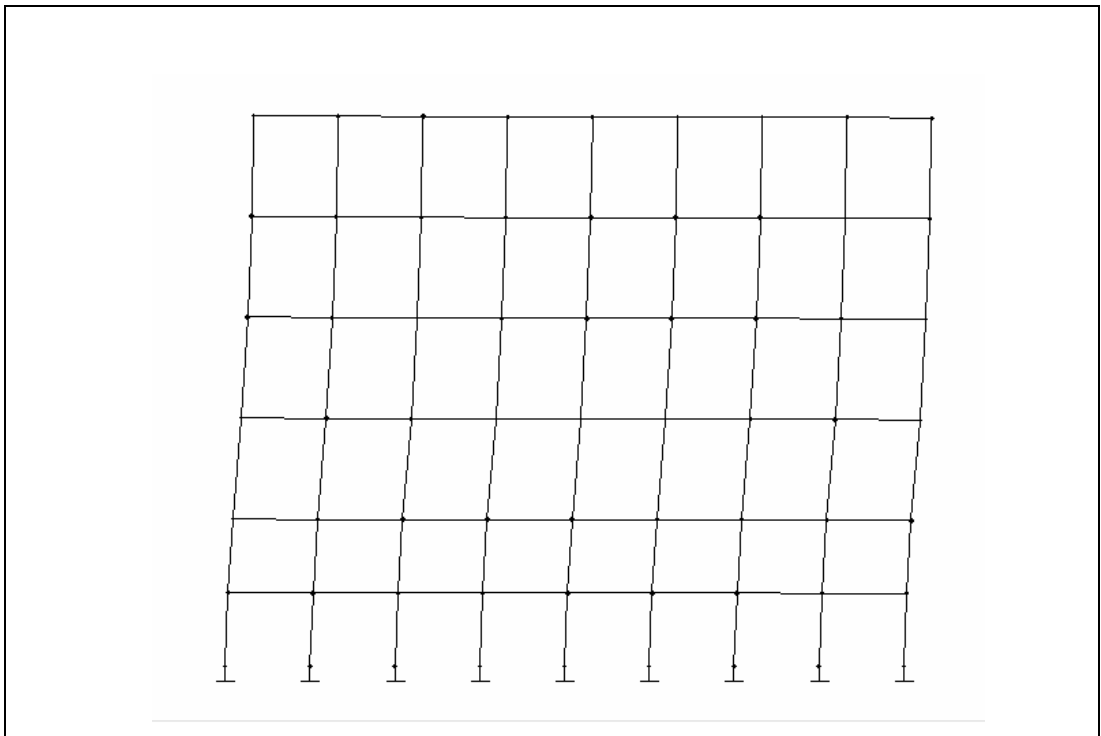
Figure 6.1 b) Second Mode of Vibration
