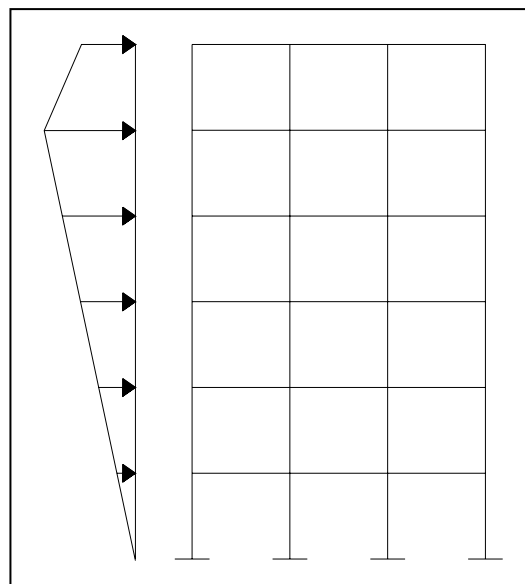
Figure 4.1 Load Pattern for Pushover Analysis
