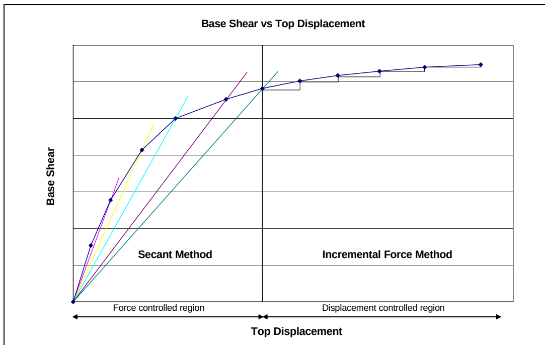
Figure 4.4 Constructing Capacity Curve
