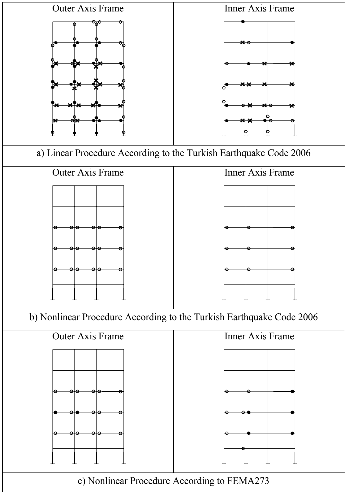
Figure 5.4 Existing System: Comparison of Element Sections Performance Levels, Immediate Occupancy Performance Level in x – Direction
