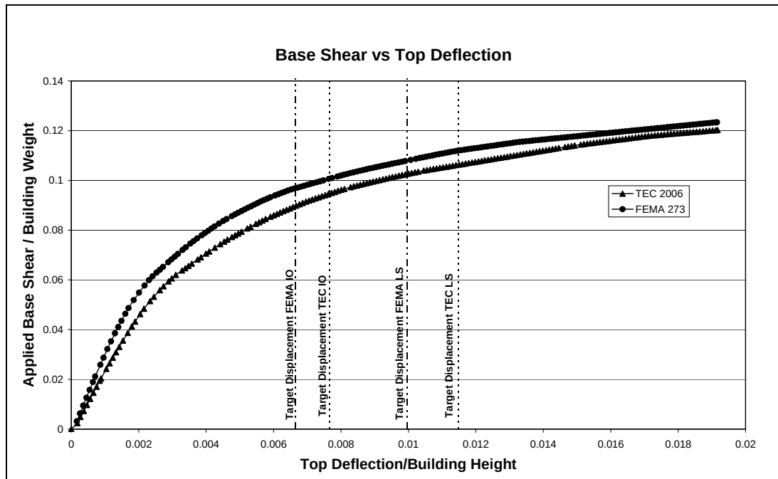
Figure 5.2 Existing System Pushover Analysis Result in x – Direction
