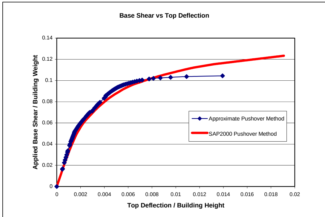
Figure 4.6 Existing System Verification of Pushover Curve in x - Direction
