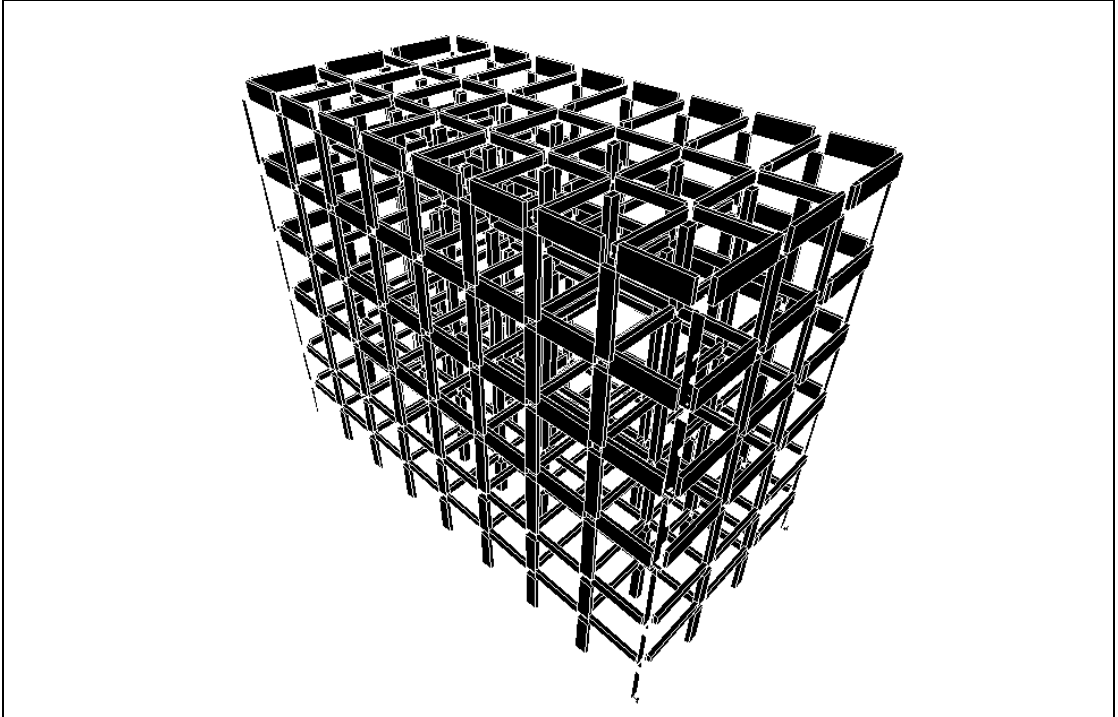
Figure 3.9 3-D View of the Existing System Model
