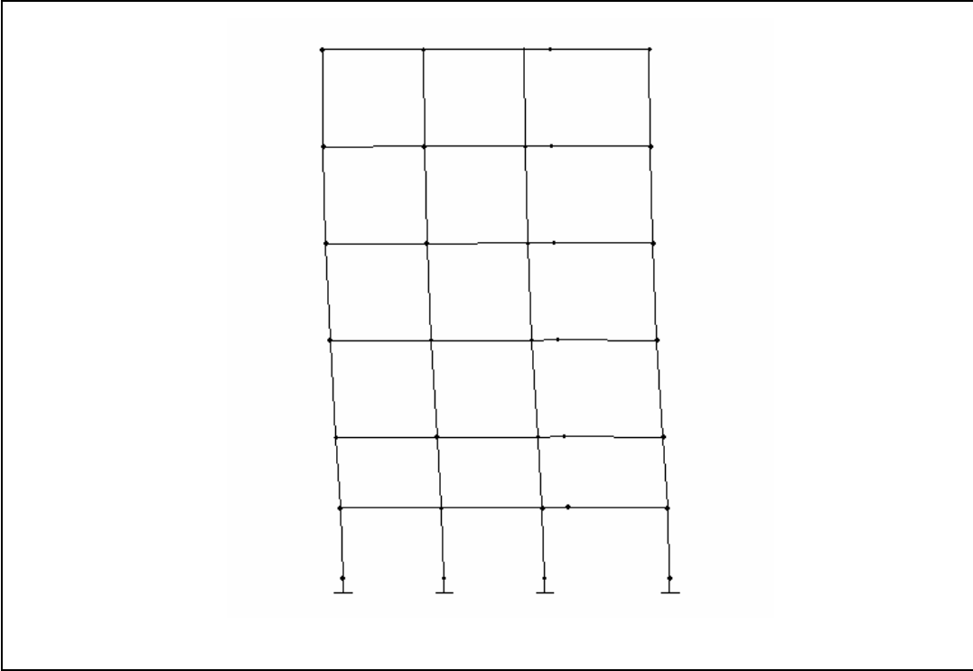
Figure 5.1 a) First Mode of Vibration
