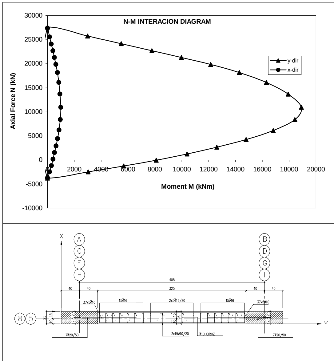
Figure A.7 Interaction Diagrams for Newly Added Shear Walls at 3 rd Storey on Axes A/B-5, C/D-5, F/G-5, H/I-5, A/B-8, C/D-8, F/G-8, H/I-8
