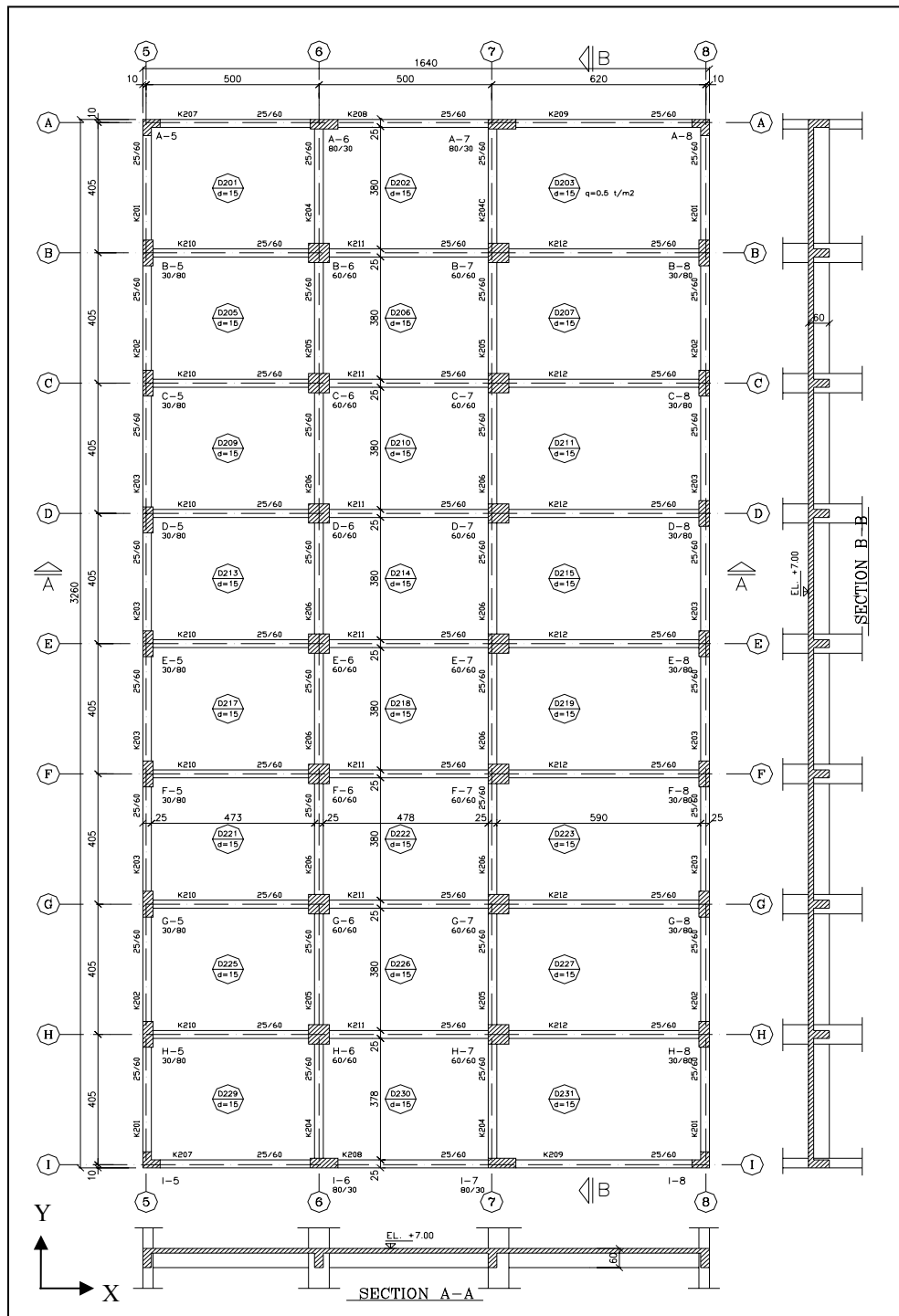
Figure 3.3 Existing System, Second Floor Plan
