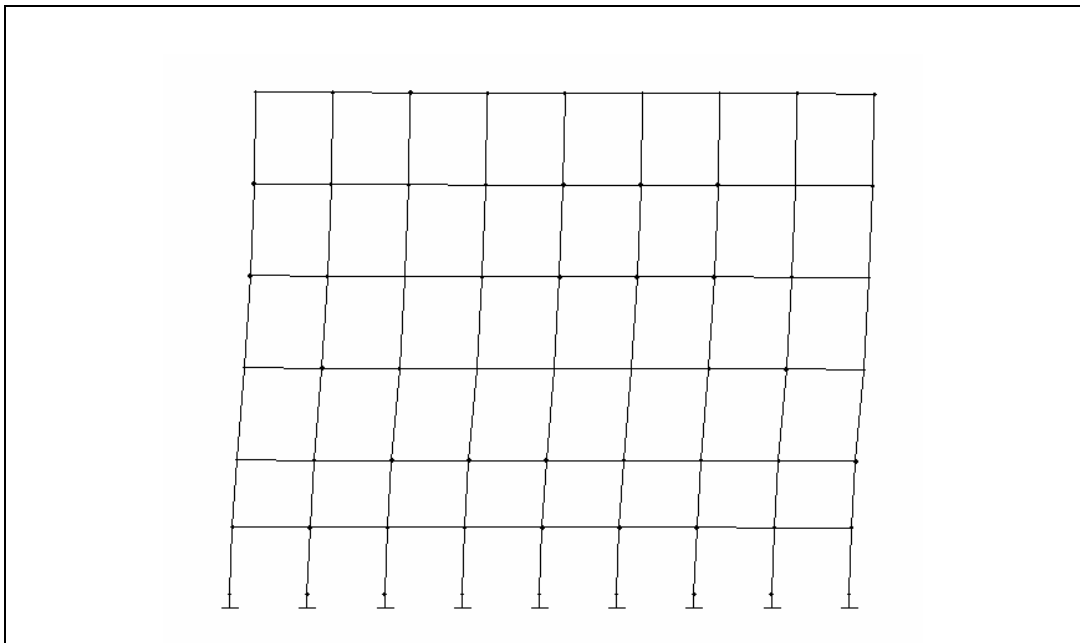
Figure 5.1 c) Third Mode of Vibration
