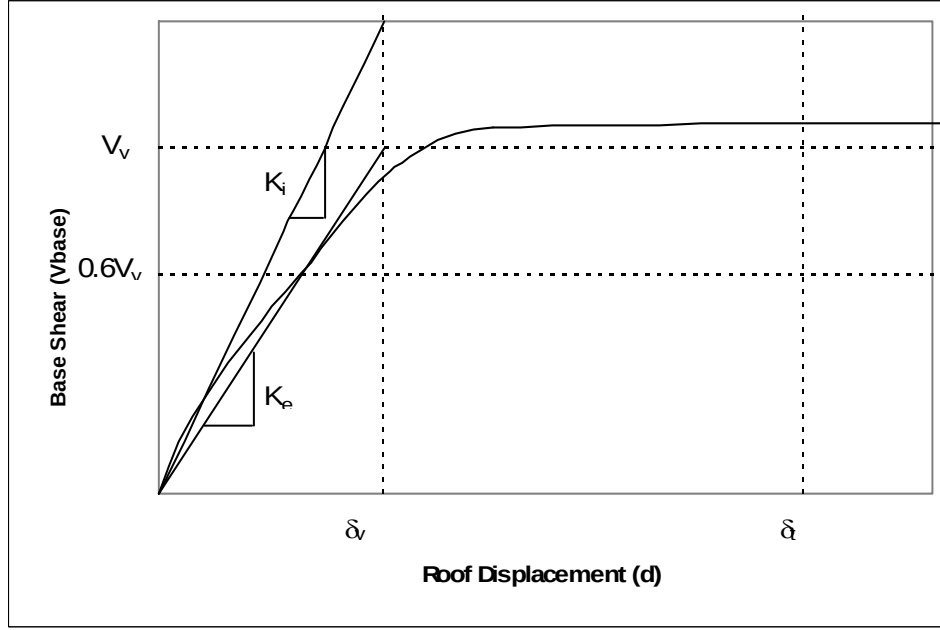
Figure 2.2 Bilinear Representation of Capacity Curve for Displacement Coefficient
