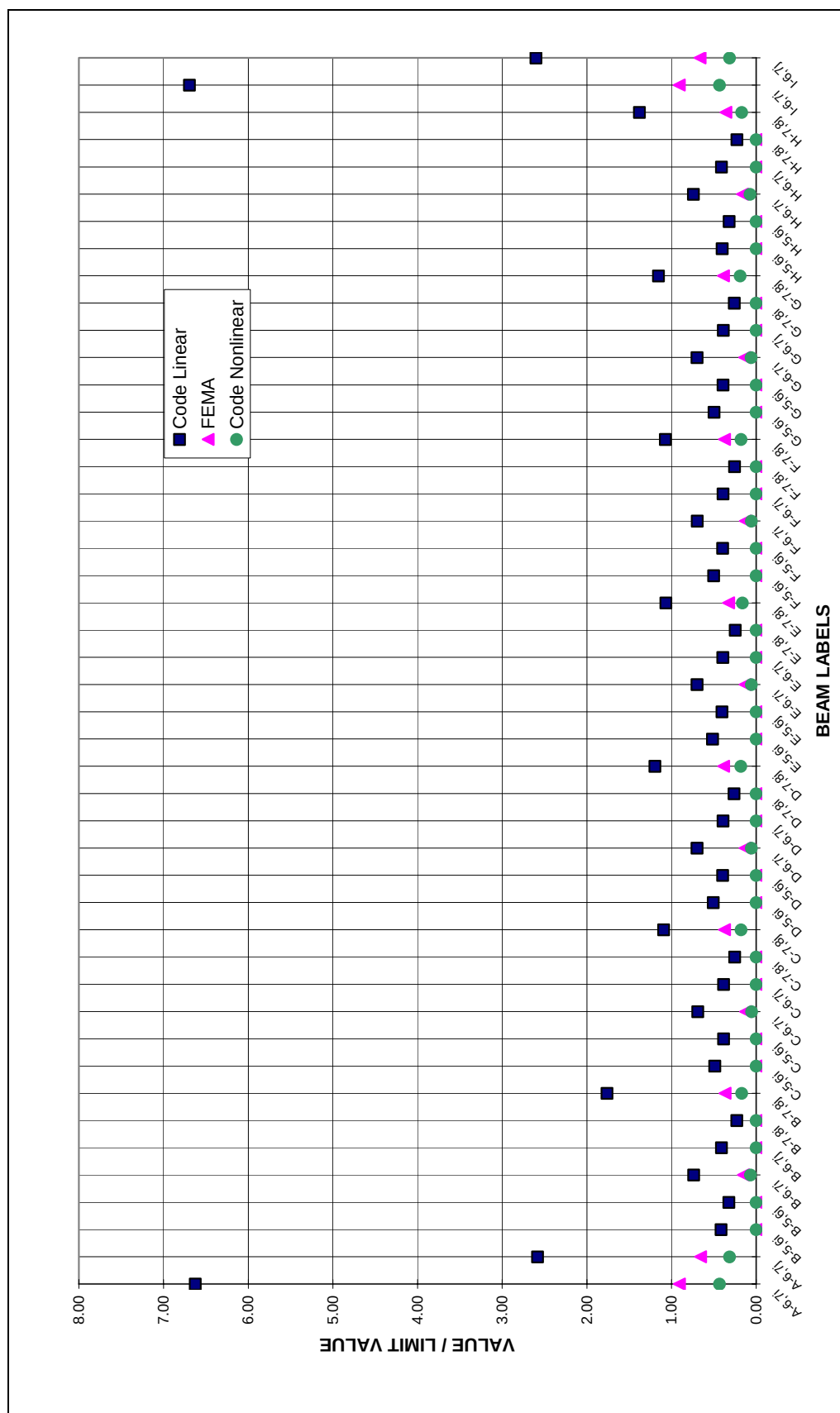
Figure C.3 Retrofitted System Life Safety Performance Level 3 rd Storey x – Direction Beams Performance Levels
