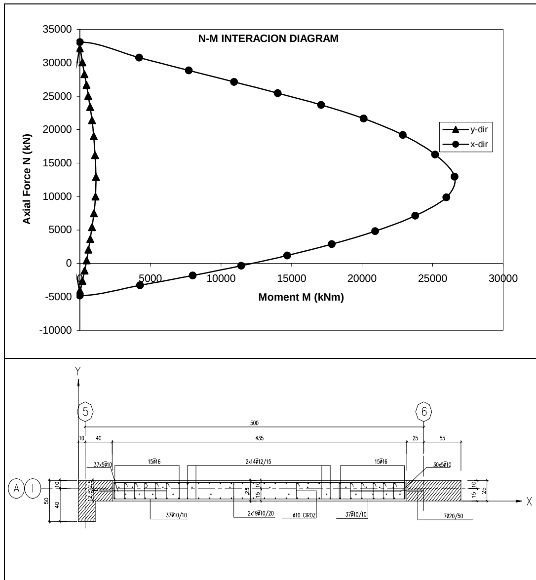
Figure A.5 Interaction Diagrams for Newly Added Shear Walls at 3 rd Storey on Axes A-5/6, I-5/6
