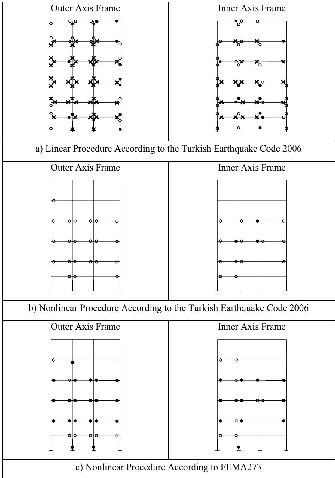
Figure 5.5 Existing System: Comparison of Element Sections Performance Levels, Life Safety Performance Level in x Direction
