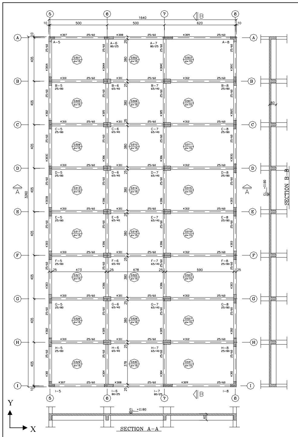
Figure 3.4 Existing System, Third, Fourth, Fifth and Sixth Floor Plans
