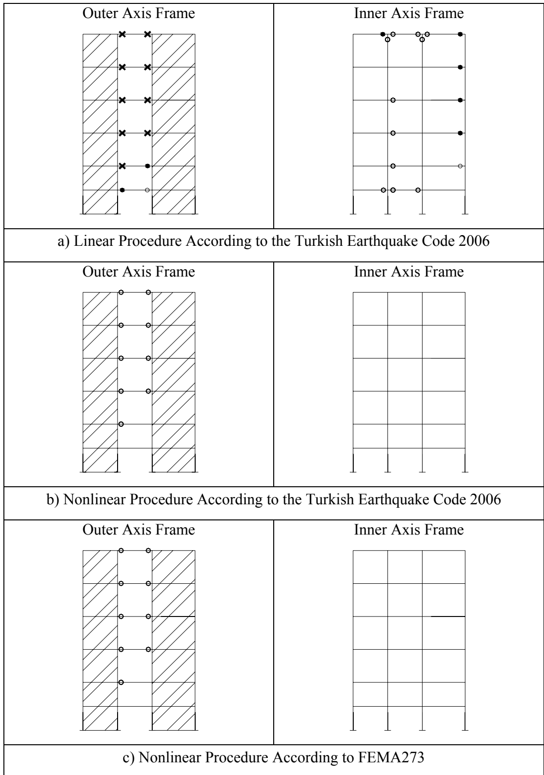
Figure 6.5 Retrofitted System: Comparison of Element Section Performance Levels, Life Safety Performance Level in x Direction
