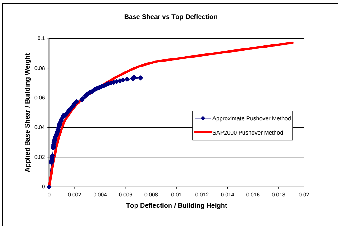
Figure 4.7 Existing System Verification of Pushover Curve in y - Direction
