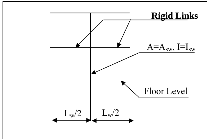
Figure 3.8 Shear Wall Model
