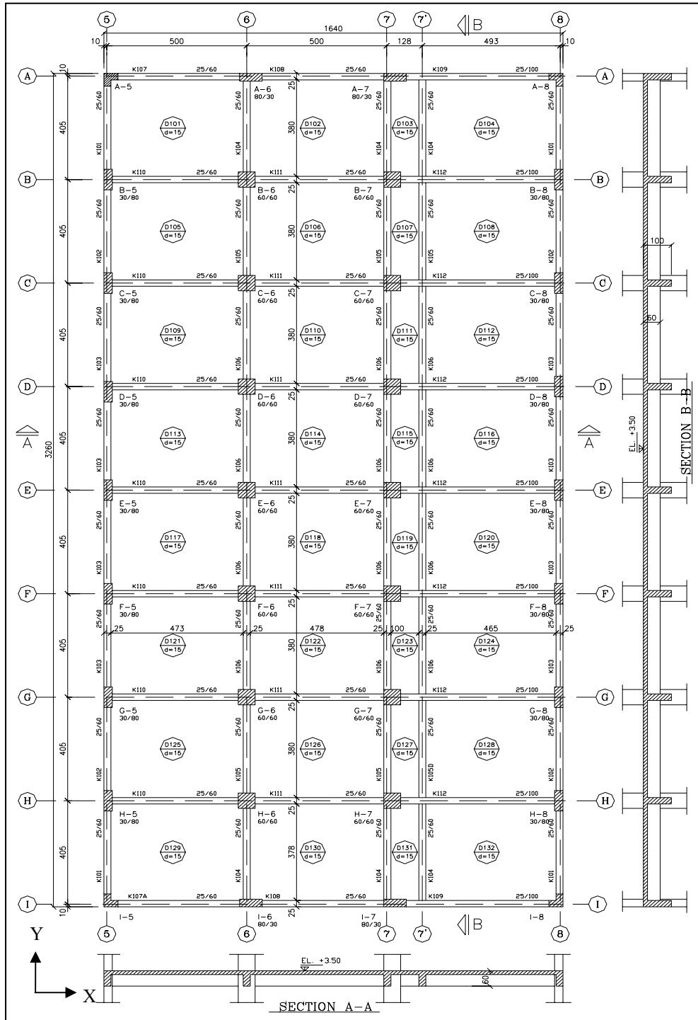
Figure 3.2. Existing System, First Floor Plan
