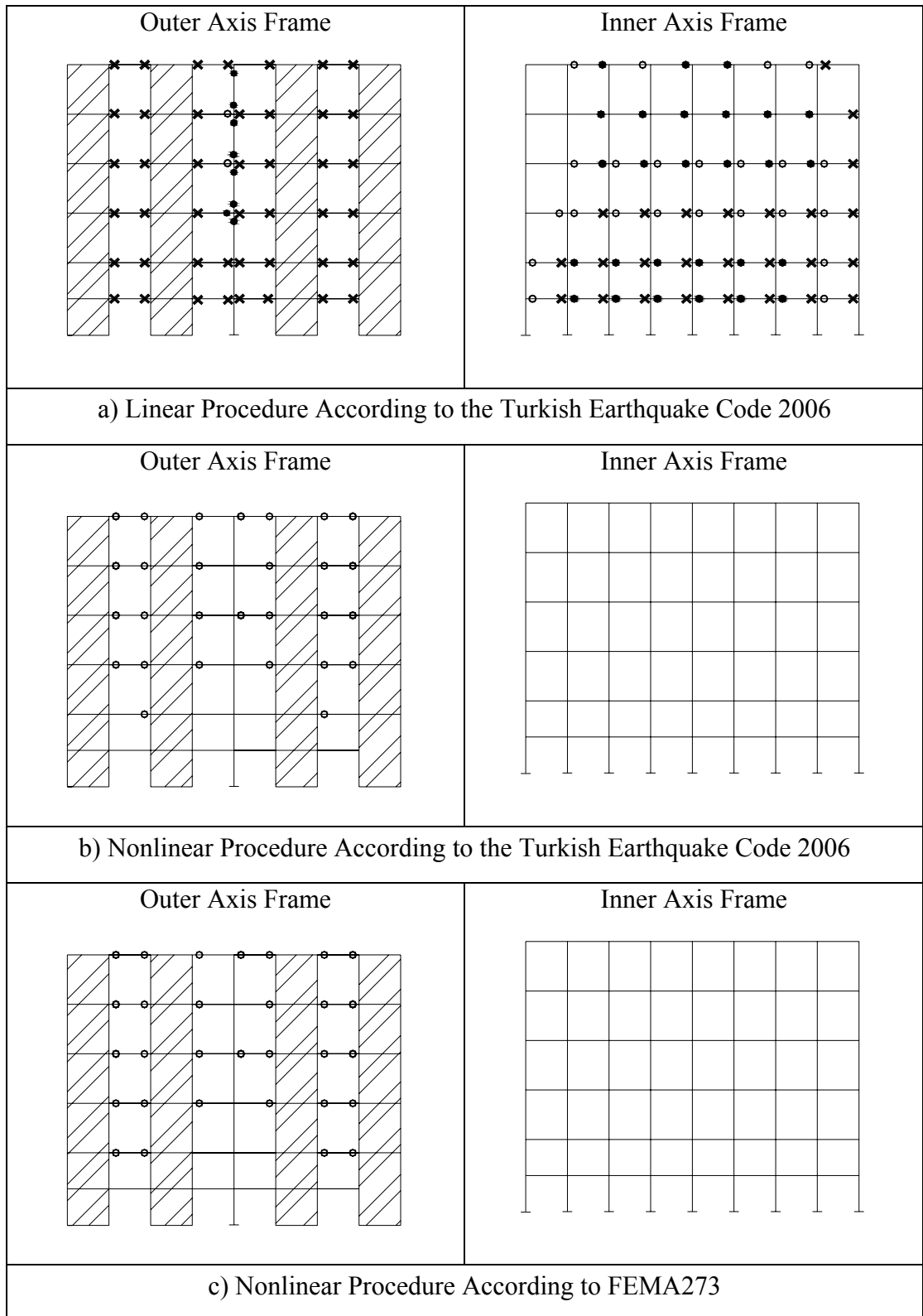
Figure 6.7 Retrofitted System: Comparison of Element Section Performance Levels, Life Safety Performance Level in y Direction
