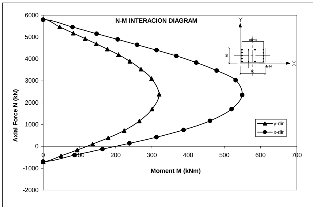
Figure A.4 Interaction Diagrams for Columns at 3 rd Storey on Axes B-7, C-7, D-7, E-7, F-7, G-7, H-7
