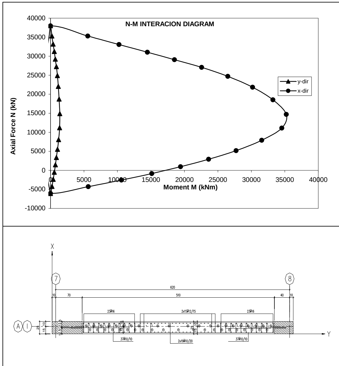
Figure A.6 Interaction Diagrams for Newly Added Shear Walls at 3 rd Storey on Axes A-7/8, I-7/8
