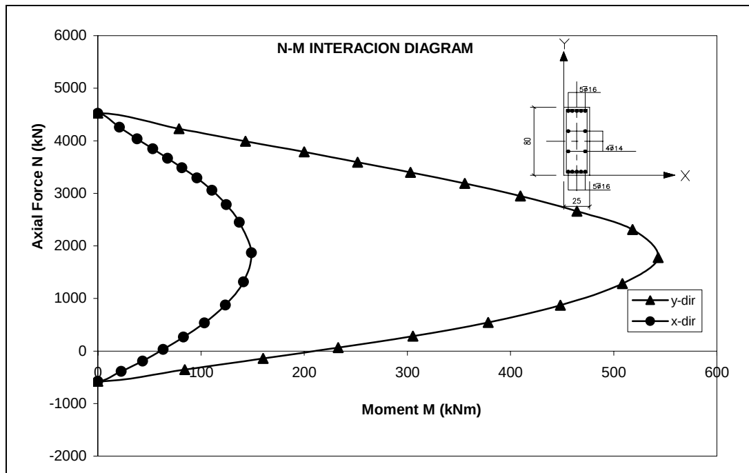
Figure A.1 Interaction Diagrams for Columns at 3 rd Storey on Axes B-5/8, C-5/8, D-5/8, E-5/8, F-5/8, G-5/8, H-5/8
