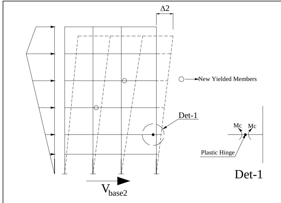
Figure 4.3 Introducing the Plastic Hinges
