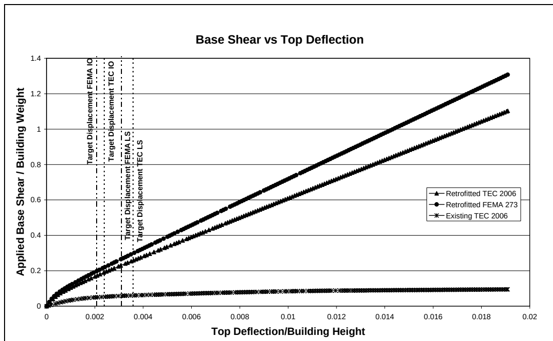
Figure 6.3 Retrofitted System Pushover Analysis Result in y-direction
