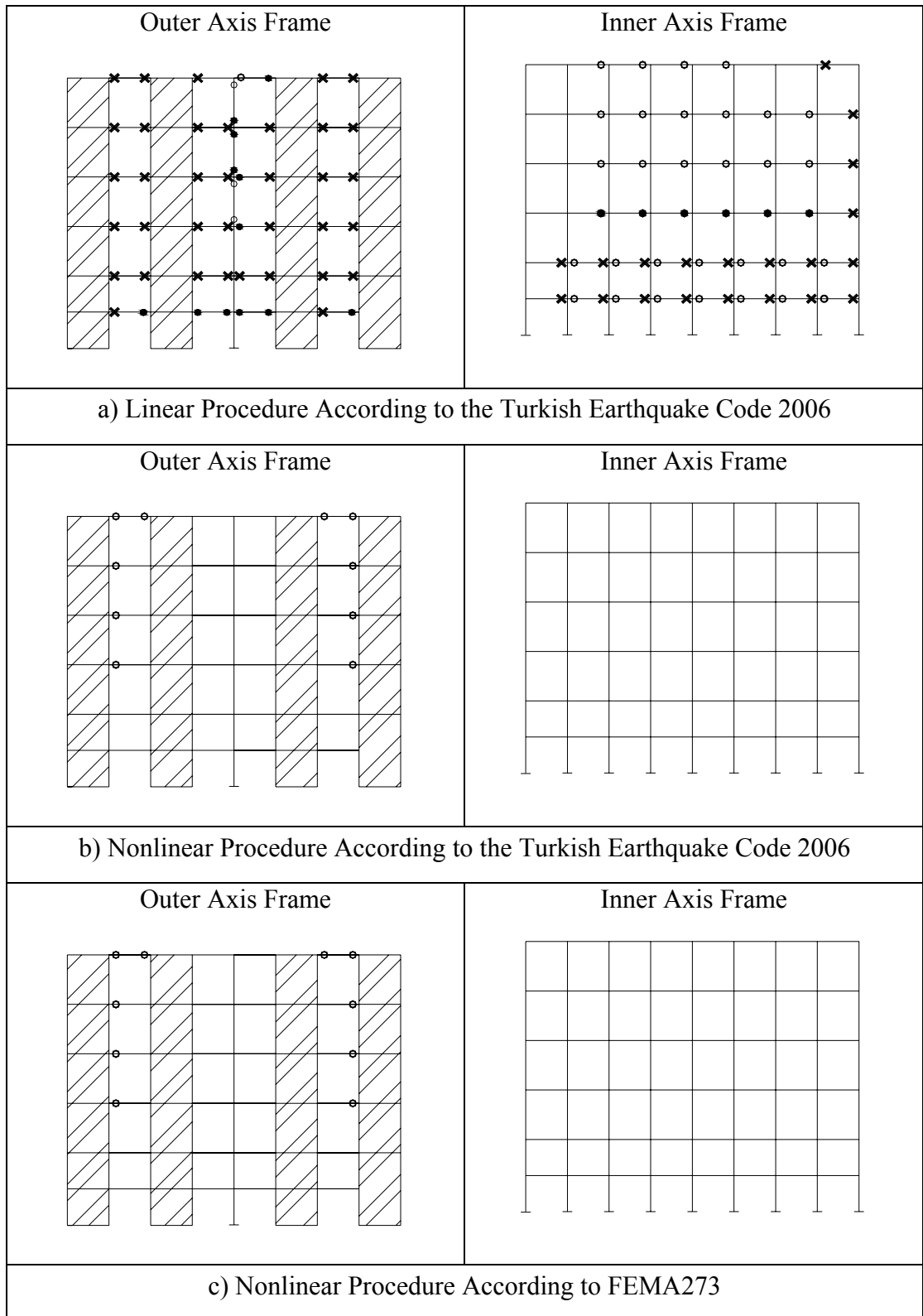
Figure 6.6 Retrofitted System: Comparison of Element Section Performance Levels, Immediate Occupancy Performance Level in y Direction
