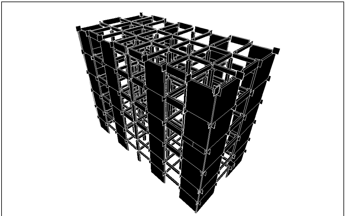
Figure 3.12 3-D View of the Retrofitted System Model
