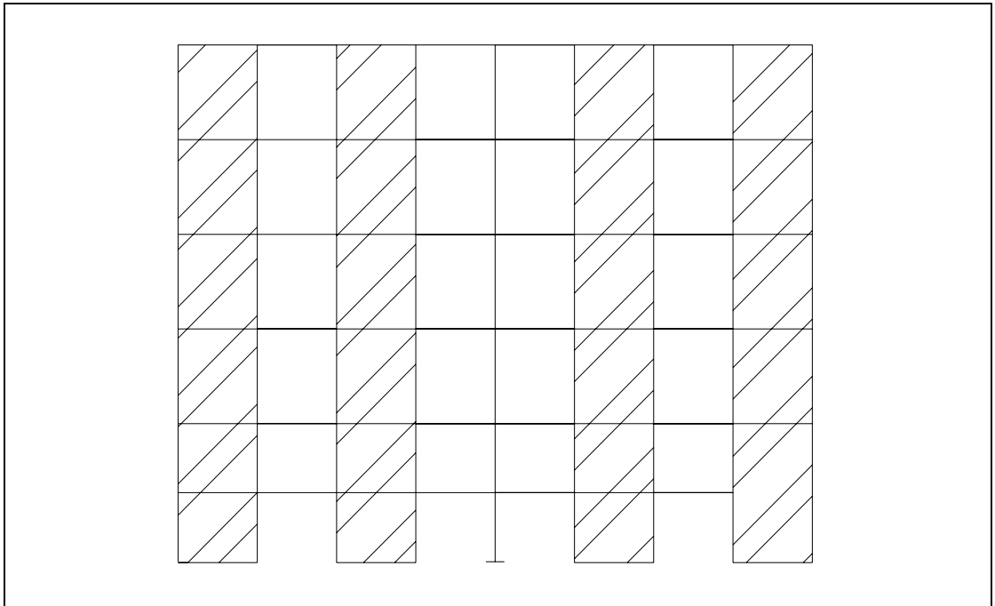
Figure 3.15 A Typical Exterior Frame in the y-Direction of the Retrofitted System Model
