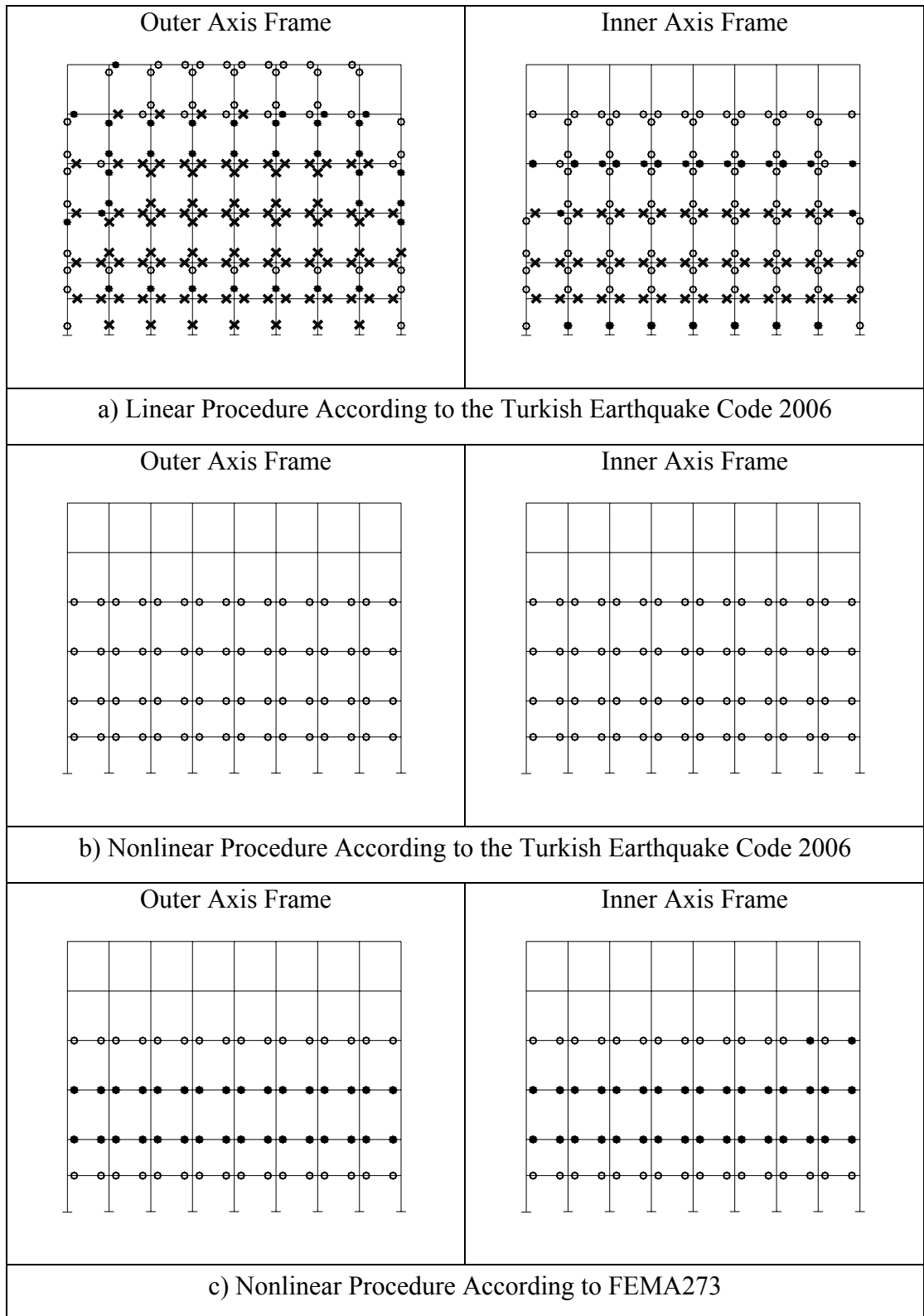
Figure 5.7 Existing System: Comparison of Element Sections Performance Levels, Life Safety Performance Level in y Direction
