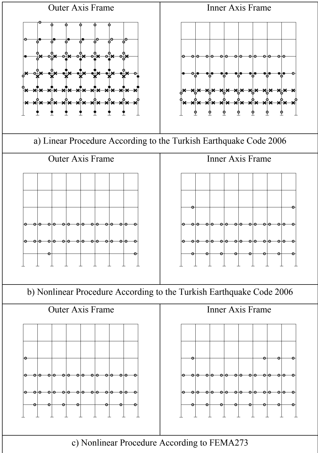
Figure 5.6 Existing System: Comparison of Element Sections Performance Levels, Immediate Occupancy Performance Level in y Direction
