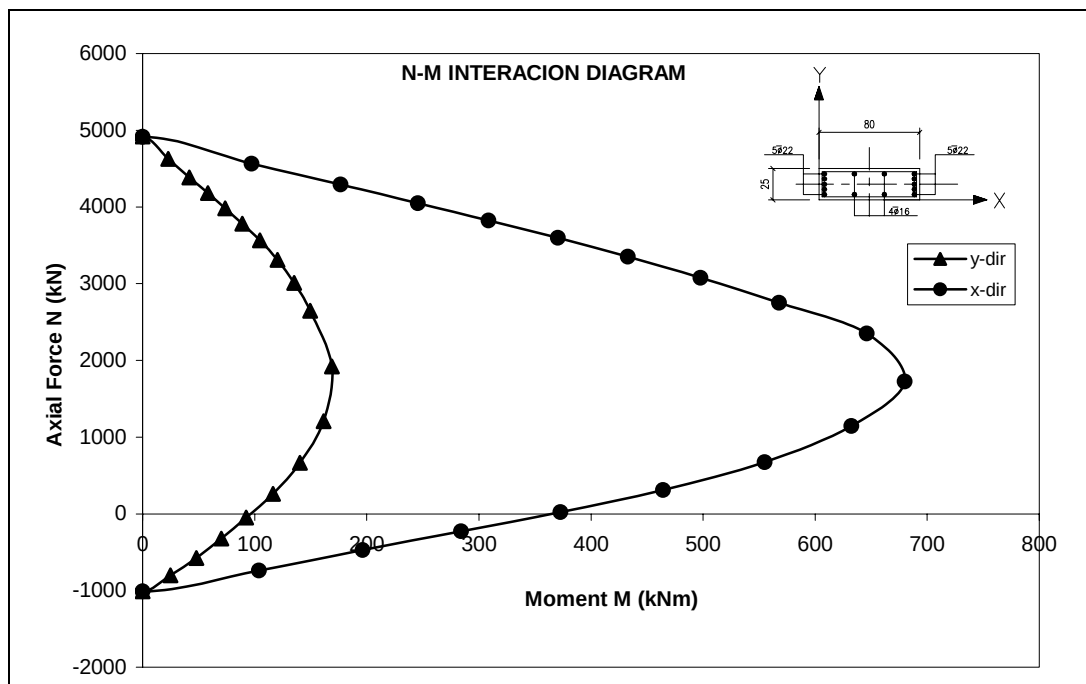
Figure A.2 Interaction Diagrams for Columns at 3 rd Storey on Axes A-6/7, I-6/7
