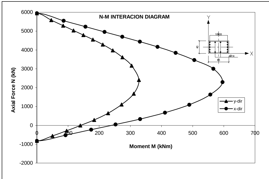
Figure A.3 Interaction Diagrams for Columns at 3 rd Storey on Axes B-6, C-6, D-6, E-6, F-6, G-6, H-6
