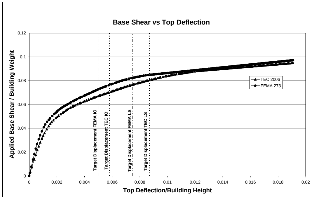
Figure 5.3 Existing System Pushover Analysis Result in y – Direction
