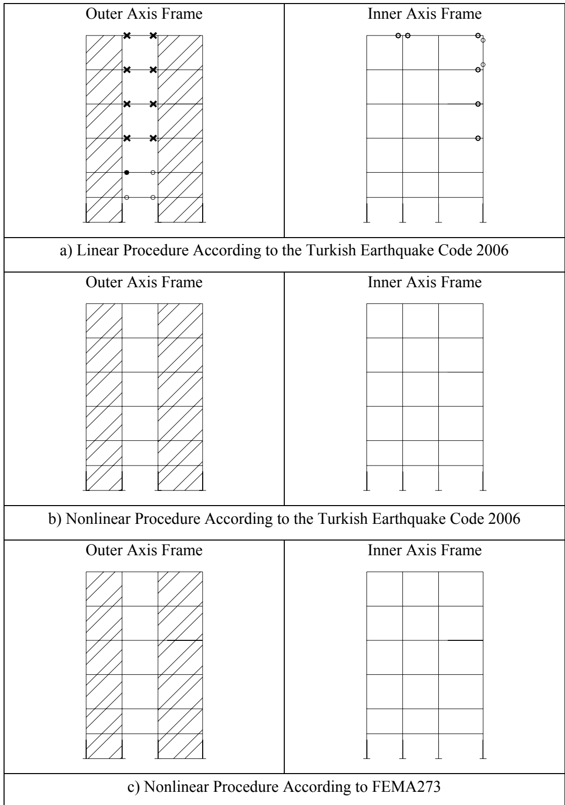
Figure 6.4 Retrofitted System: Comparison of Element Section Performance Levels, Immediate Occupancy Performance Level in x Direction
