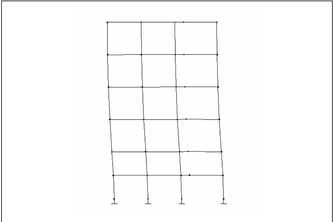
Figure 6.1 a) First Mode of Vibration
