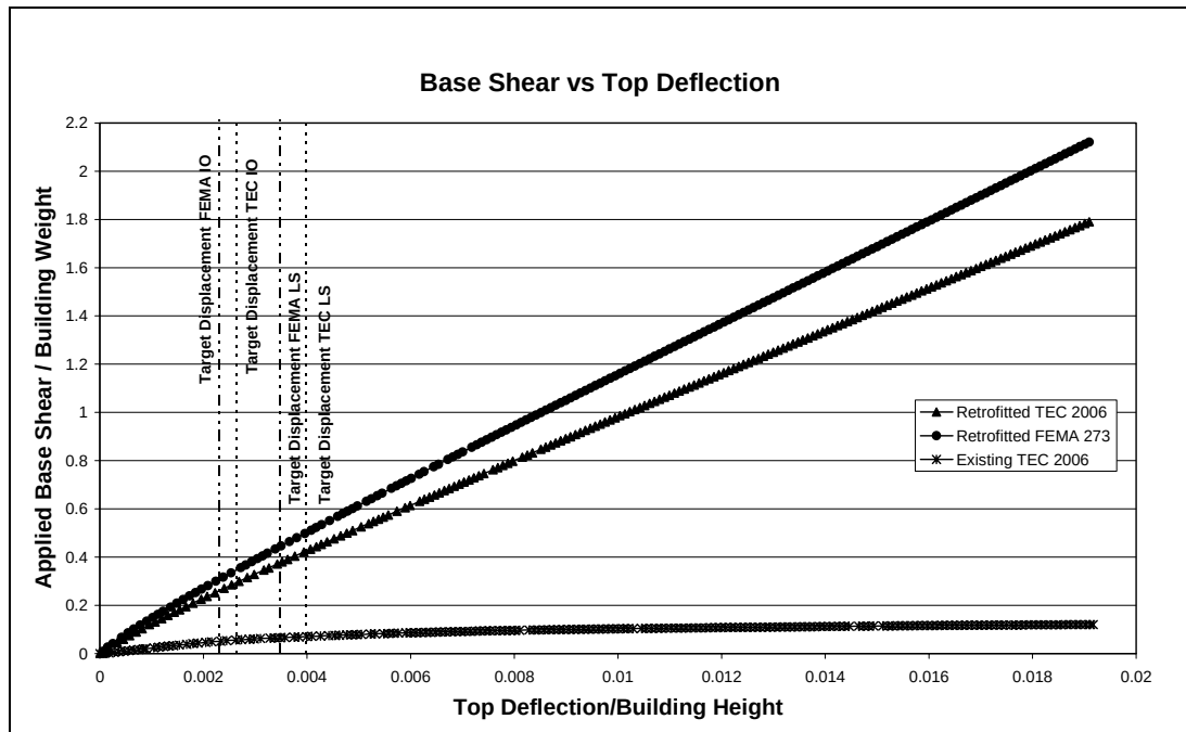
Figure 6.2 Retrofitted System Pushover Analysis Result in x-direction
