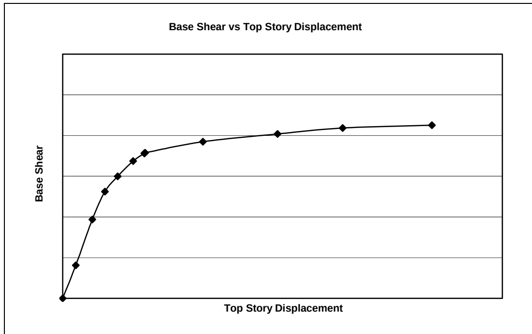
Figure 4.5 Capacity Curve
