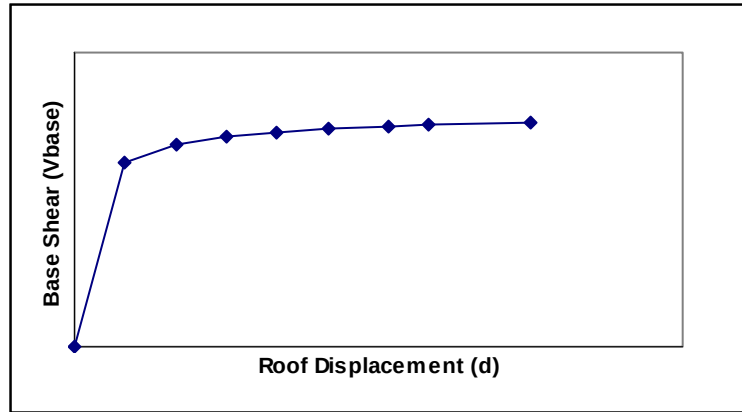
Figure 2.1 Typical Force–Displacement Relationship Obtained from Pushover Analysis
