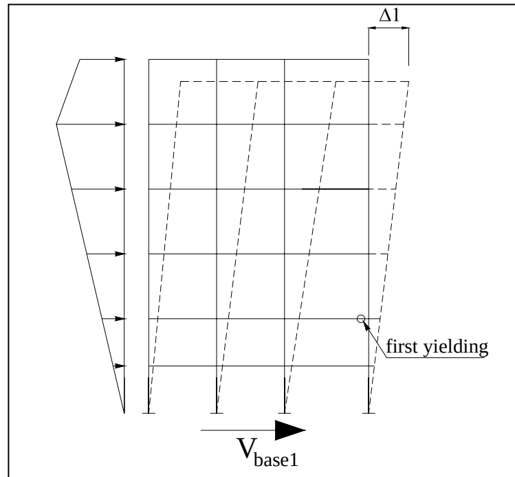
Figure 4.2 Adjust Total Base Shear for First Yielding
