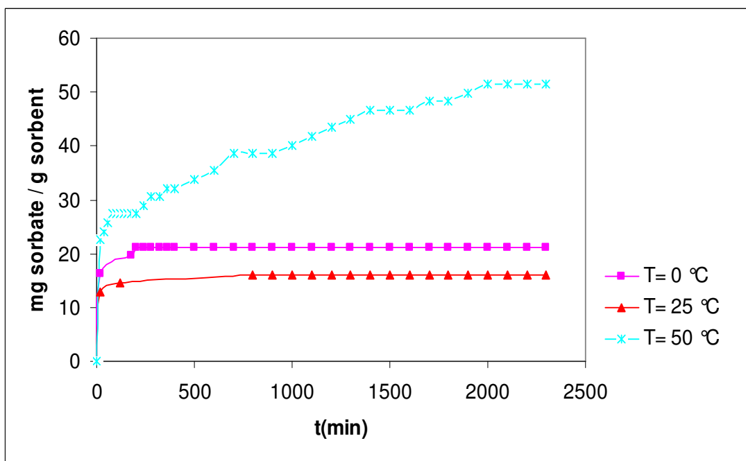
Figure 5.6 Propan-2-ol Uptake Curves in HZSM-35 at different temperatures ( P_{f,0^{\circ}\text{C}} = P_{o,0^{\circ}\text{C}} / 2 , P_{f,25^{\circ}\text{C}}, P_{f,50^{\circ}\text{C}} = P_{o,25^{\circ}\text{C}} / 2 )
