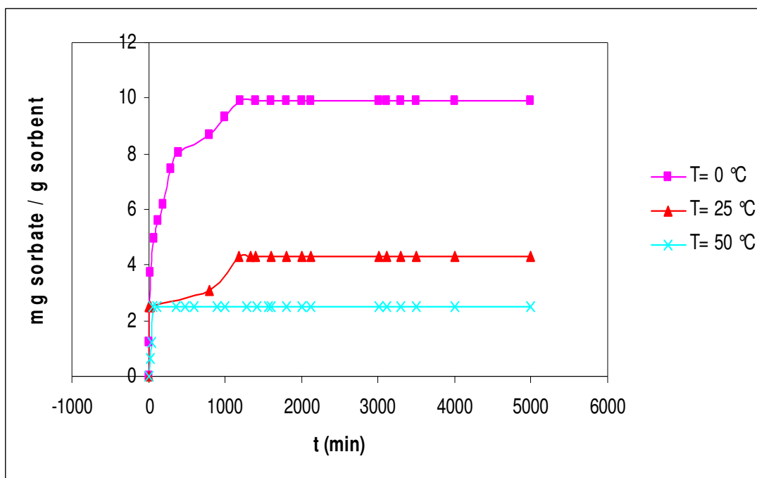
Figure 5.5 Propan-2-ol Uptake Curves in NaZSM-35 at different temperatures ( P_{f,0^{\circ}\text{C}} = P_{o,0^{\circ}\text{C}} / 2 , P_{f,25^{\circ}\text{C}}, P_{f,50^{\circ}\text{C}} = P_{o,25^{\circ}\text{C}} / 2 )
