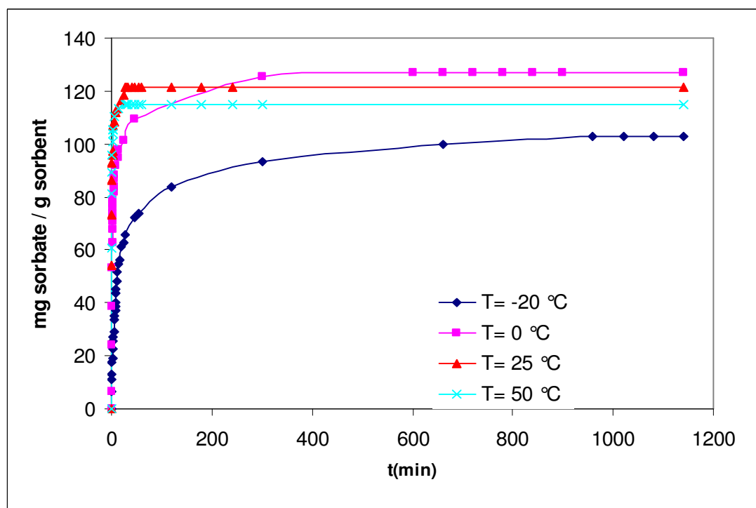
Figure 5.2. Ethanol Uptake Curves in HZSM-35 at different temperatures
