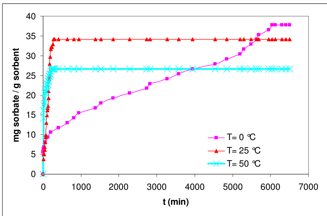
Figure 5.3 Propan-1-ol Uptake Curves in NaZSM-35 at different temperatures ( P_{f,0^{\circ}\text{C}} = P_{o,0^{\circ}\text{C}} / 2 , P_{f,25^{\circ}\text{C}}, 50^{\circ}\text{C}} = P_{o,25^{\circ}\text{C}} / 2 )
