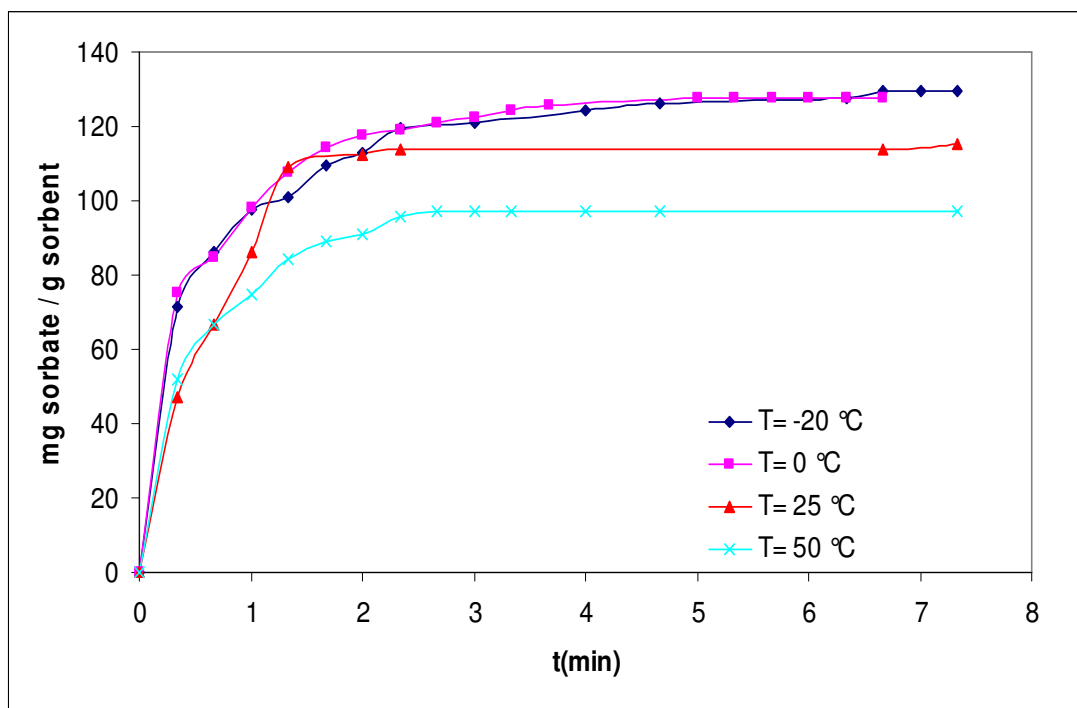
Figure 5.1 Methanol Uptake Curves in HZSM-35 at different temperatures
