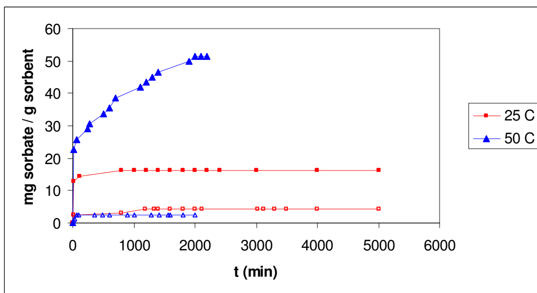
Figure 5.10 Propan-2-ol Uptake Curves in NaZSM-35 and HZSM-35 at T=25^{\circ}\text{C} and T=50^{\circ}\text{C} P_f = P_{o,25^{\circ}\text{C}} / 2 (Filled symbols denote H-ZSM35 and empty symbols denote Na-ZSM35)
