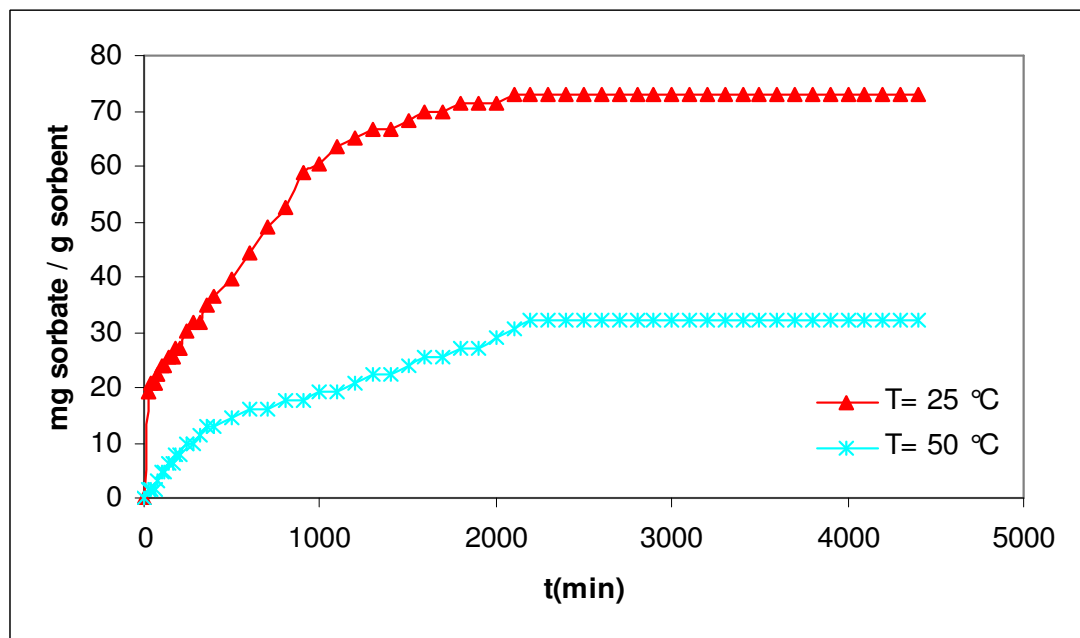
Figure 5.8 n-butanol Uptake Curves in HZSM-35 at different temperatures ( P_{f,0^{\circ}\text{C}} = P_{o,0^{\circ}\text{C}} / 2 , P_{f,25^{\circ}\text{C}}, P_{f,50^{\circ}\text{C}} = P_{o,25^{\circ}\text{C}} / 2 )
