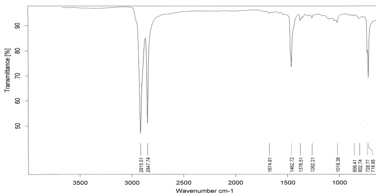
Figure 3.1 FTIR spectrum of neat HDPE
