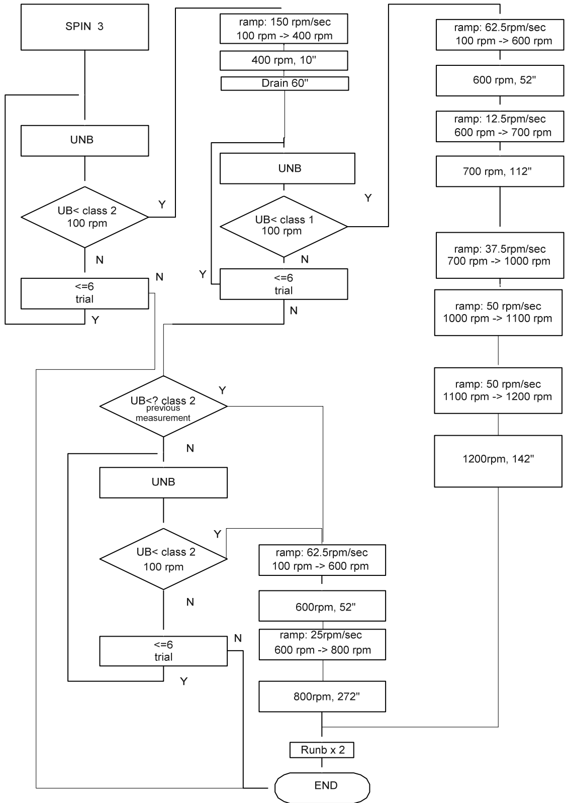
Figure 5.3 – Spin profile of a washing machine with an unbalanced load algorithm. UNB is the sub-profile containing the distributive motions and sensing at 100RPM. RUNB is the final distributive motion to prevent creasing in the laundry.
