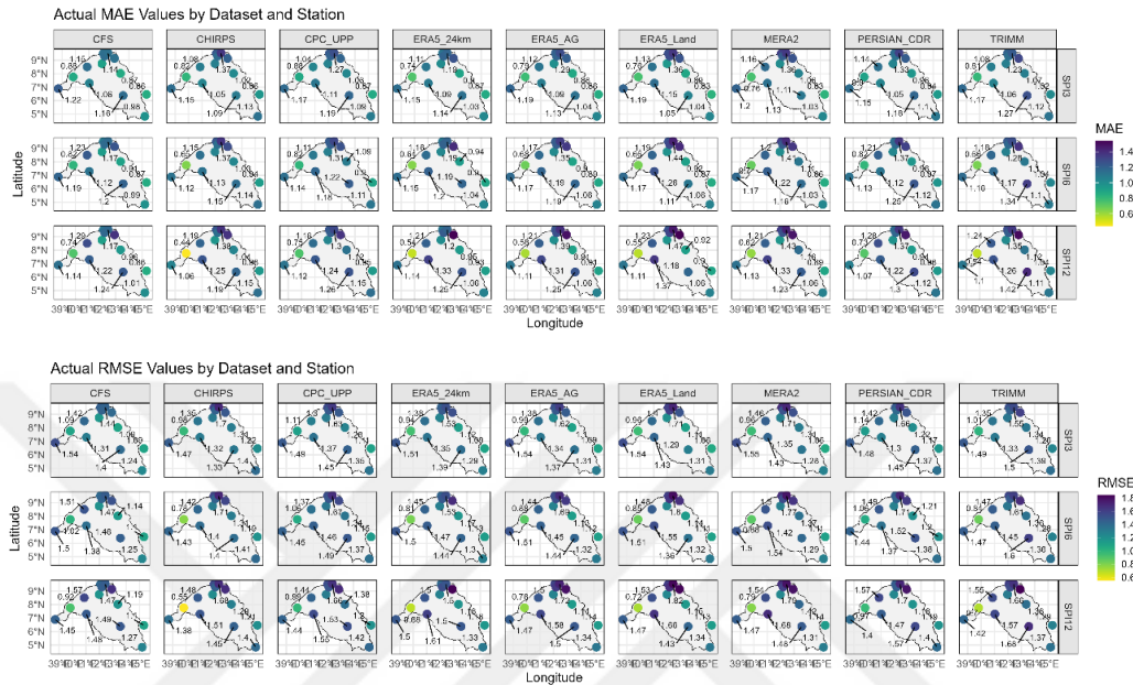
Figure 4.56. Continuous performance evaluation metrics (MAE and RMSE) of different station level
