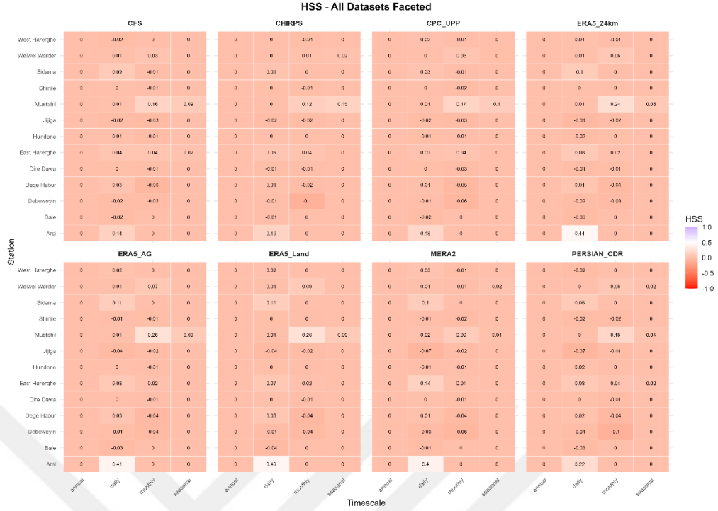
Figure 4.28. Heatmap evaluation of performance metrics (HSS) for temporal station level comparison across all datasets.
