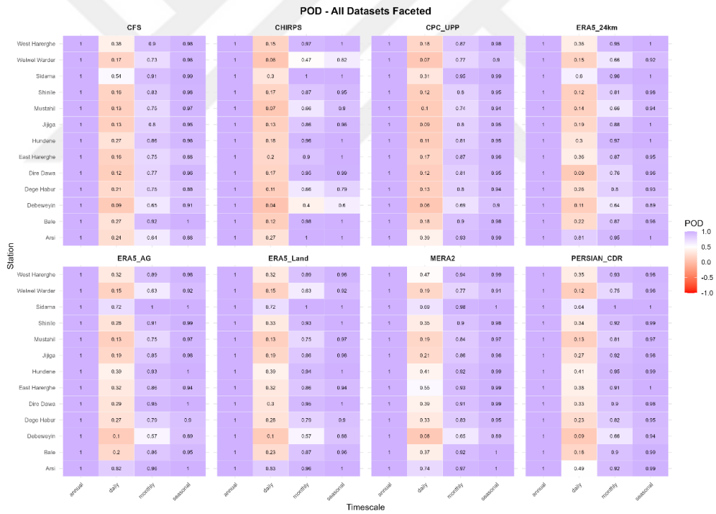
Figure 4.29. Heatmap evaluation of performance metrics (POD) for temporal station level comparison across all datasets.
