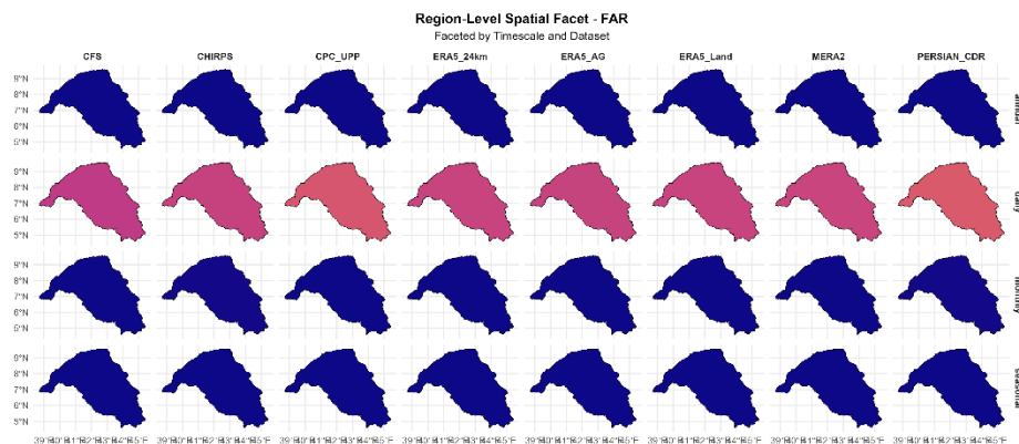
Figure 4.38. Spatio-temporal distribution of the False Alarm Ratio (FAR) for all datasets
