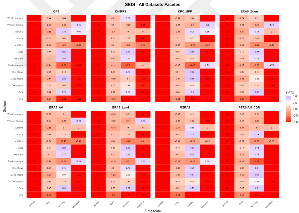
Figure 4.30. Heatmap evaluation of performance metrics (SEDI) for temporal station level comparison across all datasets
