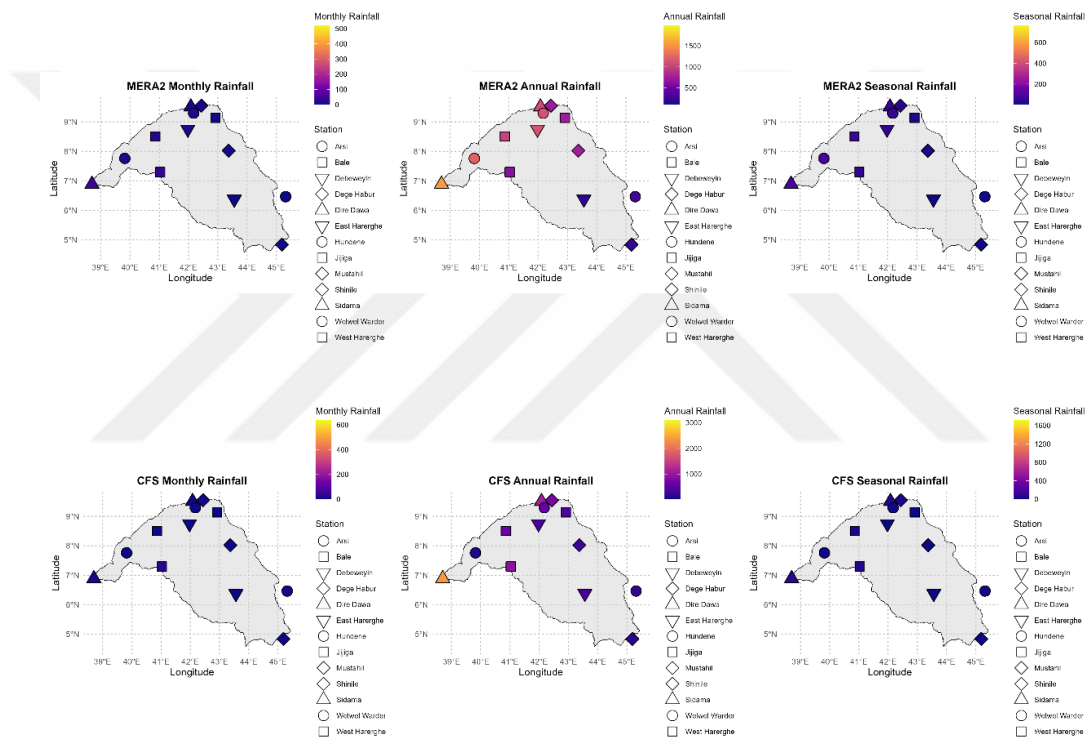
Figure 4.23. MERRA2 Monthly, seasonal and annual rainfall of different stations across Shabelle basin
