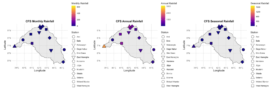
Figure 4.22. CFSR monthly, seasonal and annual rainfall of different stations across Shabelle basin
