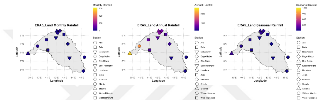
Figure 4.21. Monthly, seasonal and annual ERA5_Land precipitation observations across Shabelle Basin
