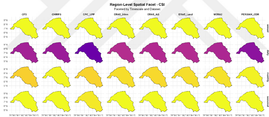
Figure 4.36. Spatio-temporal distribution of the Critical Success Index (CSI) for all datasets
