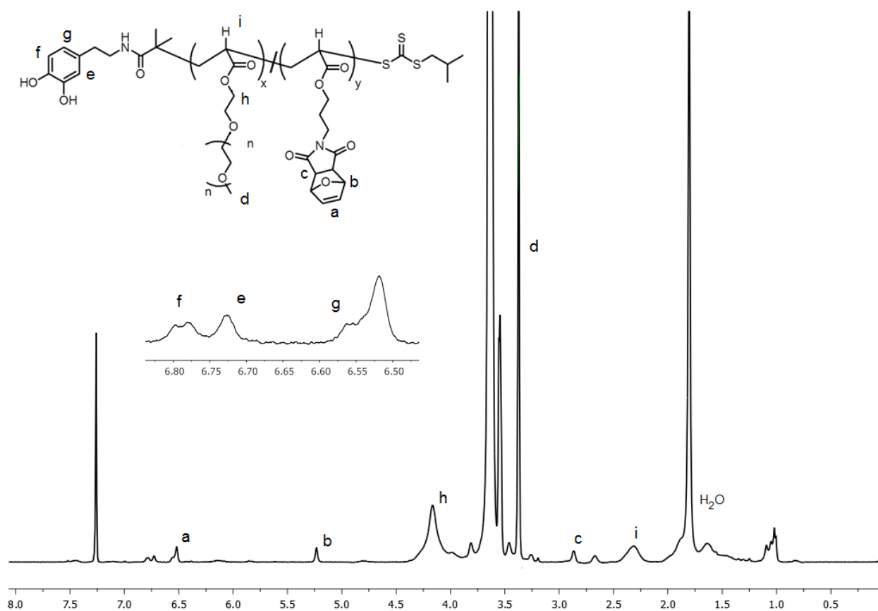
Figure 7.8. Representative ^1\text{H} NMR spectrum of catechol end-functionalized furan protected maleimide group containing copolymer FuMAP2.
