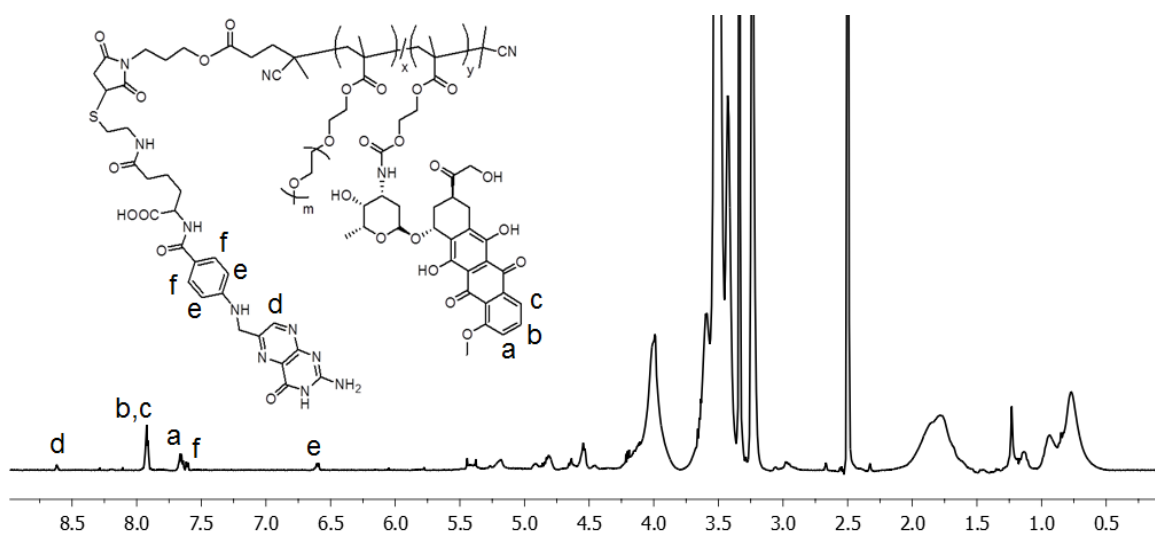
Figure 8.16. ^1\text{H} NMR spectrum of FA-SH conjugated copolymer F-P-Dox.
