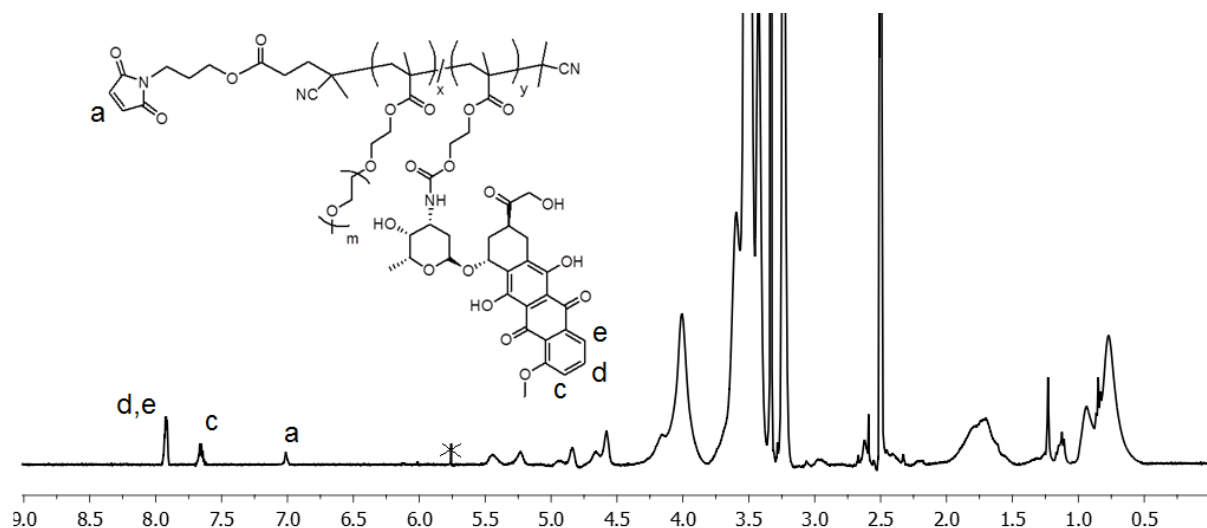
Figure 8.14. 1 H NMR spectrum of Dox-conjugated copolymer M-P-Dox.
