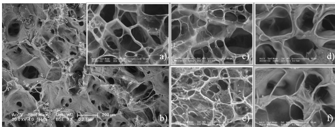
Figure 4.4. Representative ESEM images of freeze-dried hydrogels: a, b) P4CD (1:1) , c) P2CD (1:1) , d) P8CD (1:1) , e) P4CD (2:1) , f) P4CD (1:2) . Large image scale bar: 200 \mu\text{m} ; small images: 50 \mu\text{m} .
